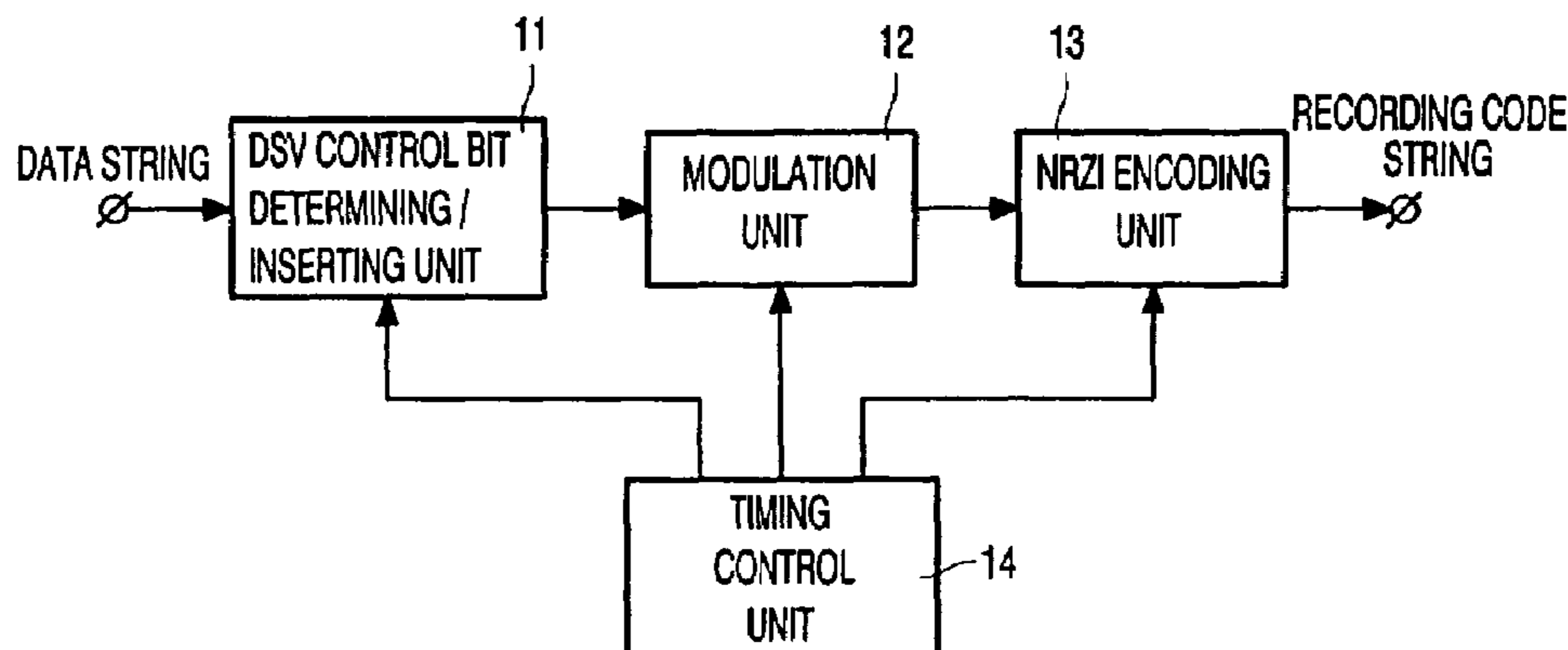
MODULATION APPARATUS 1
