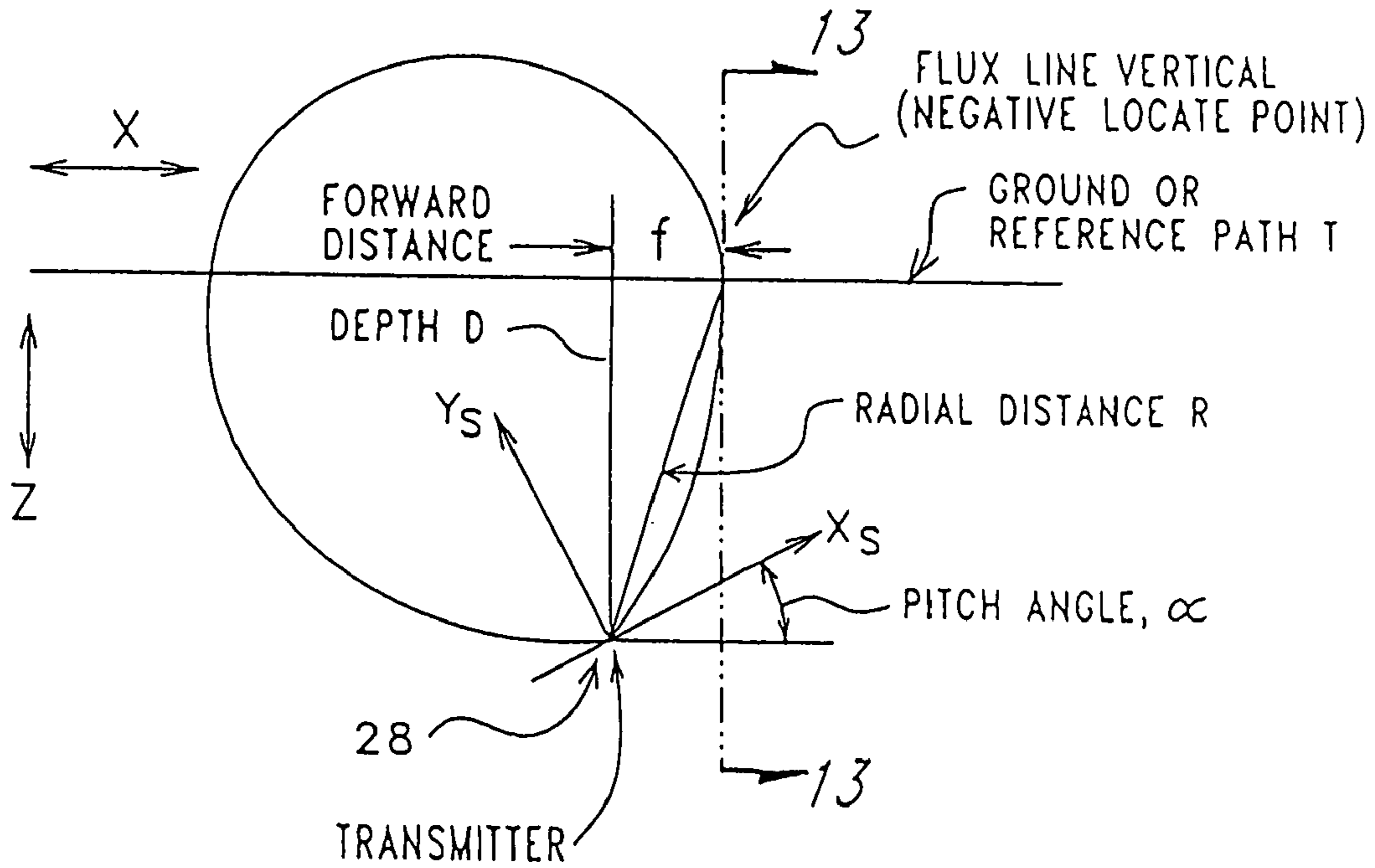
SIDE VIEW FIG. 12
