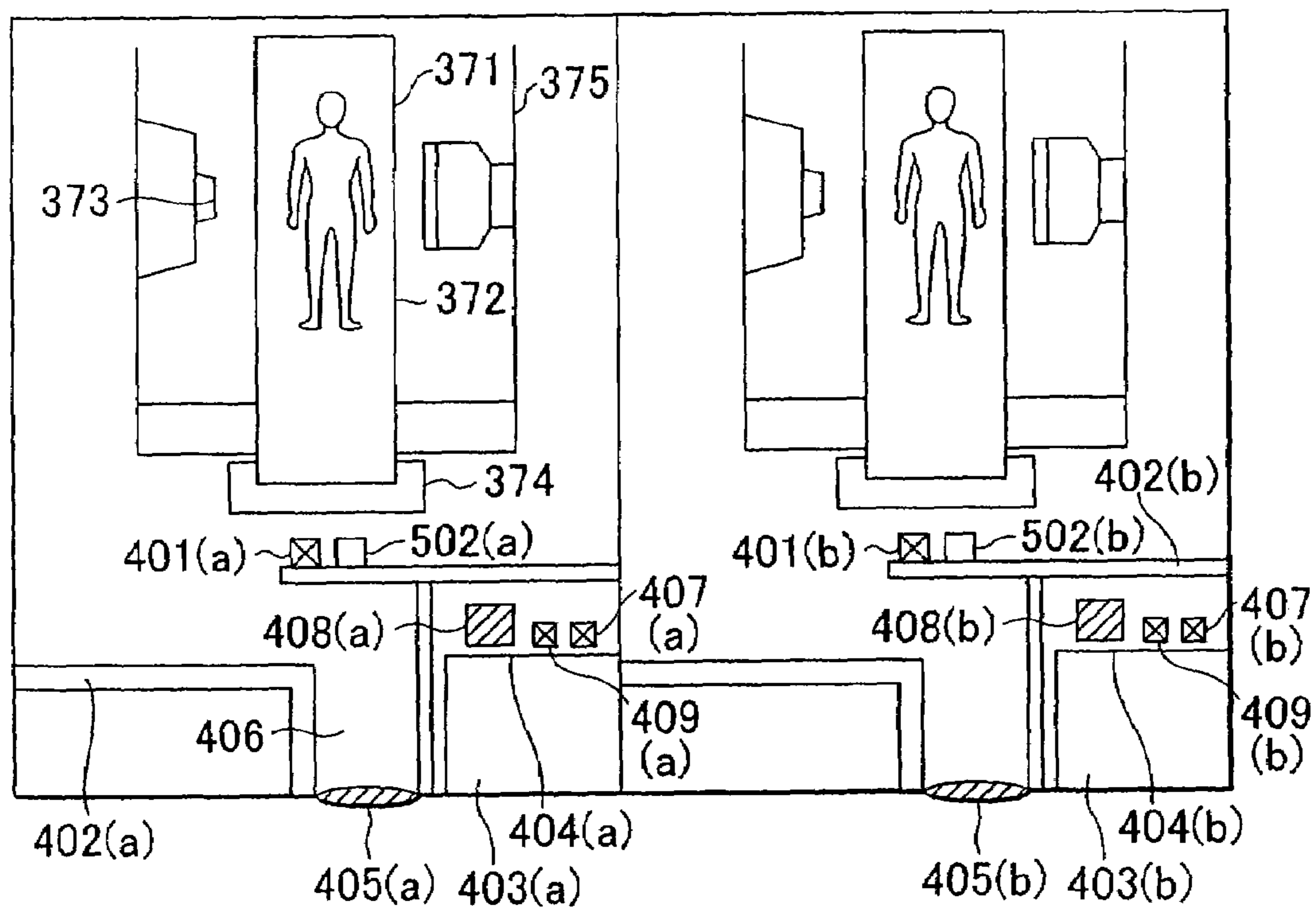
16(a):IRRADIATION ROOM 1
