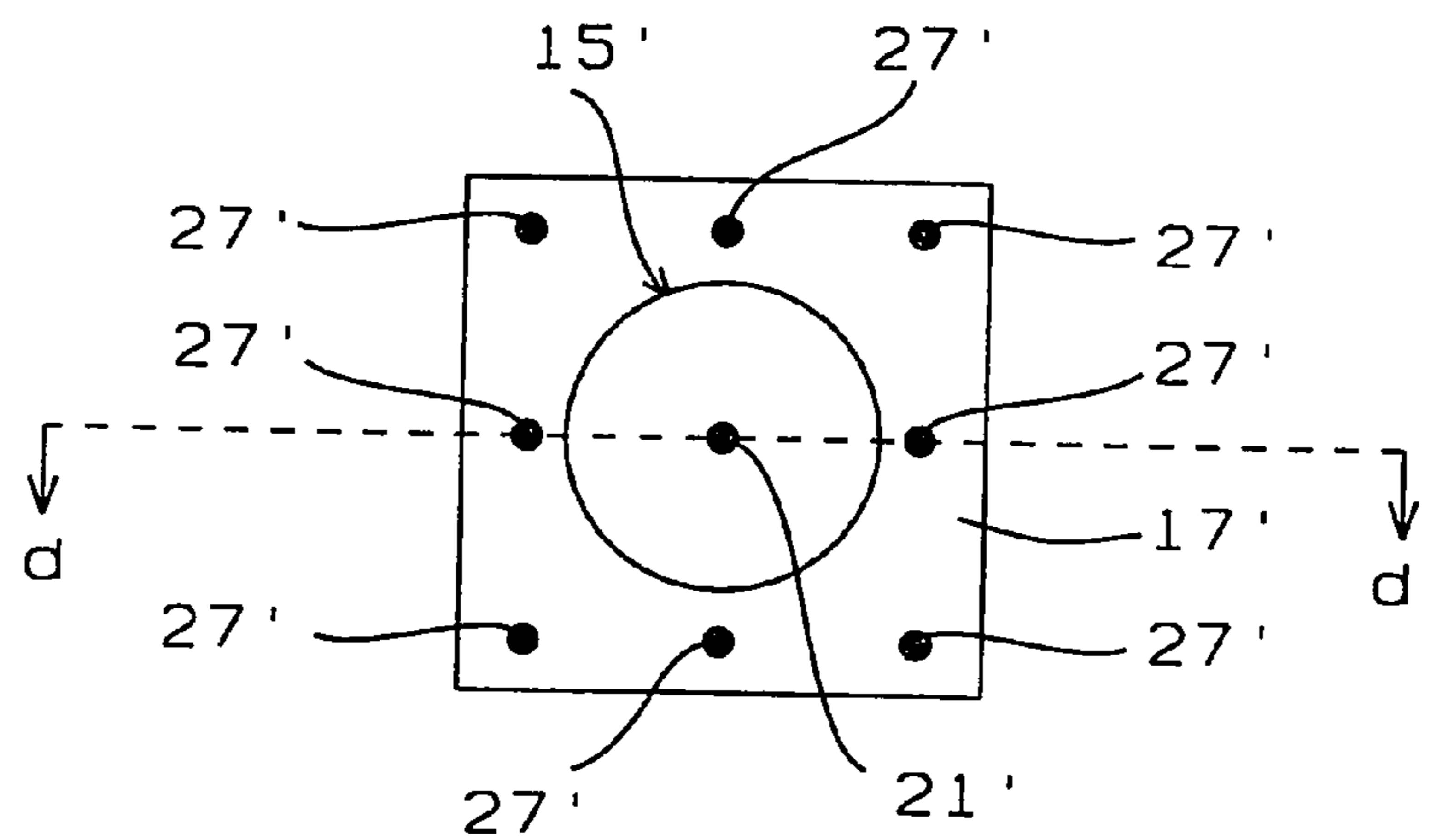
FIG. 20c - Prior Art
