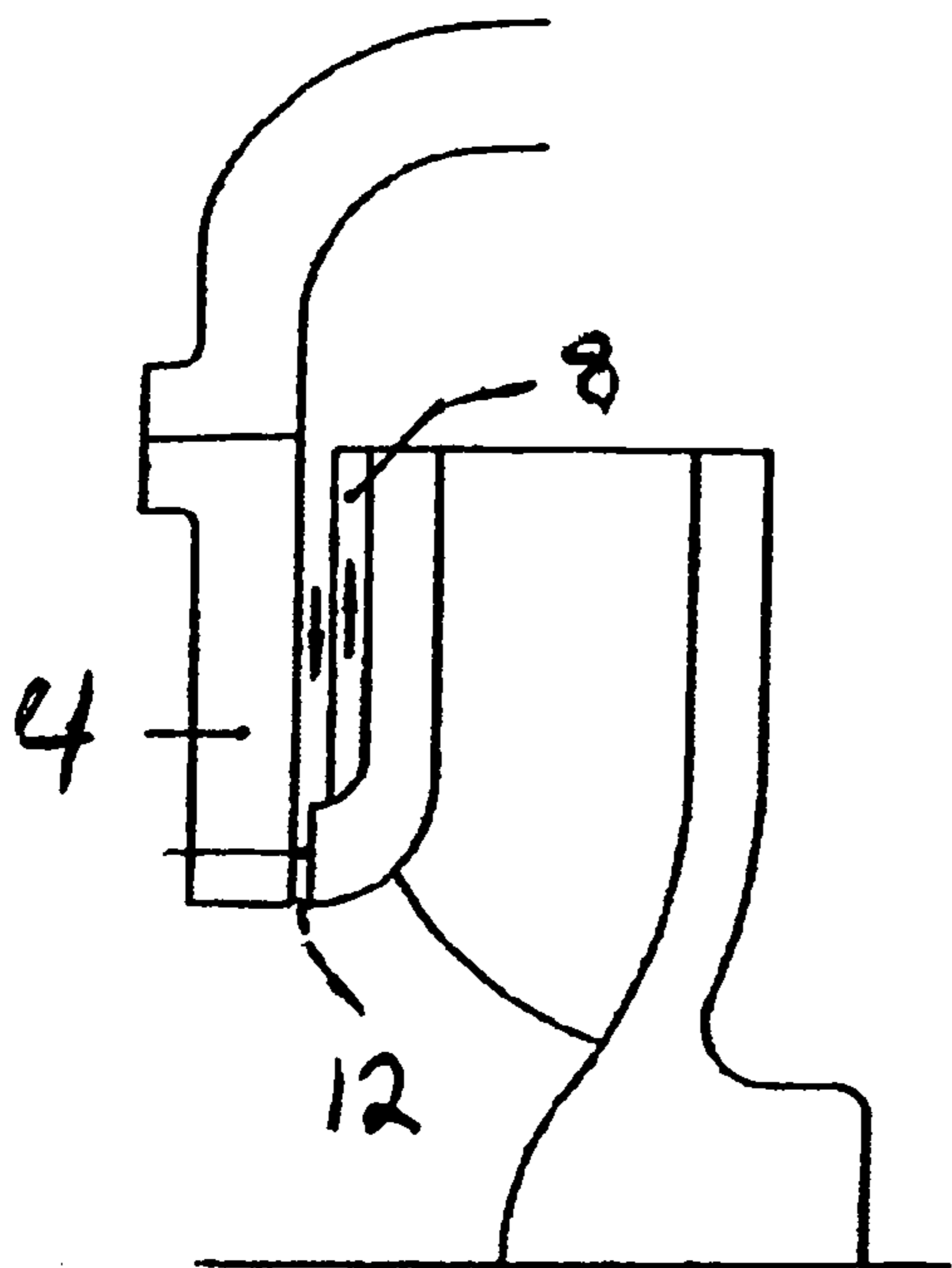
FIG. 5 PRIOR ART
