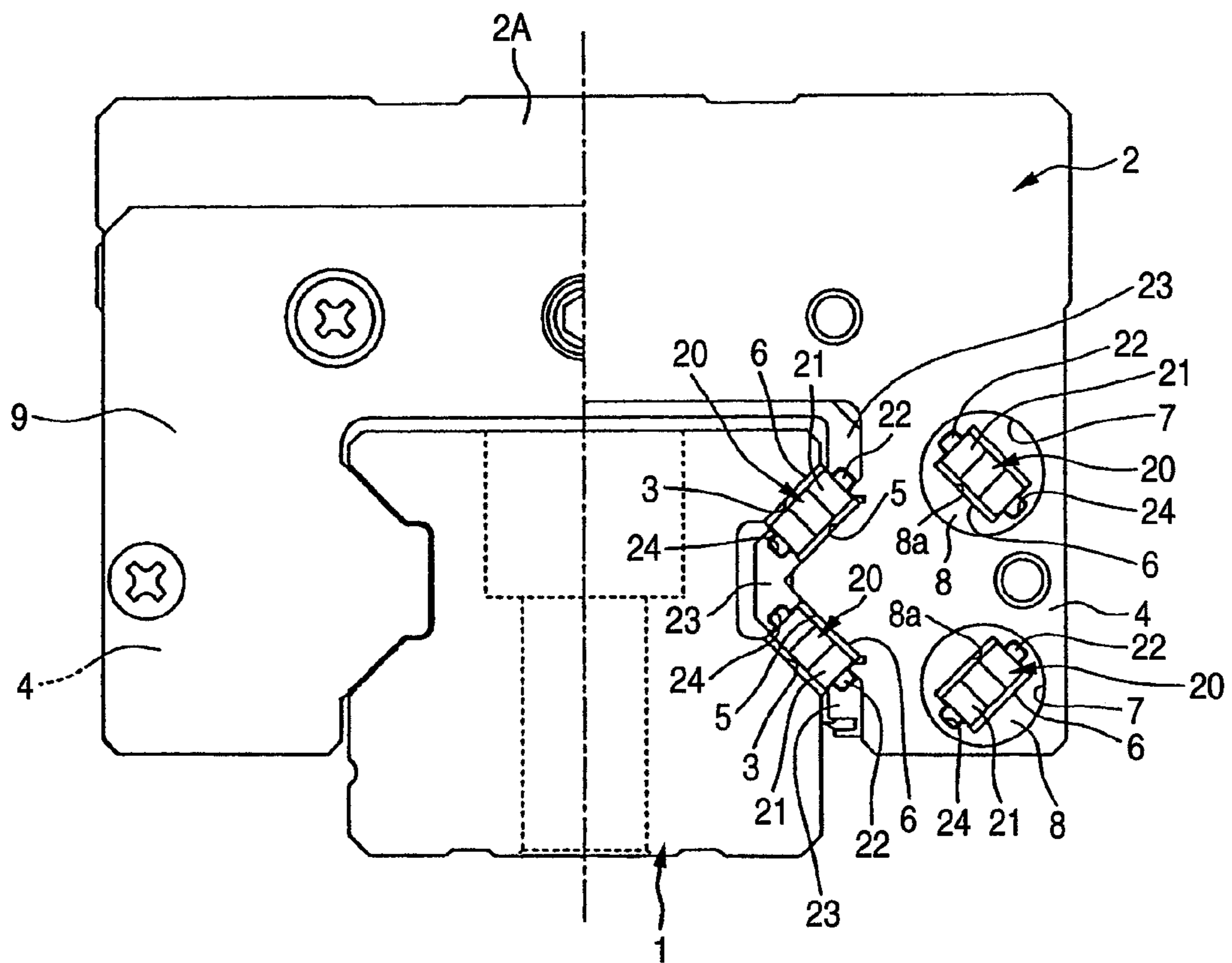
FIG. 13 PRIOR ART
