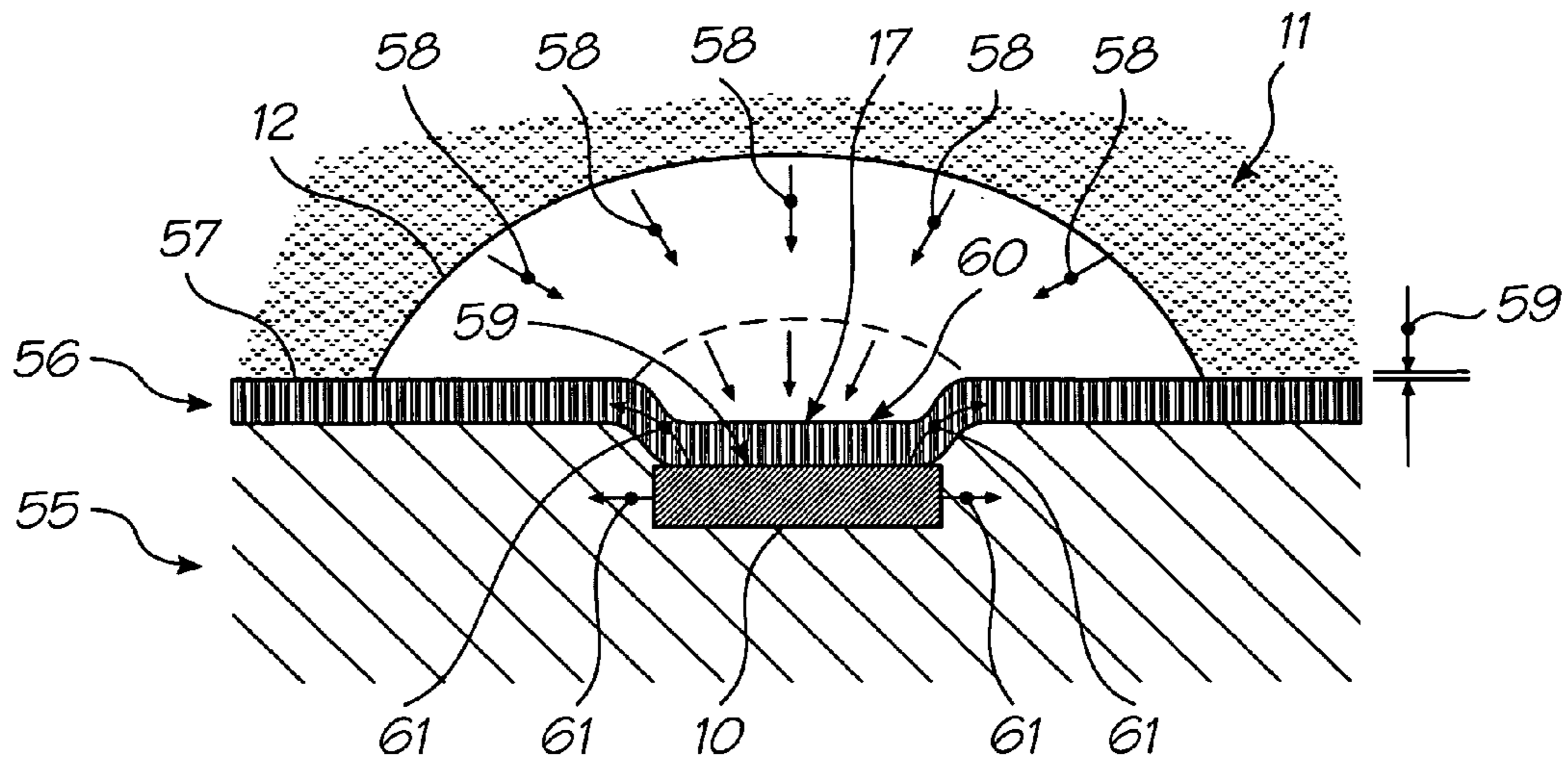
FIG. 47 (PRIOR ART)
