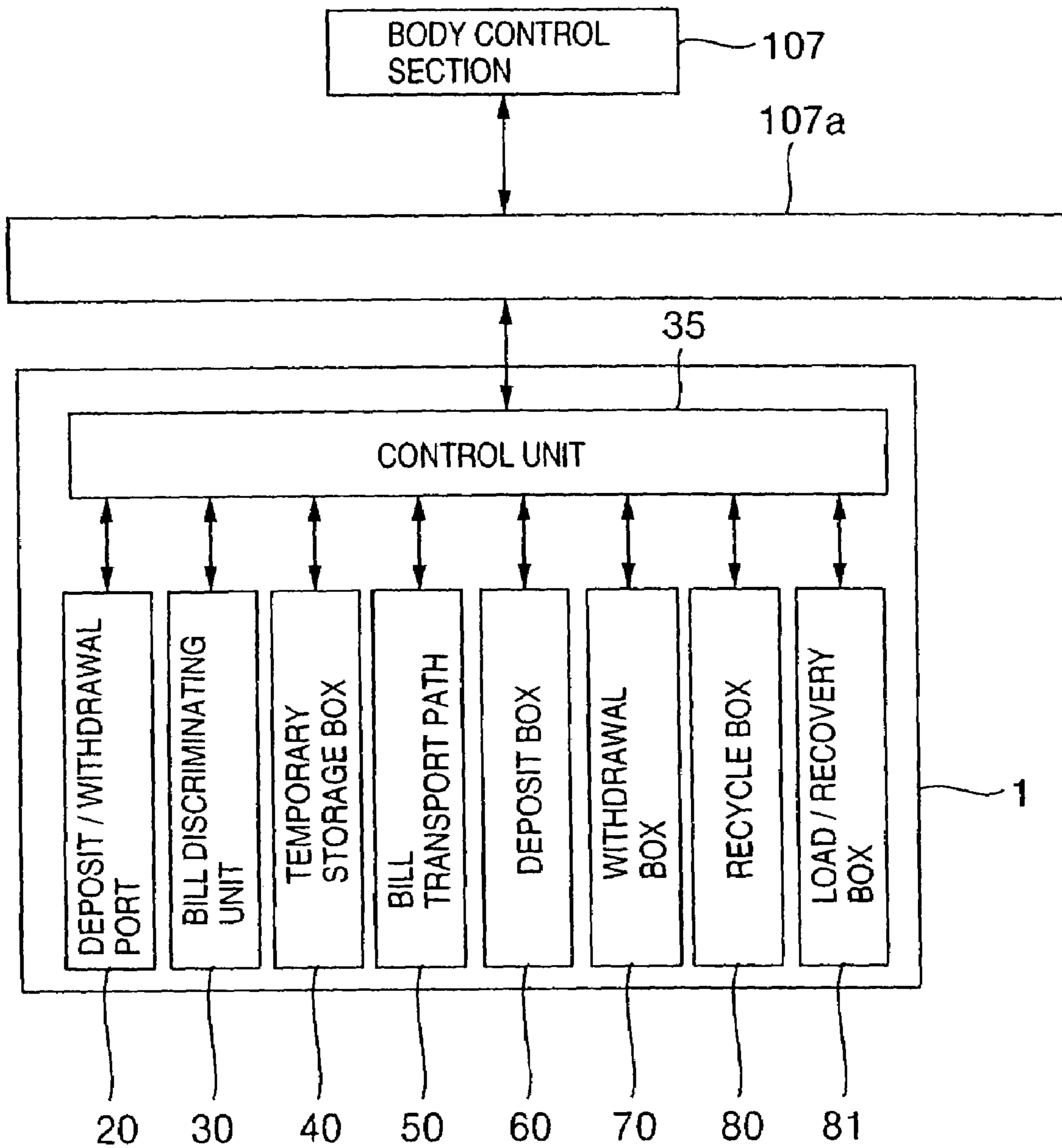
CONTROL BLOCK DIAGRAM OF BILL DEPOSIT / WITHDRAWAL MACHINE 1
