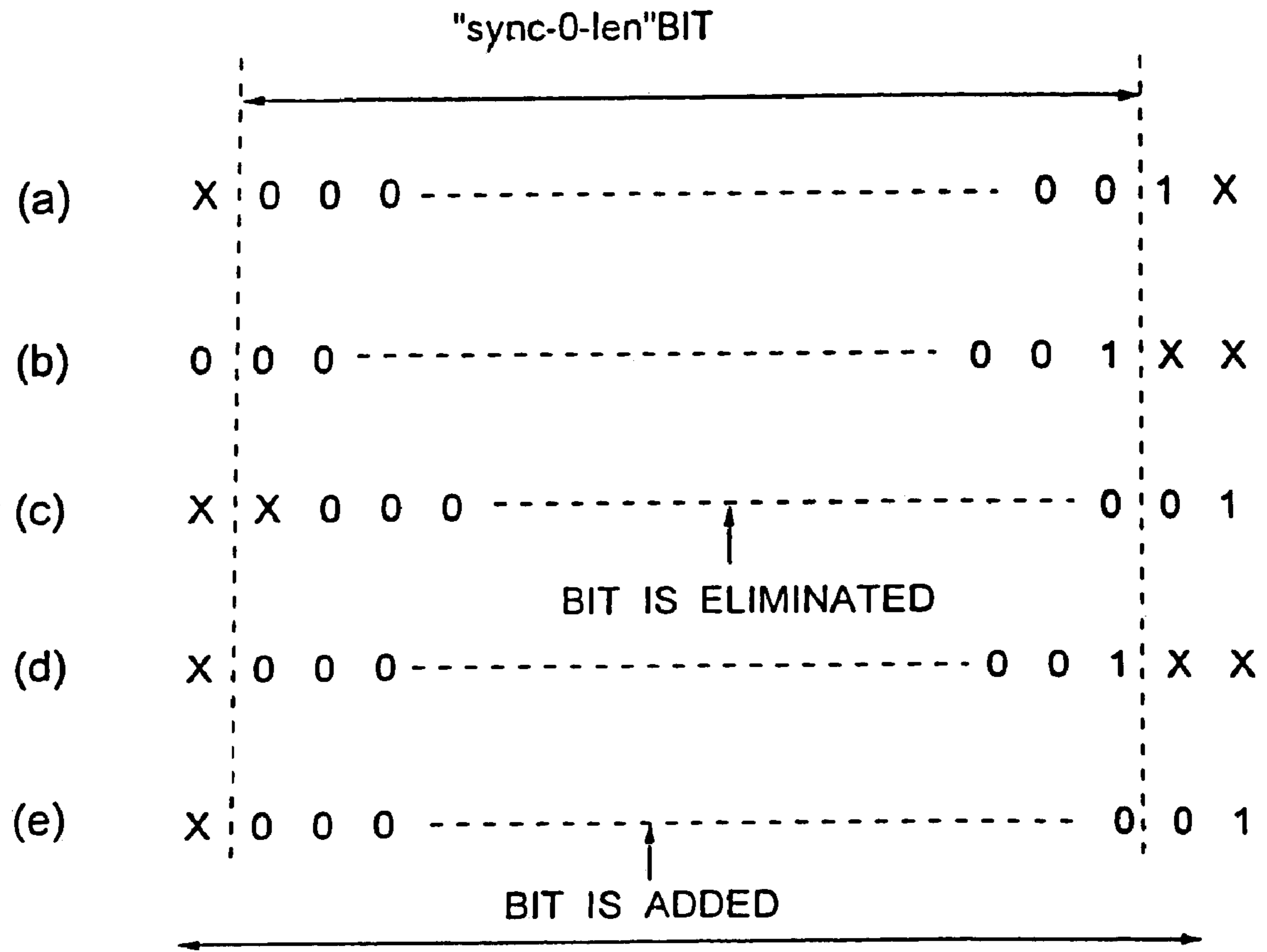
SYNCHRONIZATION CODE DETECTION WINDOW OF "sync-0-len+2"BIT
