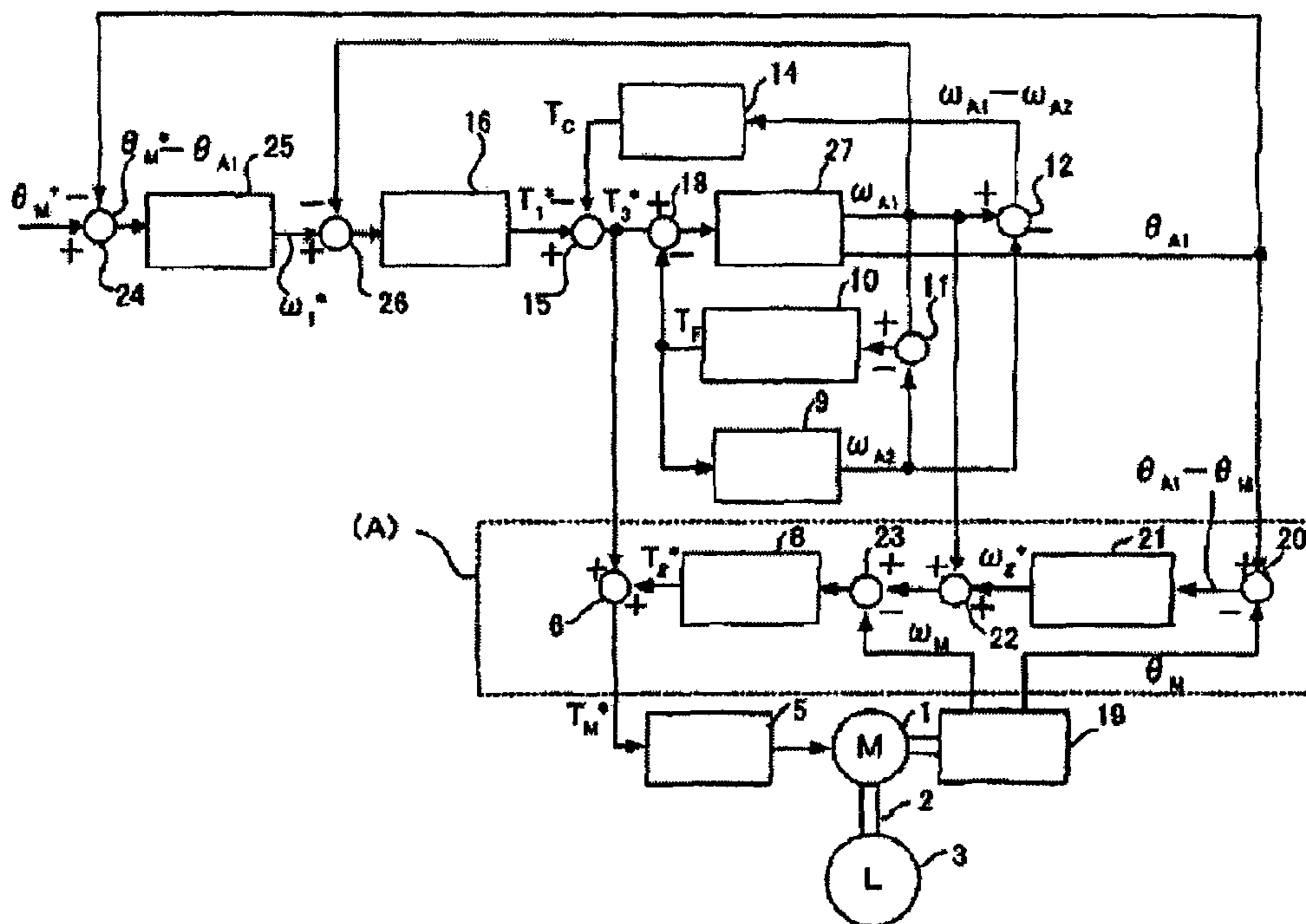
FIG. 7 PRIOR ART
