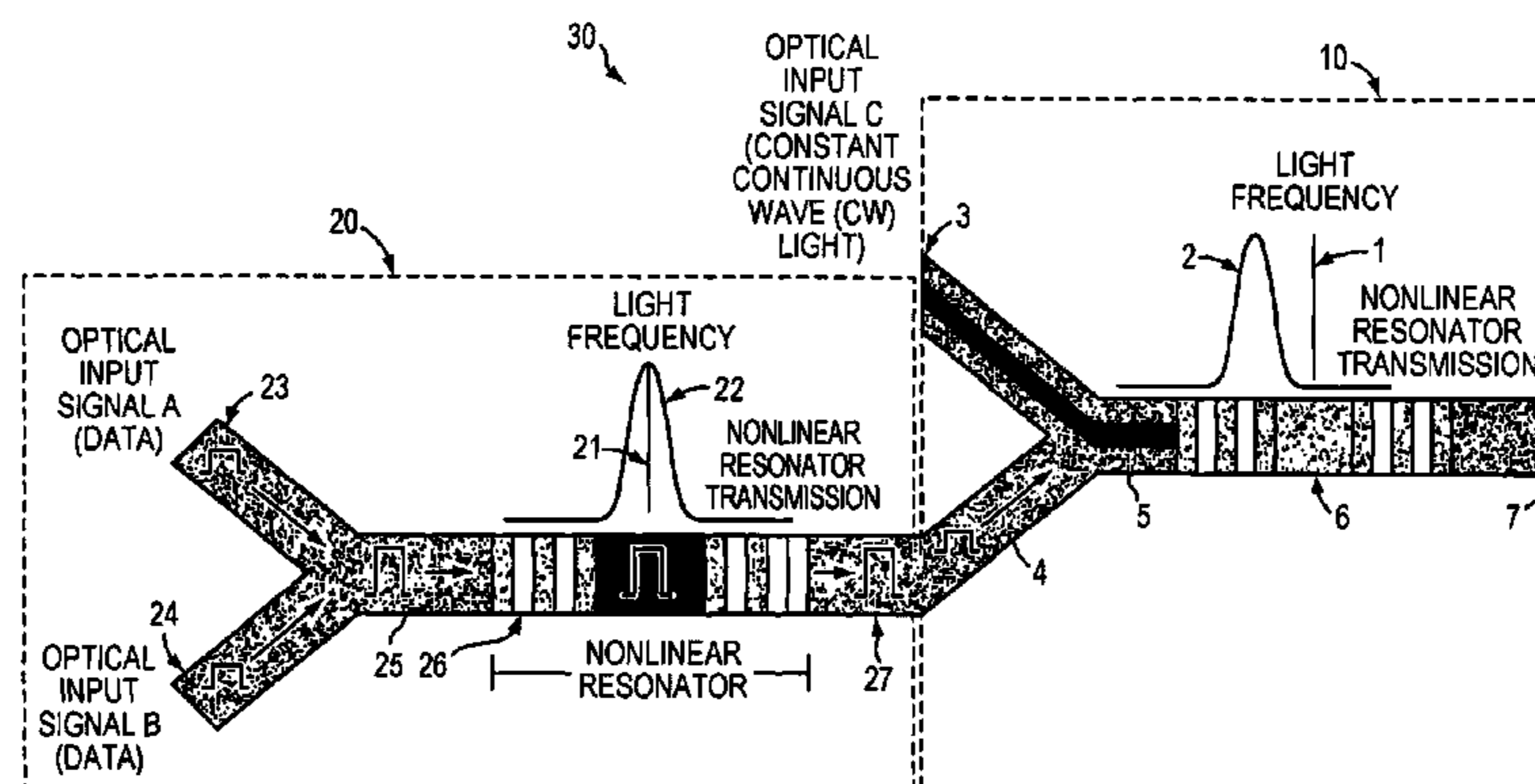
ALL-OPTICAL AND GATE RECEIVING 1 BITS AS OPTICAL INPUT SIGNALS AND OUTPUTTING A 0-BIT AS OPTICAL OUTPUT SIGNAL
