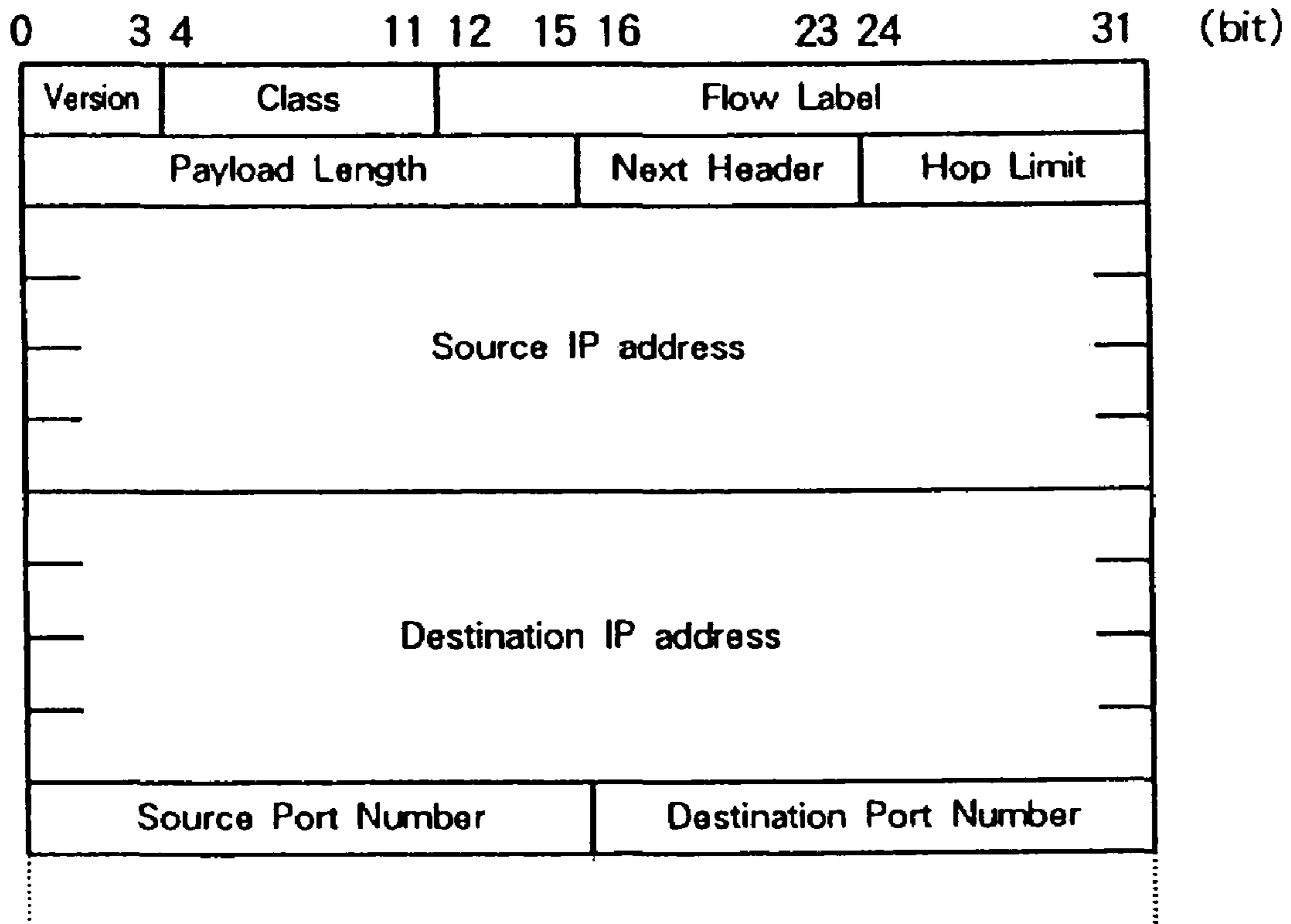
IPv6 with TCP
