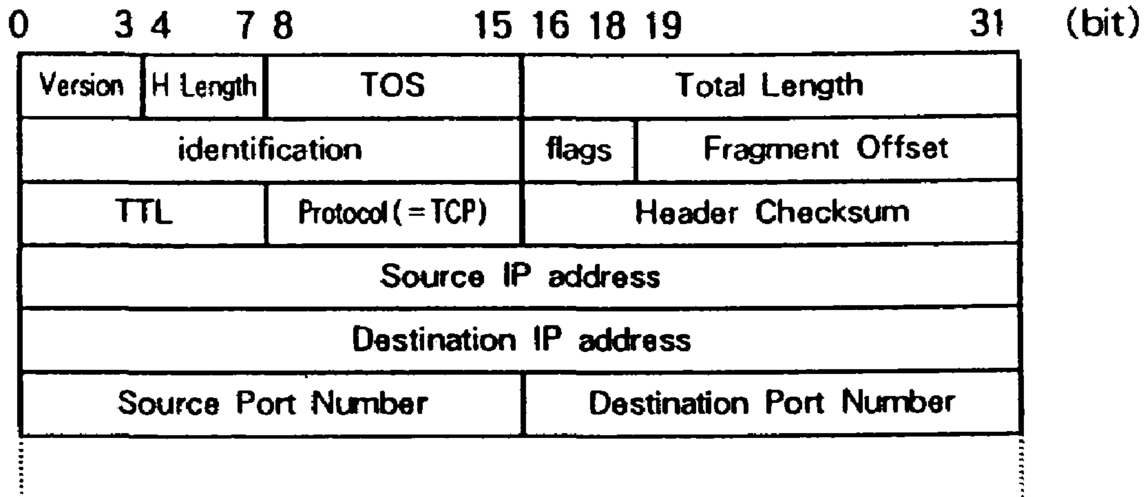
IPv4 with TCP
