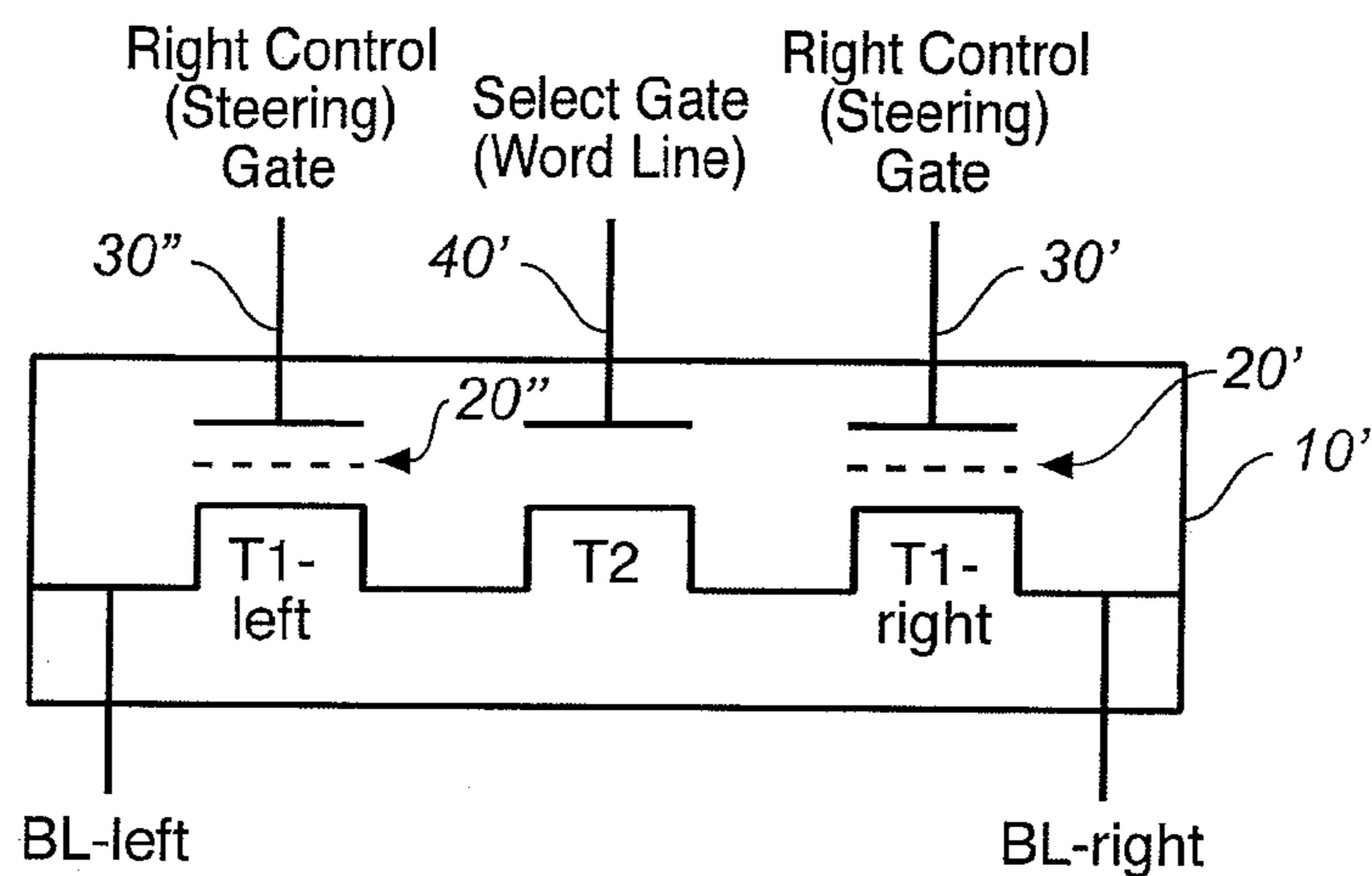
FIG. 1C (PRIOR ART)
