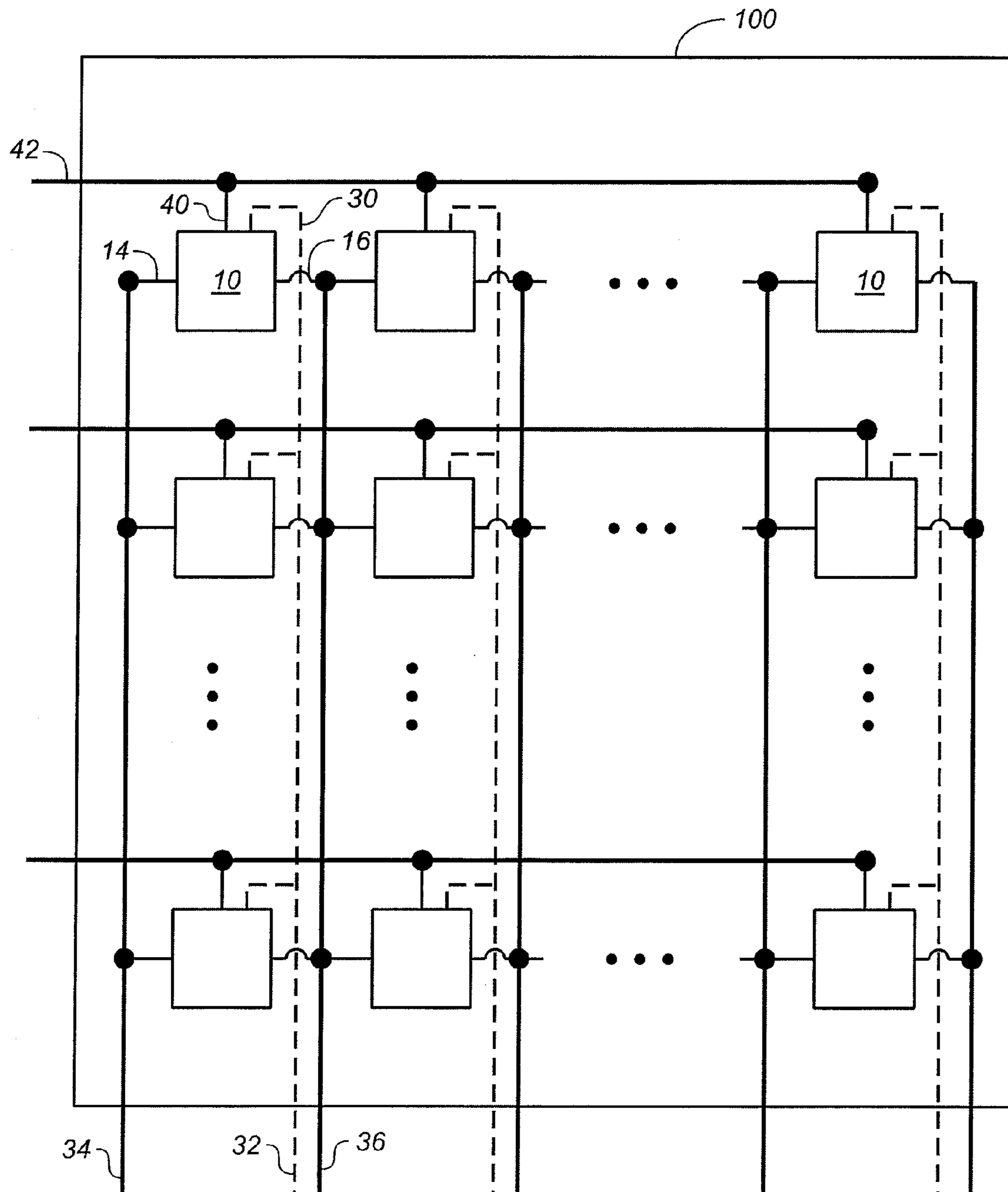
FIG. 2 (PRIOR ART)
