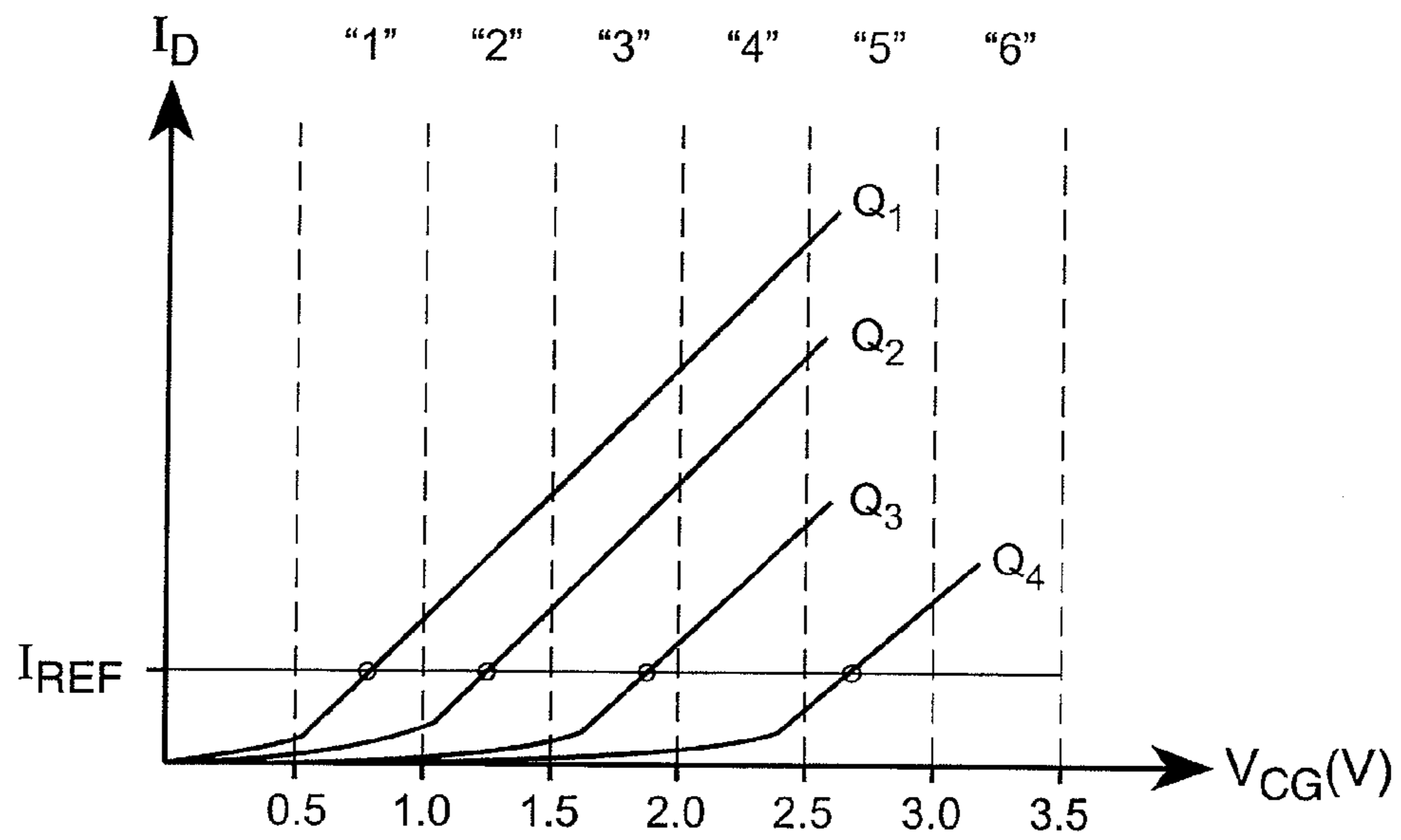
FIG. 4 (PRIOR ART)
