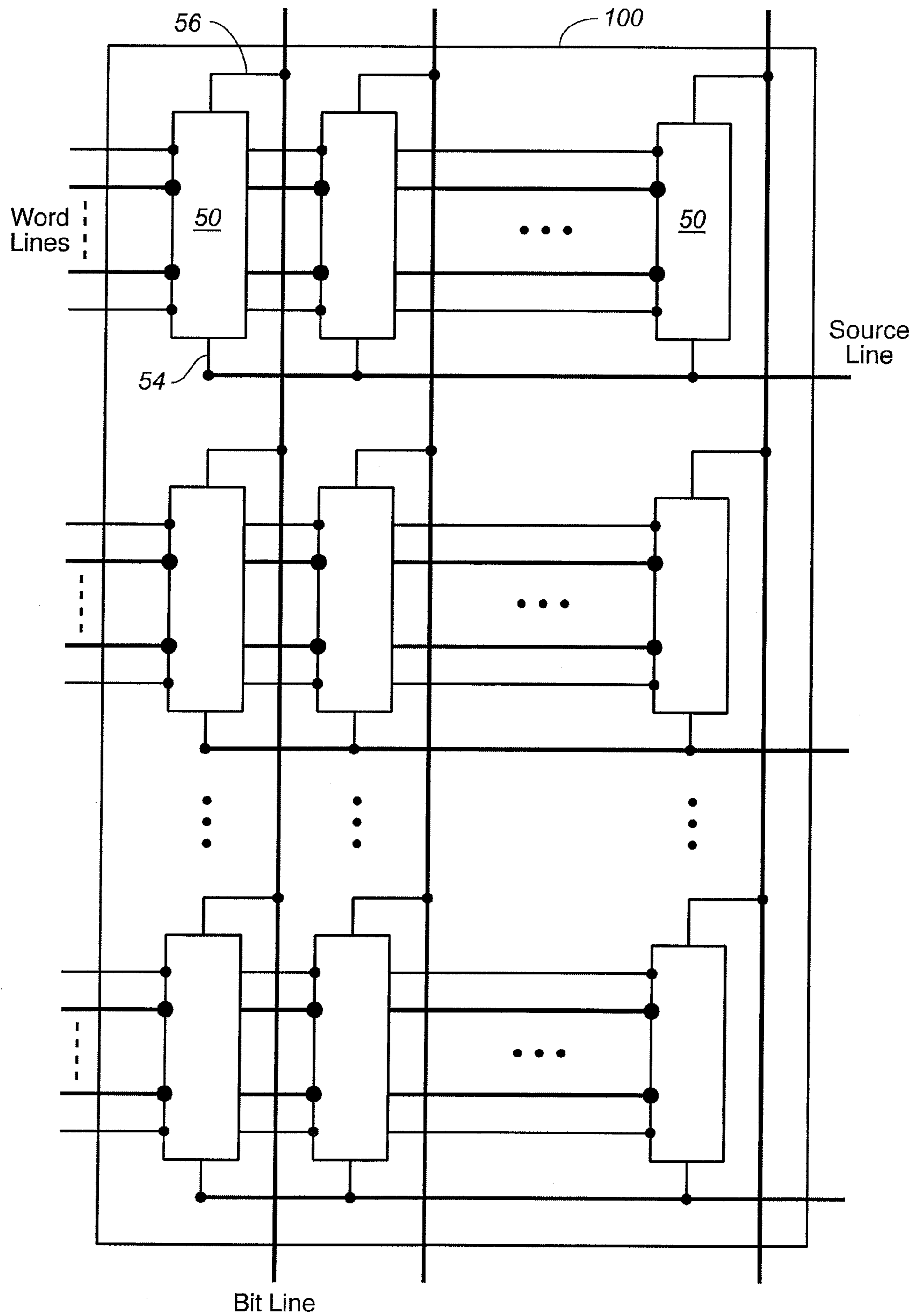
FIG. 3 (PRIOR ART)
