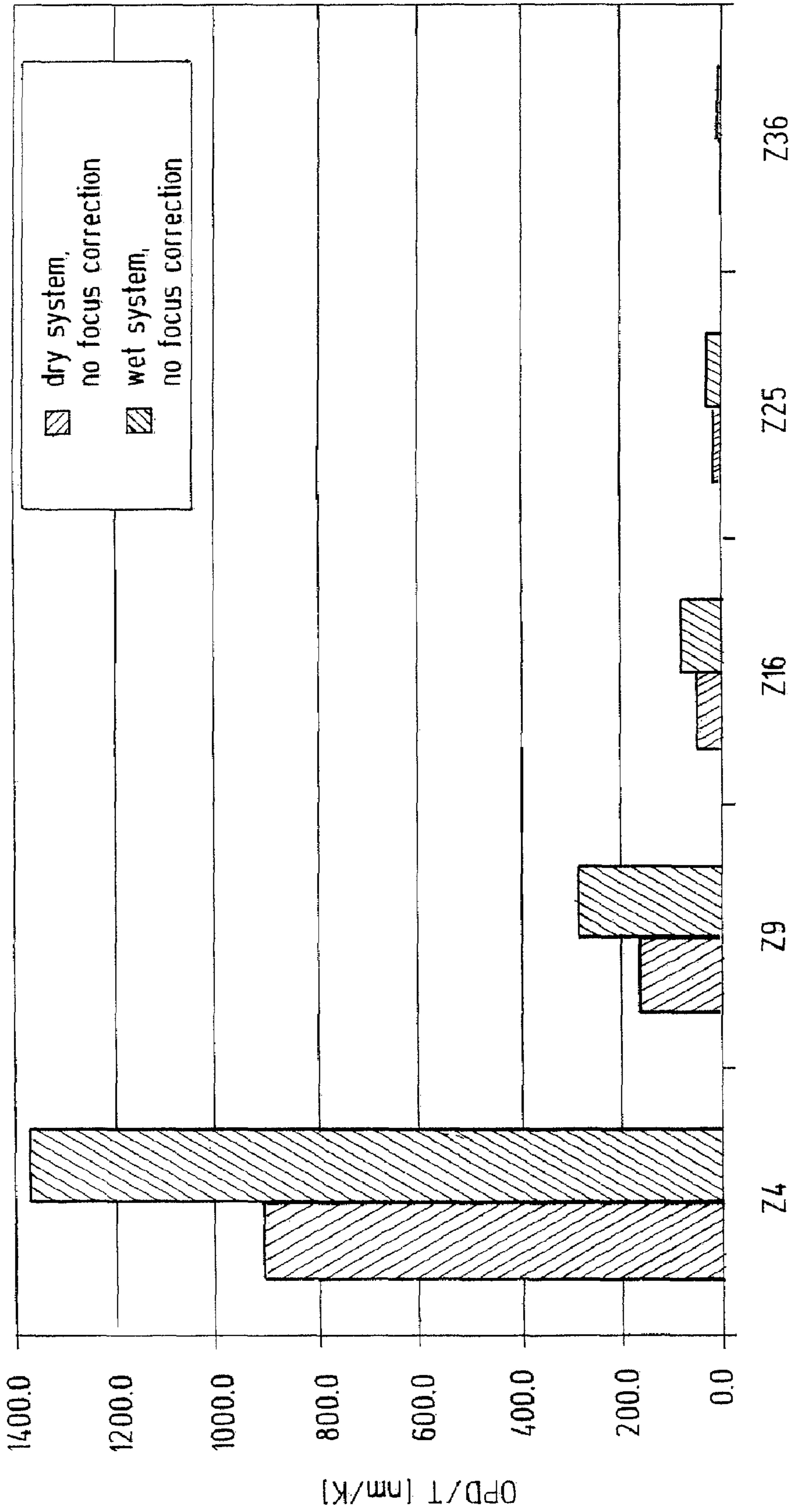
Zernike - coefficients
