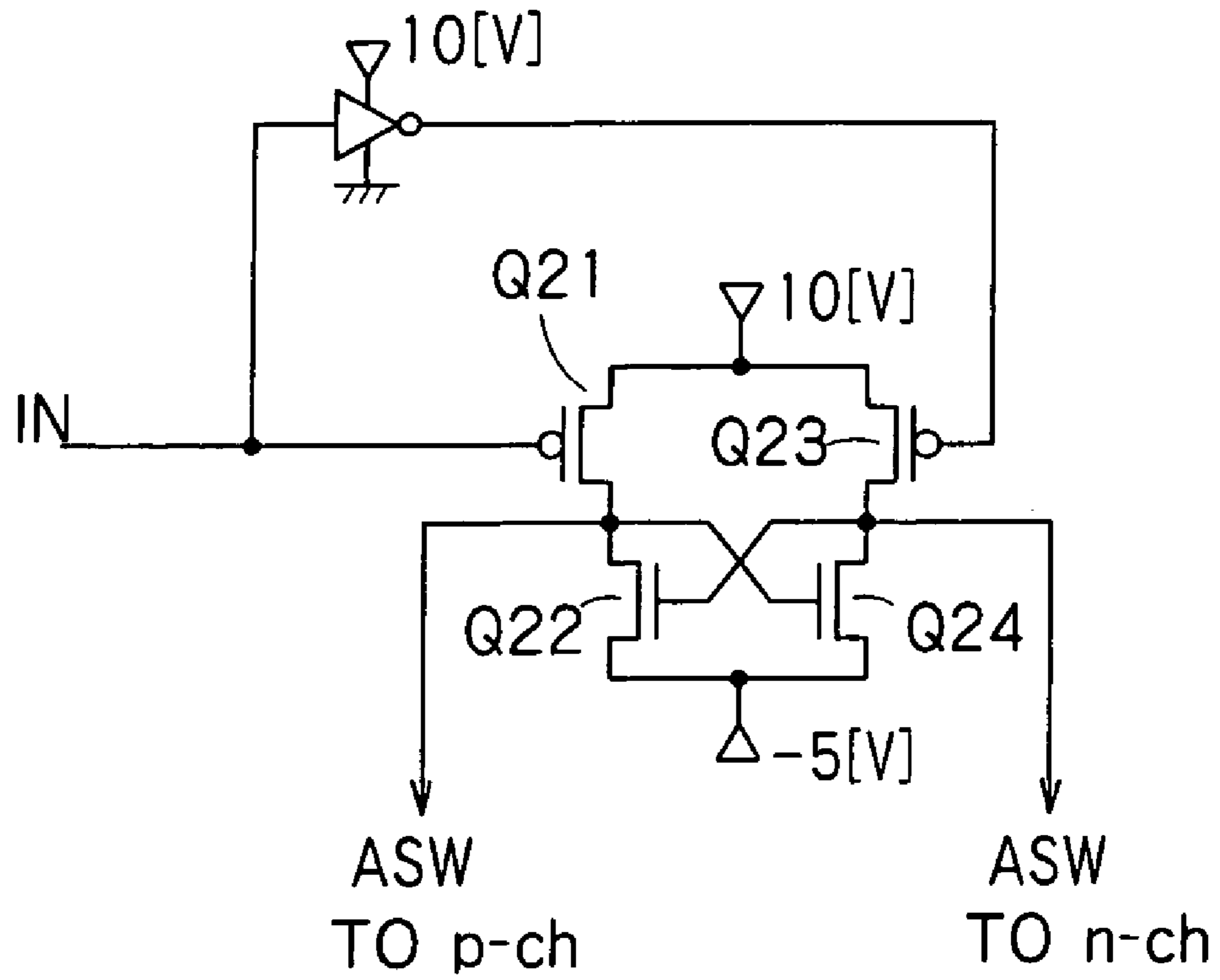
22: LEVEL CONVERSION CIRCUIT
