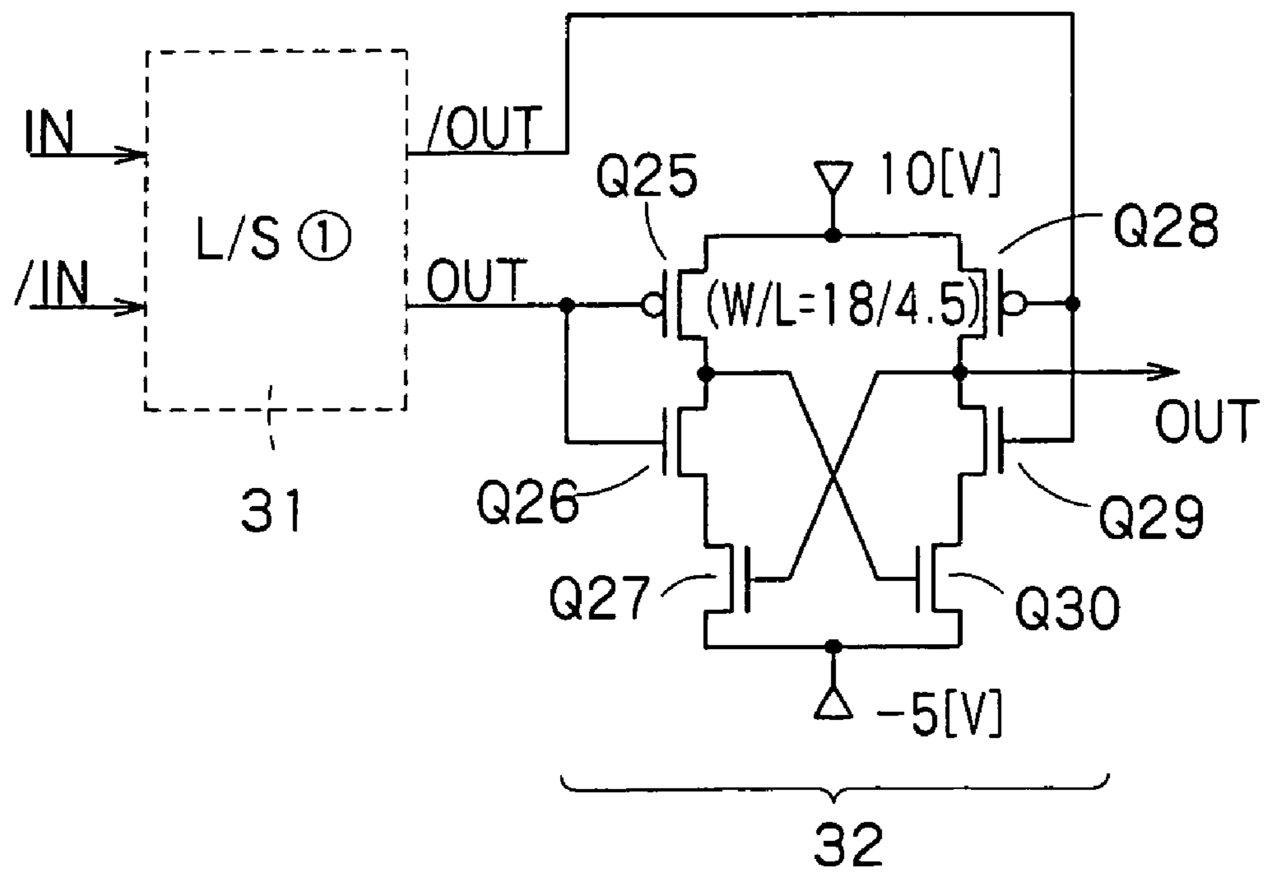
28: LEVEL CONVERSION CIRCUIT
