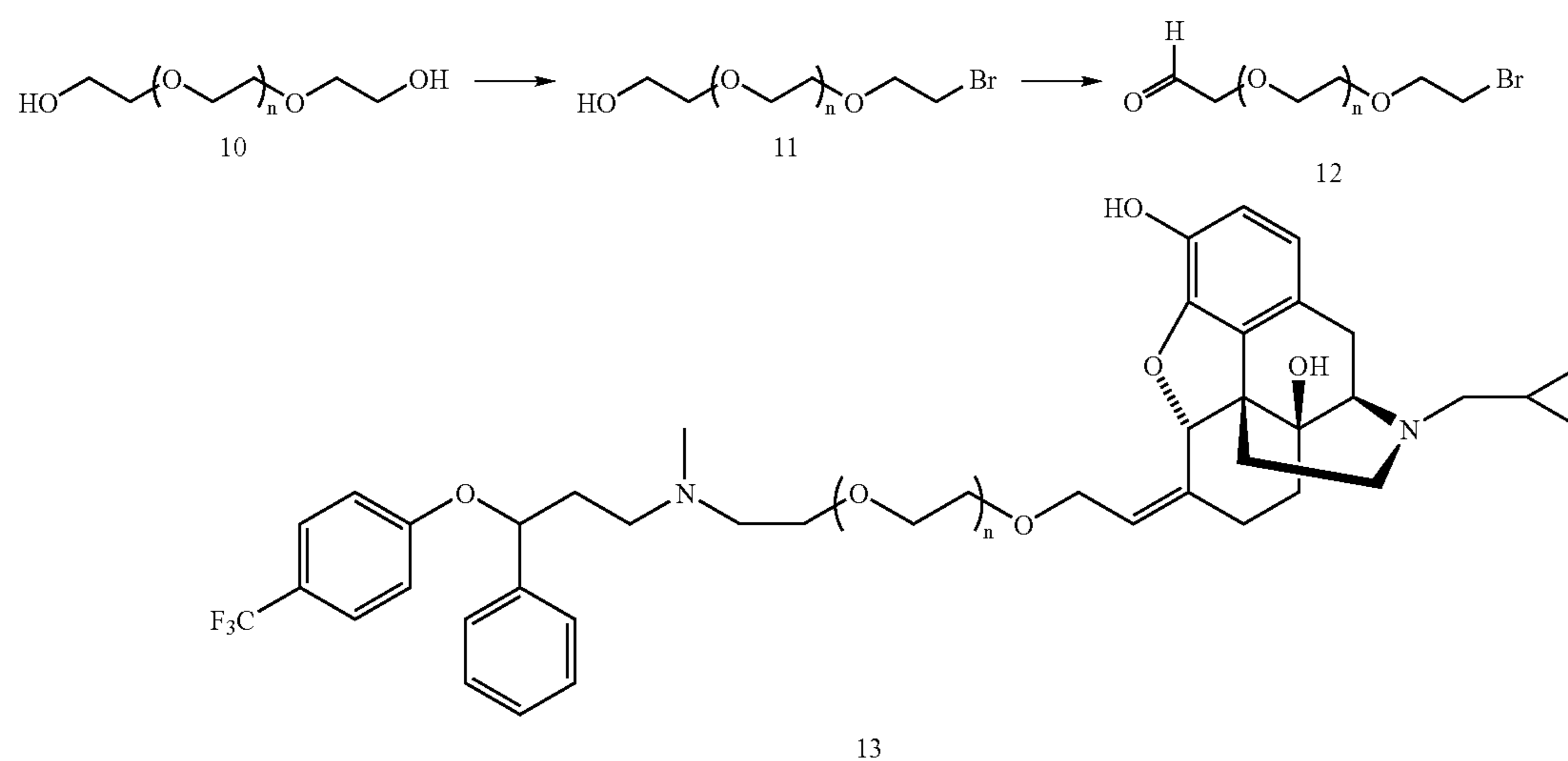
Scheme 2
