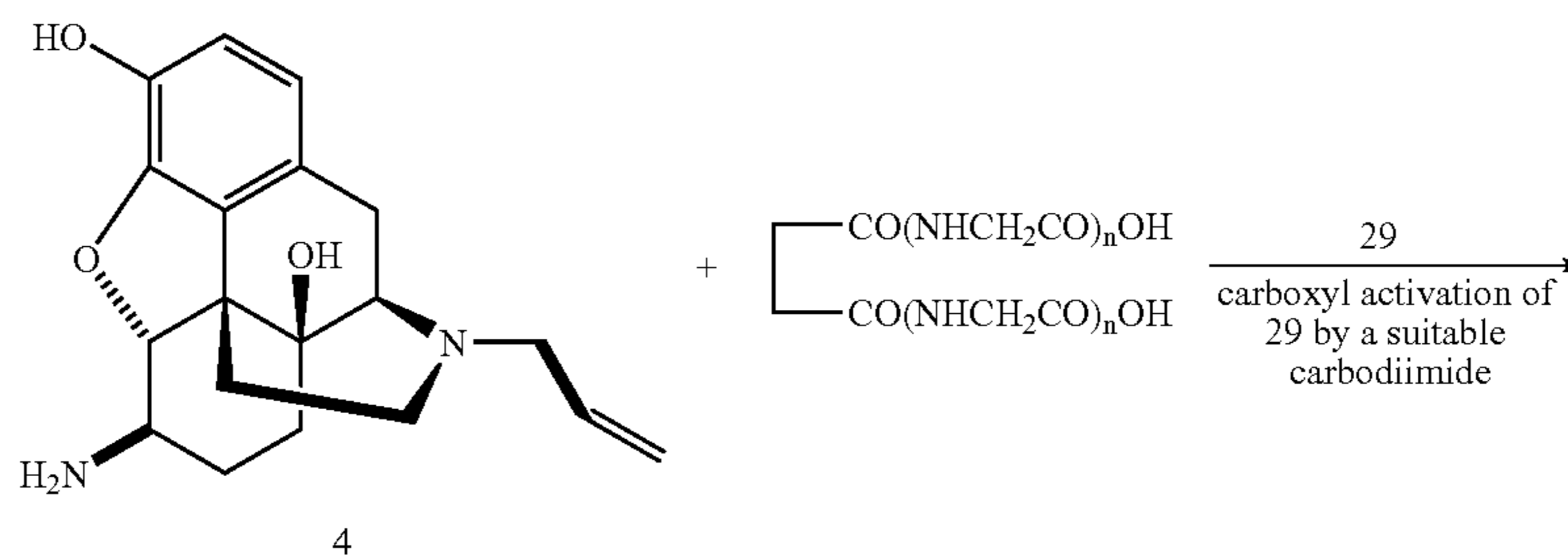
Scheme 5
