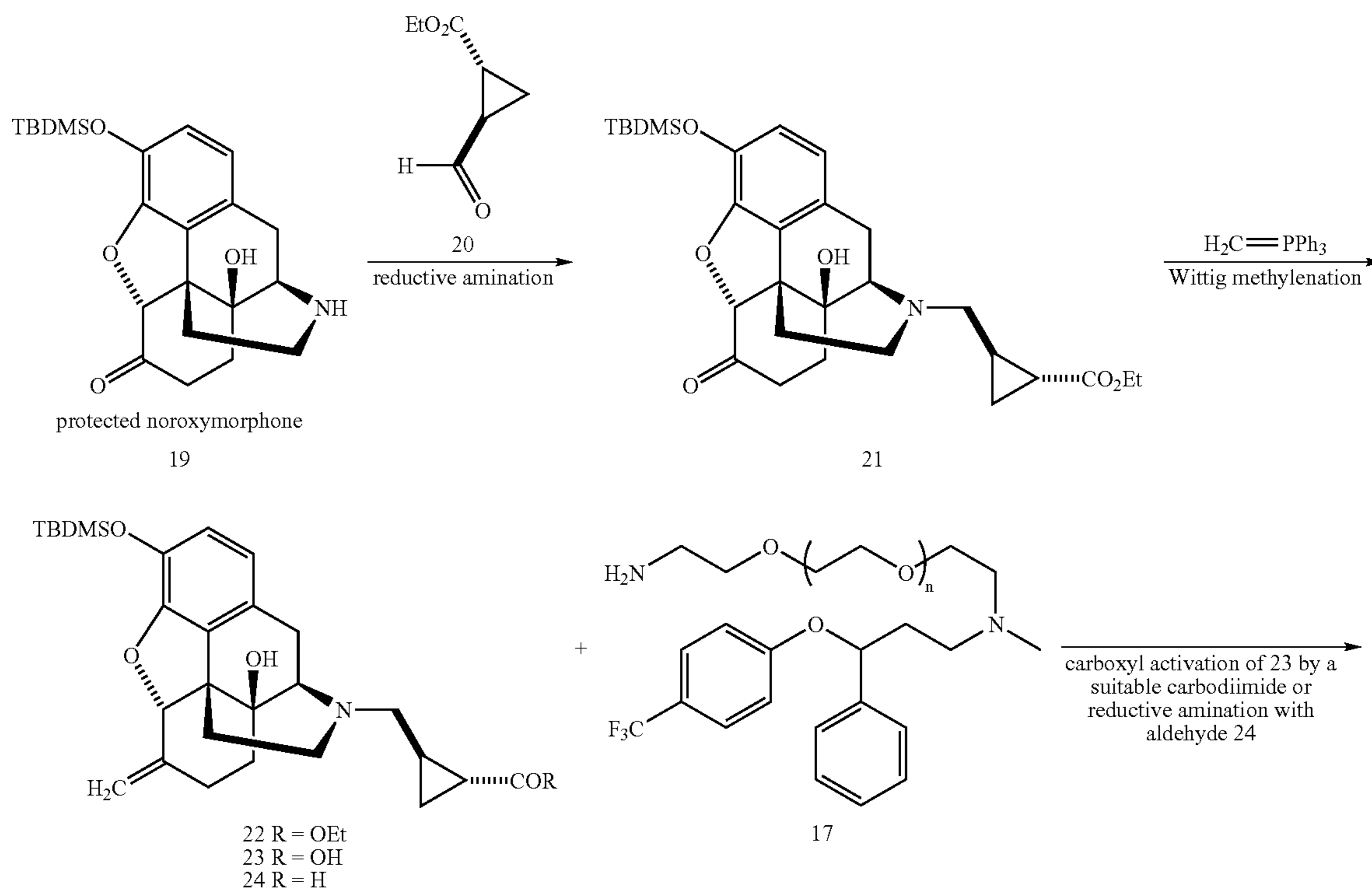
Scheme 4
