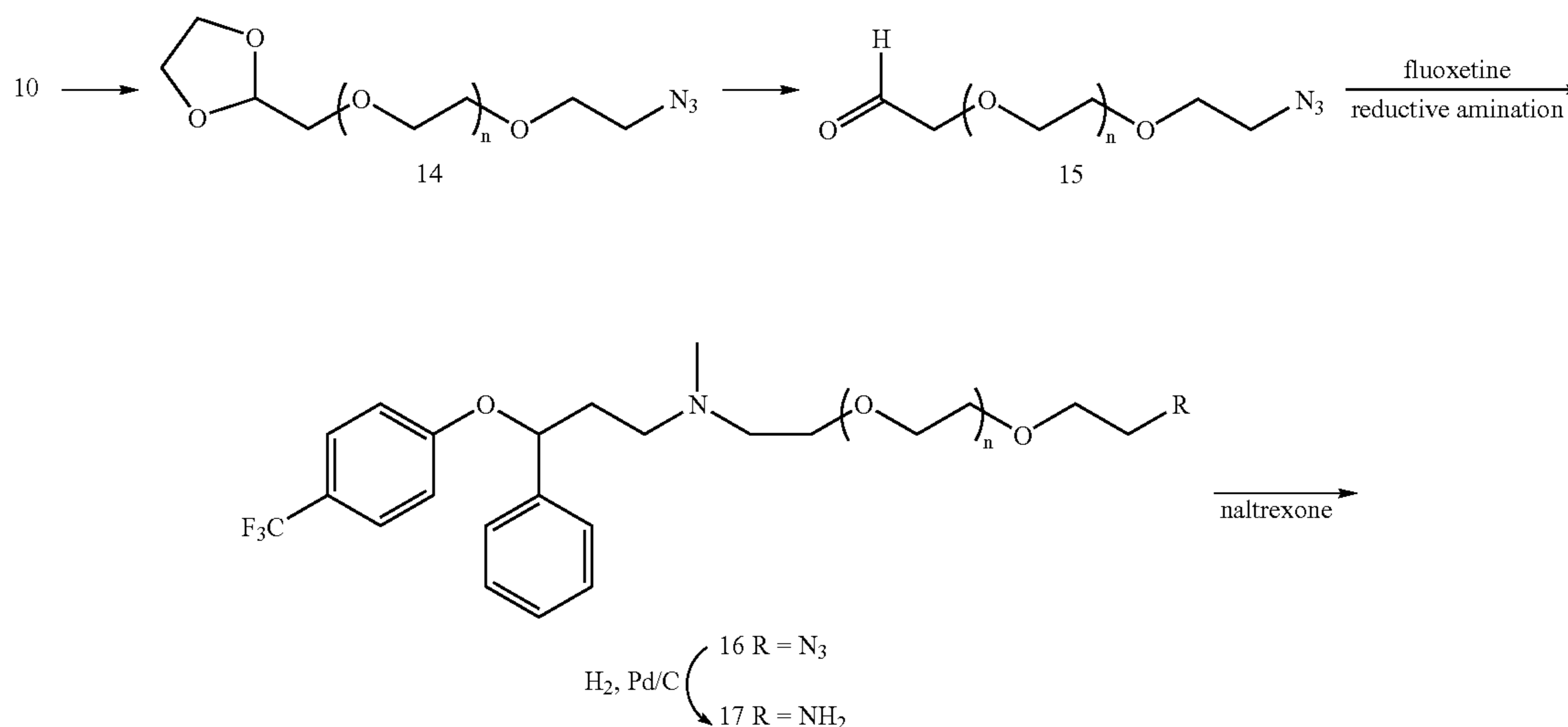
Scheme 3
