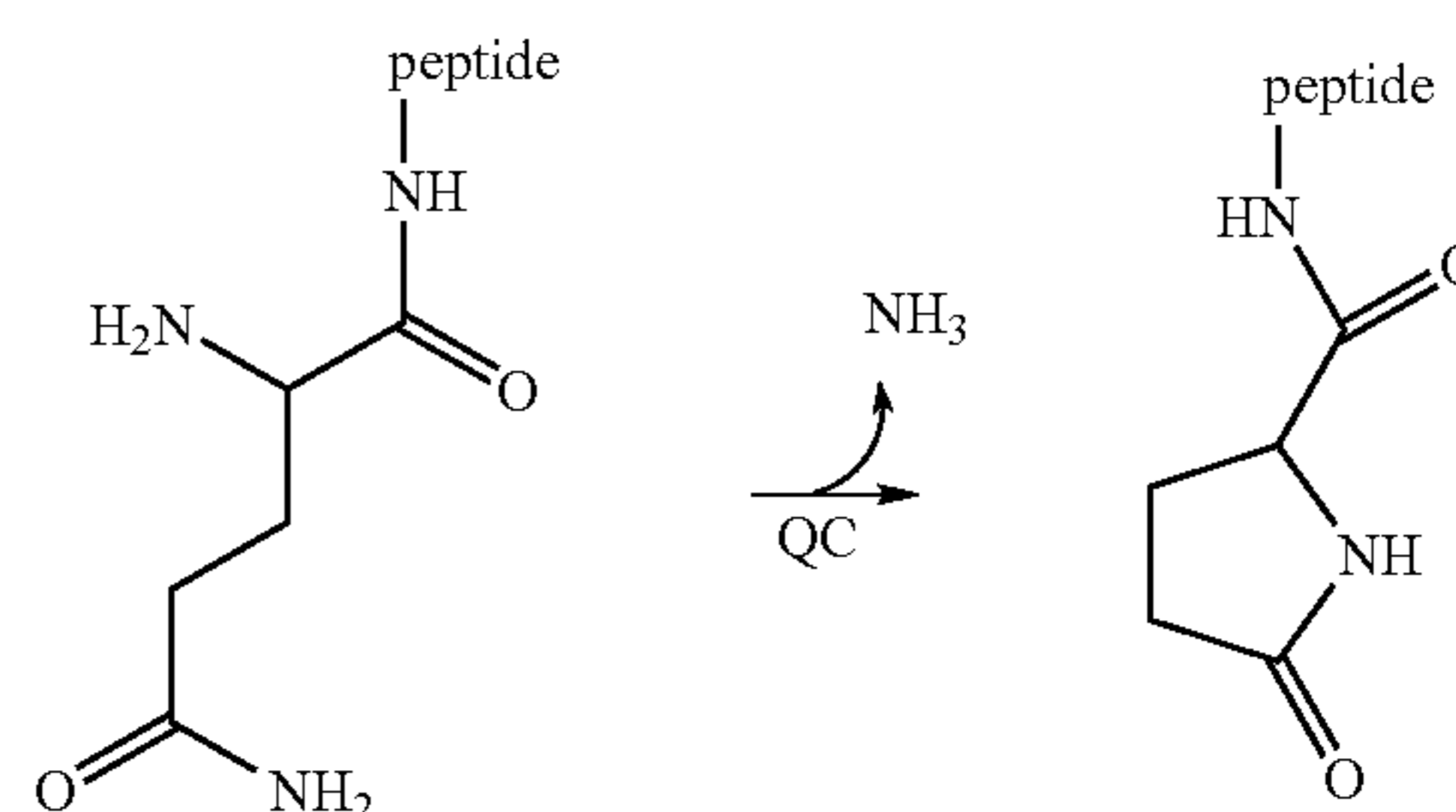
Scheme 1: Cyclization of glutamine bt QC
