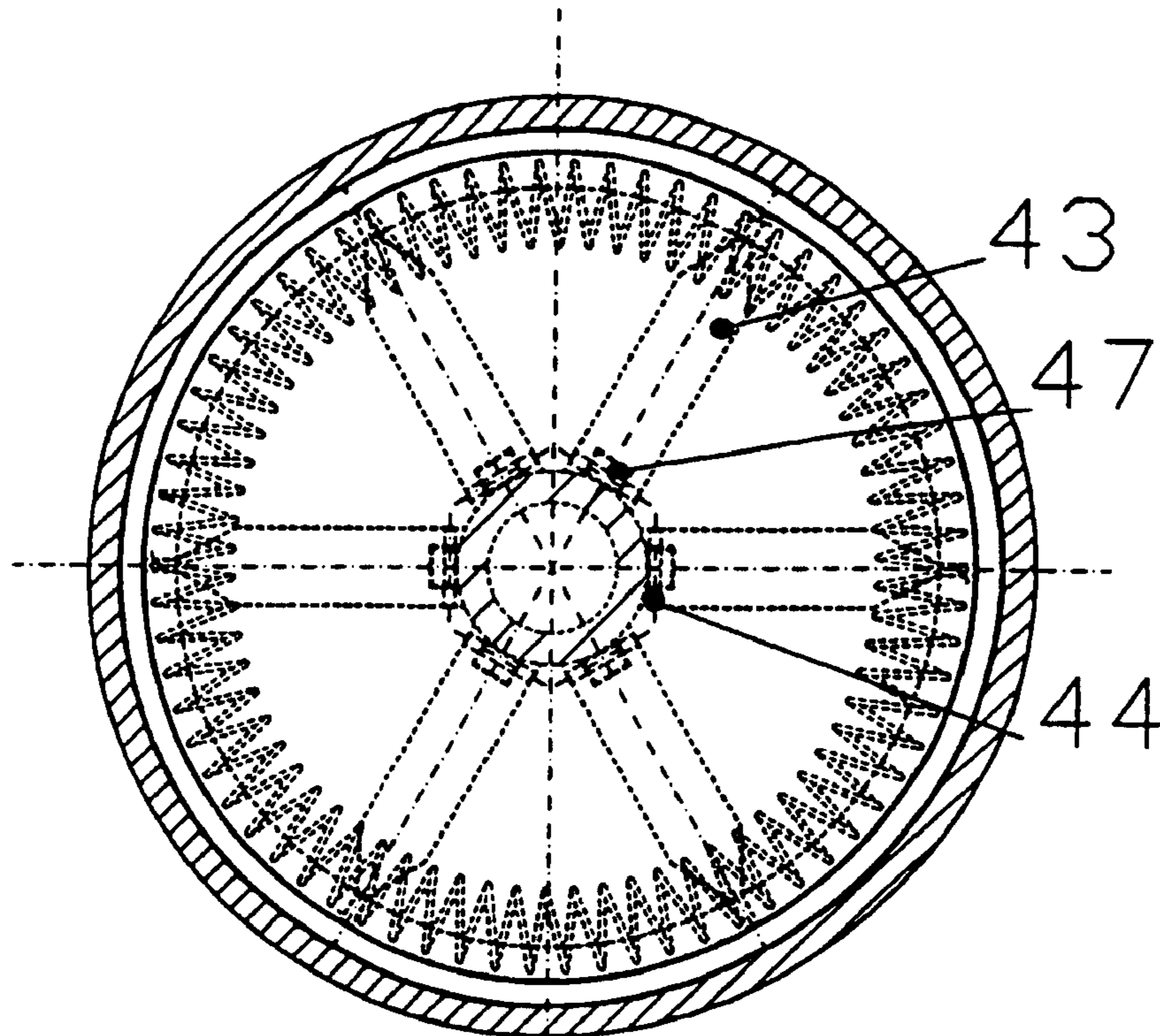
Fig.5D section C-C
