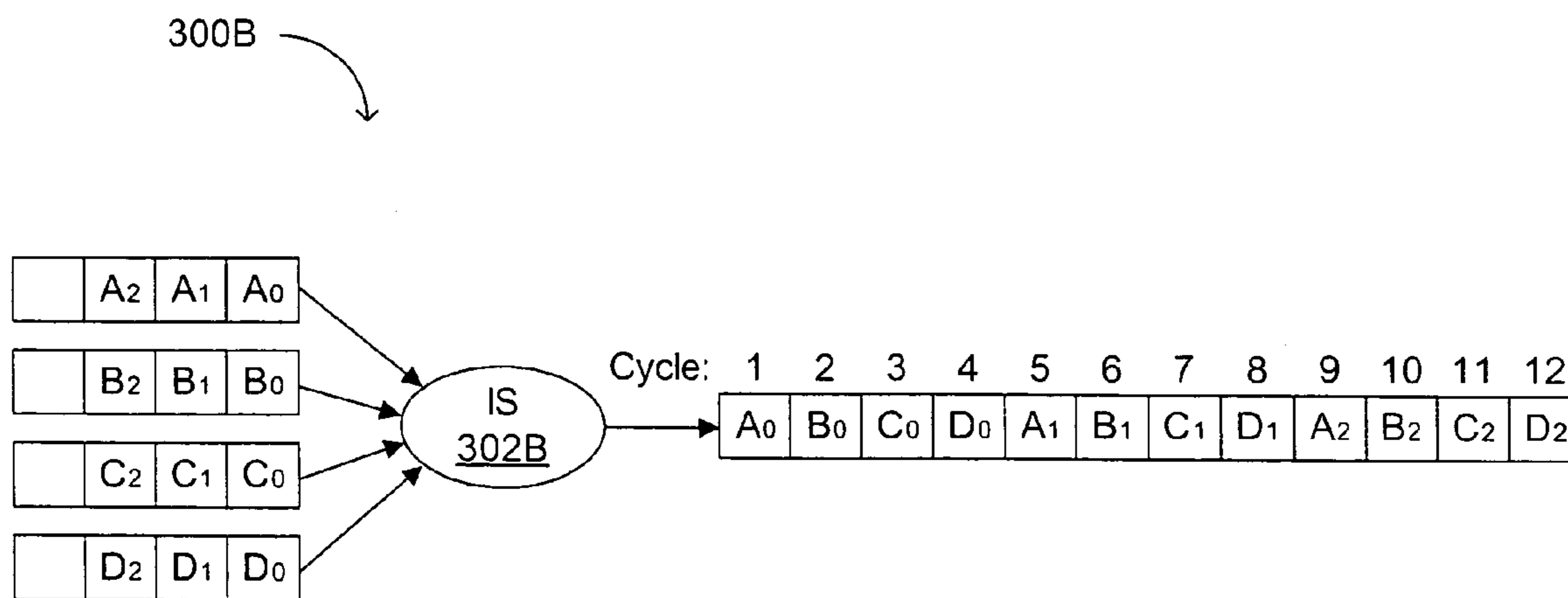
FIG. 3B (conventional)
