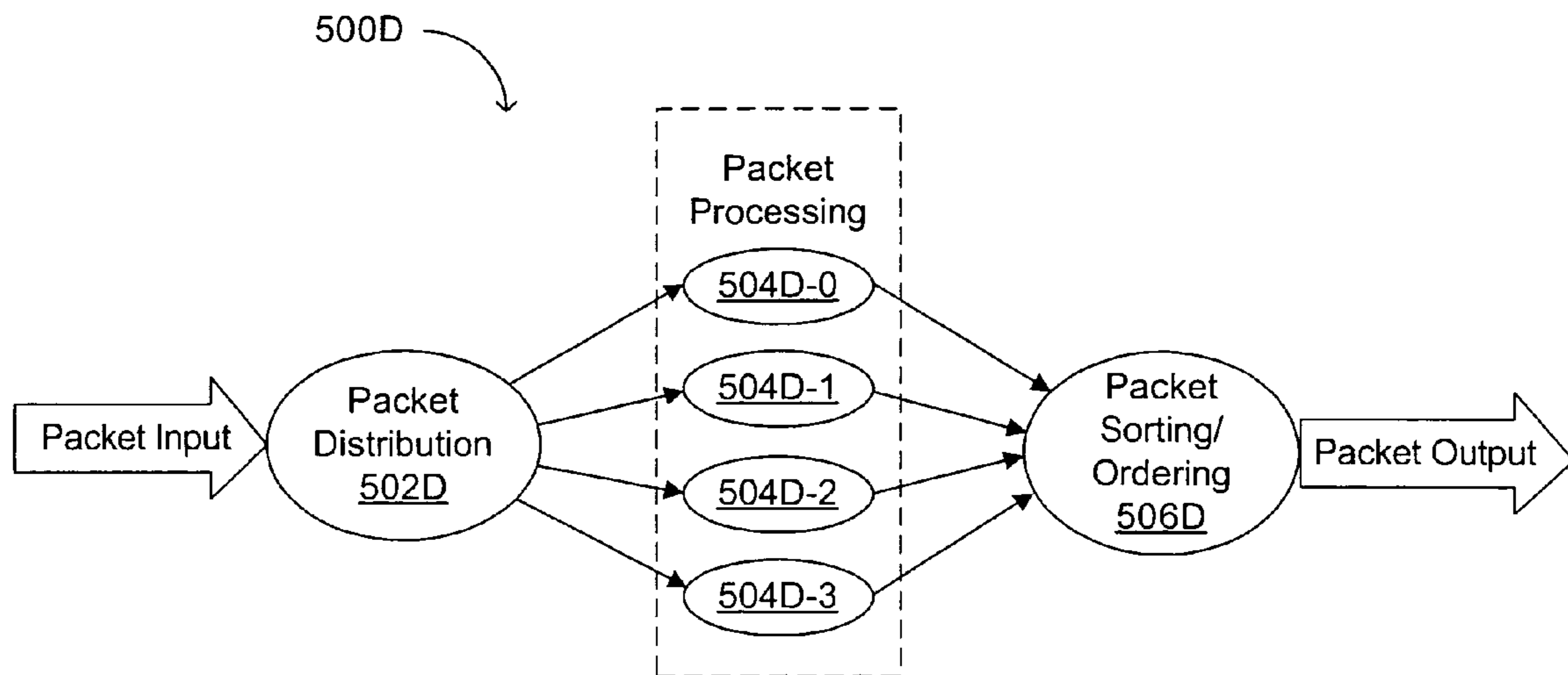
FIG. 5D (conventional)
