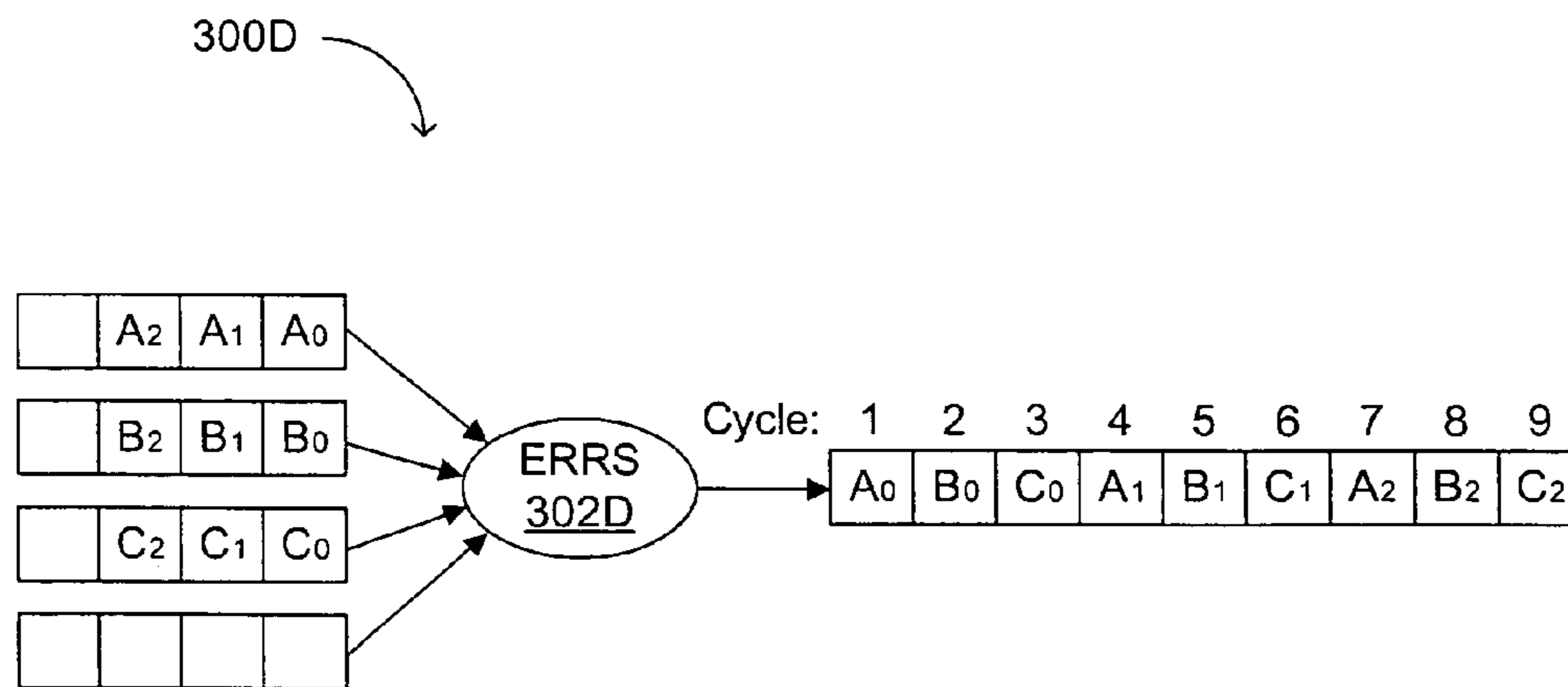
FIG. 3D
