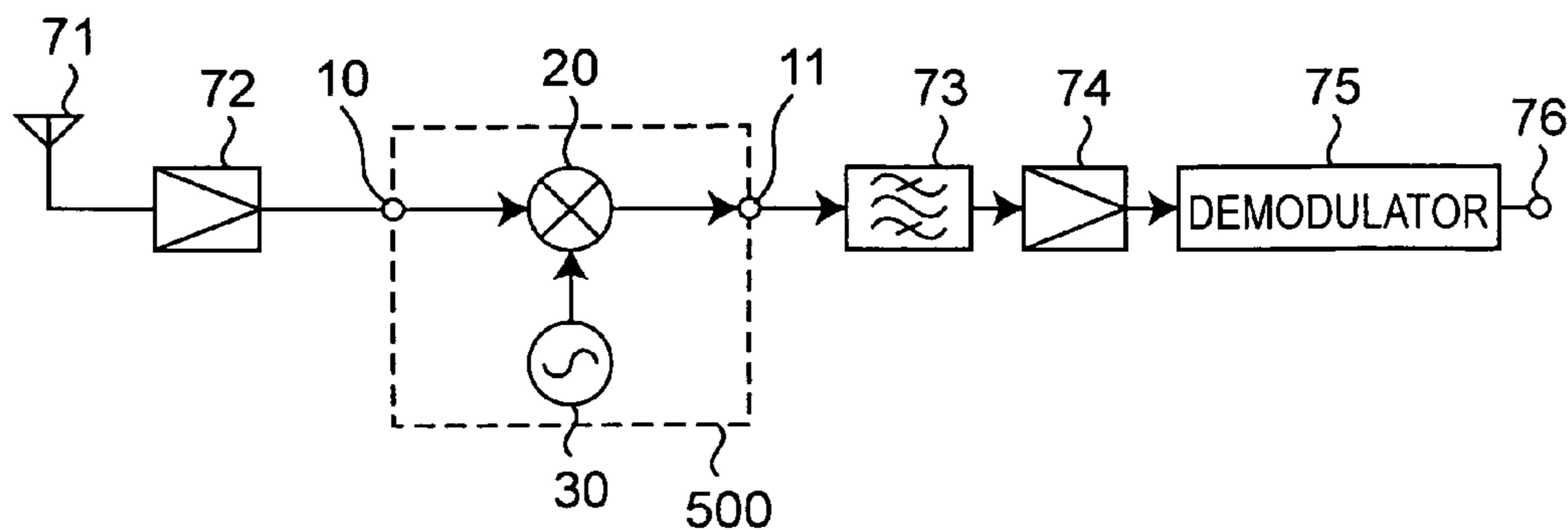
Fig.10 PRIOR ART
