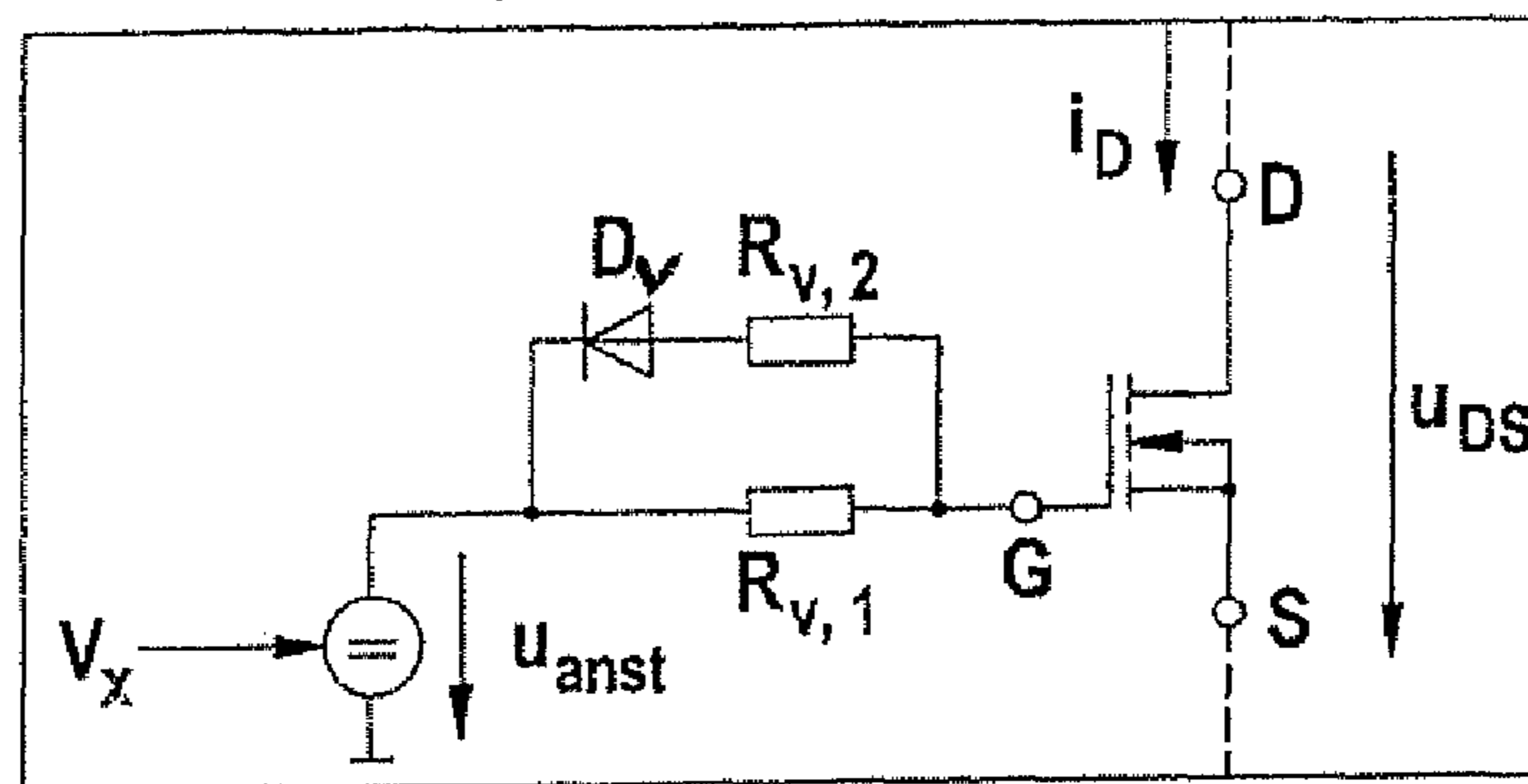
Fig. 2 PRIOR ART
