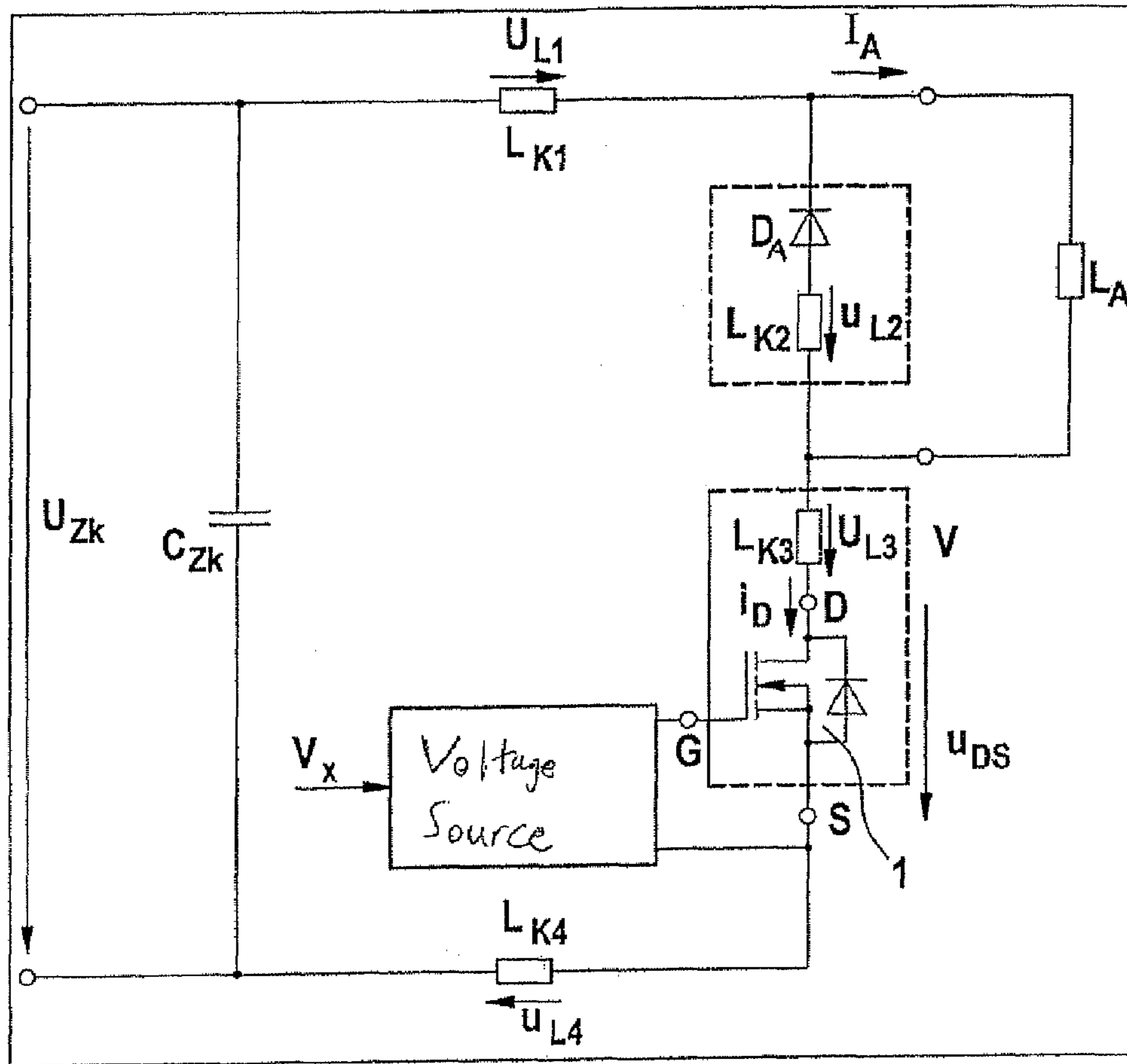
Fig. 1 PRIOR ART
