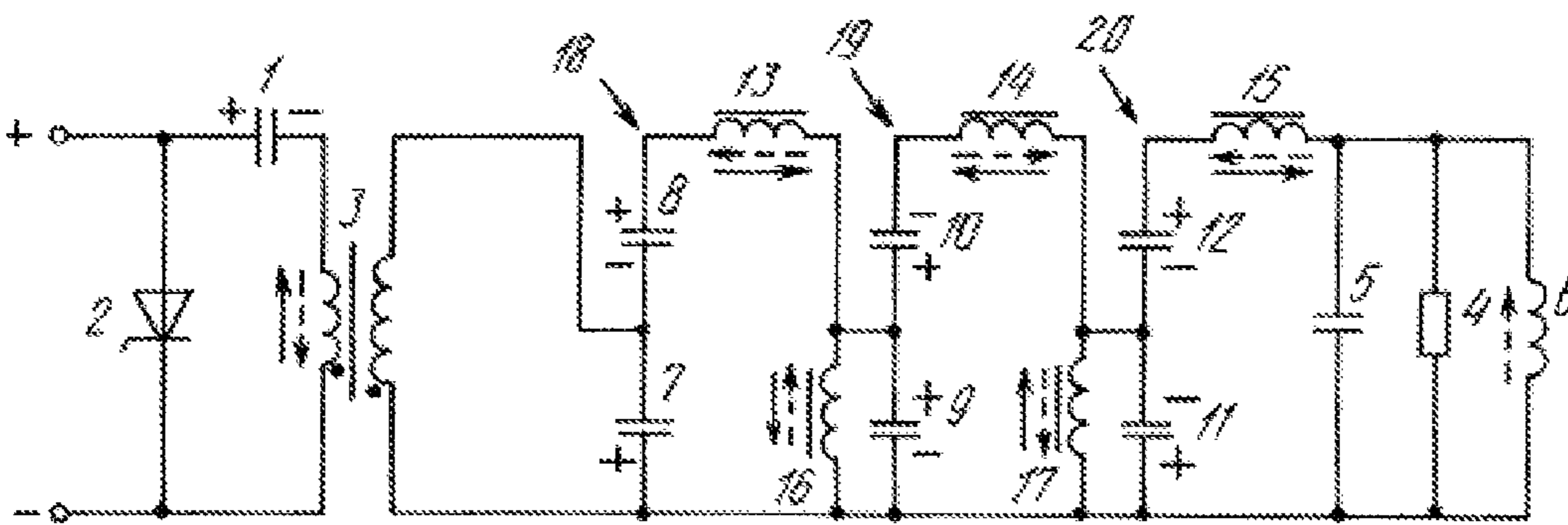
Fig. 2 – PRIOR ART
