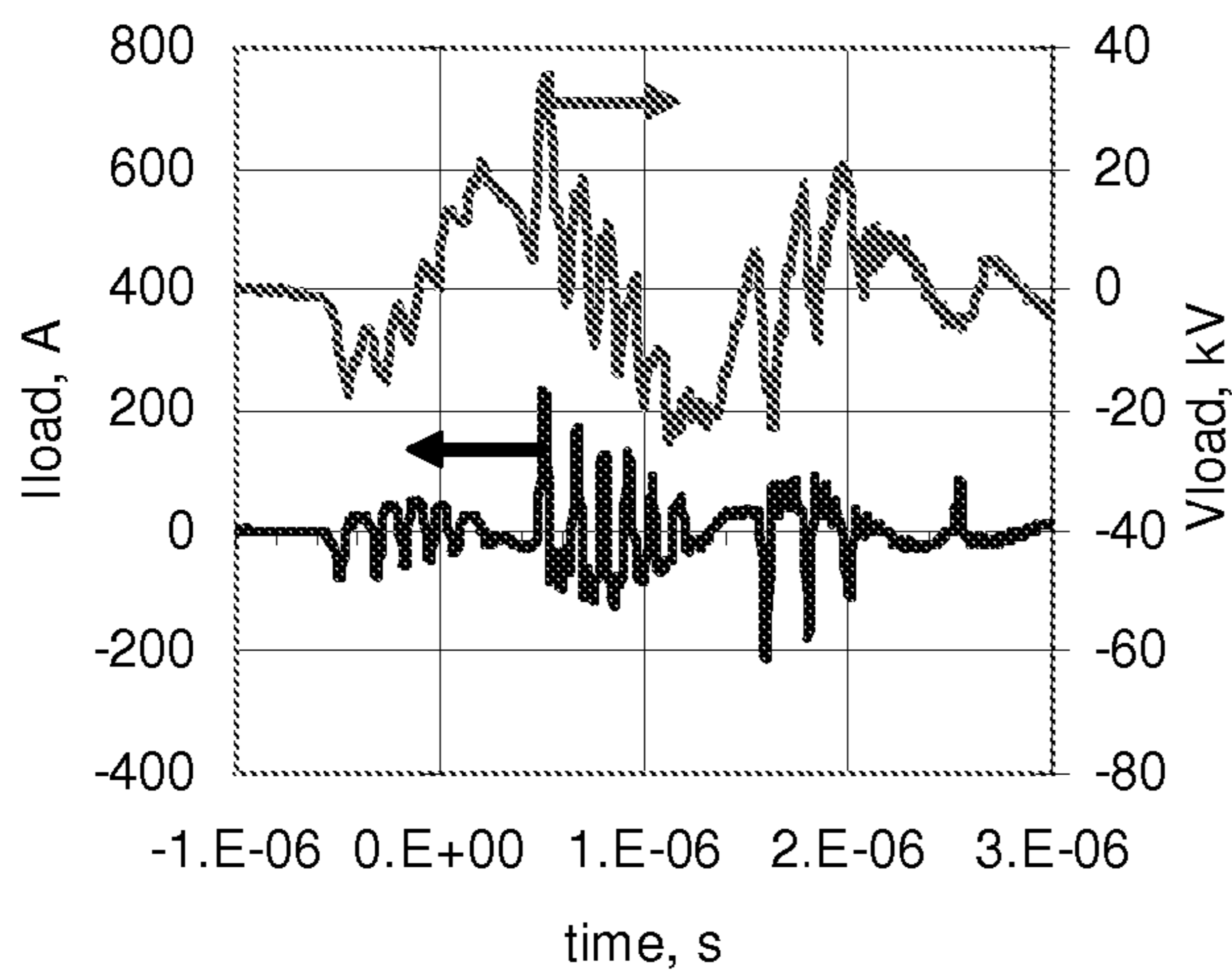
Fig. 3 – PRIOR ART
