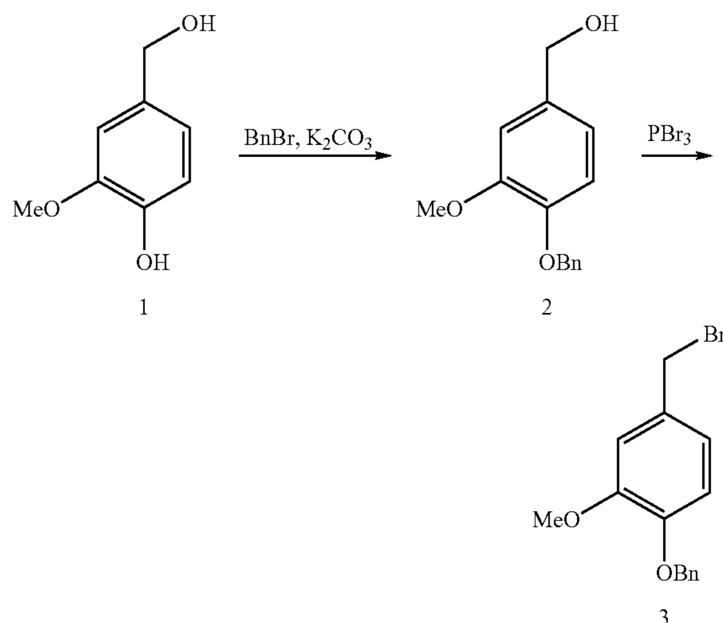
Scheme 2
