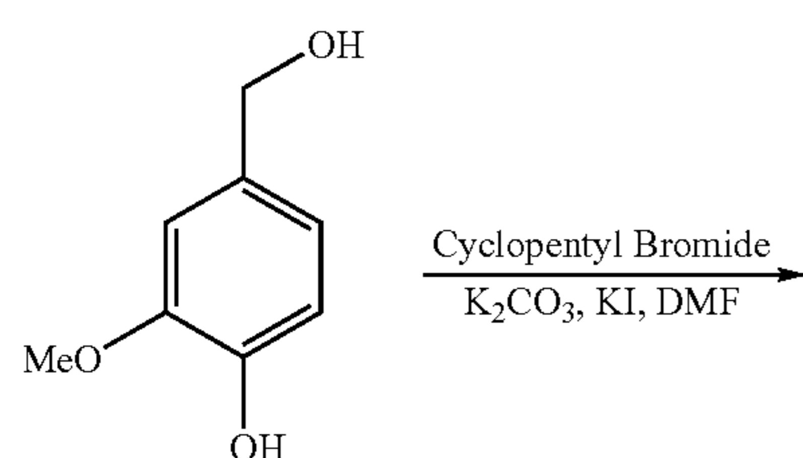
Scheme 11
