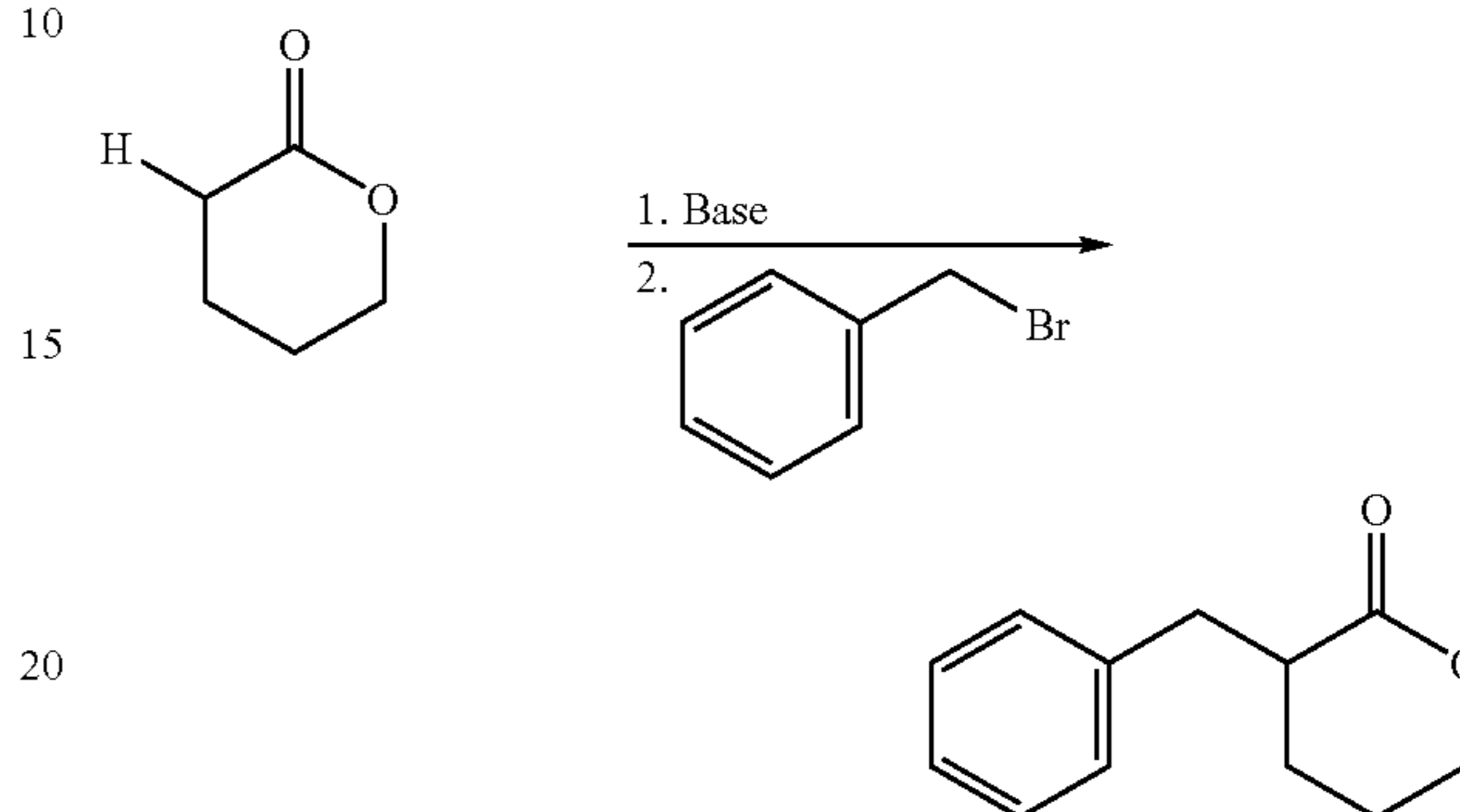
Scheme 1
