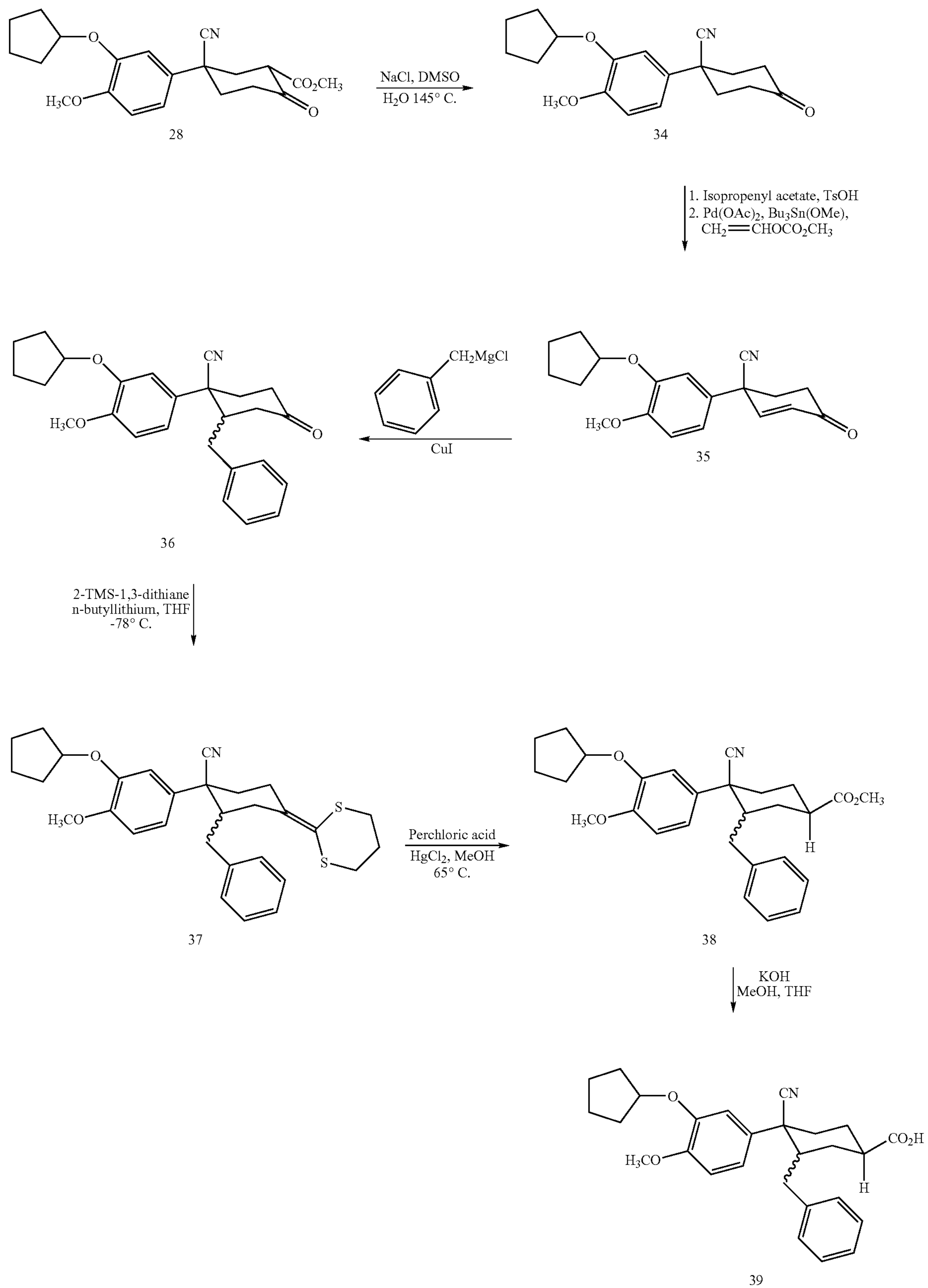
Scheme 9
