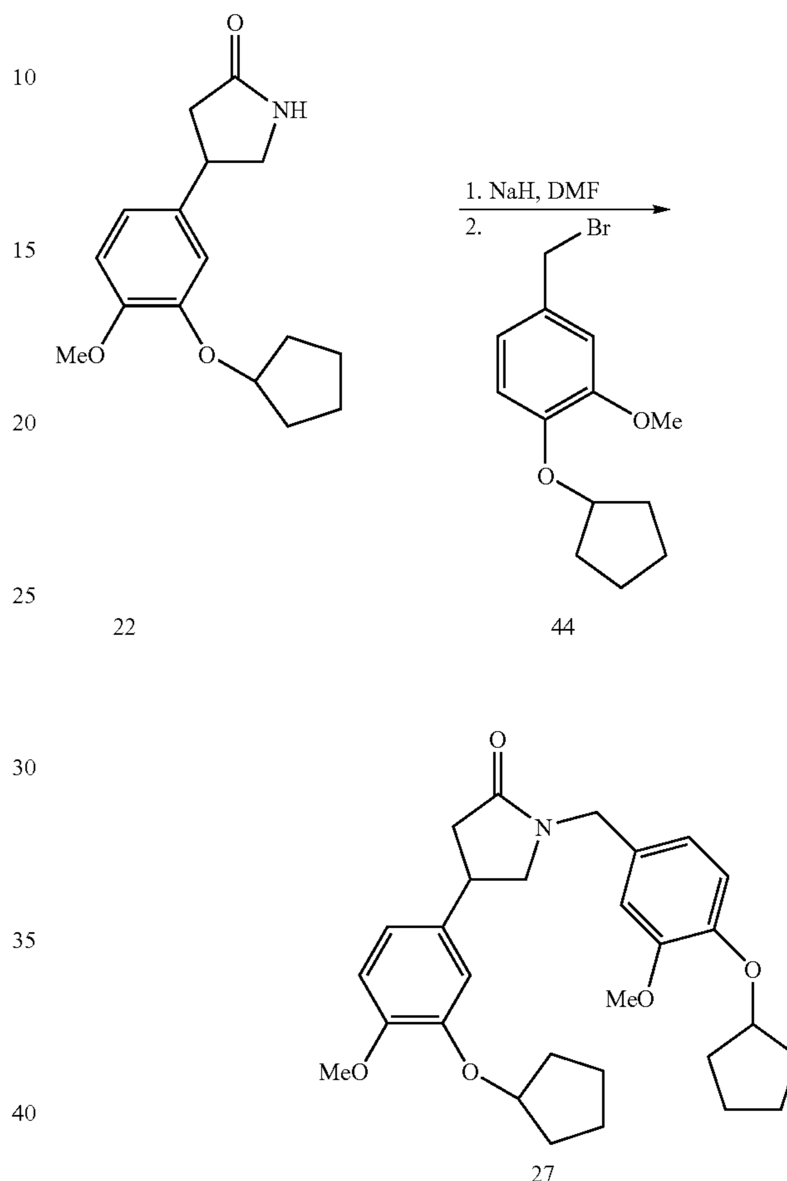
Scheme 7
