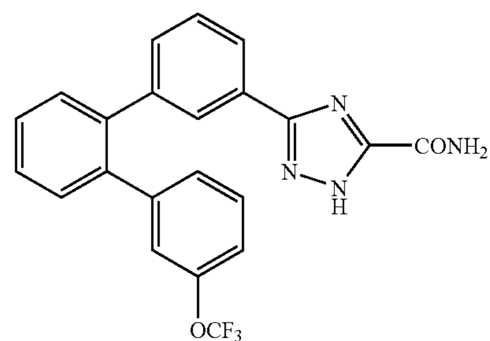
5-[2'-(3-Trifluoromethoxyphenyl)biphenyl-3-yl]2H-1,2,4-triazole-3-carboxamide
