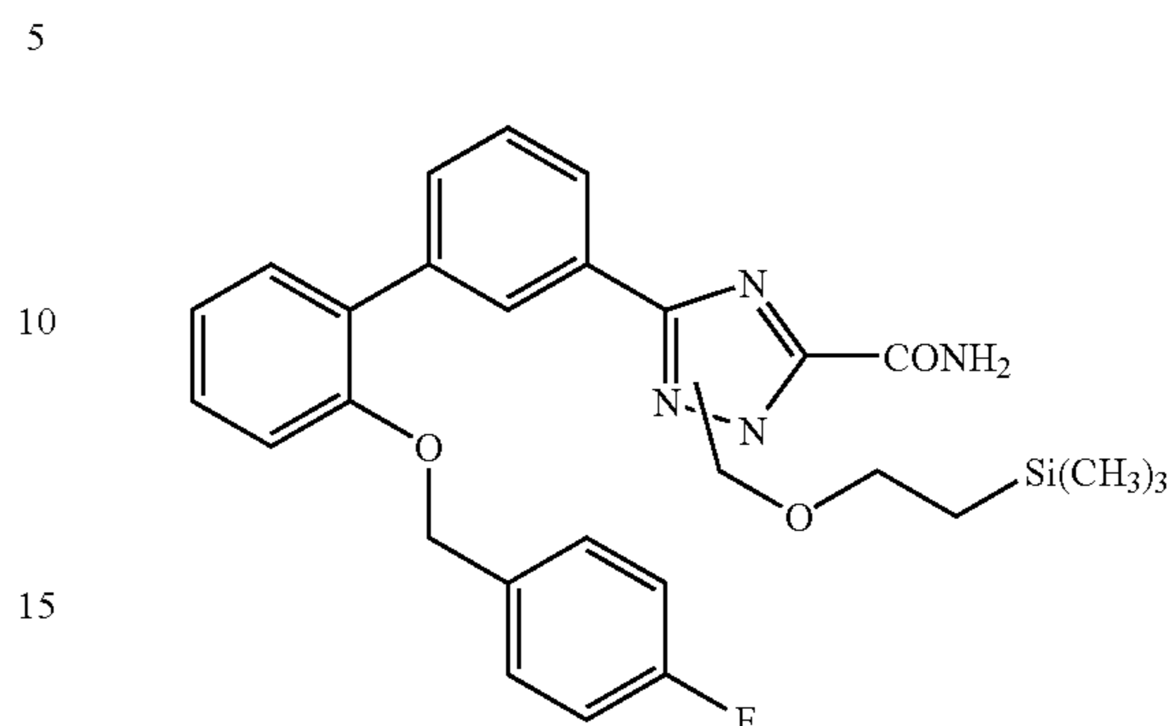
5-[5'-Fluoro-2'-(2,2,3,3,4,4,4-heptafluorobutyloxy)biphenyl-3-yl]2H-1,2,4-triazole-3-carboxylate
