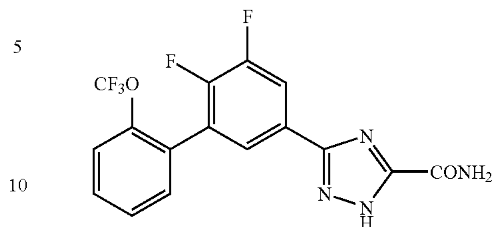
5-[5,6-Difluoro-2'-(trifluoromethoxy)biphenyl-3-yl] 2H-1,2,4-triazole-3-carboxamide
