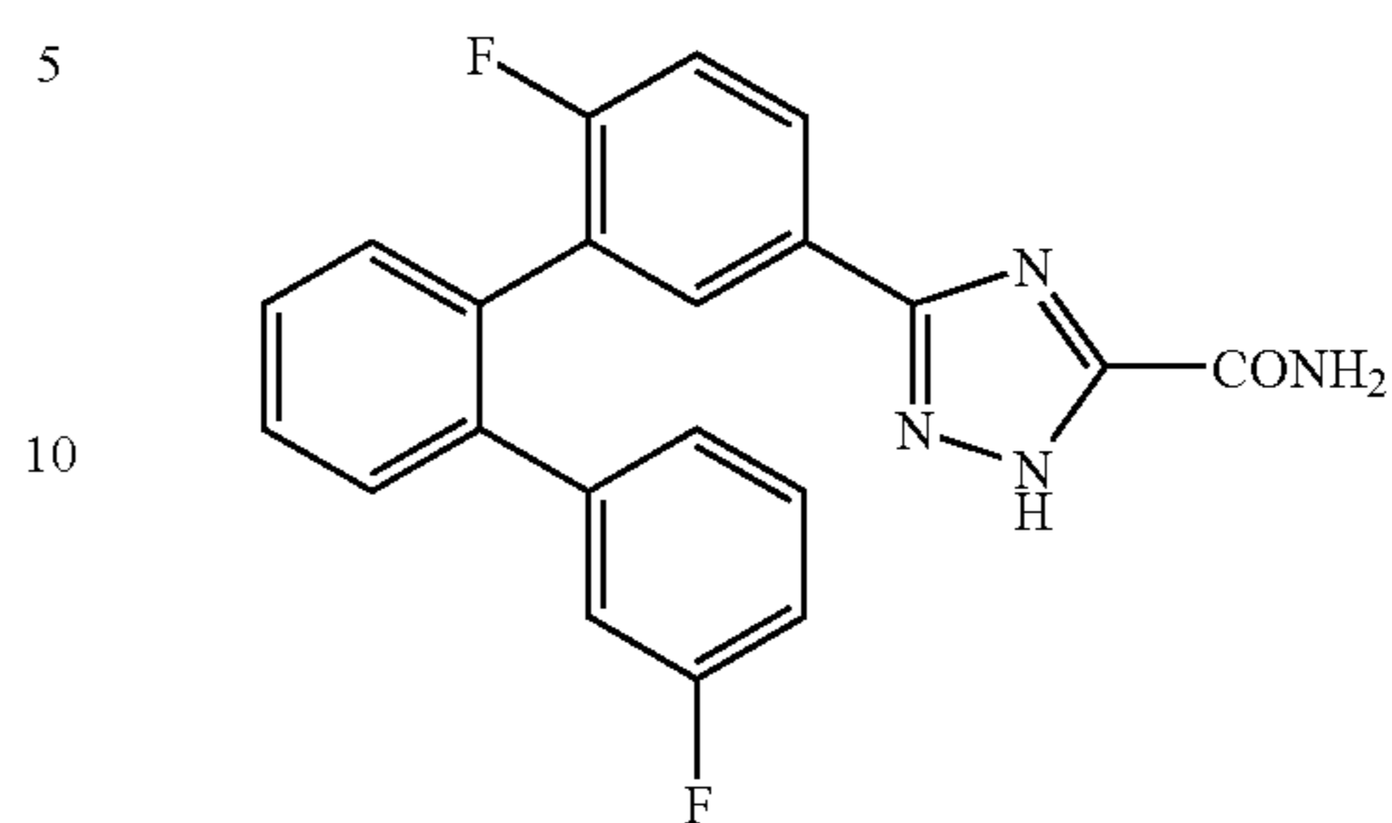
5-[6-Fluoro-2'-(3-fluorophenyl)biphenyl-3-yl]2H-1,2,4-triazole-3-carboxamide
