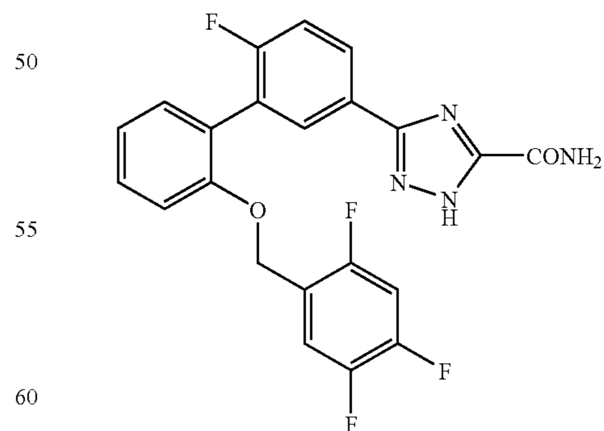
5-[6-Fluoro-2'-(2,4,5-trifluorobenzoyloxy)biphenyl-3-yl]2H-1,2,4-triazole-3-carboxamide
