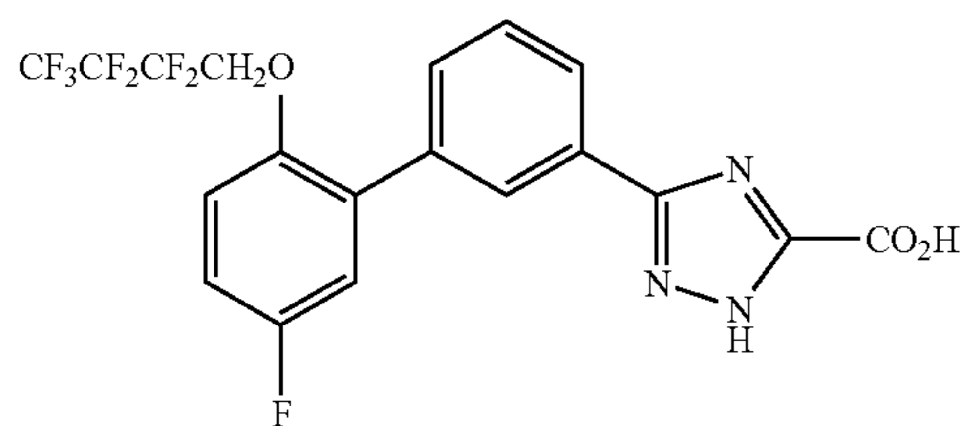
5-[5'-Fluoro-2'-(2,2,3,3,4,4,4-heptafluorobutyloxy)biphenyl-3-yl]2H-1,2,4-triazole-3-carboxylate
