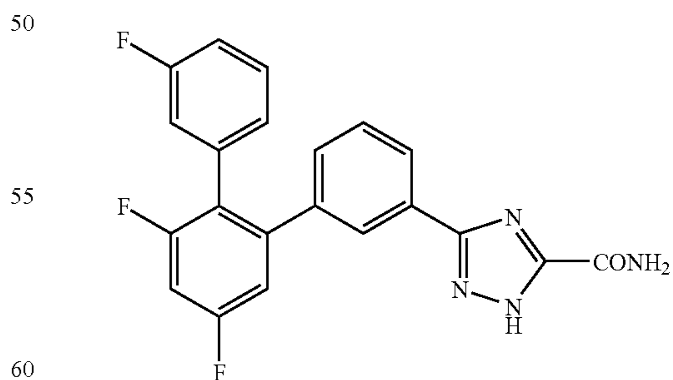
5-[3',5'-Difluoro-2'-(3-fluorophenyl)biphenyl-3-yl]2H-1,2,4-triazole-3-carboxamide
