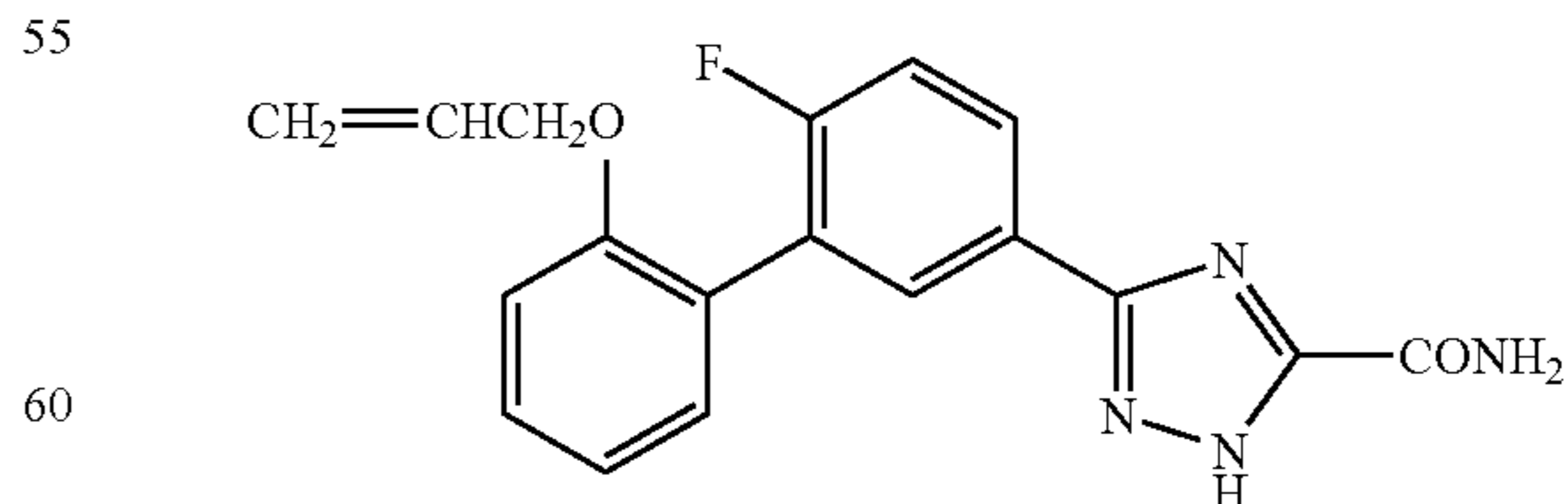
5-[6-Fluoro-2'-(allyloxy)biphenyl-3-yl]2H-1,2,4- triazole-3-carboxamide
