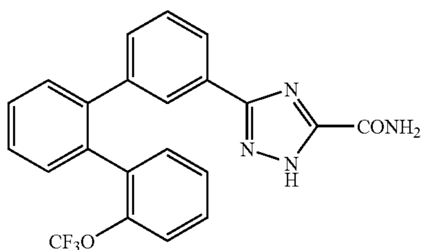
5-[2'-(2-Trifluoromethoxyphenyl)biphenyl-3-yl]2H-1,2,4-triazole-3-carboxamide
