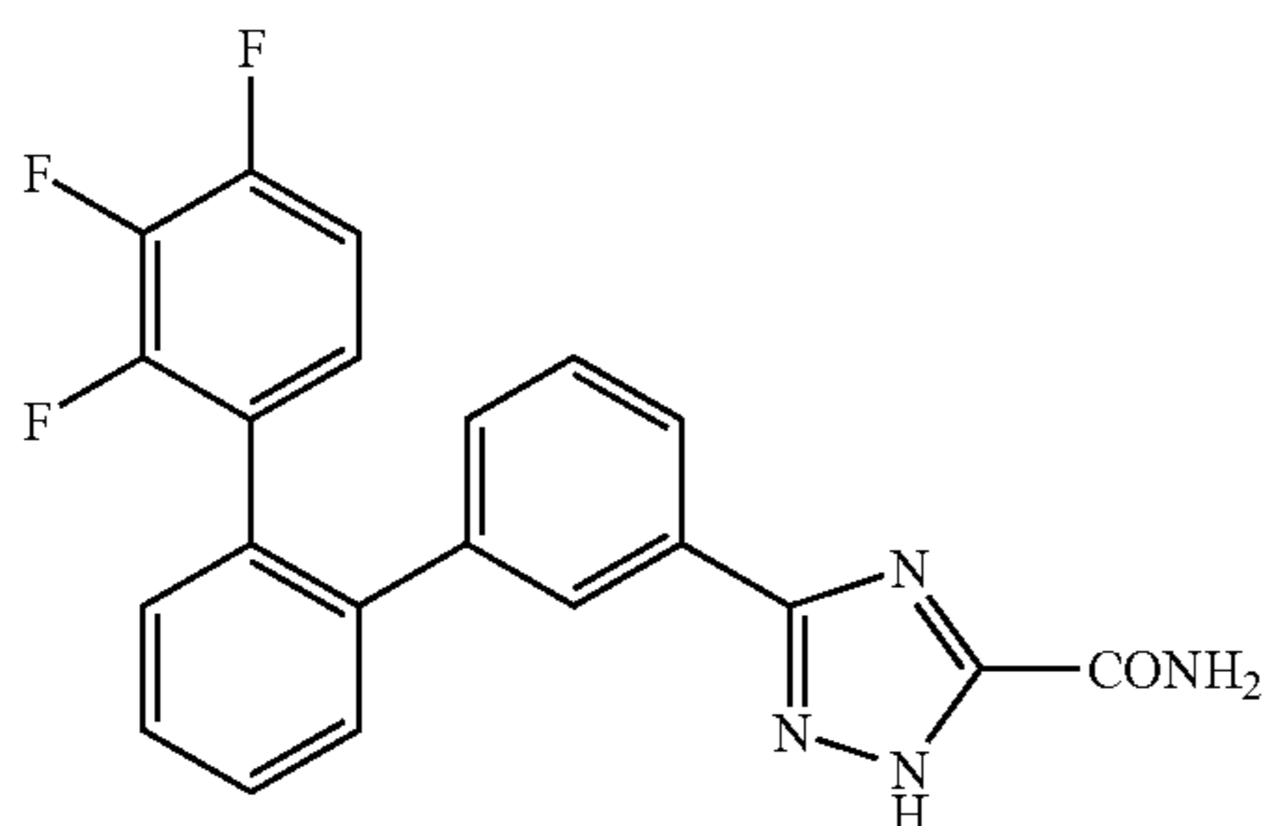
5-[2'-(2,3,4-Trifluorophenyl)biphenyl-3-yl]2H-1,2,4-triazole-3-carboxamide
