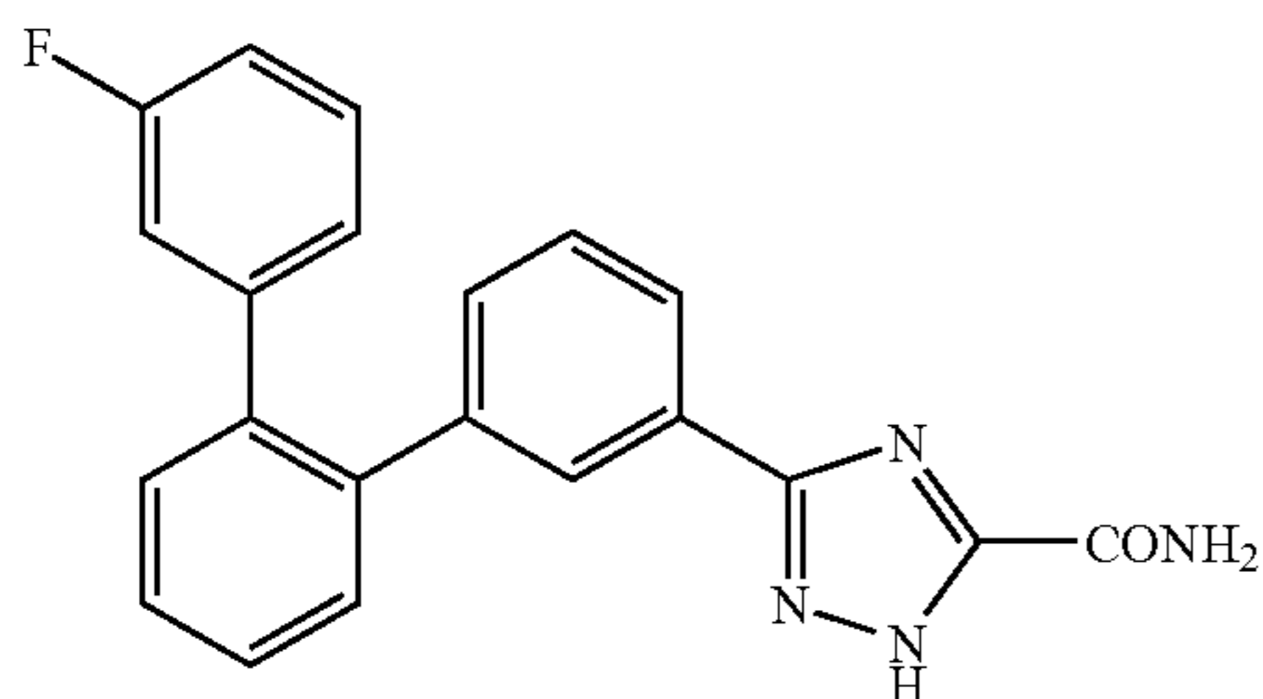
5-[2'-(3-Fluorophenyl)biphenyl-3-yl]2H-1,2,4-triazole-3-carboxamide
