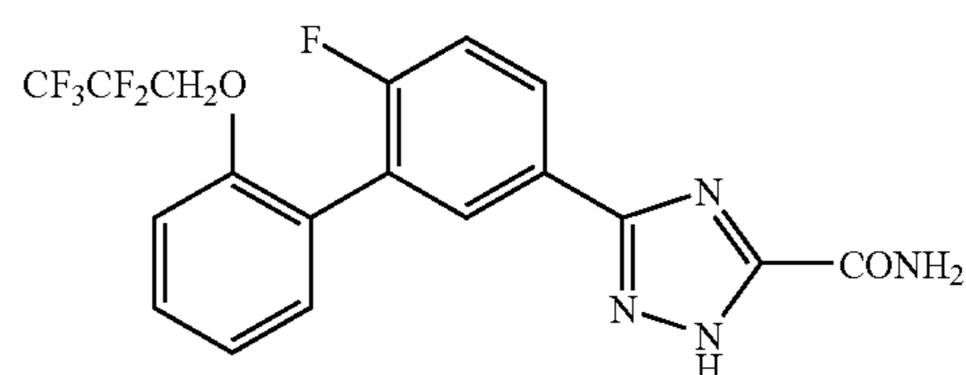
5-[6-Fluoro-2'-(2,2,3,3,3-pentafluoropropoxy)bi-phenyl-3-yl]2H-1,2,4-triazole-3-carboxamide
