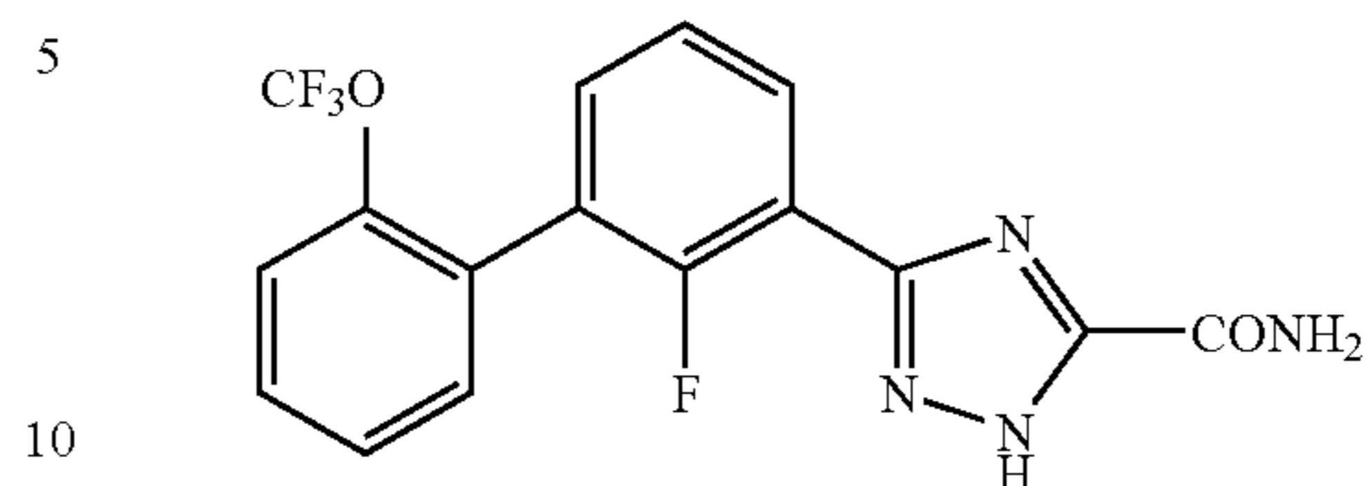
5-[2-Fluoro-2'-(trifluoromethoxy)biphenyl-3-yl]2H-1,2,4-triazole-3-carboxamide
