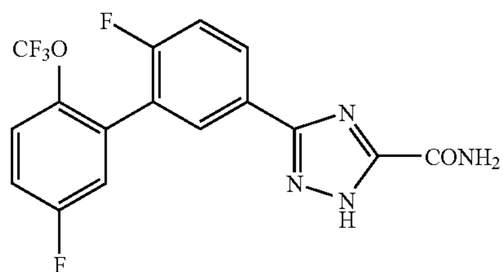
5-[5',6-Difluoro-2'-(trifluoromethoxy)biphenyl-3-yl] 2H-1,2,4-triazole-3-carboxamide
