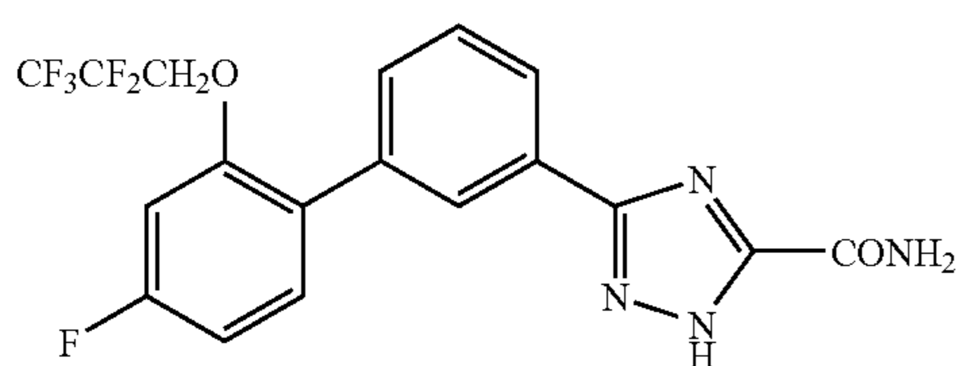
5-[4'-Fluoro-2'-(2,2,3,3,3-pentafluoropropoxy)biphenyl-3-yl]2H-1,2,4-triazole-3-carboxamide
