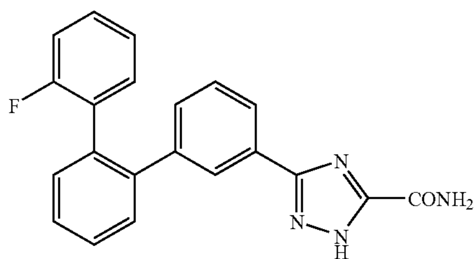
5-[2'-(2-Fluorophenyl)biphenyl-3-yl]2H-1,2,4-triazole-3-carboxamide
