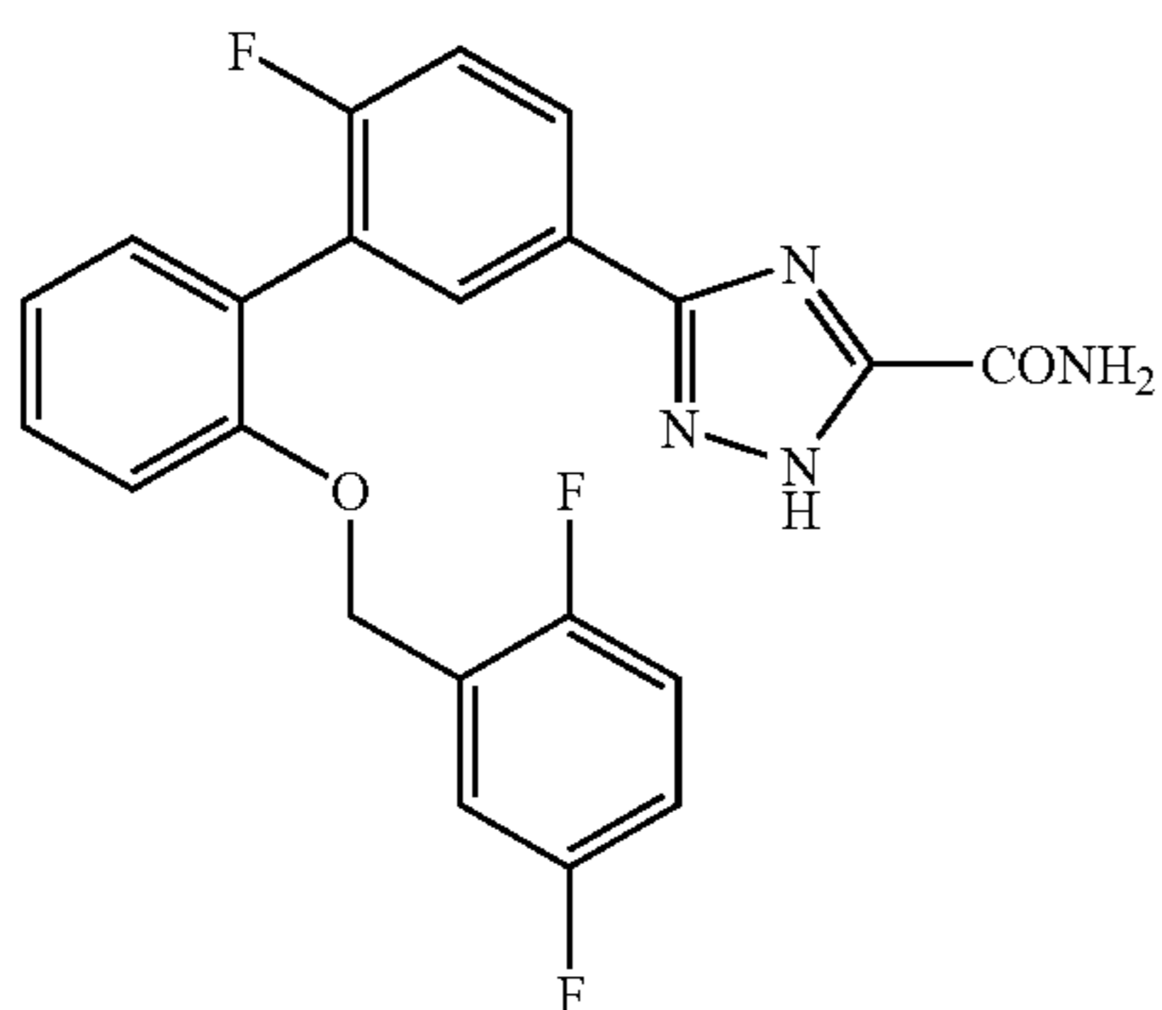
5-[6-Fluoro-2'-(2,5-difluorobenzoyloxy)biphenyl-3-yl]2H-1,2,4-triazole-3-carboxamide
