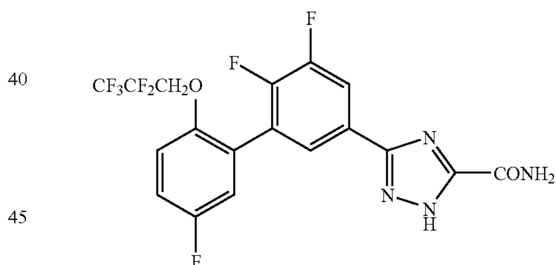
5-[5,5',6-Trifluoro-2'-(2,2,3,3,3-pentafluoropropoxy) biphenyl-3-yl]2H-1,2,4-triazole-3-carboxamide
