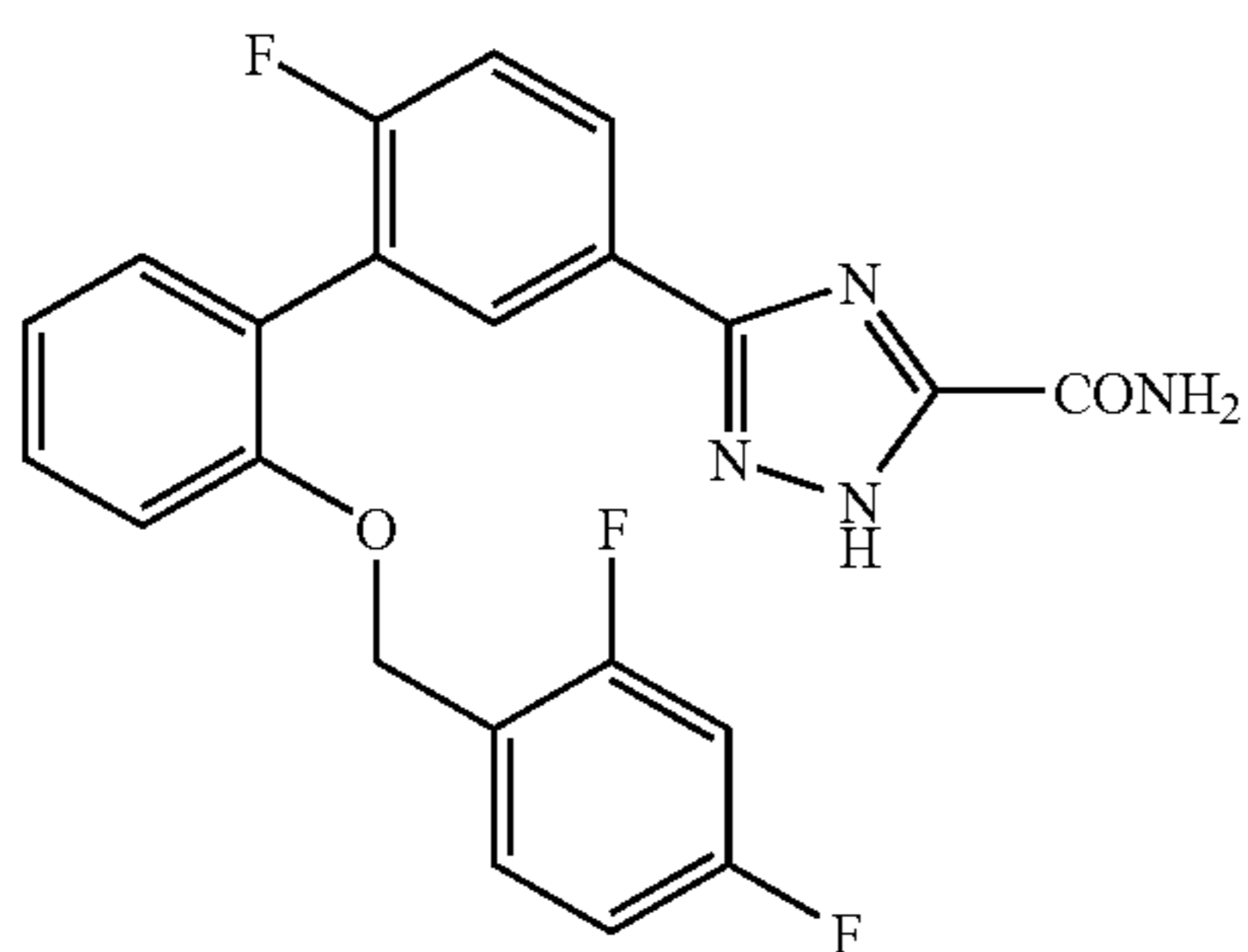
5-[6-Fluoro-2'-(2,4-difluorobenzoyloxy)biphenyl-3-yl]2H-1,2,4-triazole-3-carboxamide
