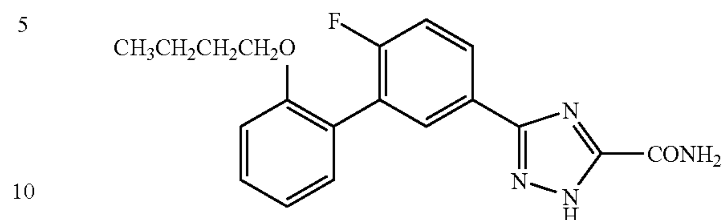
5-[6-Fluoro-2'-(n-butyloxy)biphenyl-3-yl]2H-1,2,4- triazole-3-carboxamide
