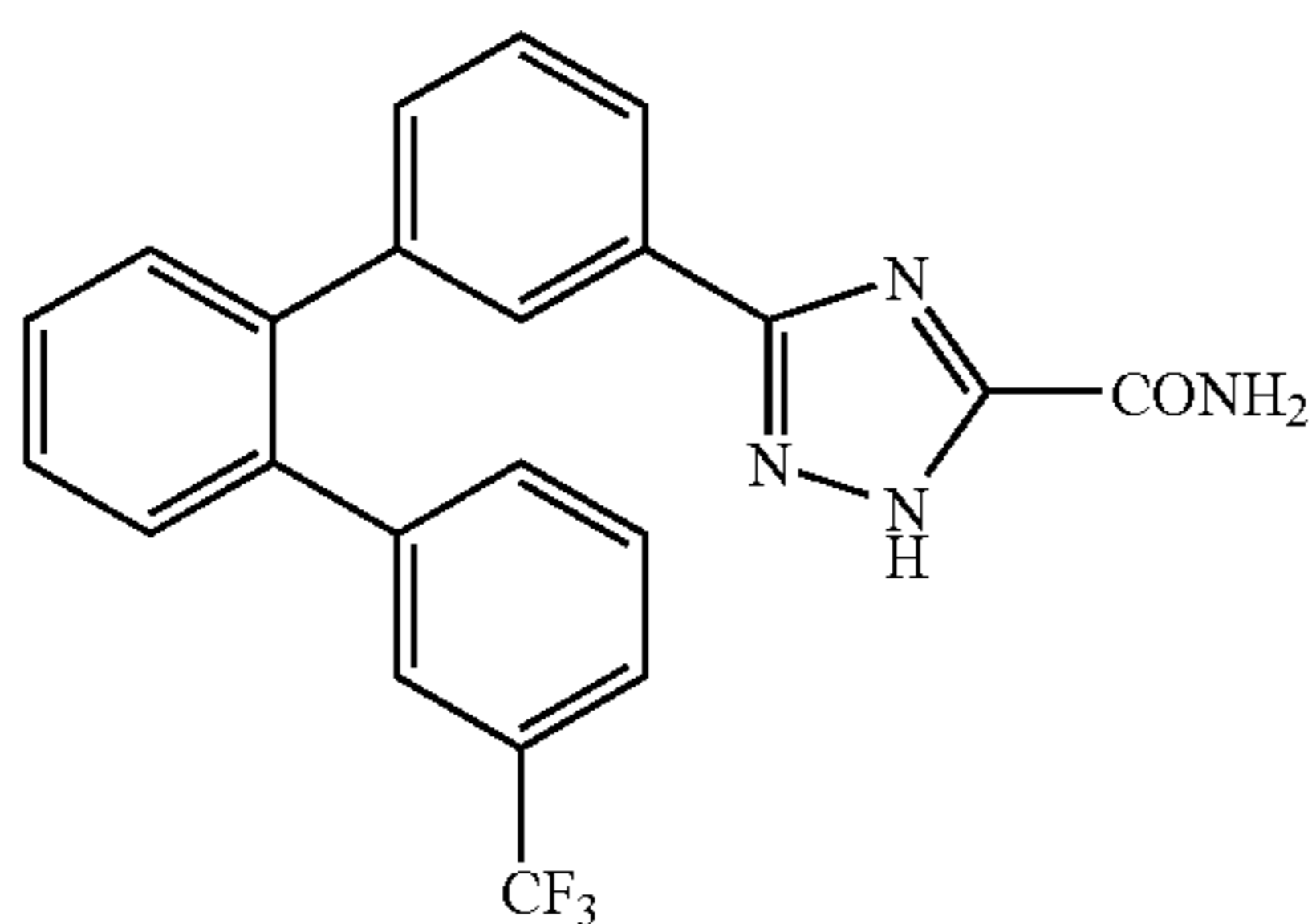
5-[2'-(3-Trifluoromethylphenyl)biphenyl-3-yl]2H-1,2,4-triazole-3-carboxamide
