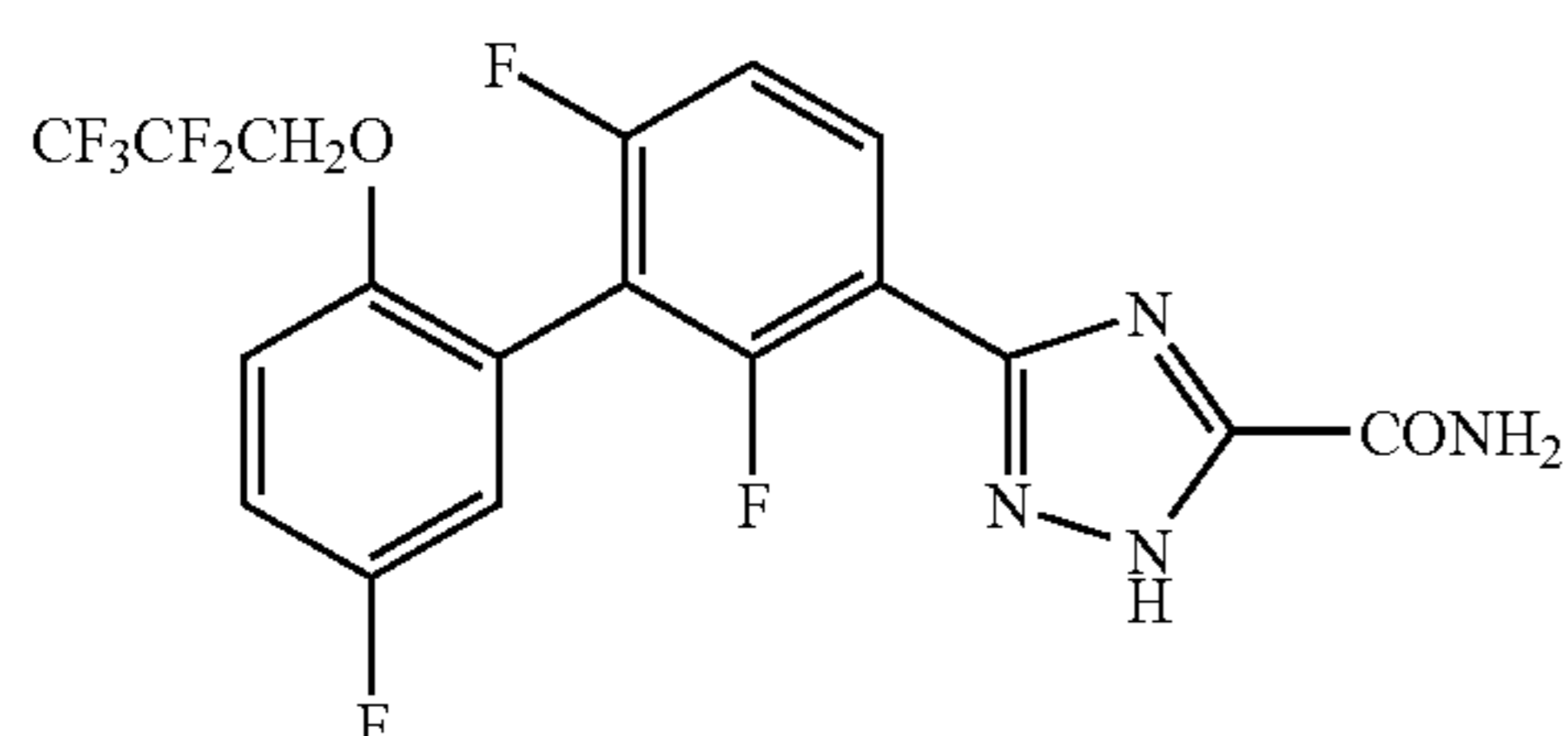
5-[2,5',6-Trifluoro-2'-(2,2,3,3,3-pentafluoropropoxy) biphenyl-3-yl]2H-1,2,4-triazole-3-carboxamide
