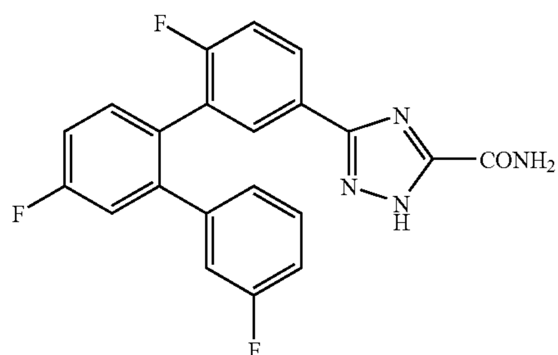
5-[6-Fluoro-4'-fluoro-2'-(3-fluorophenyl)biphenyl-3-yl]2H-1,2,4-triazole-3-carboxamide
