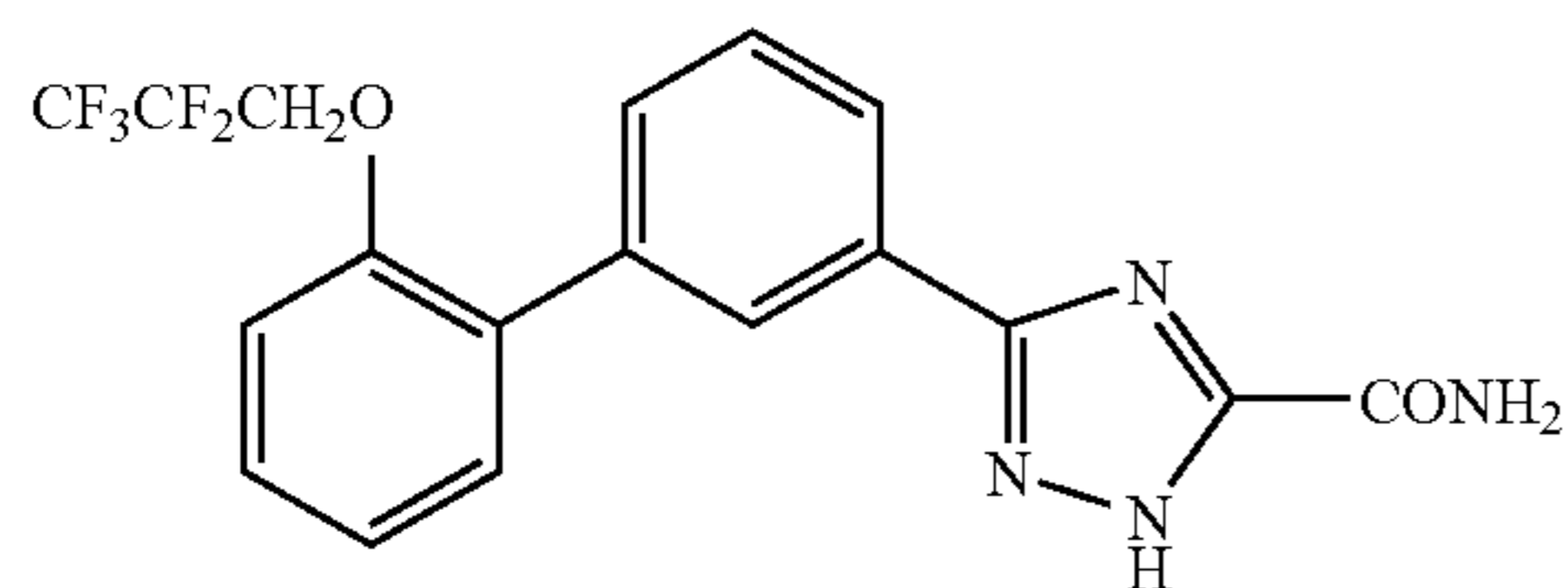
5-[2'-(2,2,3,3,3-pentafluoropropoxy)biphenyl-3-yl] 2H-1,2,4-triazole-3-carboxamide
