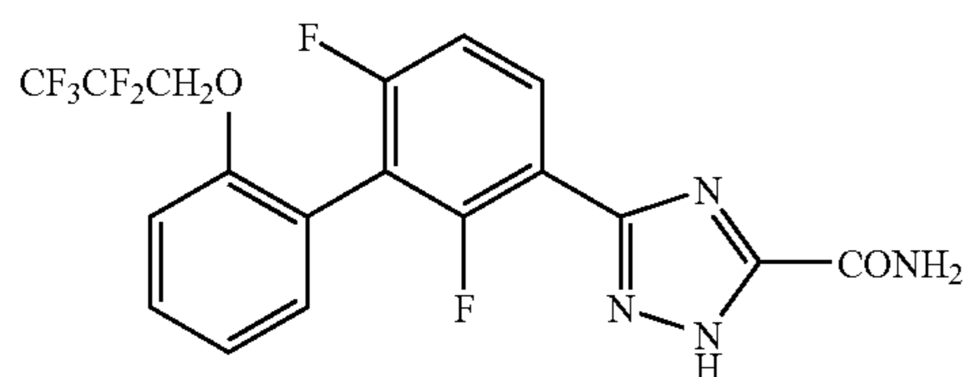
5-[2,6-Difluoro-2'-(2,2,3,3,3-pentafluoropropoxy) biphenyl-3-yl]2H-1,2,4-triazole-3-carboxamide
