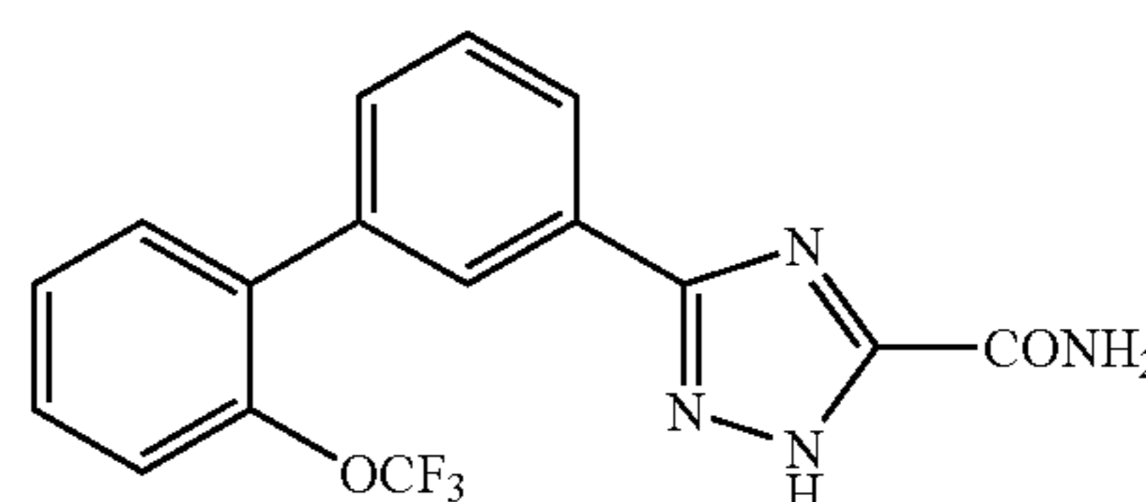
3-[3-((2-Trifluoromethoxy)phenyl)phenyl]-1,2,4-triazole-5-carboxamide
