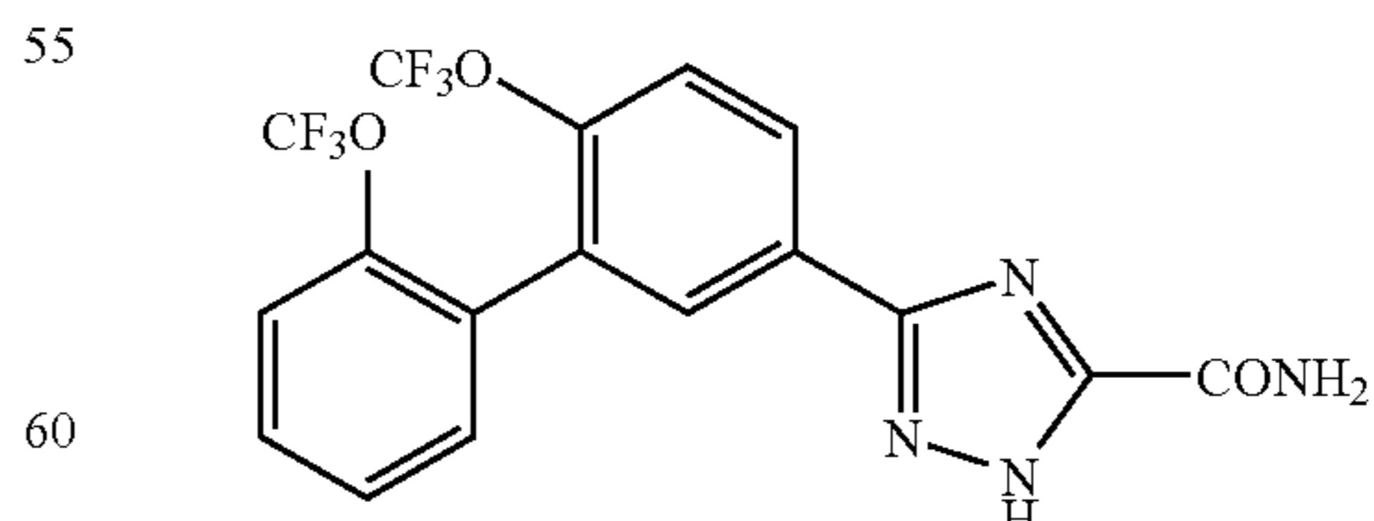
5-[2',6'-Bis(trifluoromethoxy)biphenyl-3-yl]2H-1,2,4-triazole-3-carboxamide
