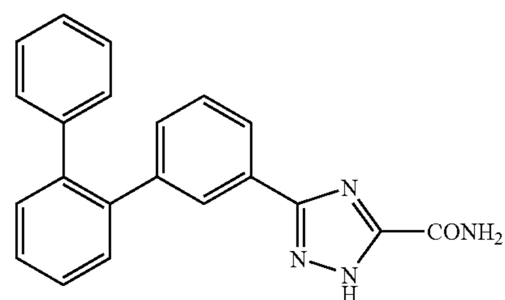
5-[2'-(Phenyl)biphenyl-3-yl]2H-1,2,4-triazole-3-carboxamide
