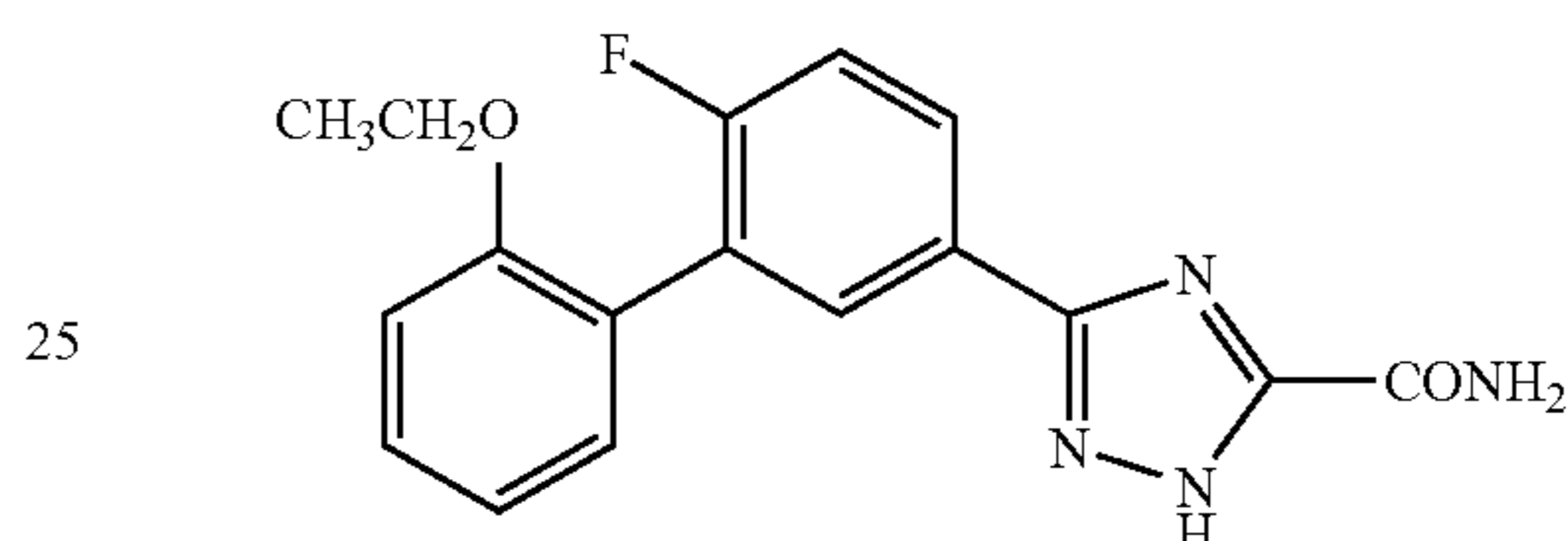
5-[6-Fluoro-2'-(ethoxy)biphenyl-3-yl]2H-1,2,4-triazole-3-carboxamide
