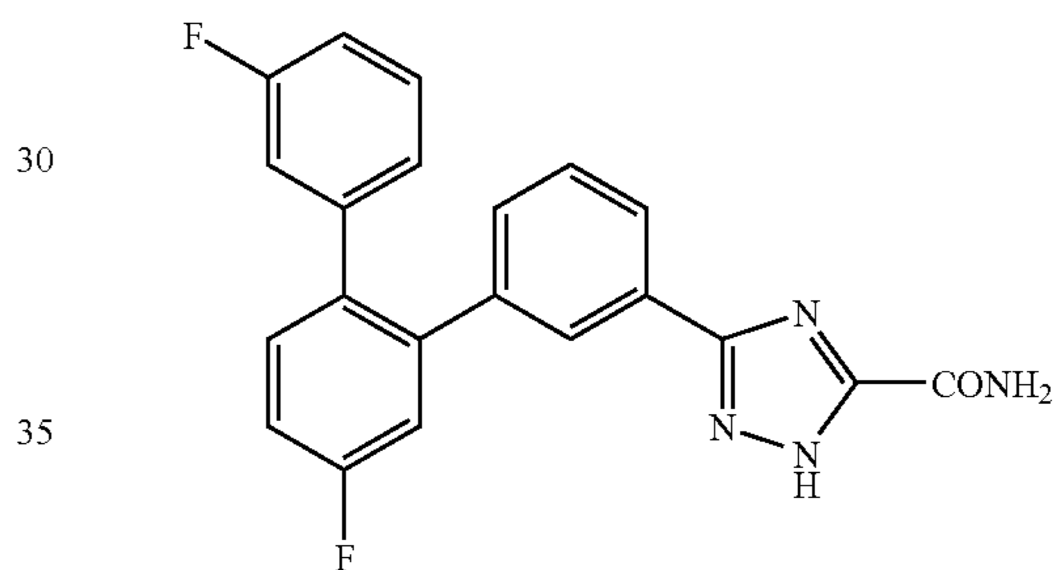
5-[5'-Fluoro-2'-(3-fluorophenyl)biphenyl-3-yl]2H-1,2,4-triazole-3-carboxamide
