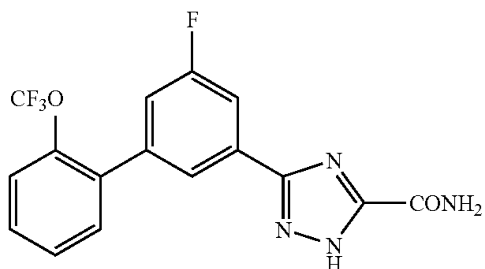
5-[5-Fluoro-2'-(trifluoromethoxy)biphenyl-3-yl]2H-1,2,4-triazole-3-carboxamide
