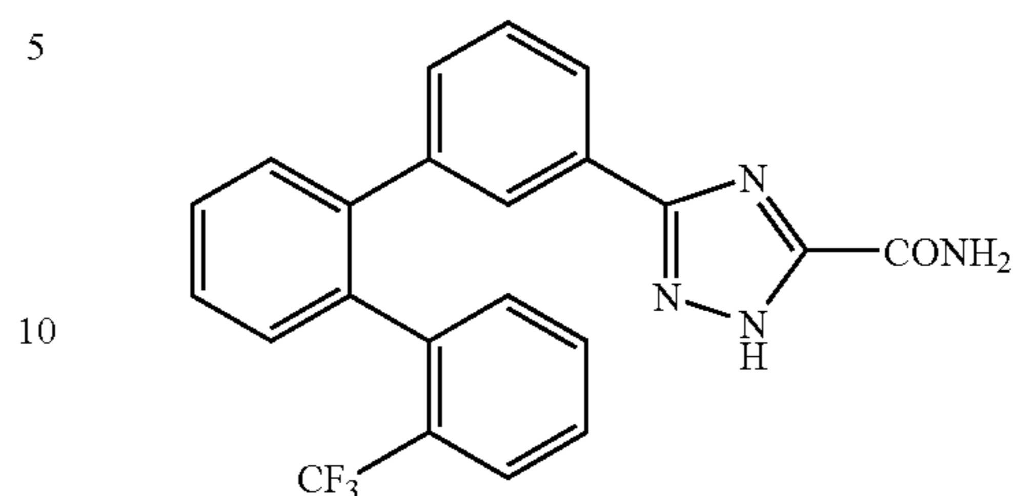
5-[2'-(2-trifluoromethylphenyl)biphenyl-3-yl]2H-1,2,4-triazole-3-carboxamide
