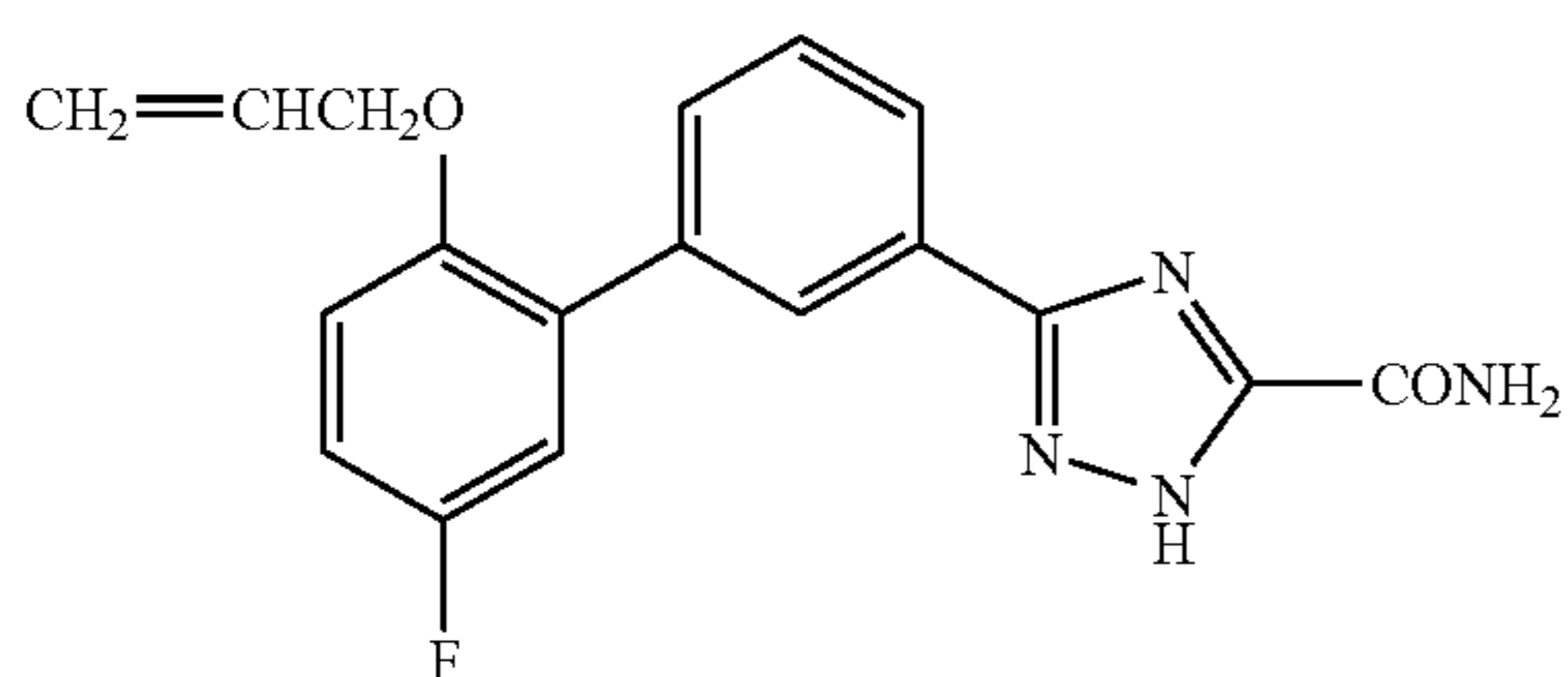
5-[5'-Fluoro-2'-(allyloxy)biphenyl-3-yl]2H-1,2,4-triazole-3-carboxamide
