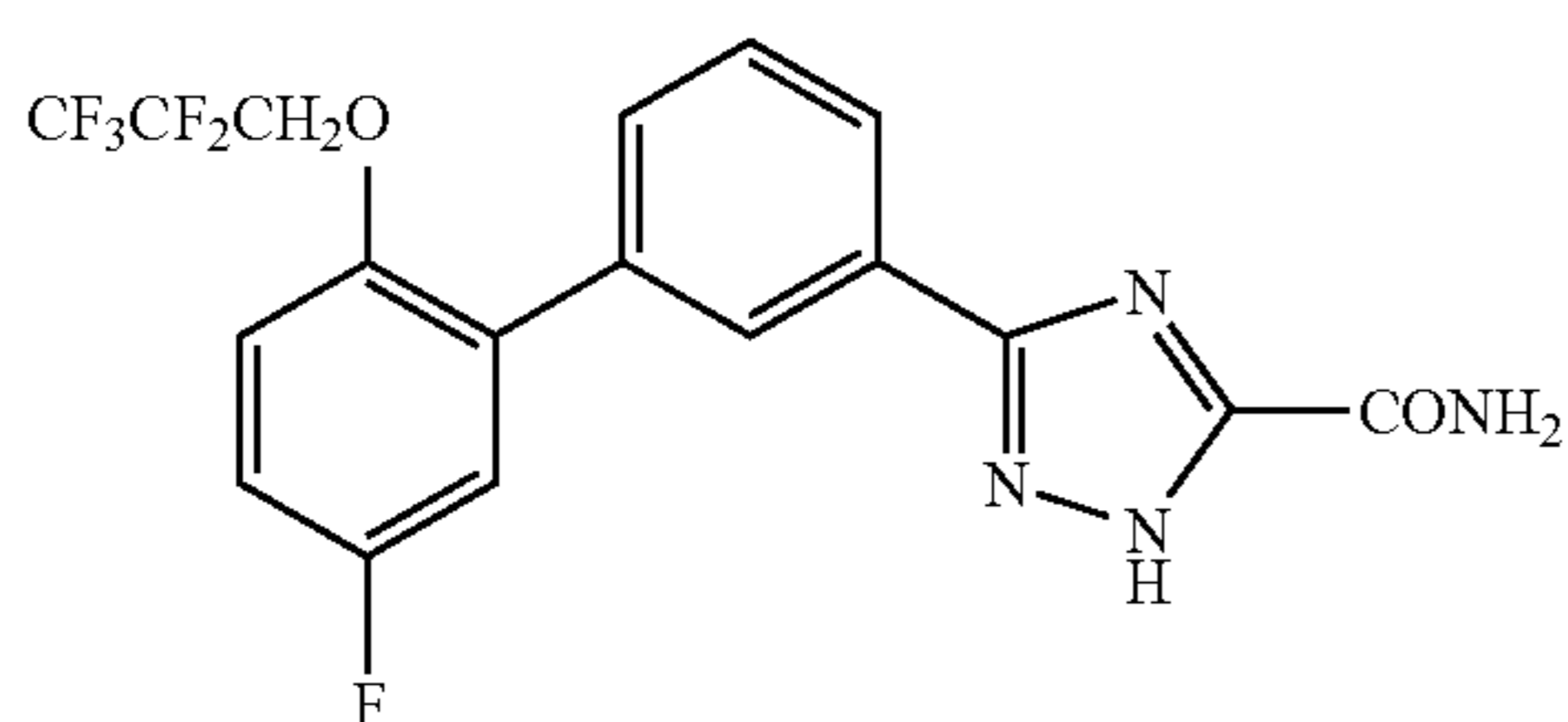
5-[5'-Fluoro-2'-(2,2,3,3,3-pentafluoropropoxy)biphenyl-3-yl]2H-1,2,4-triazole-3-carboxamide
