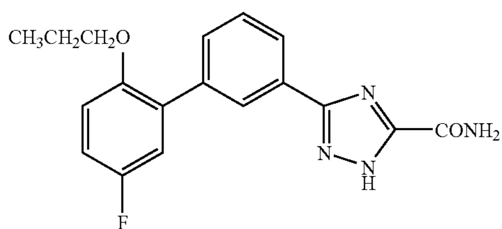
5-[5'-Fluoro-2'-(n-propyloxy)biphenyl-3-yl]2H-1,2,4-triazole-3-carboxamide
