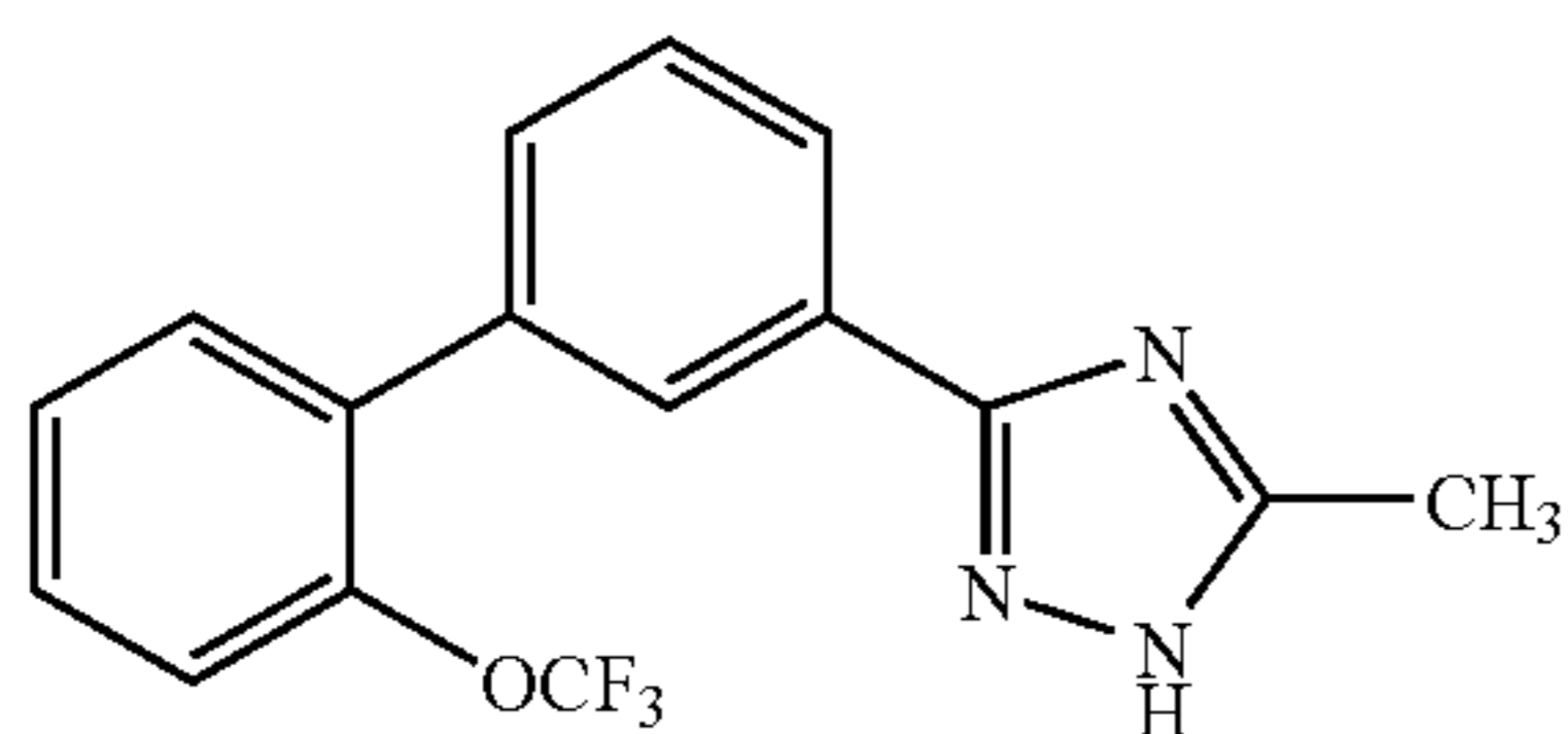
5-Methyl-3-[3-((2-trifluoromethoxy)phenyl)phenyl]-1,2,4-triazole
