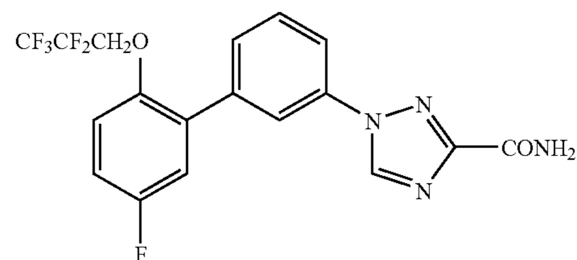
1-[5'-Fluoro-2'-(2,2,3,3,3-pentafluoropropoxy)biphenyl-3-yl]-1,2,4-triazole-3-carboxamide
