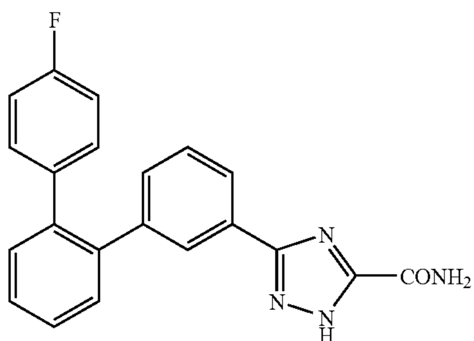
5-[2'-(4-Fluorophenyl)biphenyl-3-yl]2H-1,2,4-triazole-3-carboxamide
