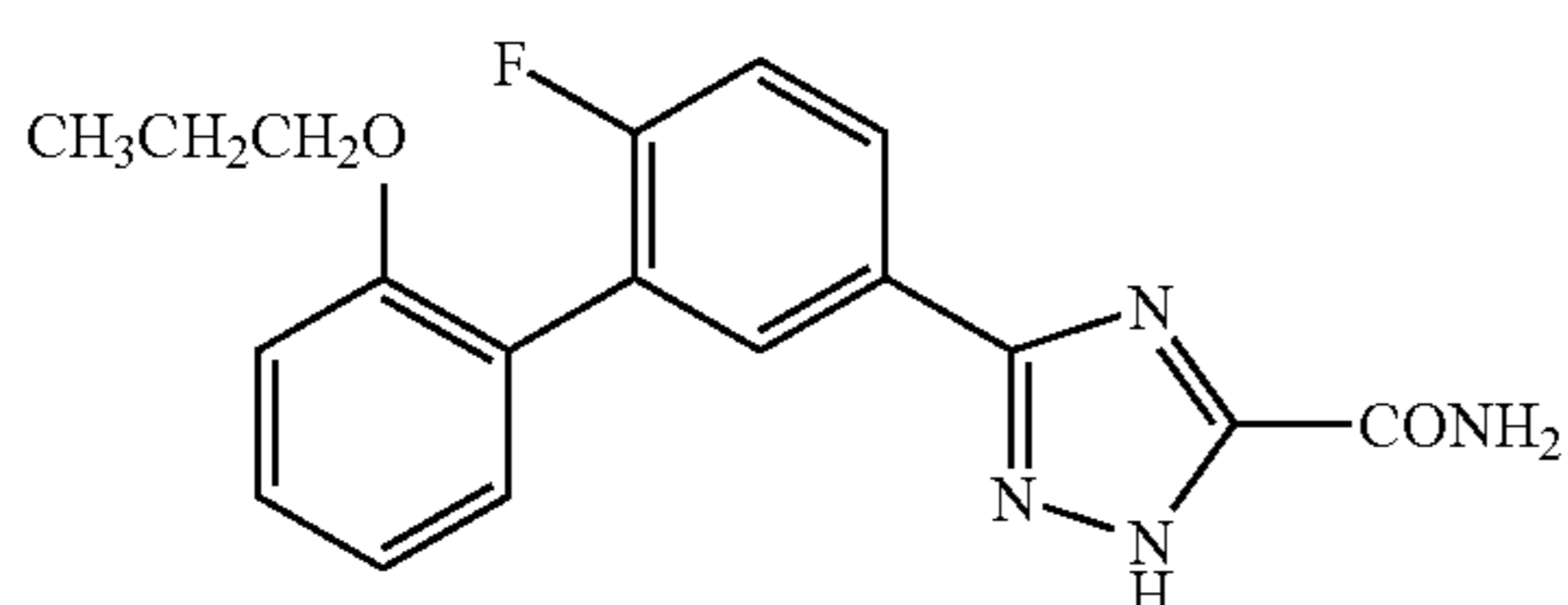
5-[6-Fluoro-2'-(n-propyloxy)biphenyl-3-yl]2H-1,2,4-triazole-3-carboxamide
