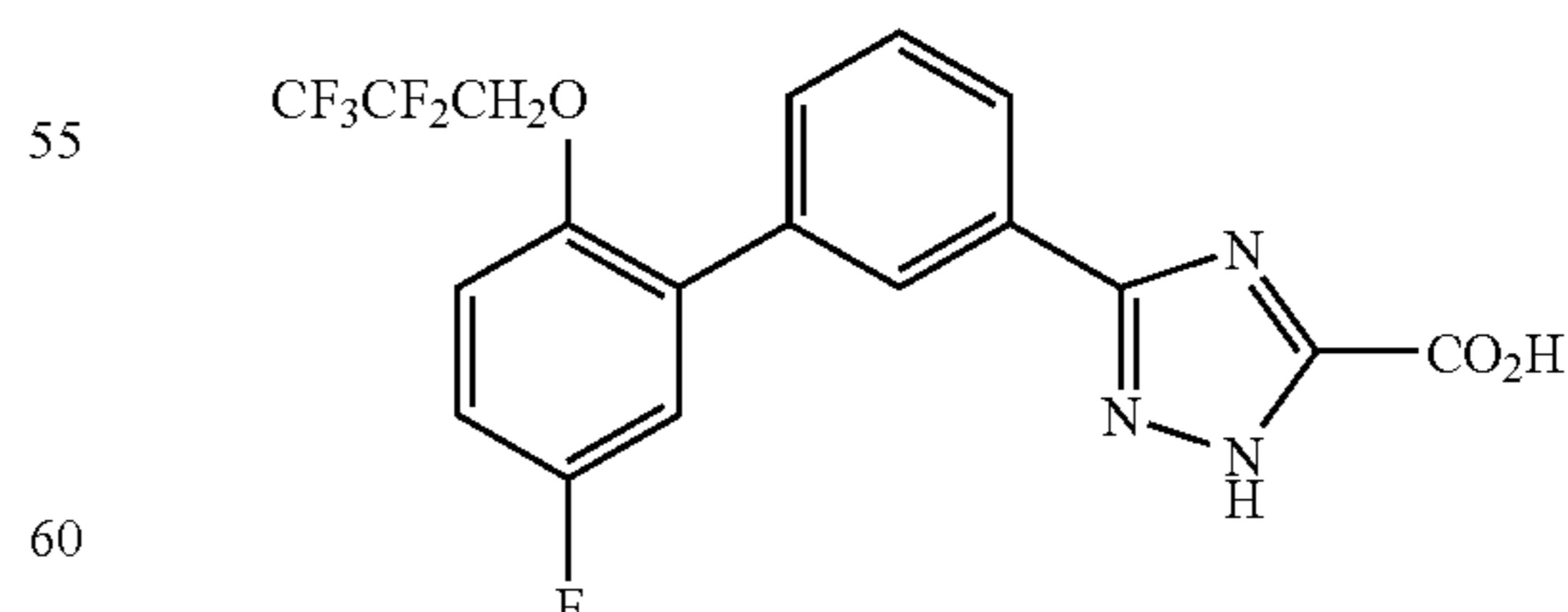
5-[5'-Fluoro-2'-(2,2,3,3,3-pentafluoropropoxy) biphenyl-3-yl]2H-1,2,4-triazole-3-carboxylate
