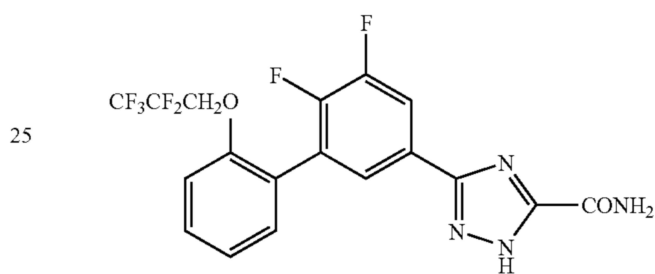
5-[5,6-Difluoro-2'-(2,2,3,3,3-pentafluoropropoxy) biphenyl-3-yl]2H-1,2,4-triazole-3-carboxamide
