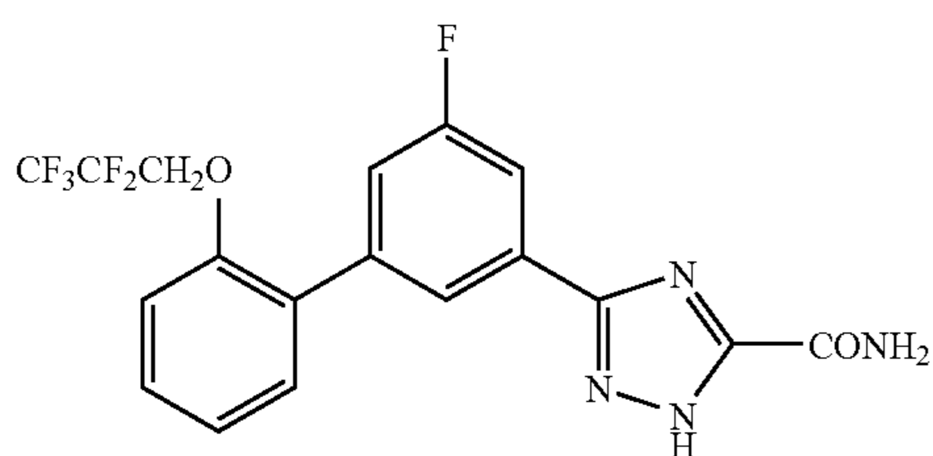
5-[5-Fluoro-2'-(2,2,3,3,3-pentafluoropropoxy)biphenyl-3-yl]2H-1,2,4-triazole-3-carboxamide
