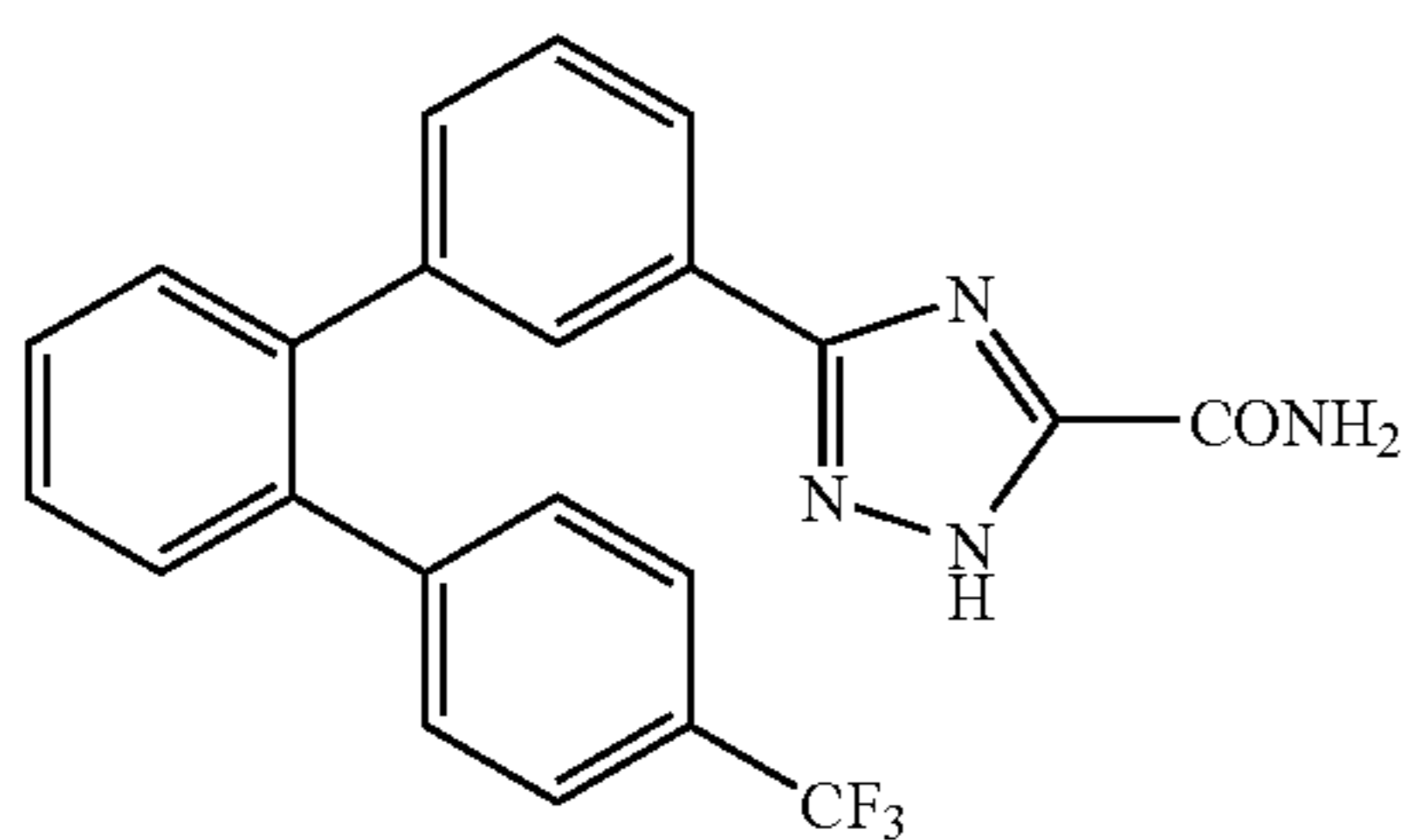
5-[2'-(4-Trifluoromethylphenyl)biphenyl-3-yl]2H-1,2,4-triazole-3-carboxamide
