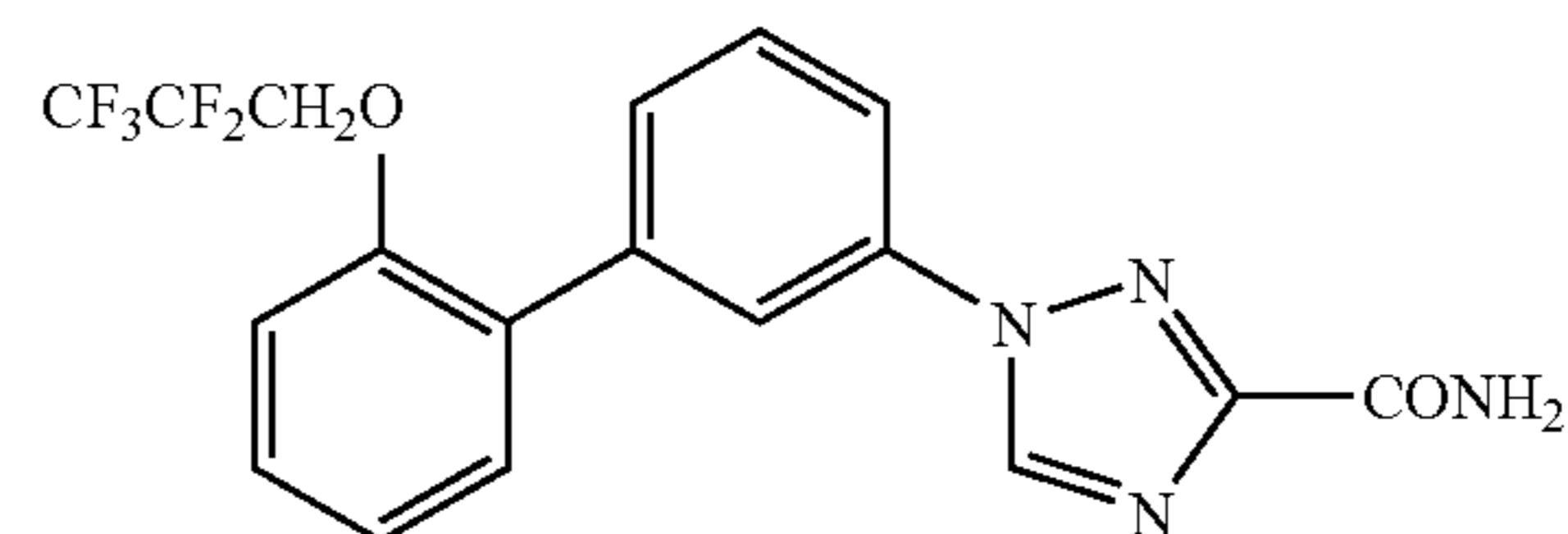
1-[2'-(2,2,3,3,3-Pentafluoropropoxy)biphenyl-3-yl]-1,2,4-triazole-3-carboxamide
