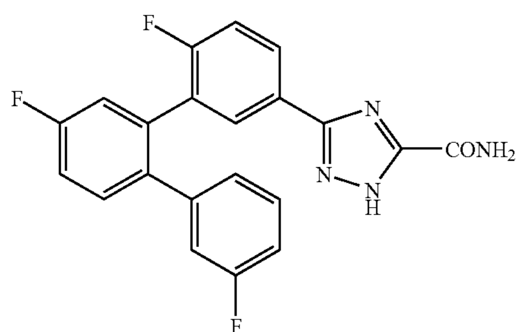
5-[6-Fluoro-5'-fluoro-2'-(3-fluorophenyl)biphenyl-3-yl]2H-1,2,4-triazole-3-carboxamide
