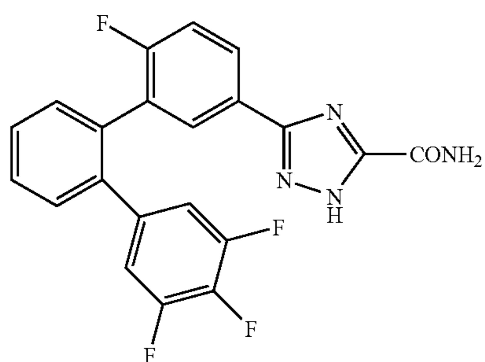
5-[6-Fluoro-2'-(3,4,5-trifluorophenyl)biphenyl-3-yl] 2H-1,2,4-triazole-3-carboxamide
