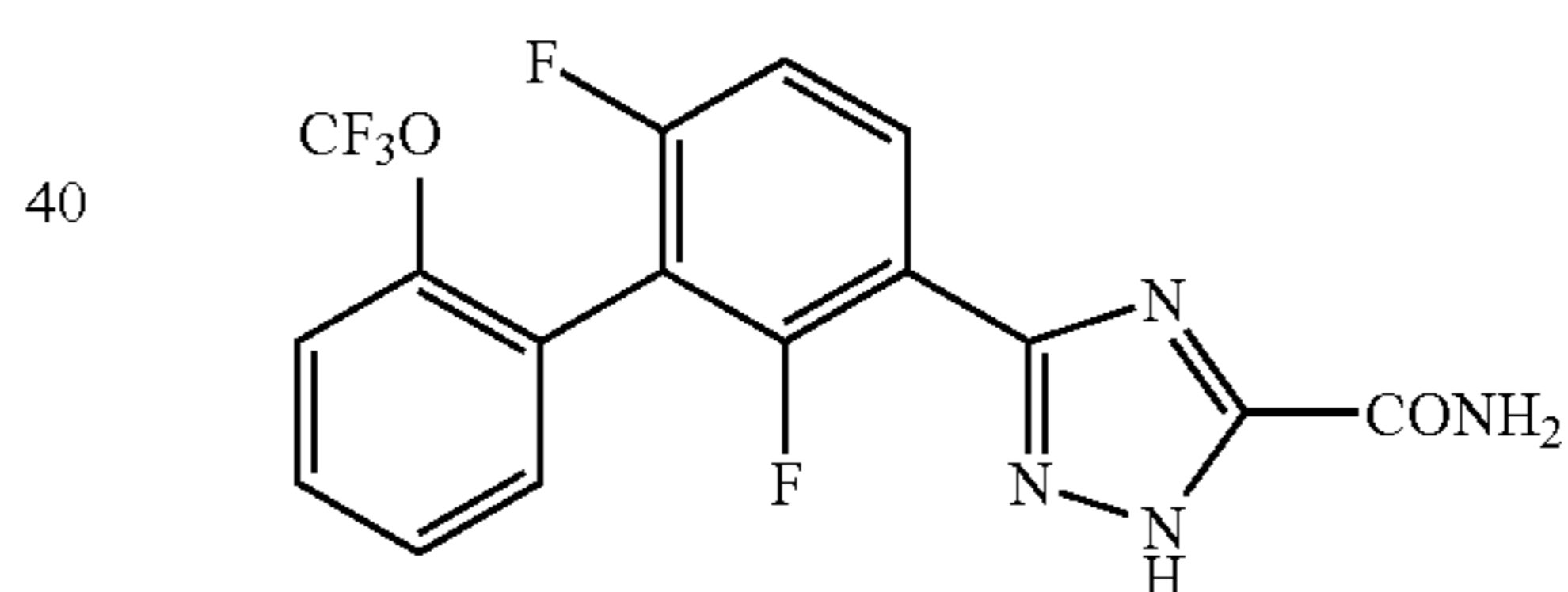
5-[2,6-Difluoro-2'-(trifluoromethoxy)biphenyl-3-yl]2H-1,2,4-triazole-3-carboxamide
