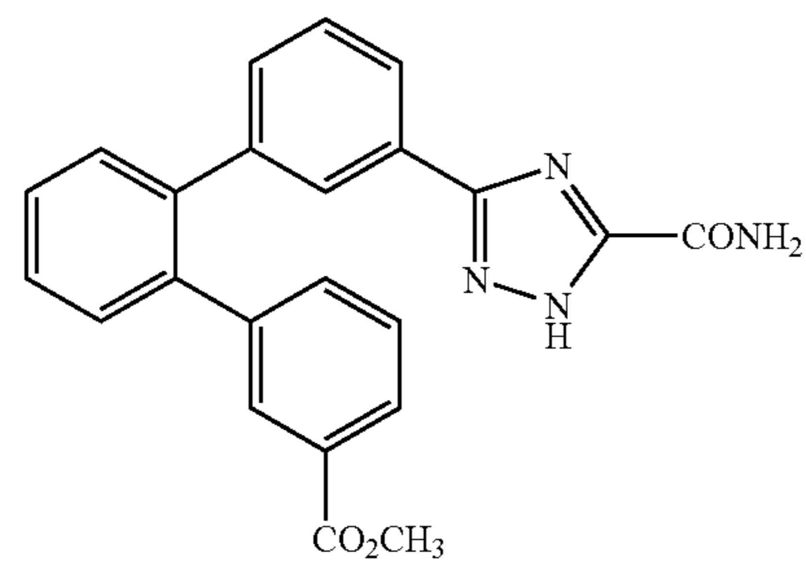
5-[2'-(3-Carbomethoxyphenyl)biphenyl-3-yl]2H-1,2,4-triazole-3-carboxamide
