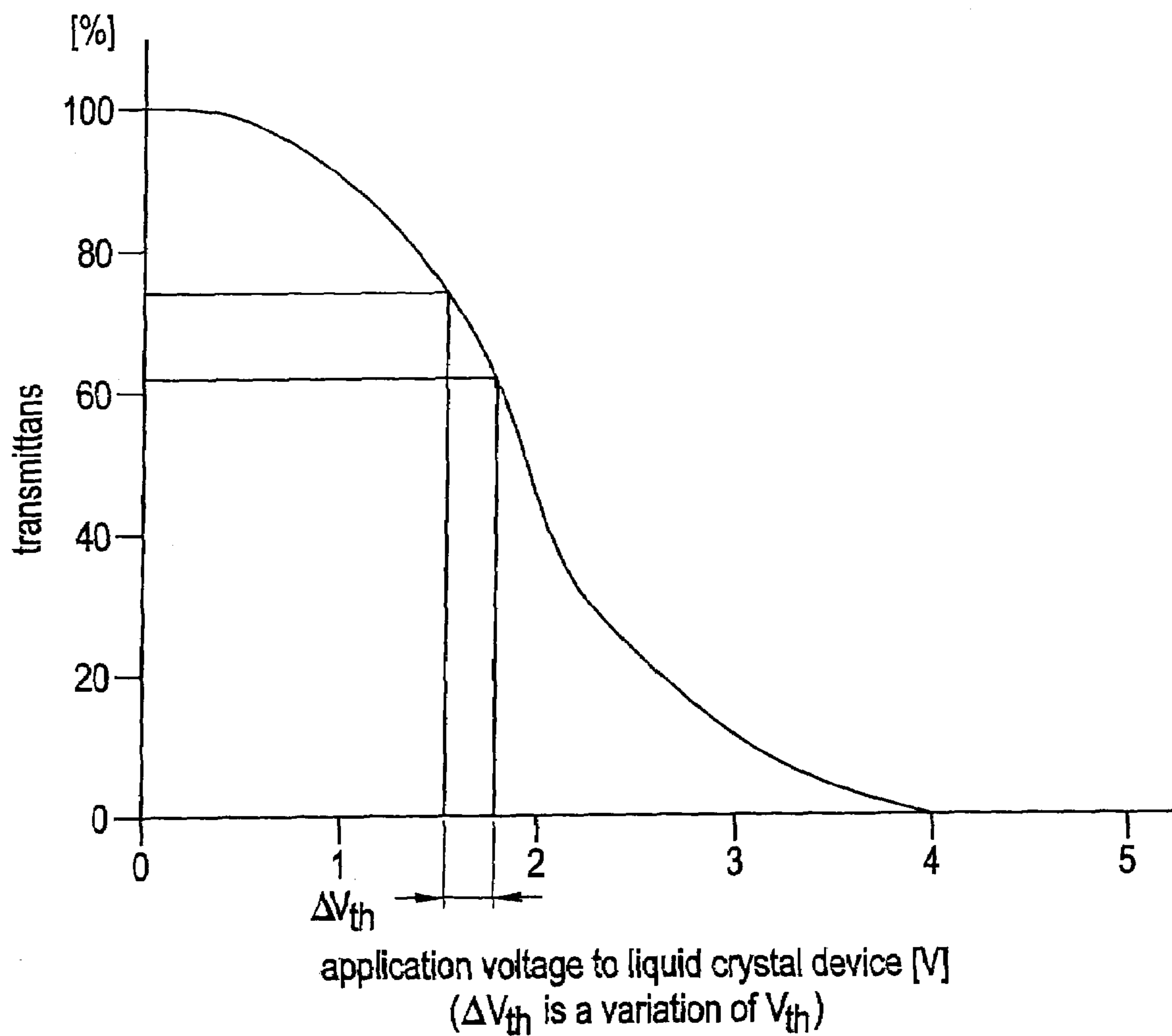
FIG. 11 PRIOR ART
