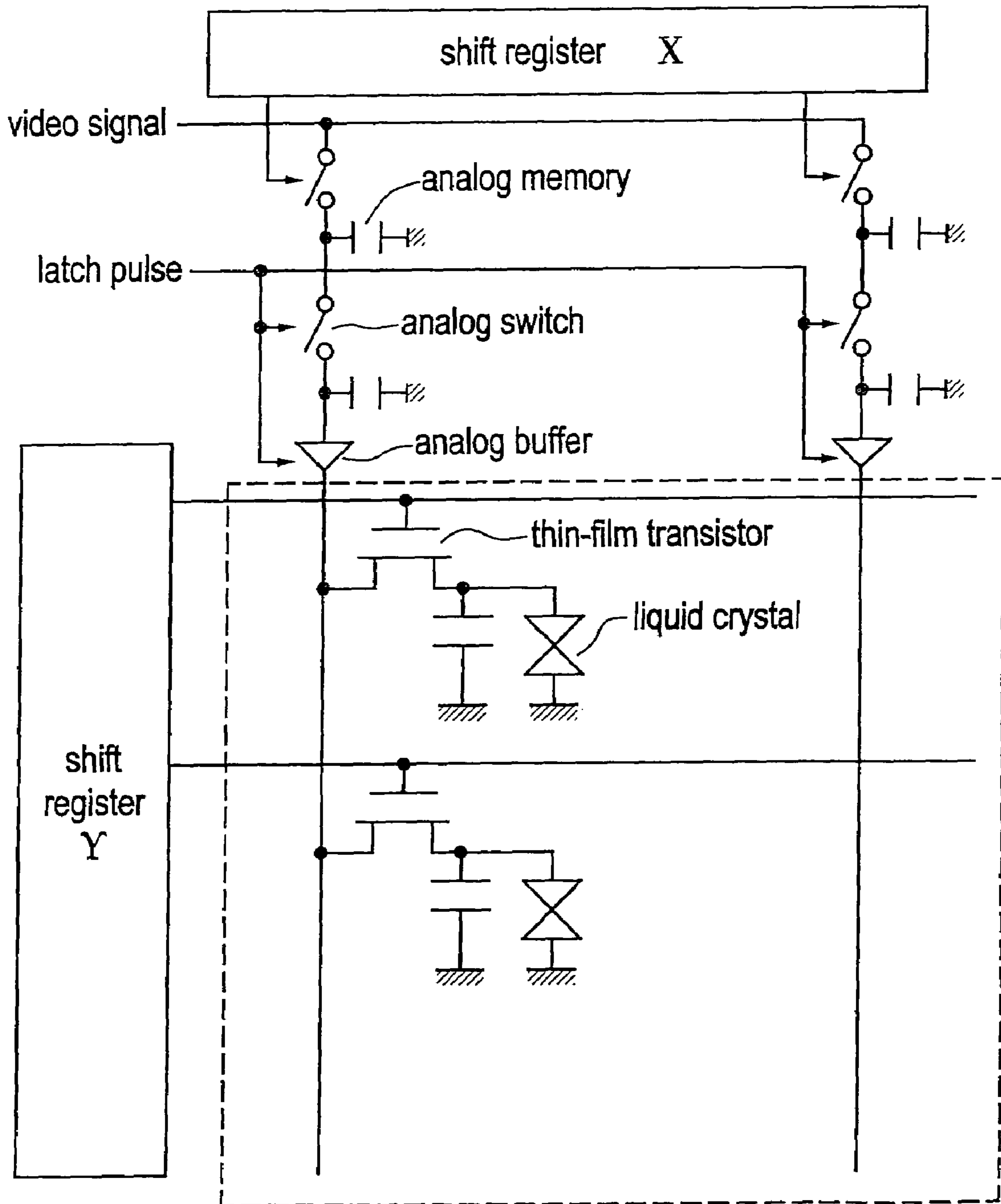
FIG. 9 PRIOR ART
