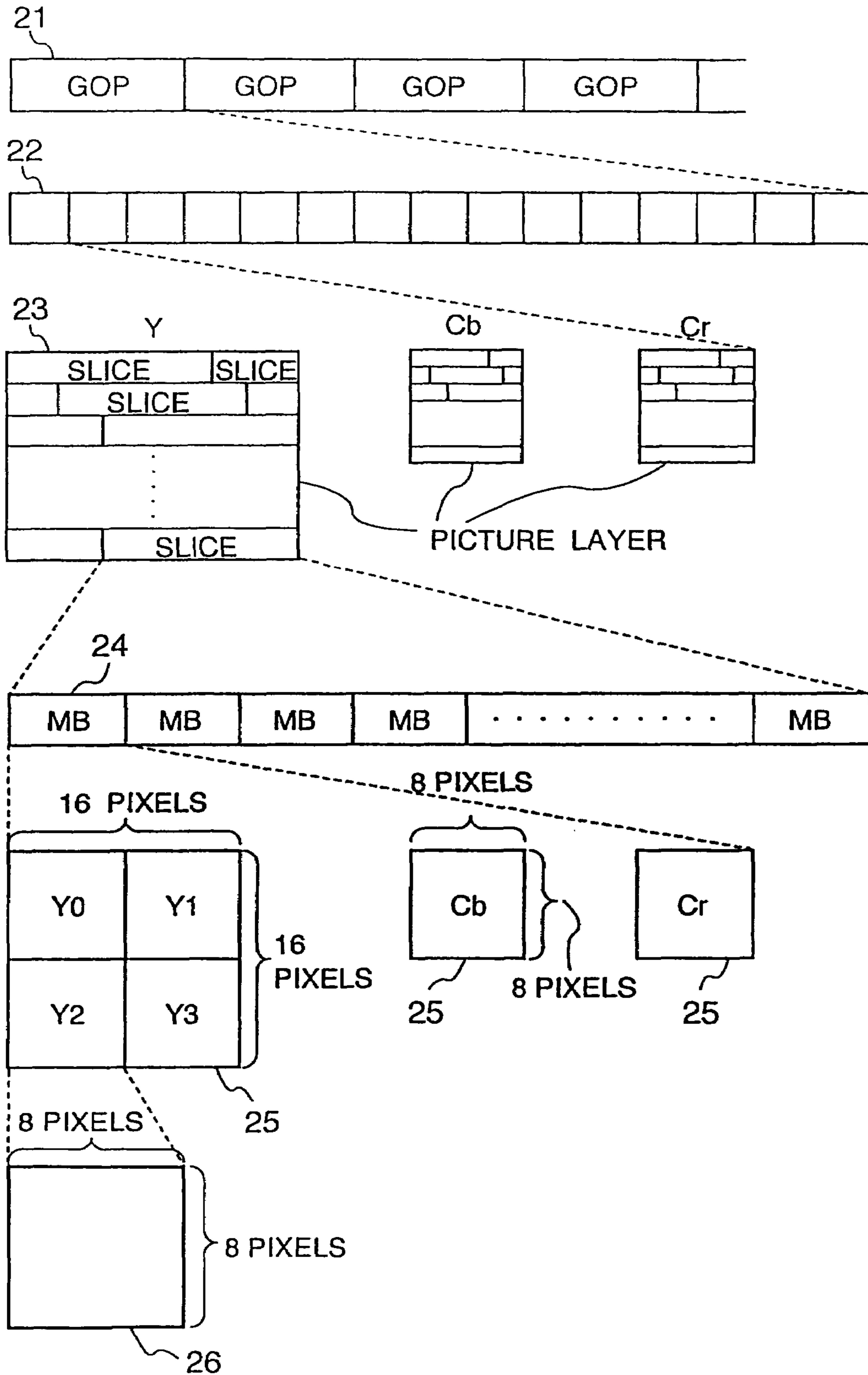
FIG. 30 PRIOR ART
