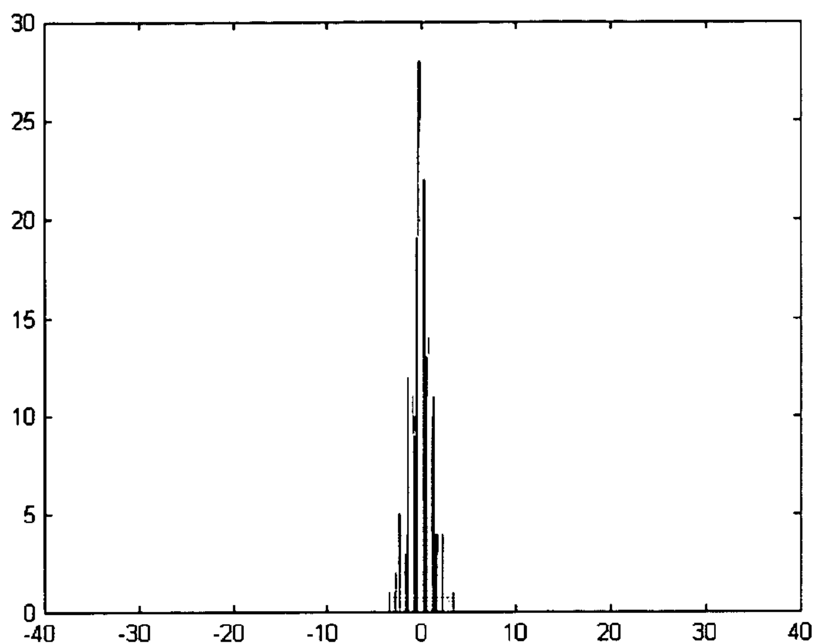
Figure 3: the distribution of the difference value \alpha .
