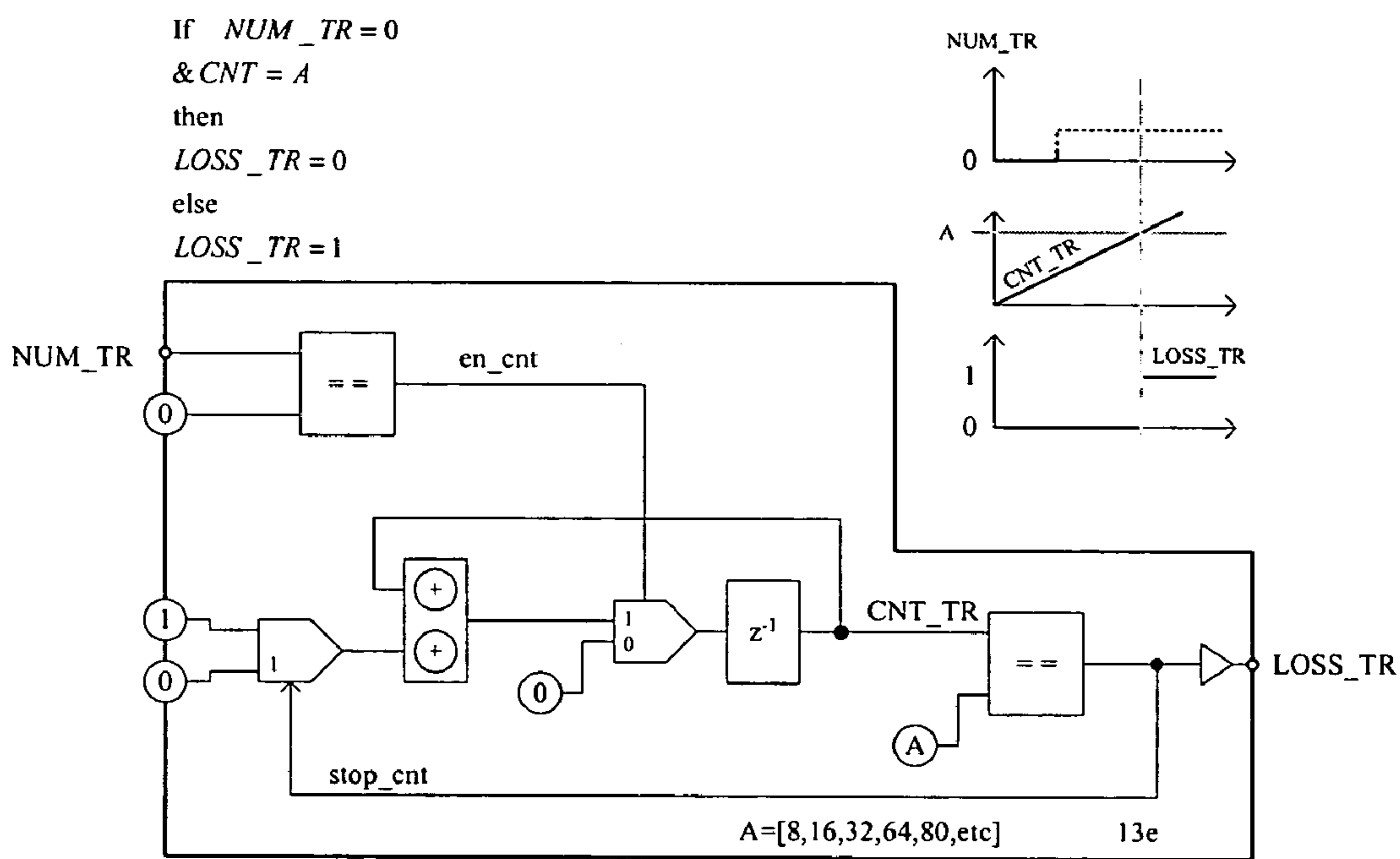
Transition Loss Detection Unit (TLDU)
