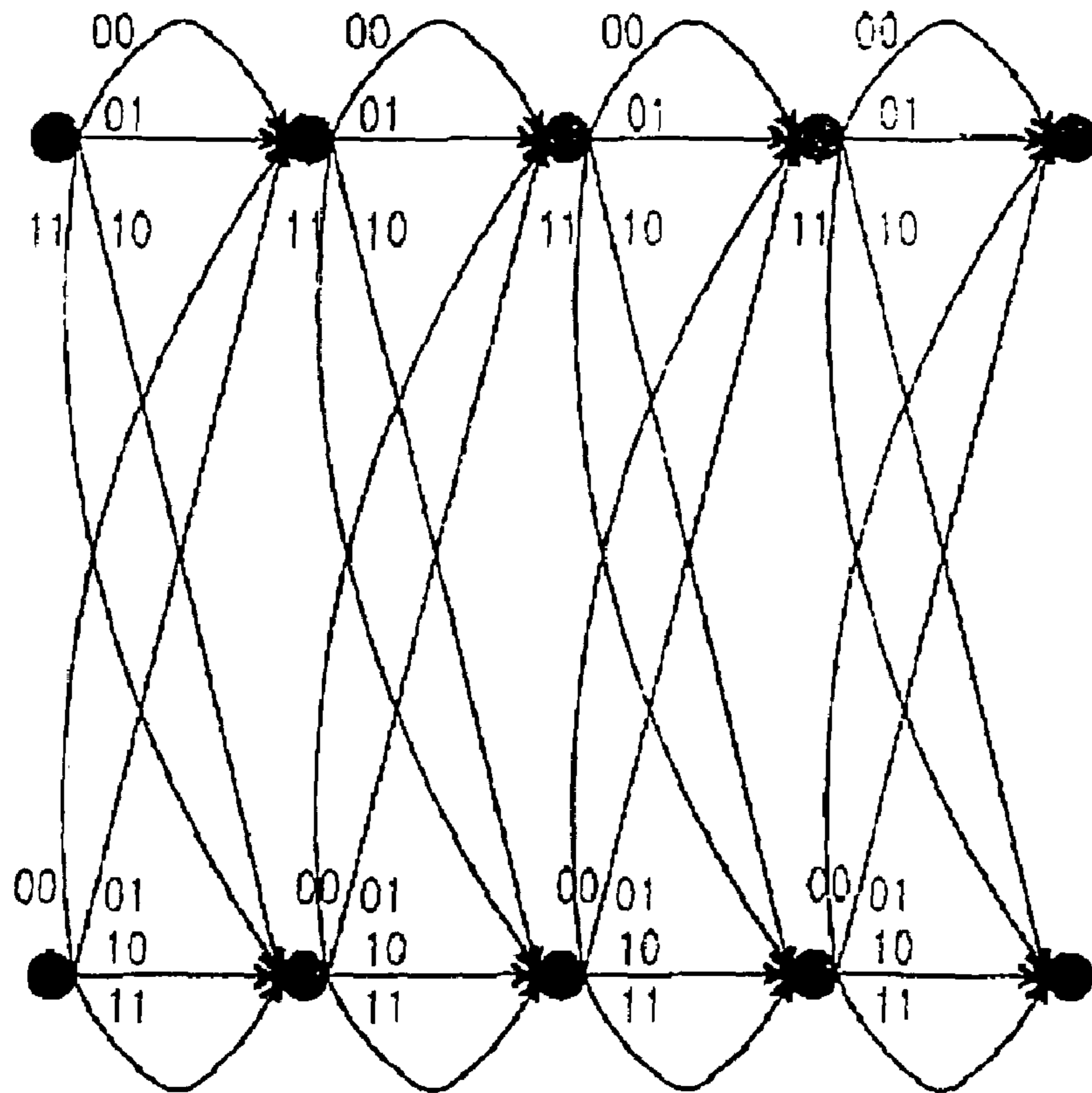
FIG.13 (PRIOR ART)
