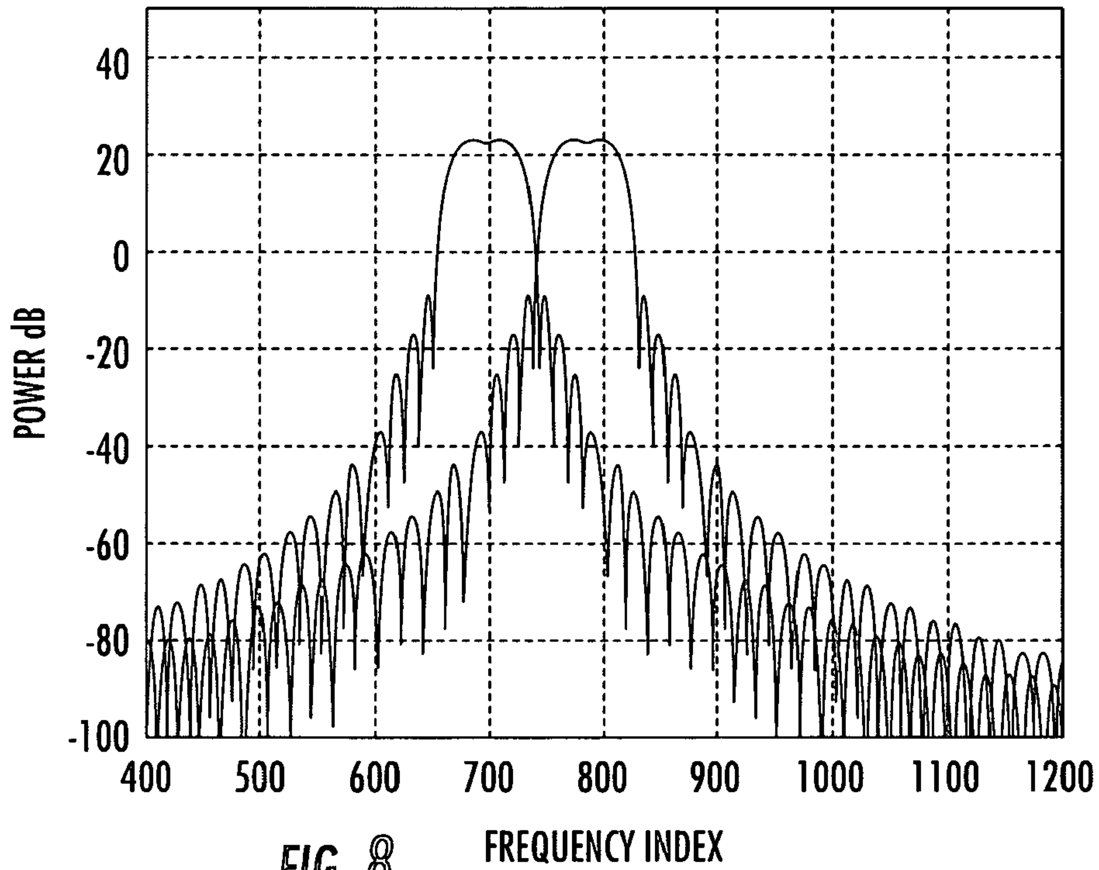
FREQUENCY SPECTRUM WITH POLYPHASE FILTERING
