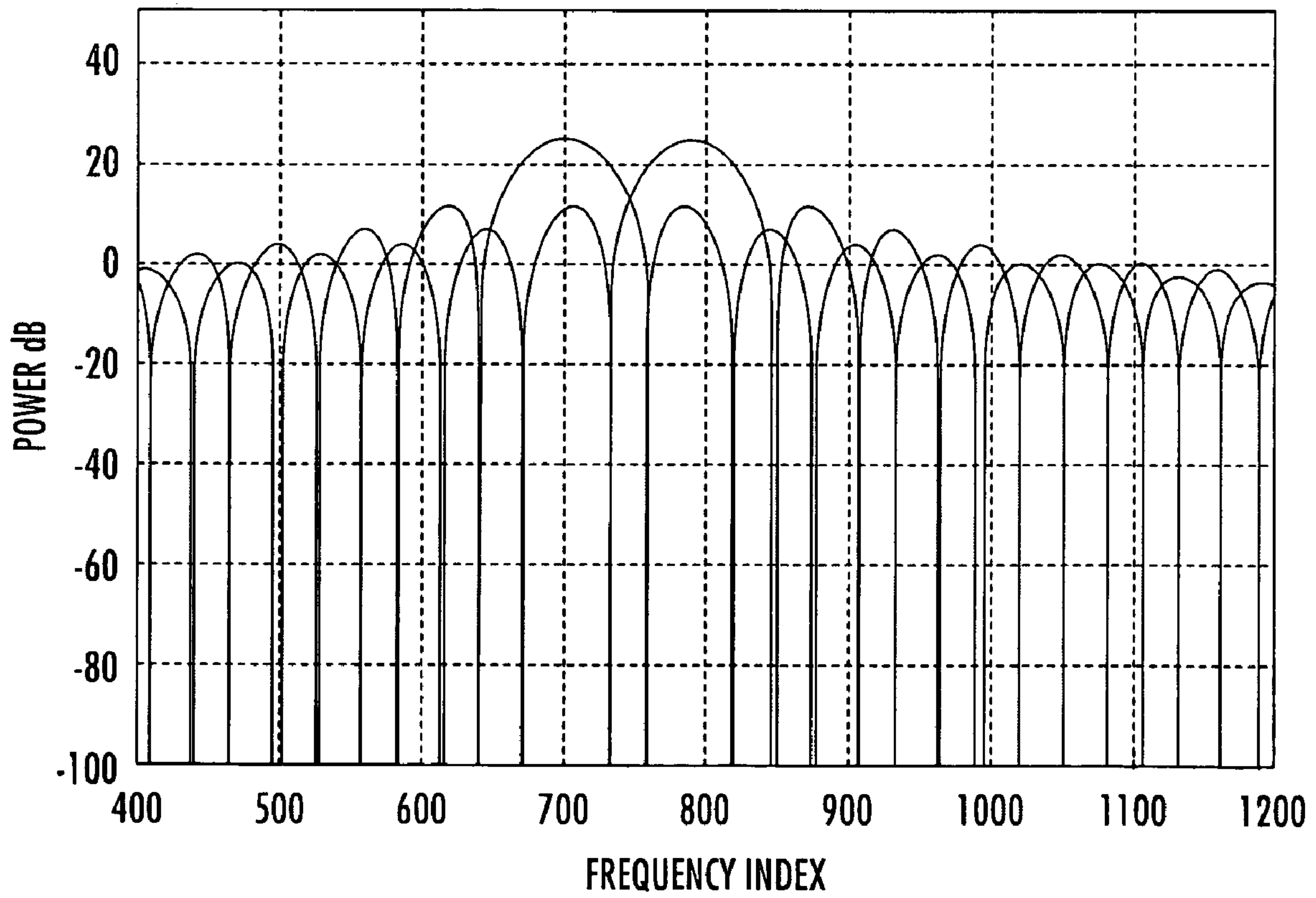
FREQ. SPECTRUM OFMD, 1/2 T s CYCLIC EXTENSION
