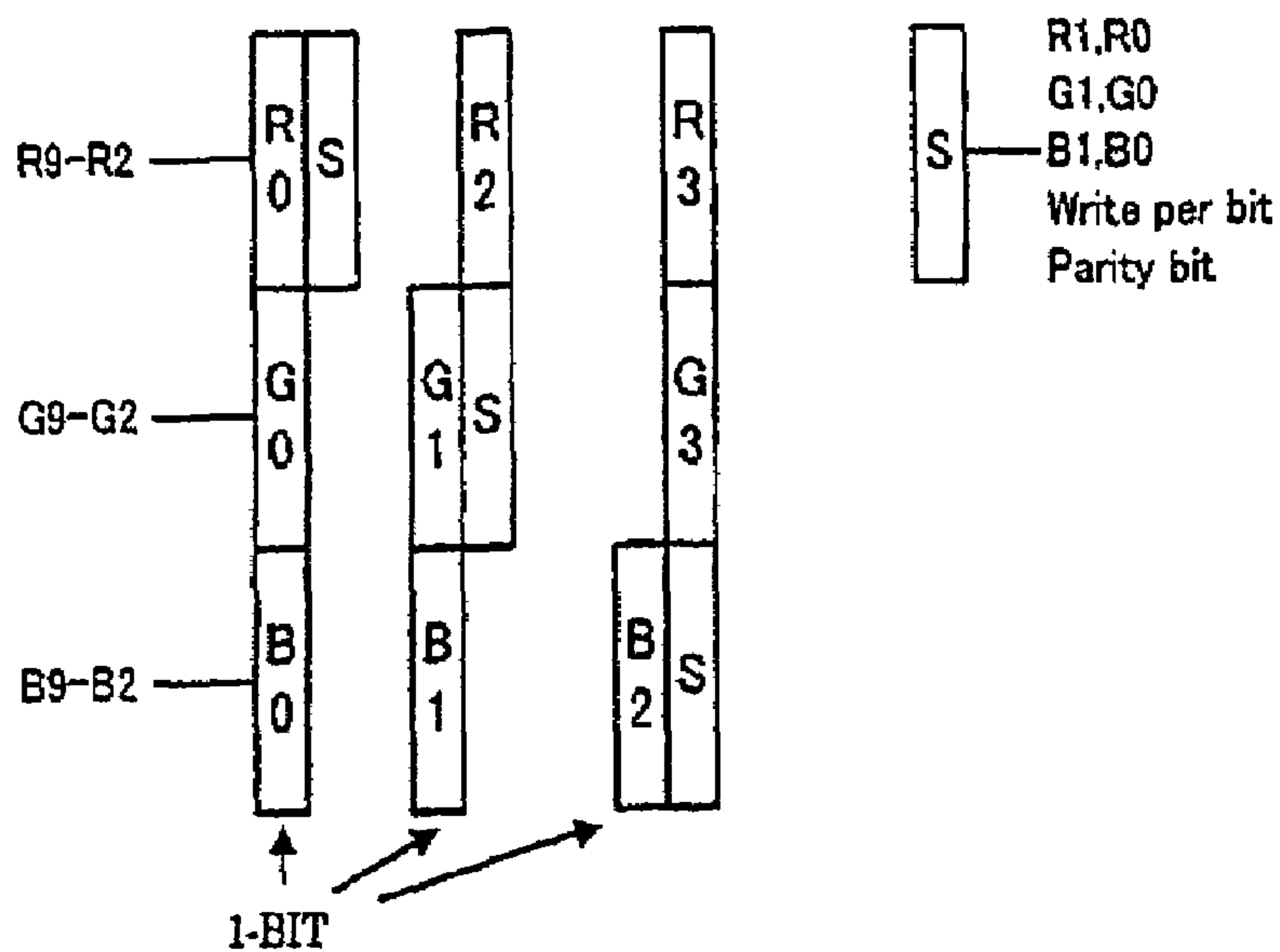
(b) BIT ASSIGN OF 30-BIT COLOR
