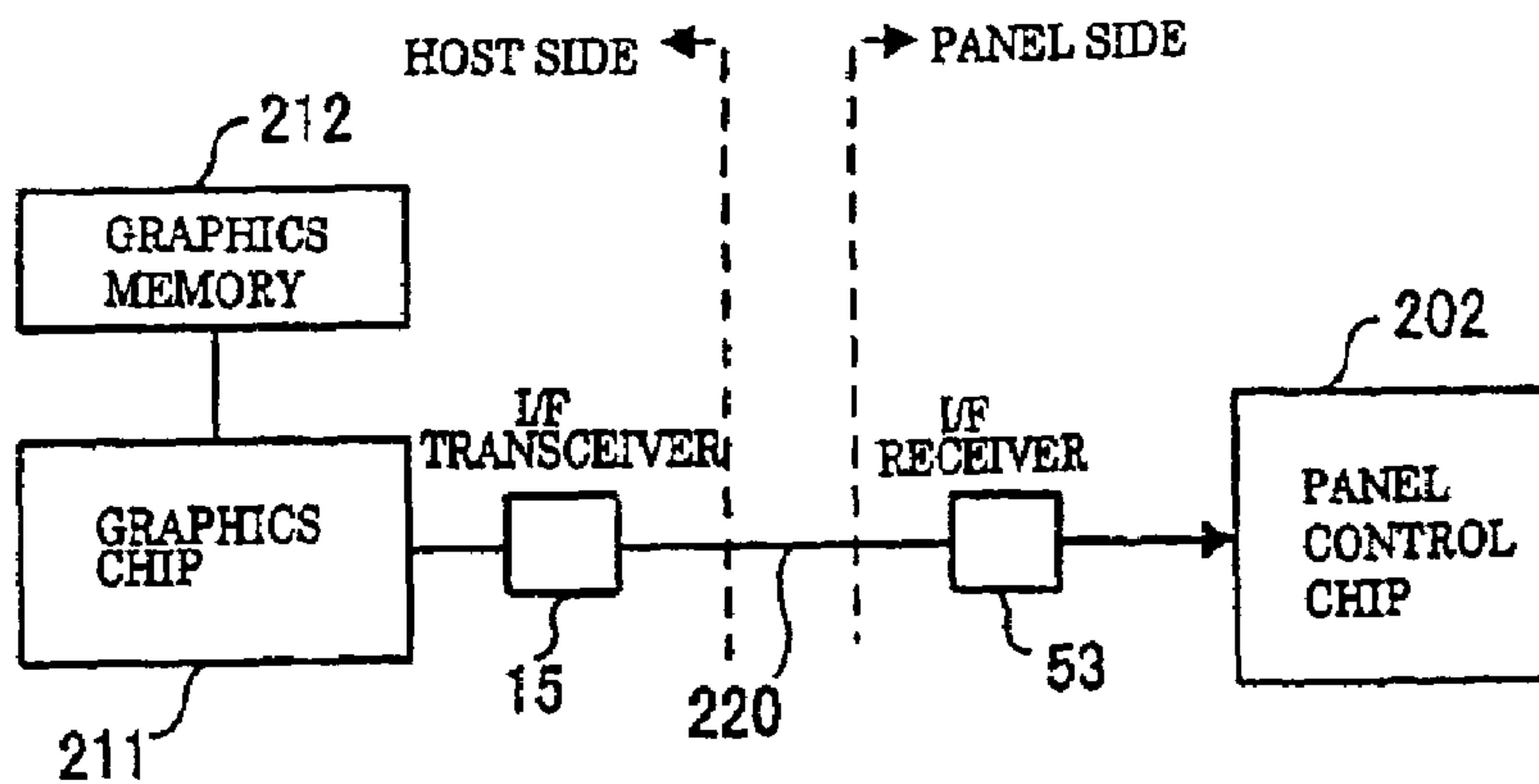
(b) LIMITATION OF DATA BAND WIDTH
