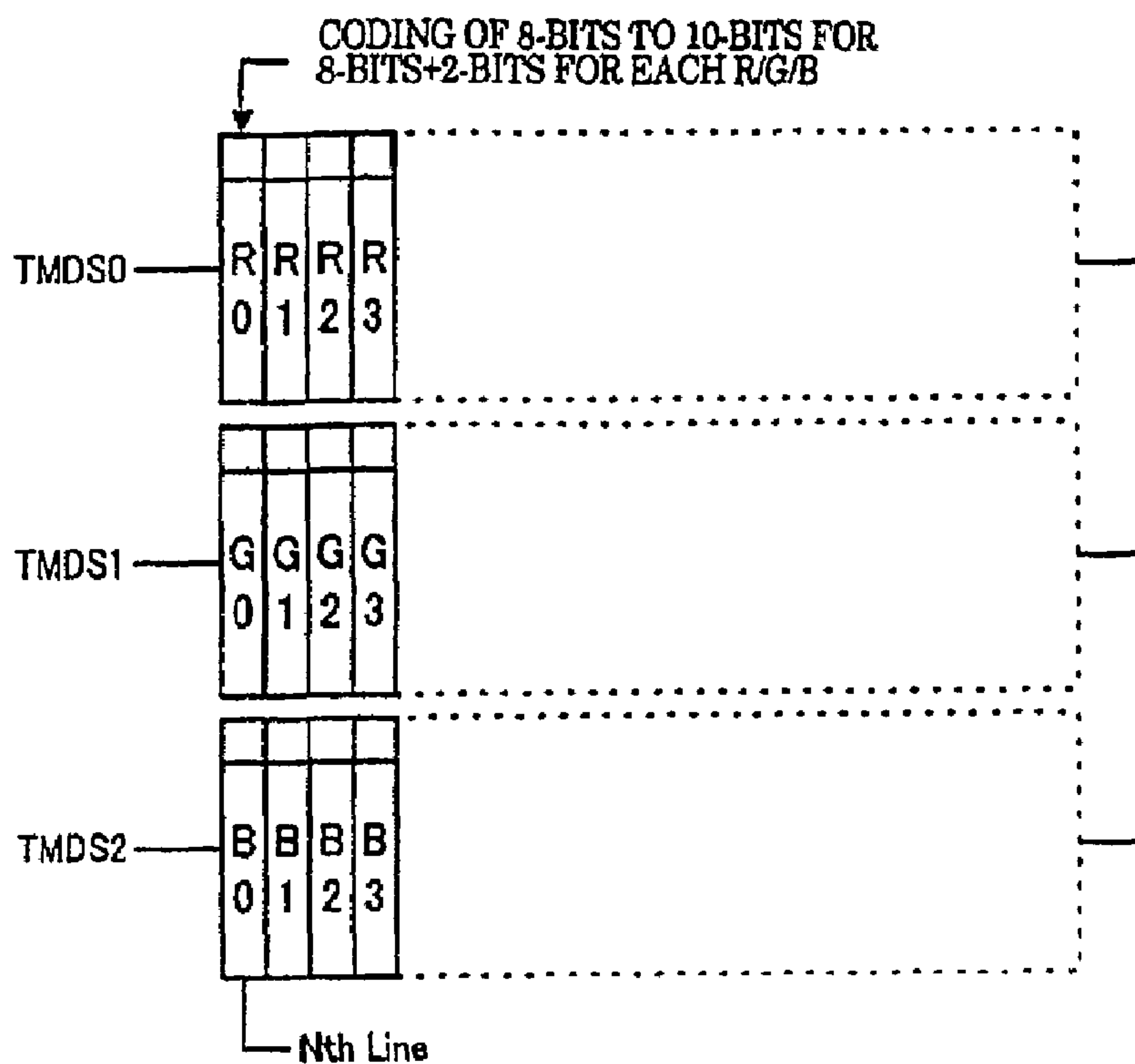
(a) TMDS DATA TRANSFER
