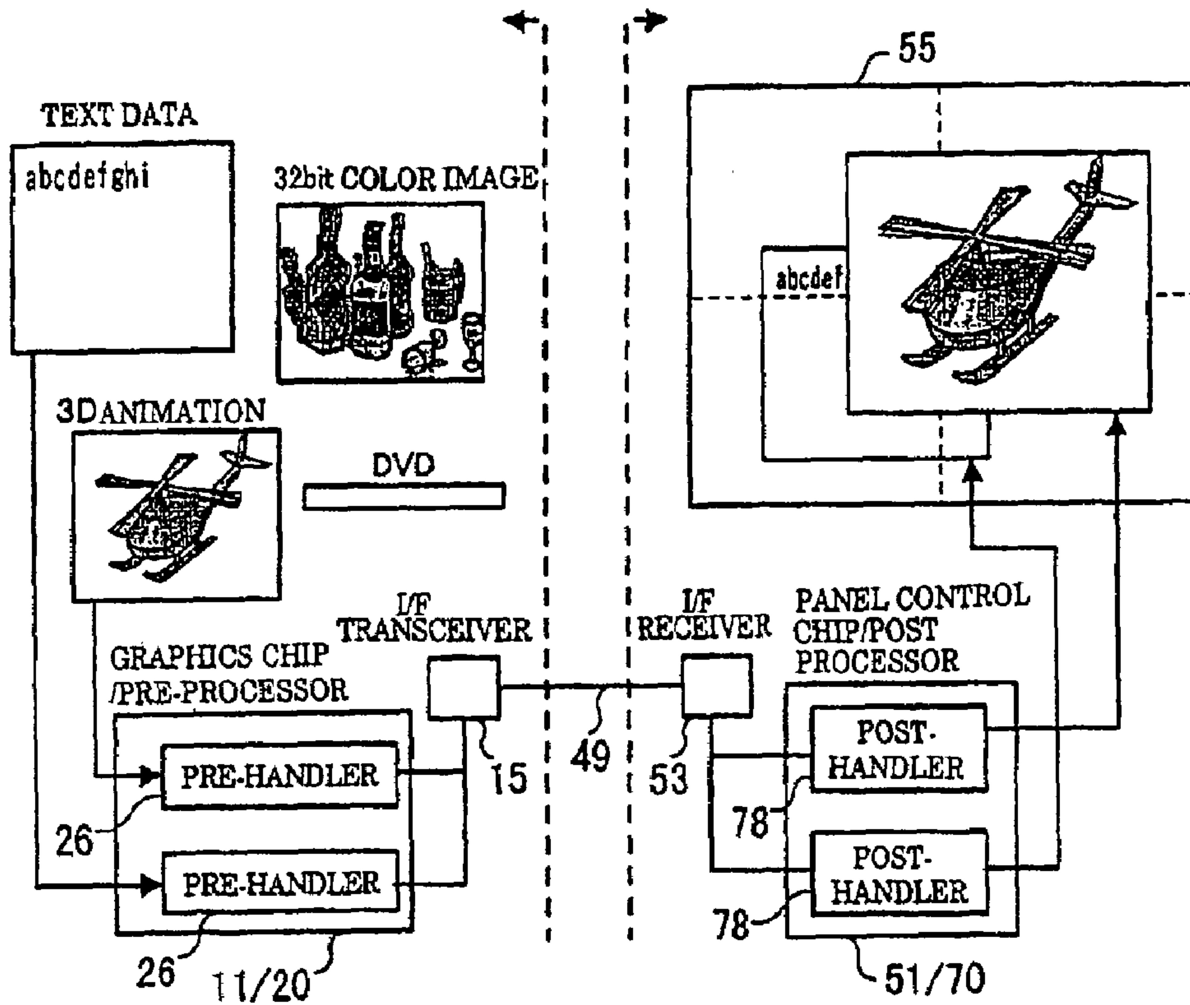
(a) DATA SOURCE AND PROCESSING SYSTEM
