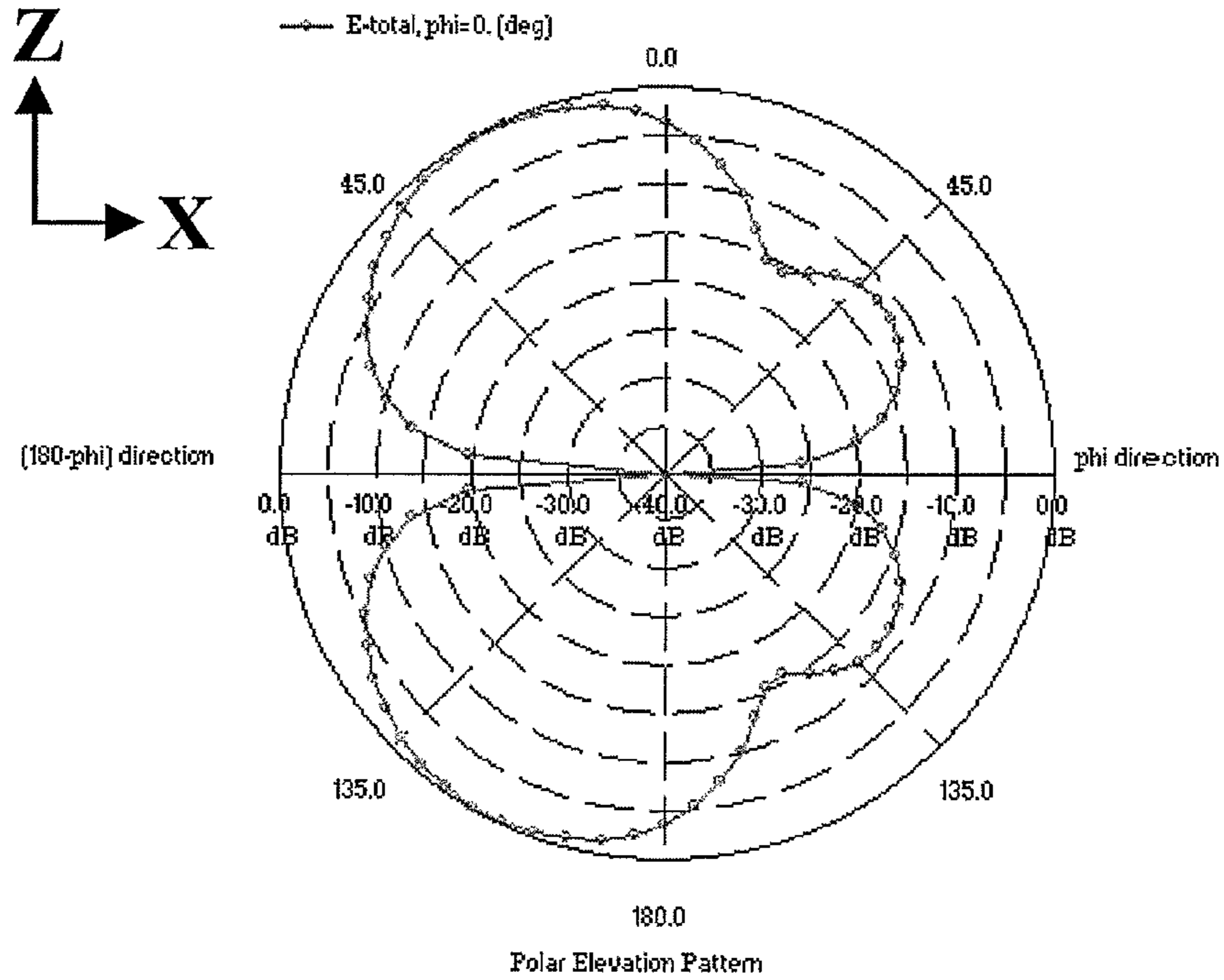
FIG. 2 (PRIOR-ART)
