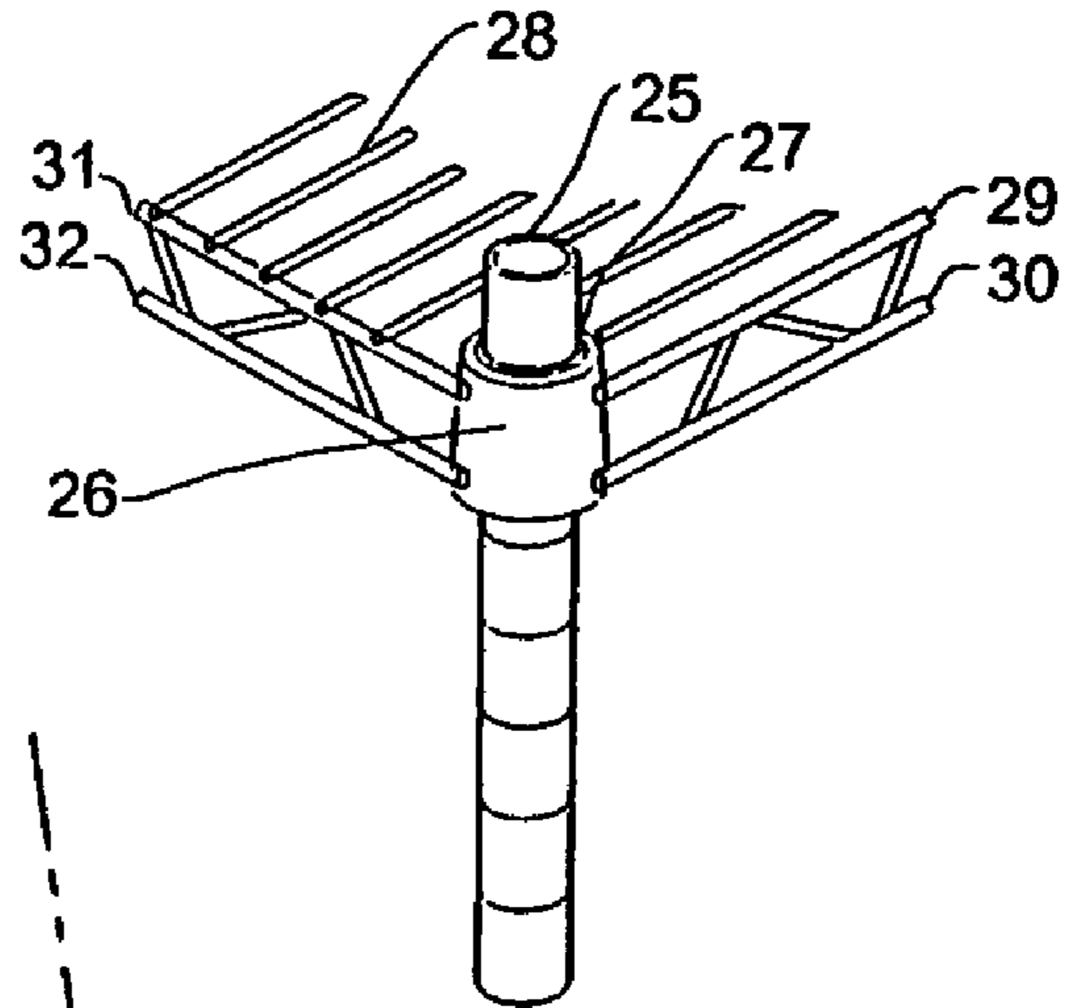
Fig. 2 (Prior Art)
