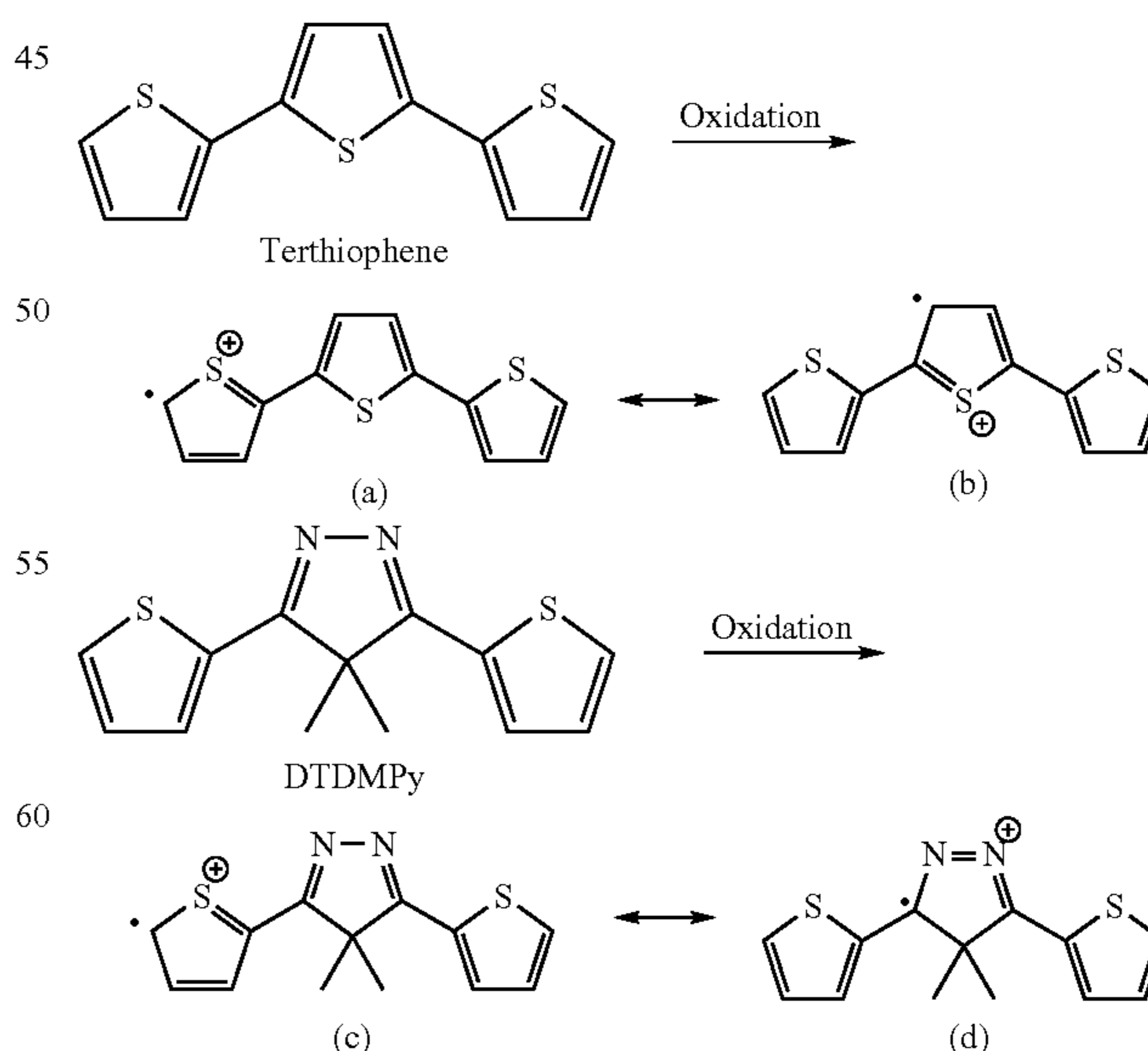
Oxidation of terthiophene showing structures giving rise to (a) desirable 2,5-linkages and (b) often-undesirable 3,5-linkages; oxidation of DTDMPy showing structures leading to (c) polymer and (d) monomer re-neutralization.
