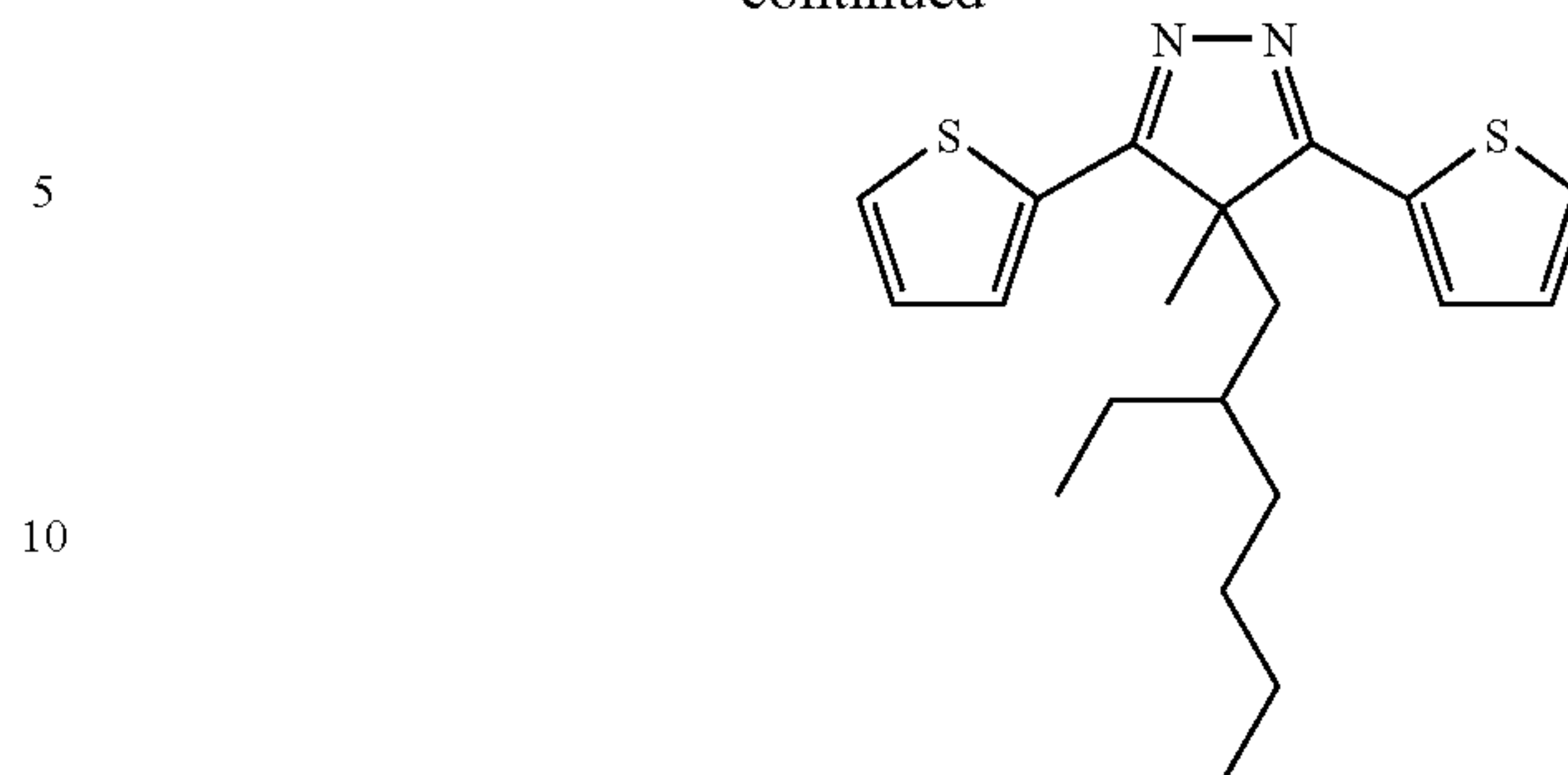
Diagram 3. Synthesis of 3,5-dithien-2-yl-4-methyl-4-oligoether-pyrazole.
