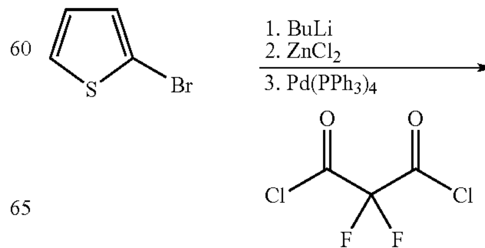
Diagram 4. Synthesis of 3,5-dithien-2-yl-4,4-difluoropyrazole.
