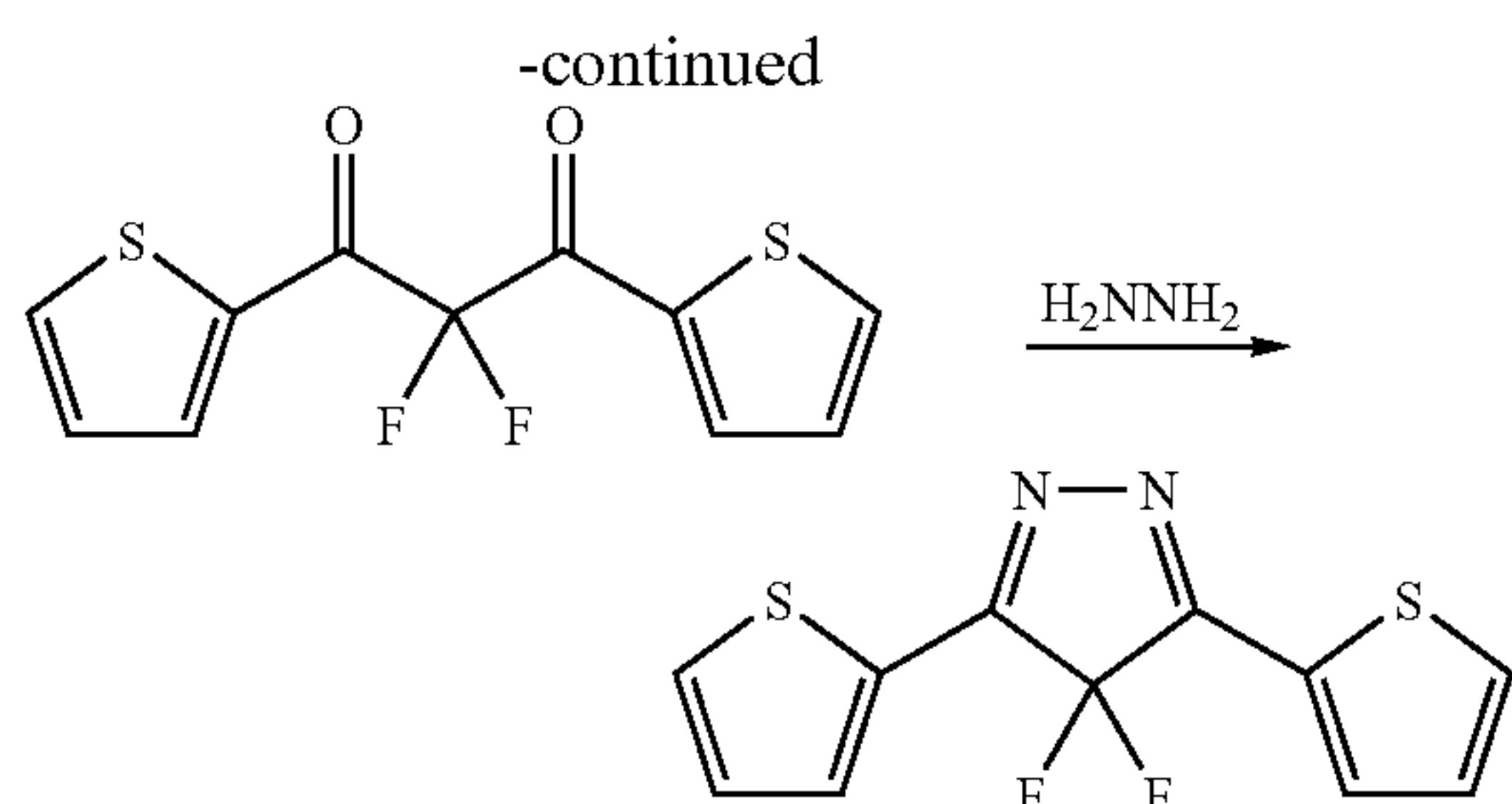
Diagram 5. Synthesis of 3,5-dithien-3'-organo-2-yl-4,4-dimethylpyrazole.
