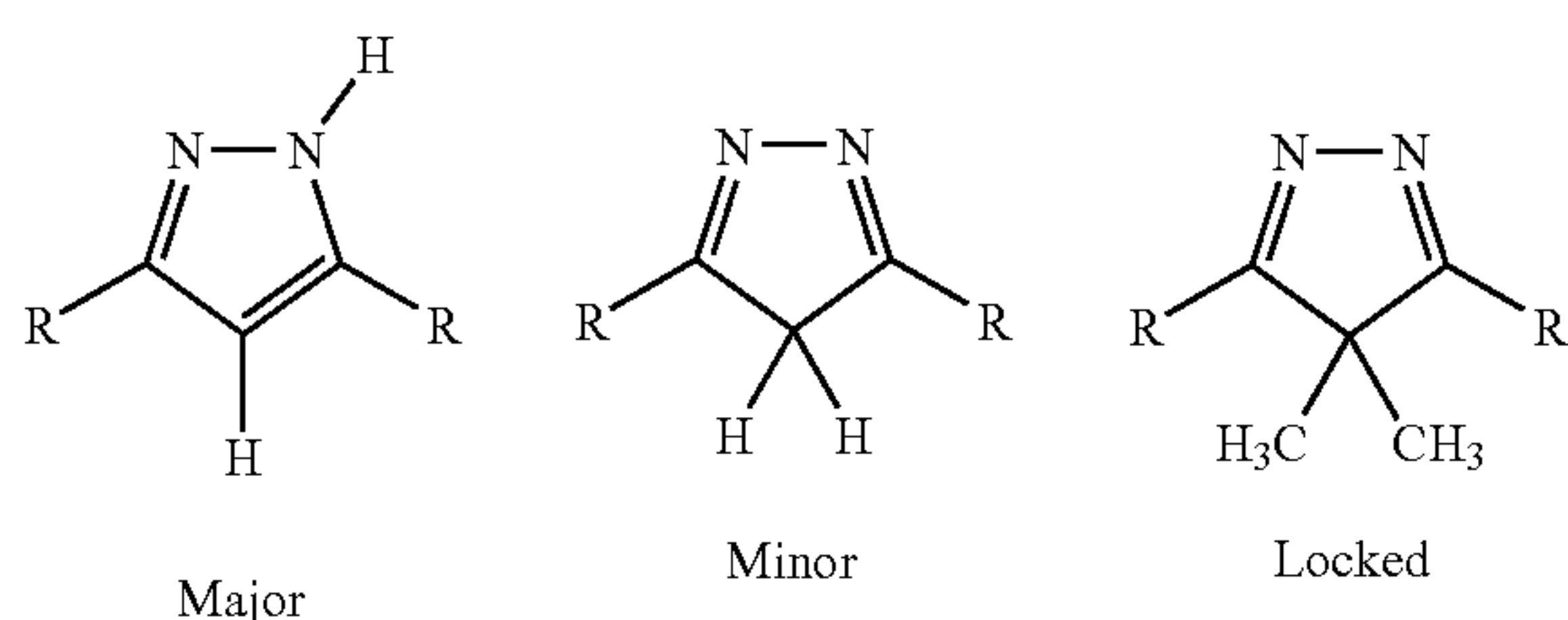
Diagram 6. Resonance structures of a 3,5-substituted pyrazole showing a conjugation-breaking major resonance struc-
