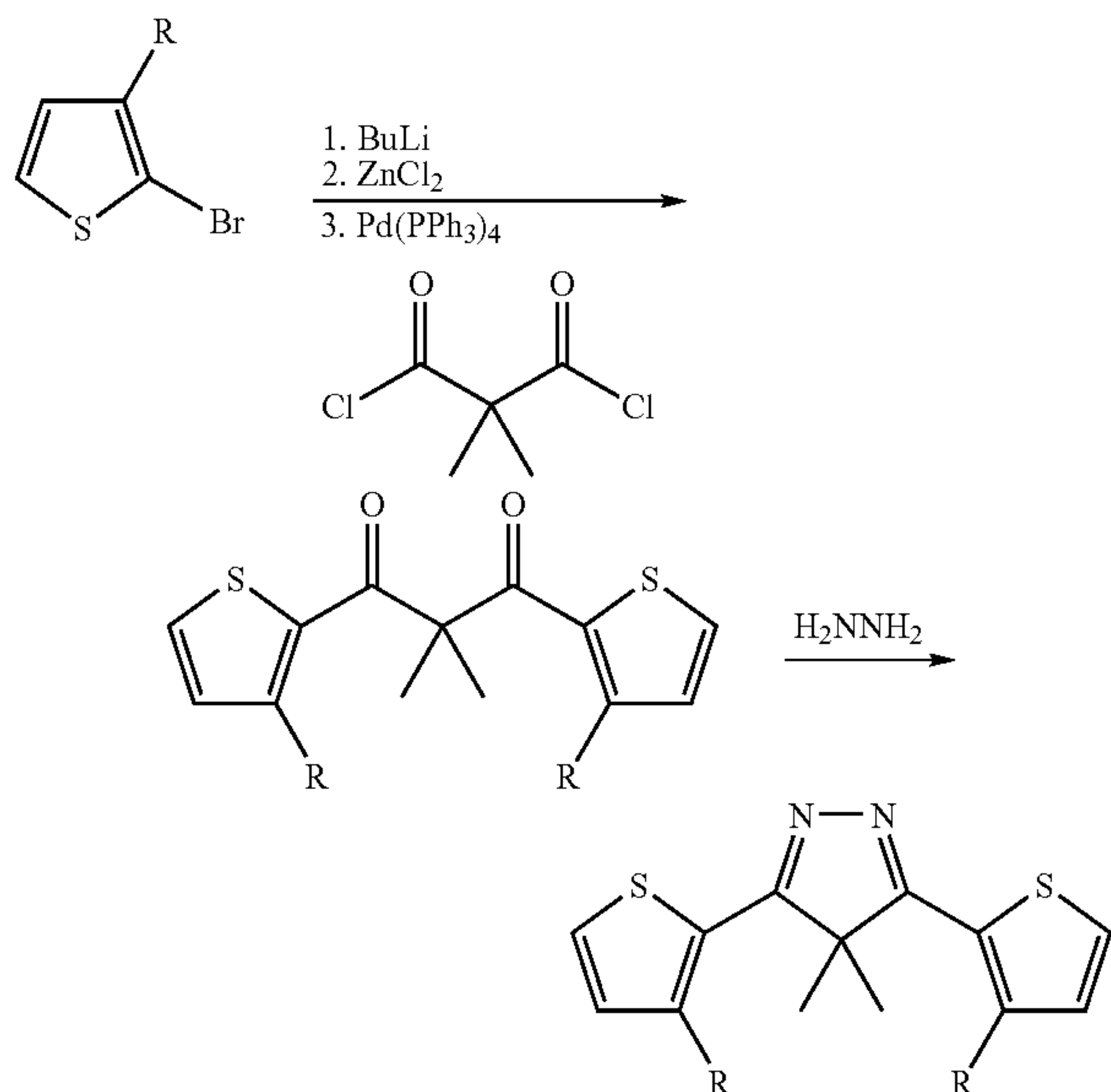
Diagram 5. Synthesis of 3,5-dithien-3'-organo-2-yl-4,4-dimethylpyrazole.
