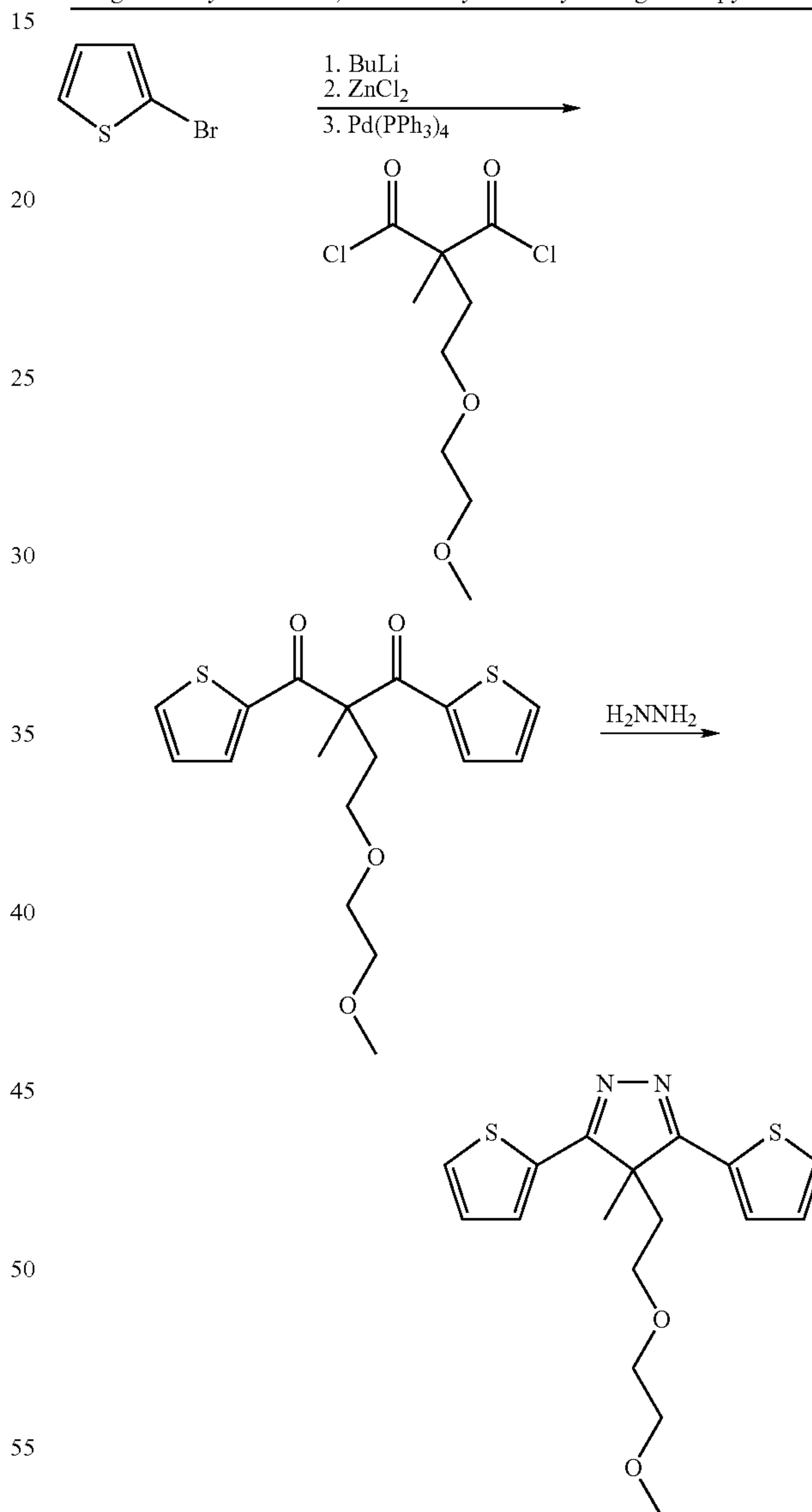
Diagram 4. Synthesis of 3,5-dithien-2-yl-4,4-difluoropyrazole.
