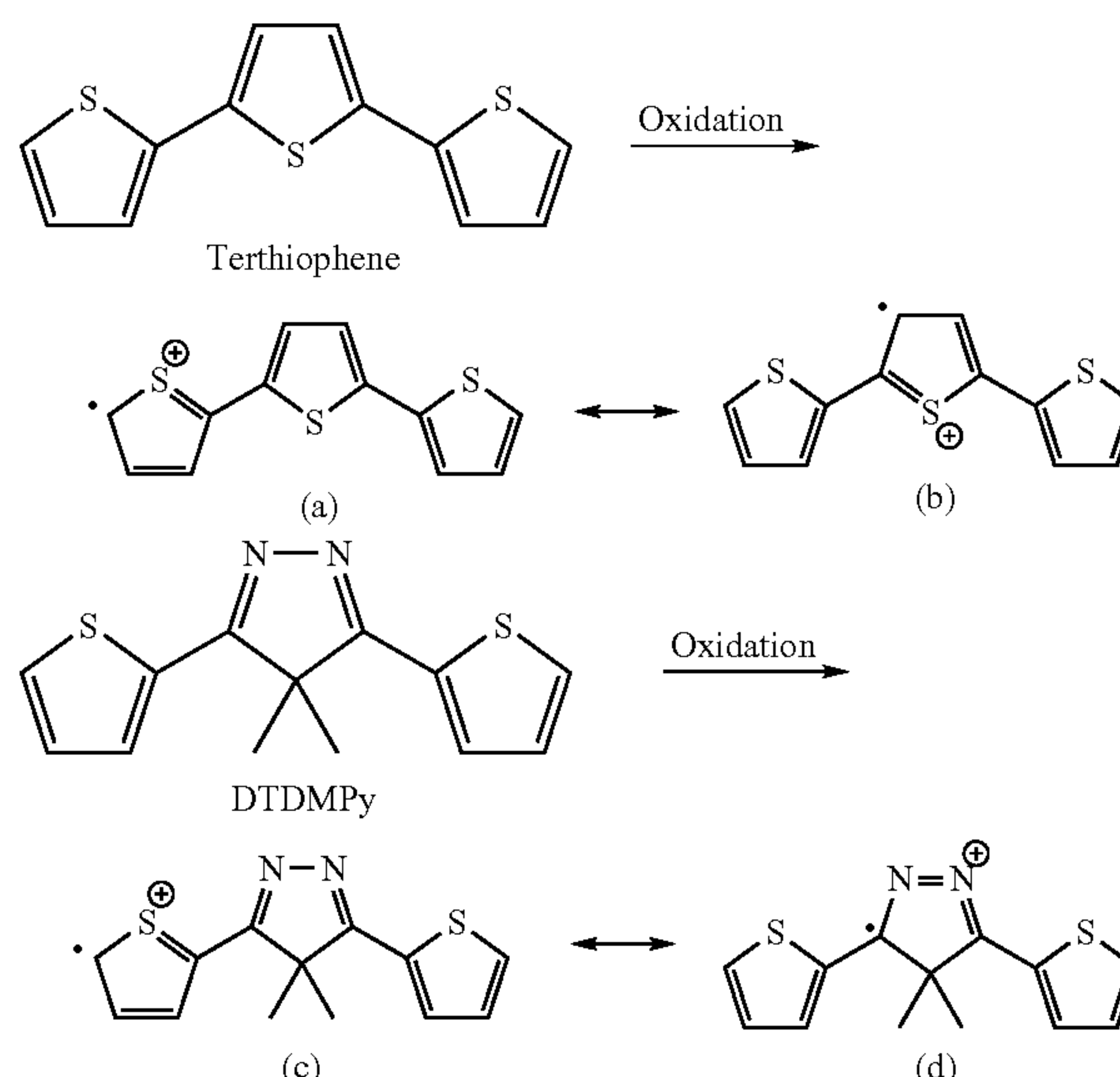
Oxidation of terthiophene showing structures giving rise to (a) desirable 2,5-linkages and (b) often-undesirable 3,5-linkages; oxidation of DTDMPy showing structures leading to (c) polymer and (d) monomer re-neutralization.
