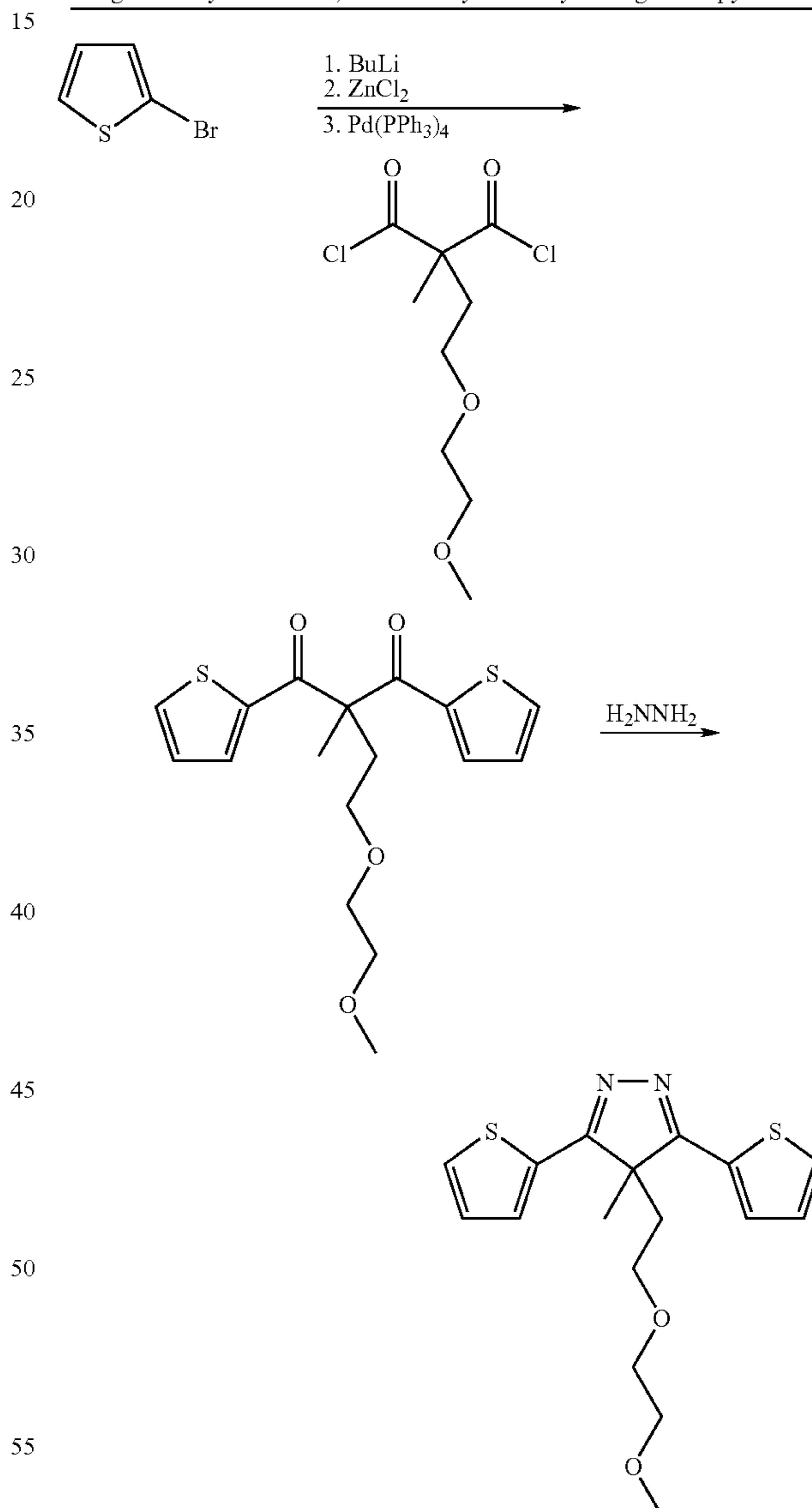
Diagram 4. Synthesis of 3,5-dithien-2-yl-4,4-difluoropyrazole.
