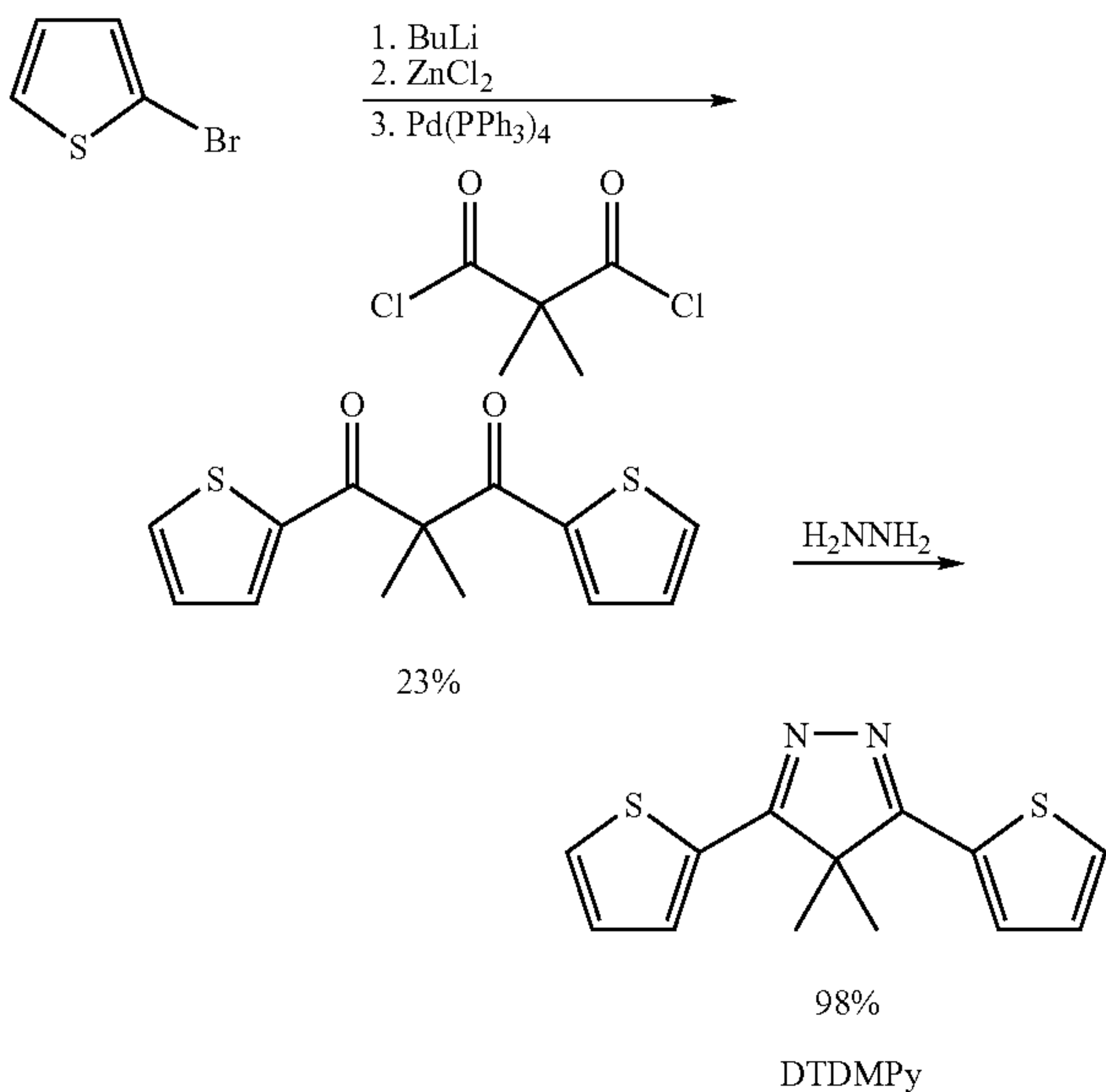
Diagram 1. Synthesis of 3,5-dithien-2-yl-4,4-dimethylpyrazole (DTDMPy).
