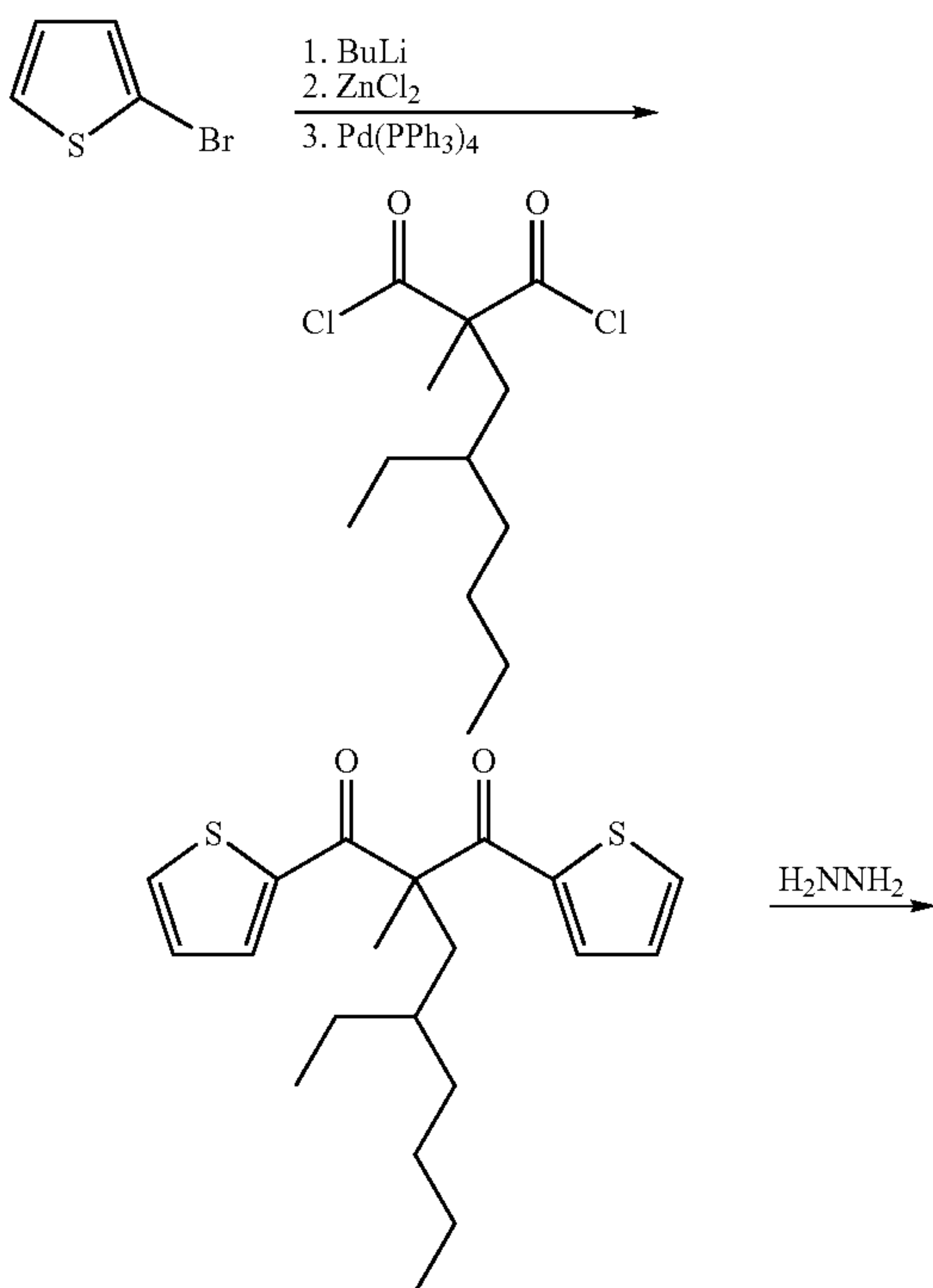
Diagram 2. Synthesis of 3,5-dithien-2-yl-4-methyl-4-alkyl-pyrazole.
