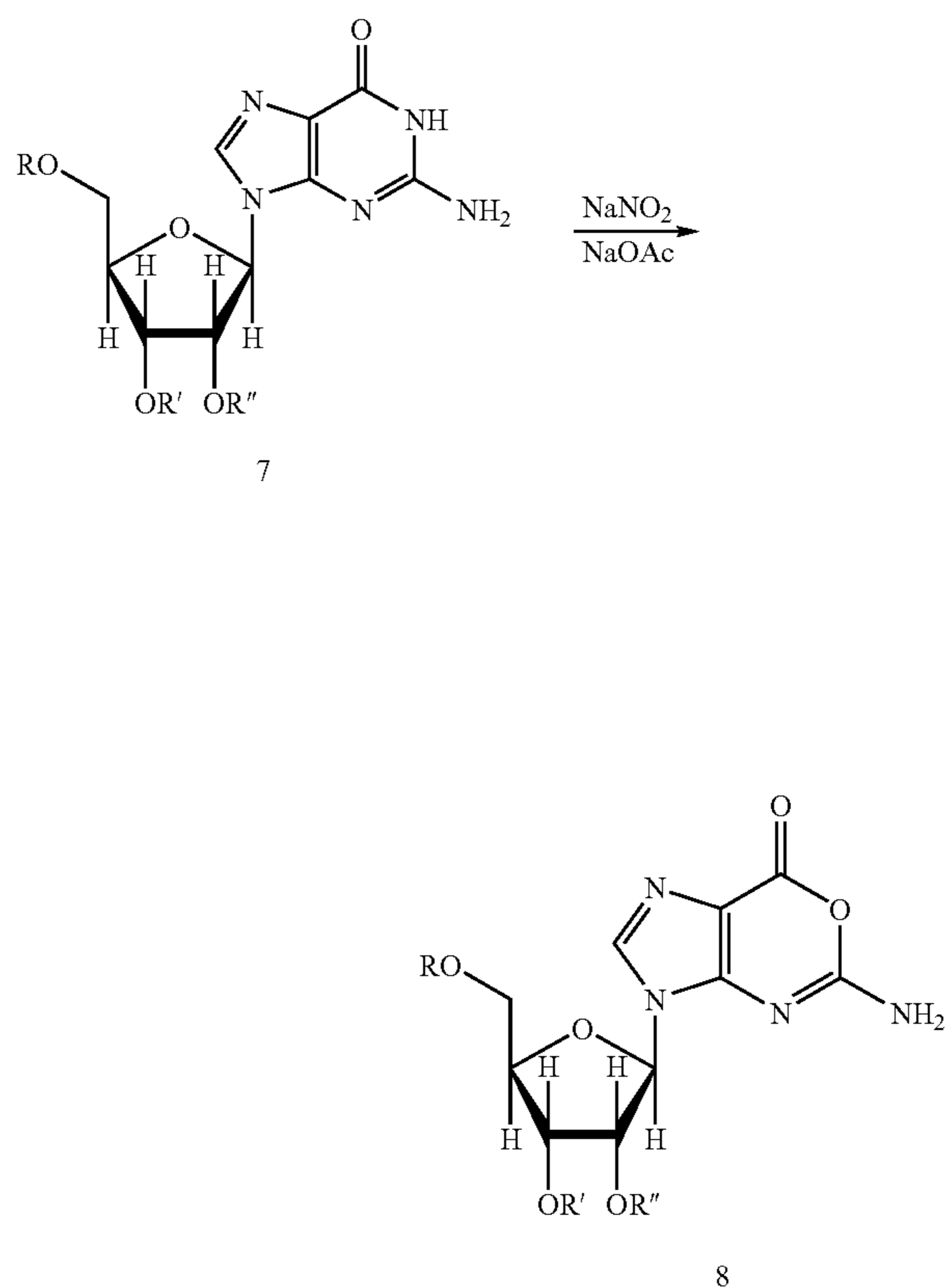
Scheme 4
