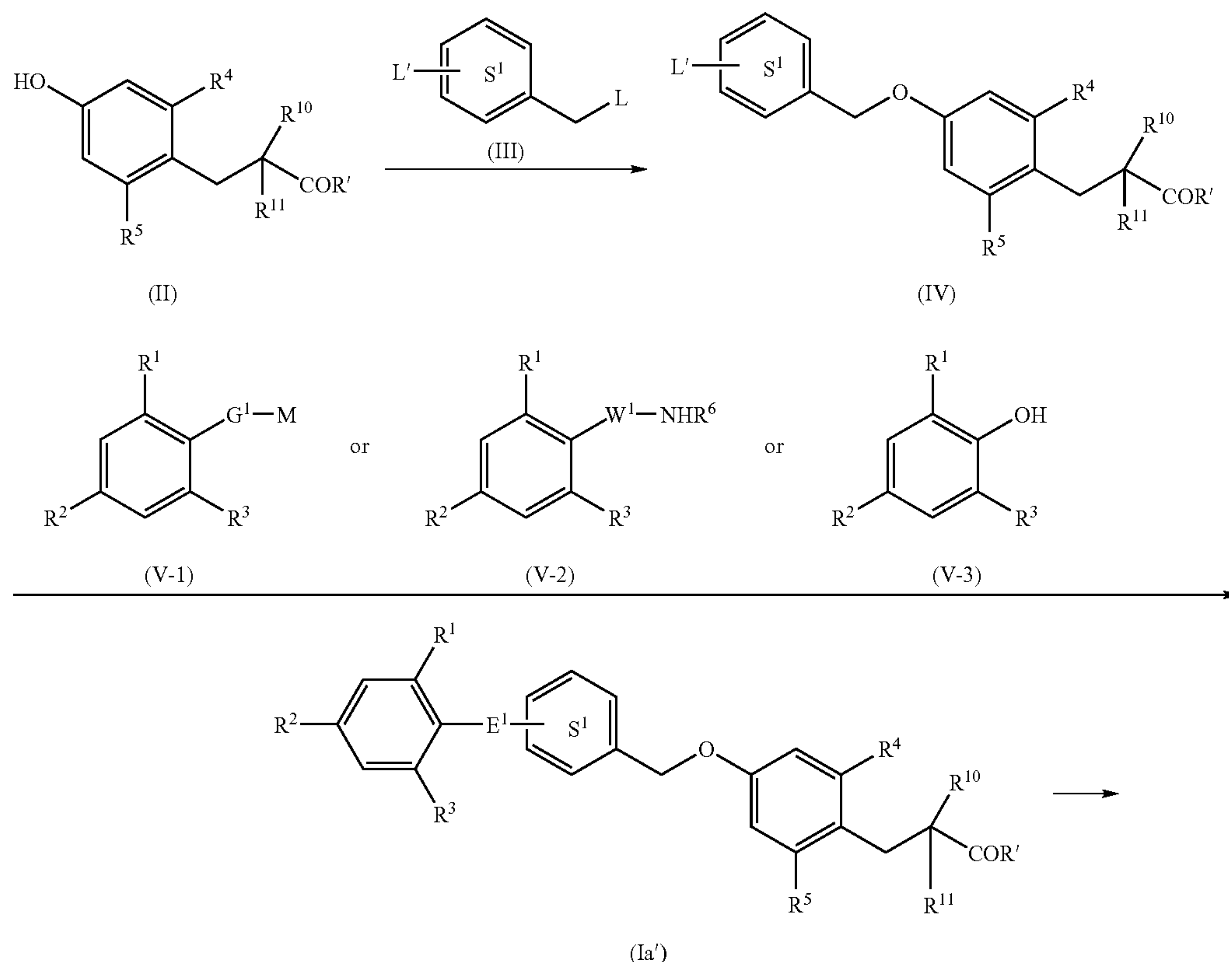
Reaction Scheme 1
