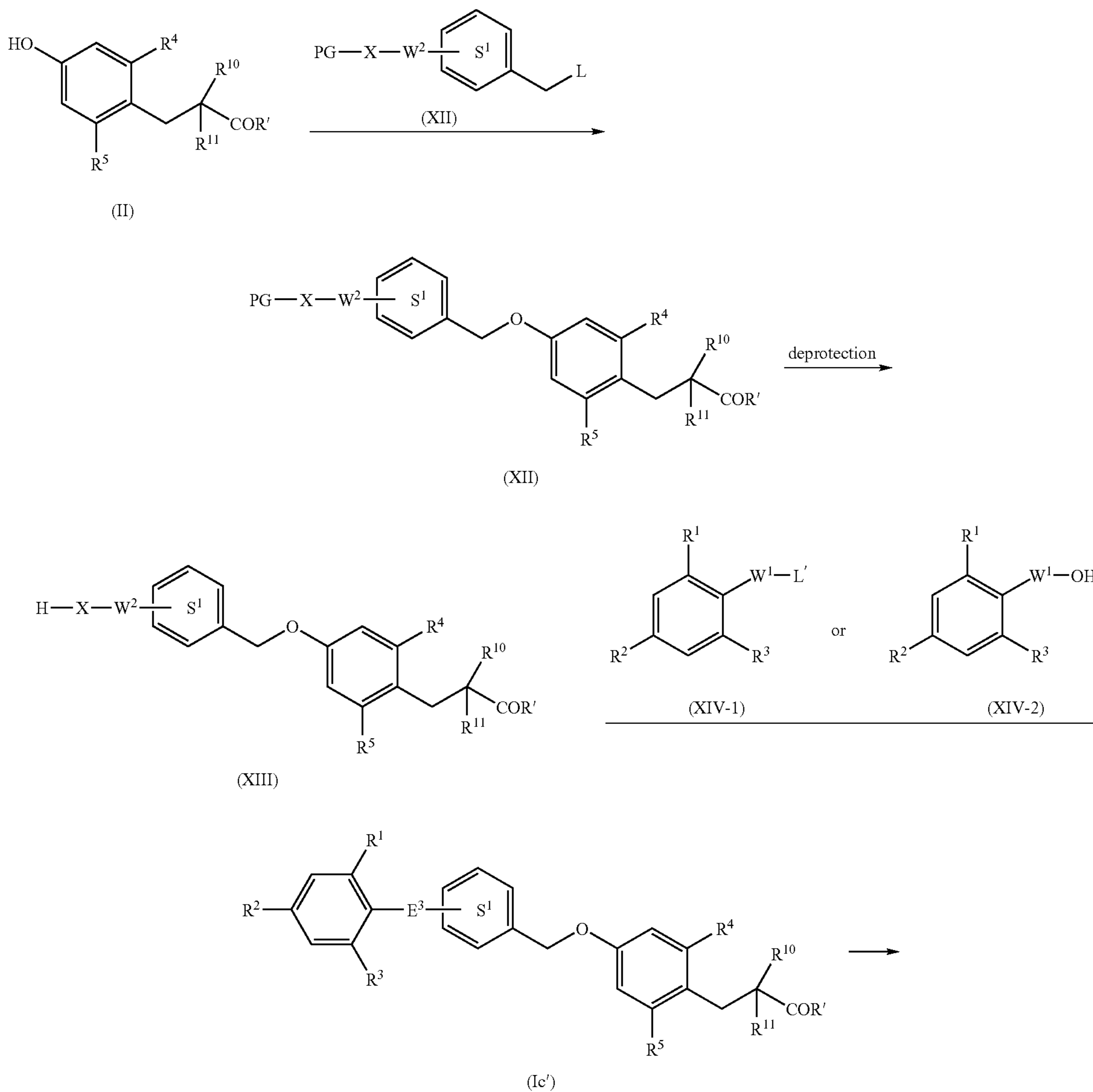
Reaction Scheme 3
