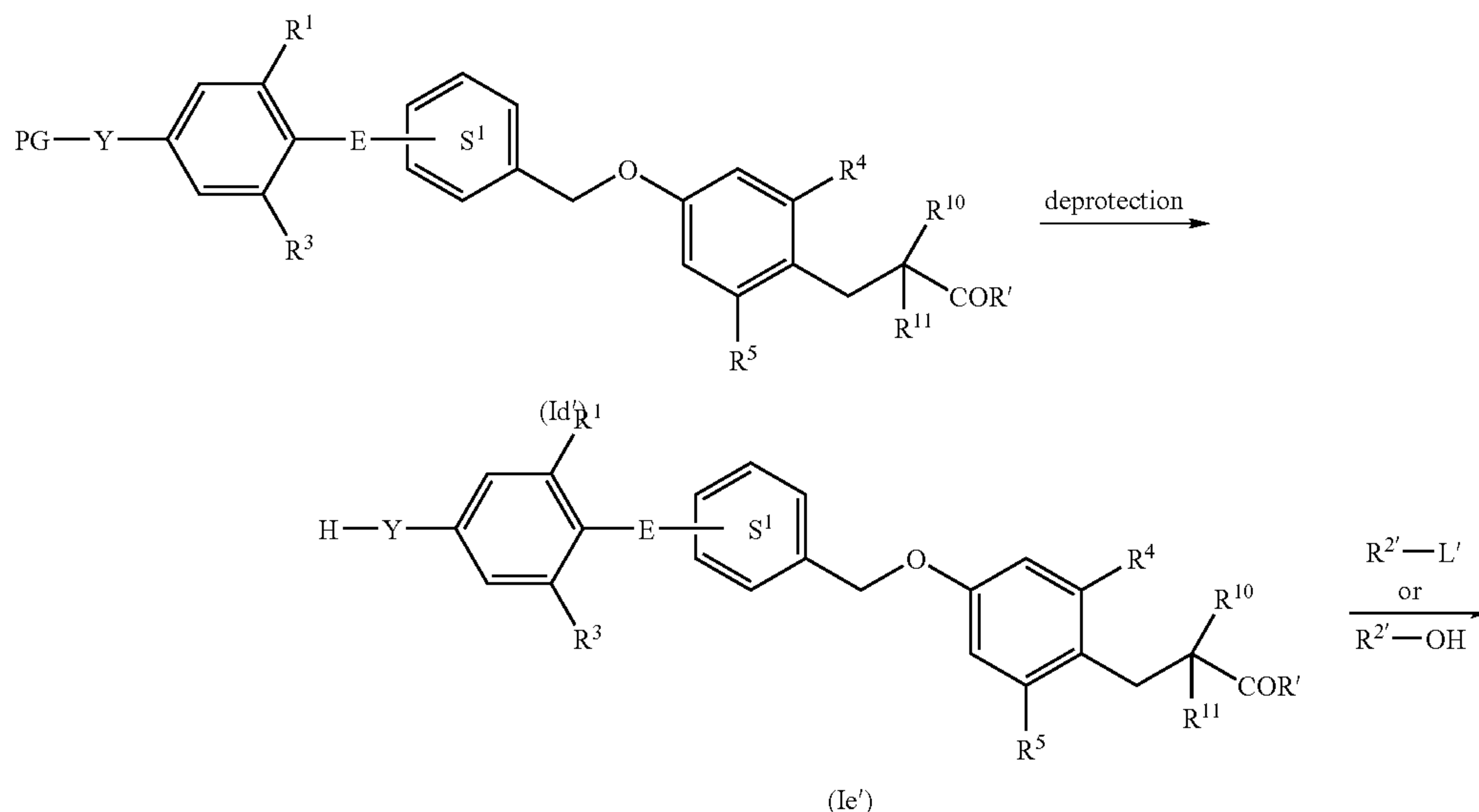
Reaction Scheme 4
