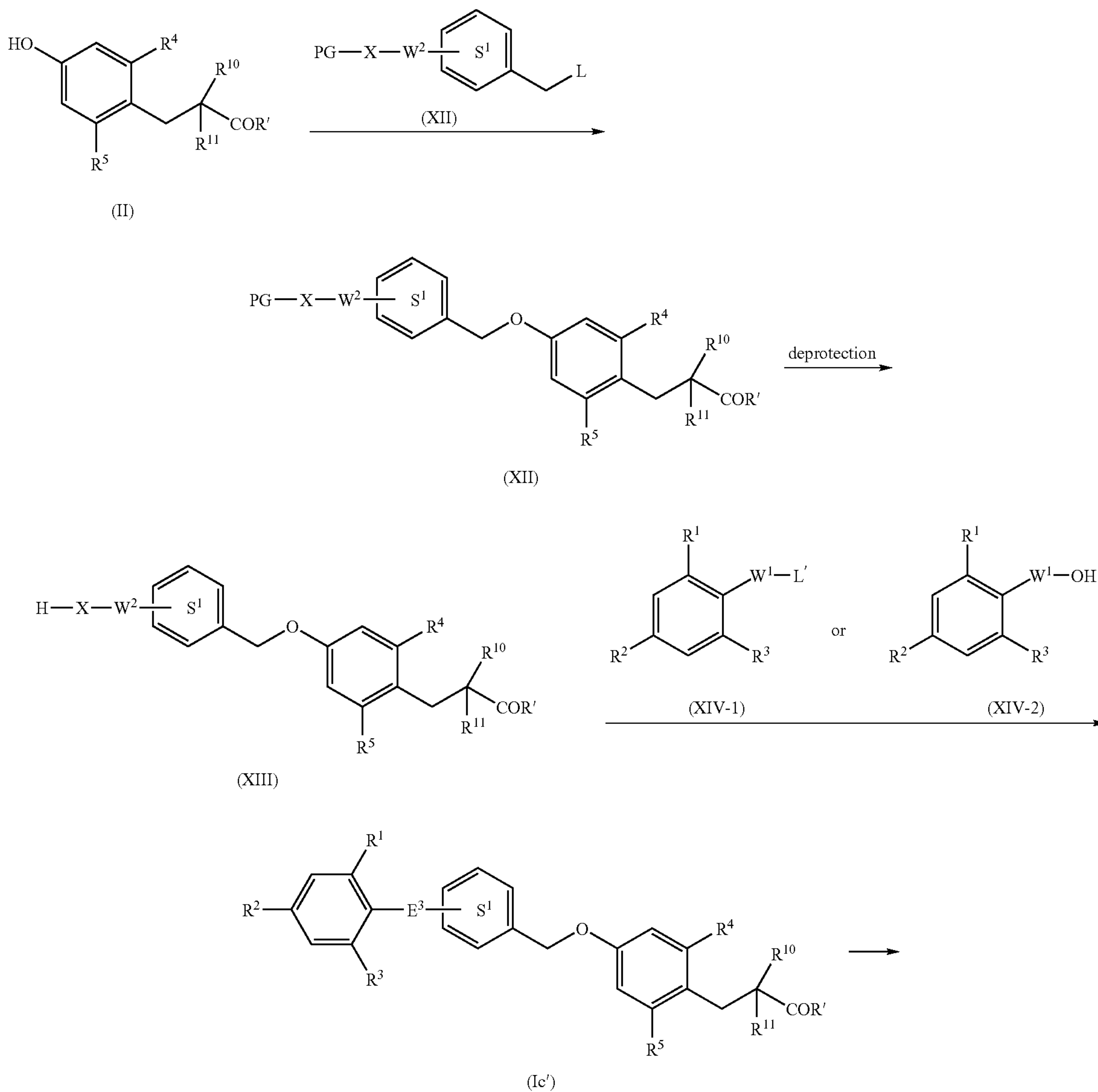
Reaction Scheme 3
