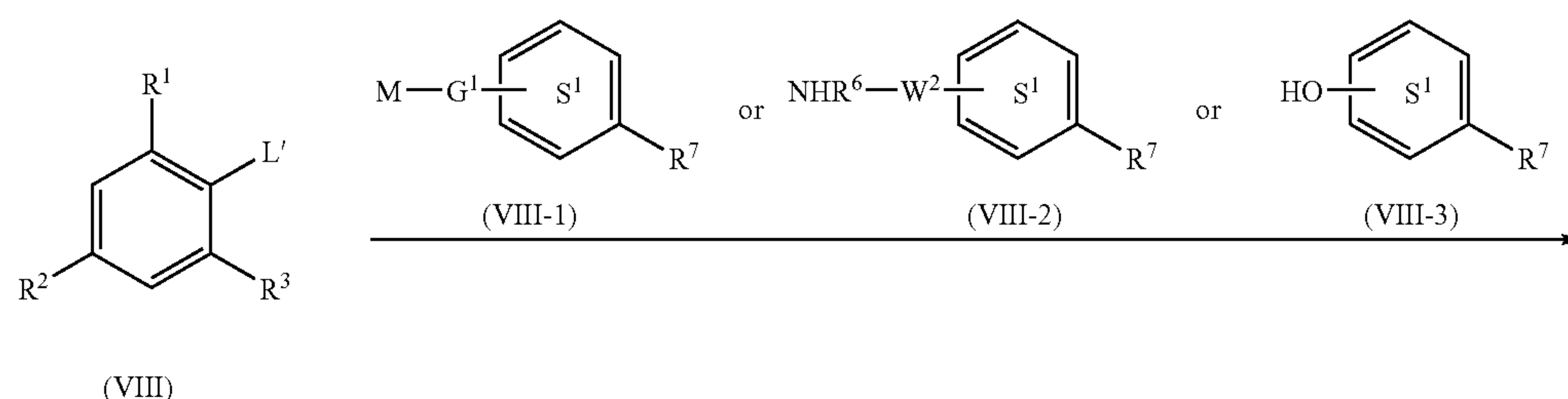
Reaction Scheme 2'
