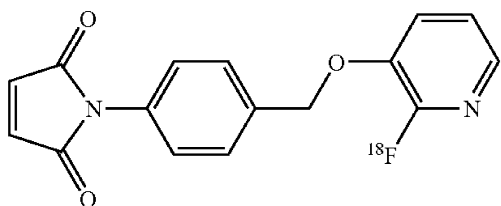
1-[4-(2-[ 18 F]Fluoro-pyridin-3-yloxymethyl)-phenyl]-pyrrole-2, 5-dione
