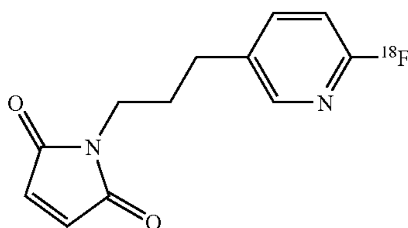
1-[3-(6-[ 18 F]Fluoro-pyridin-3-yl)-propyl]-pyrrole-2, 5-dione
