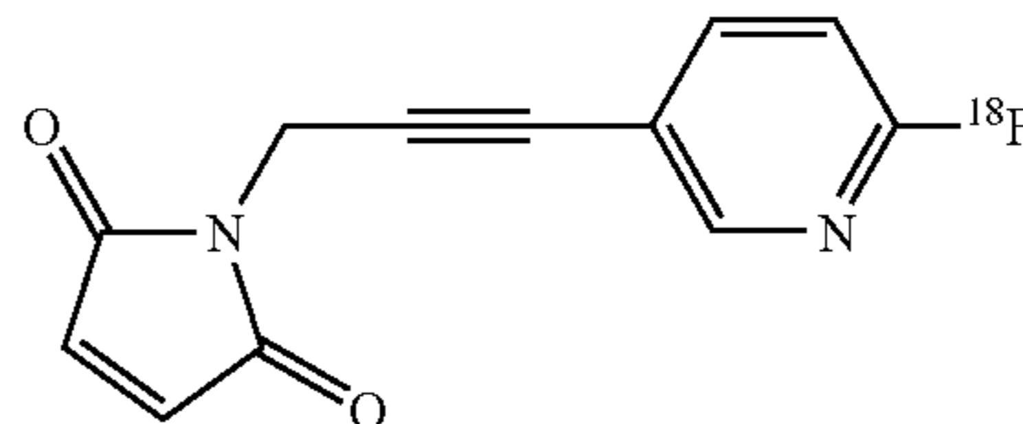
1-[3-(6-[ 18 F]Fluoro-pyridin-3-yl)-allyl]-pyrrole-2, 5-dione
