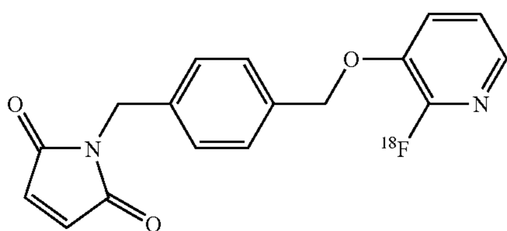
1-[4-(2-[ 18 F]Fluoro-pyridin-3-yloxymethyl)-benzyl]-pyrrole-2, 5-dione
