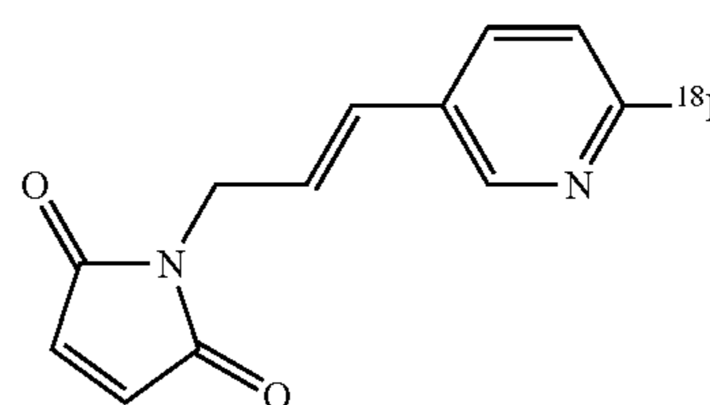
1-[3-(6-[ 18 F]Fluoro-pyridin-3-yl)-allyl]-pyrrole-2, 5-dione
