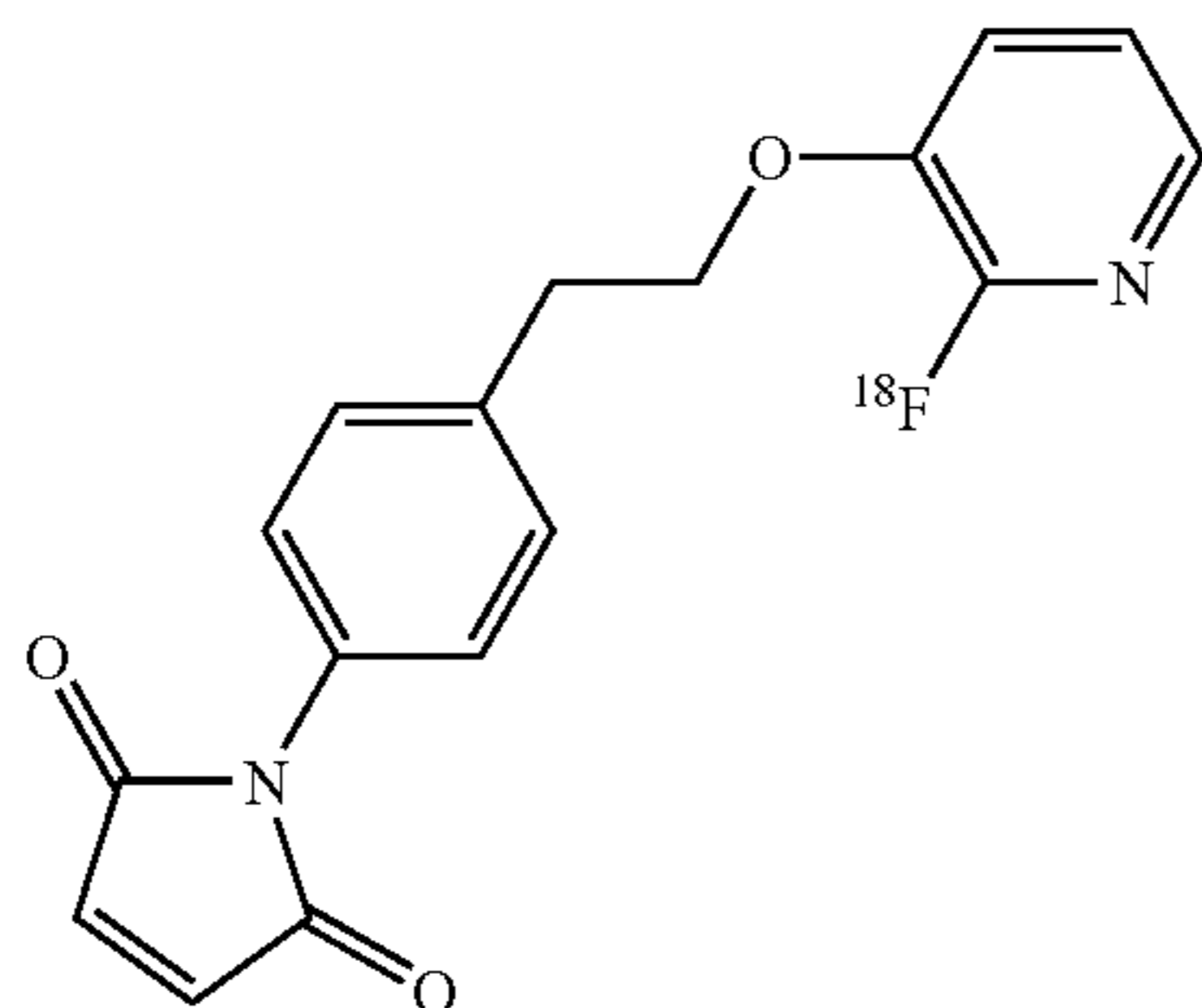
1-[4-(2-(2-[ 18 F]Fluoro-pyridin-3-yloxy)-ethyl)-phenyl]-pyrrole-2, 5-dione
