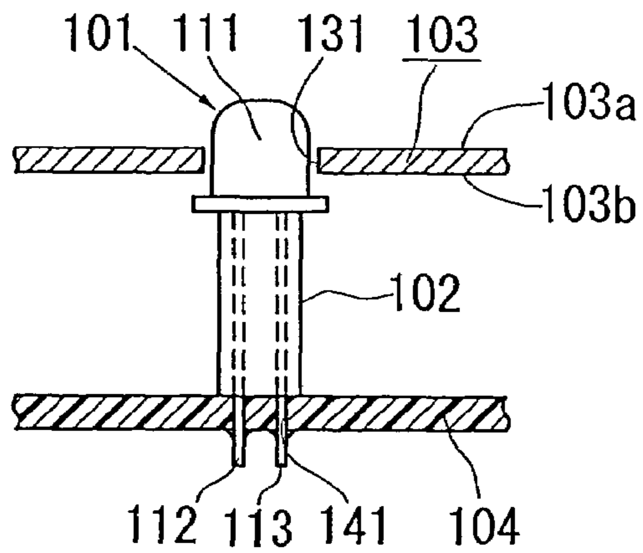
FIG. 10 PRIOR ART
