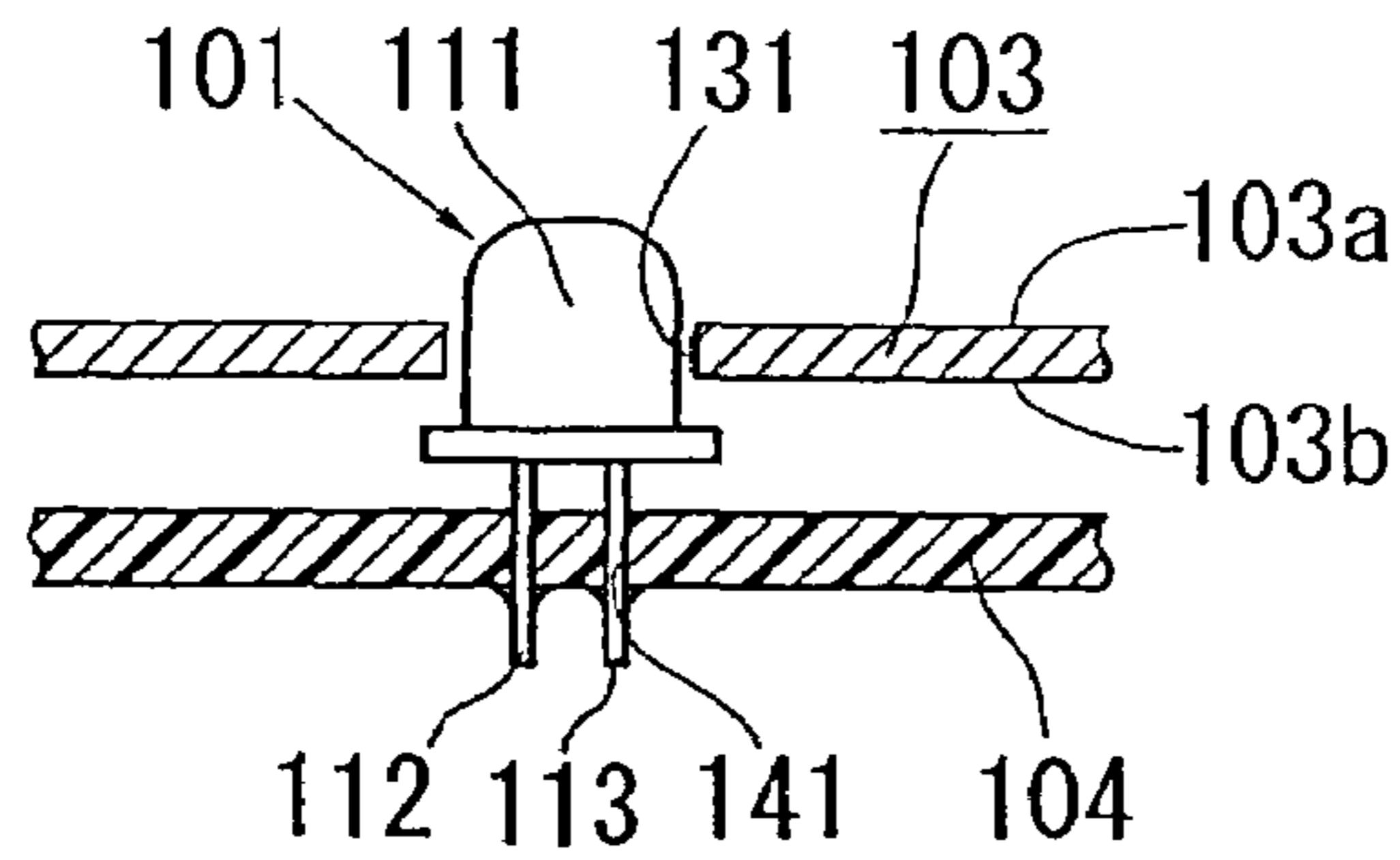
FIG. 8 PRIOR ART
