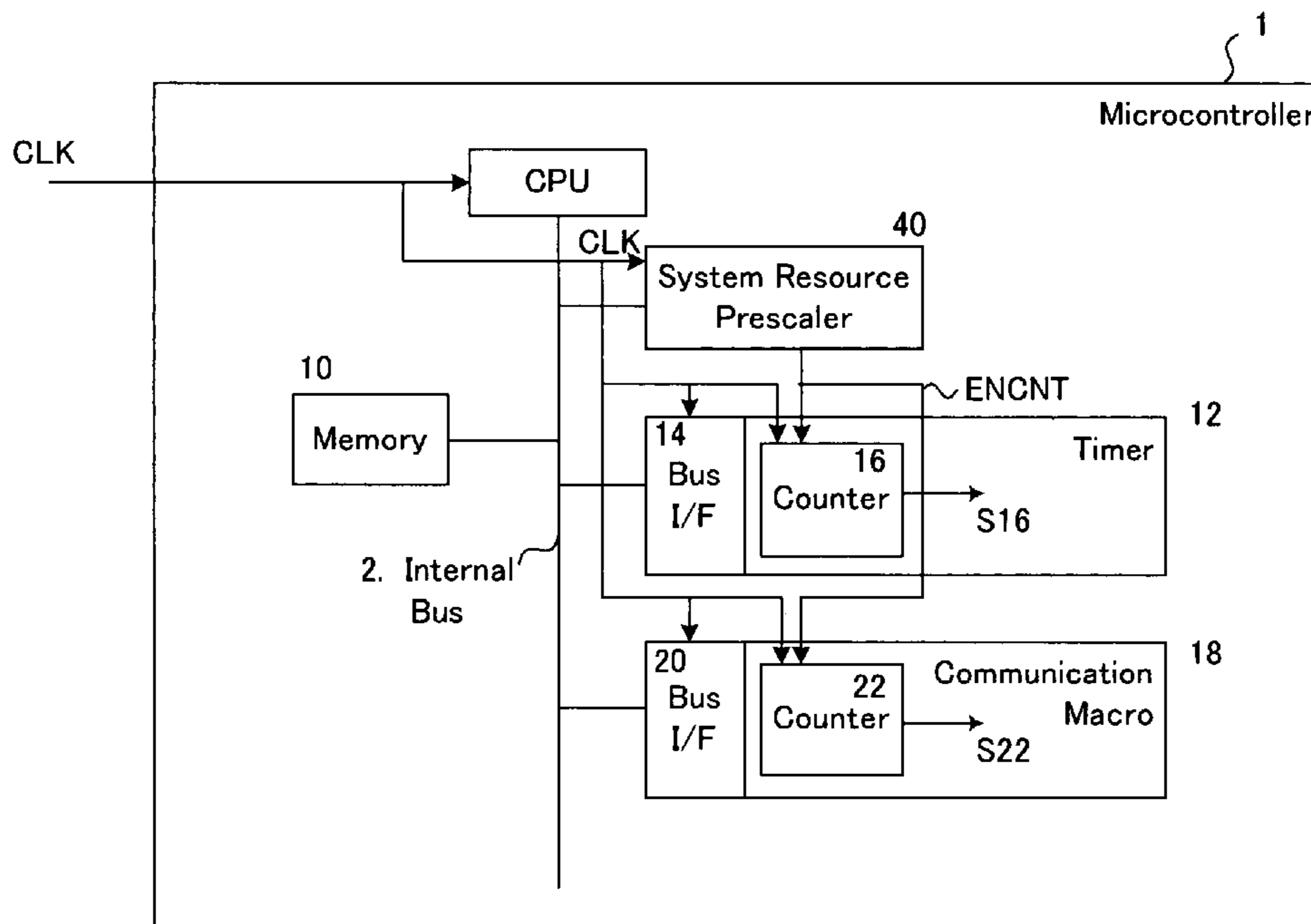
Microcontroller of Embodiment
