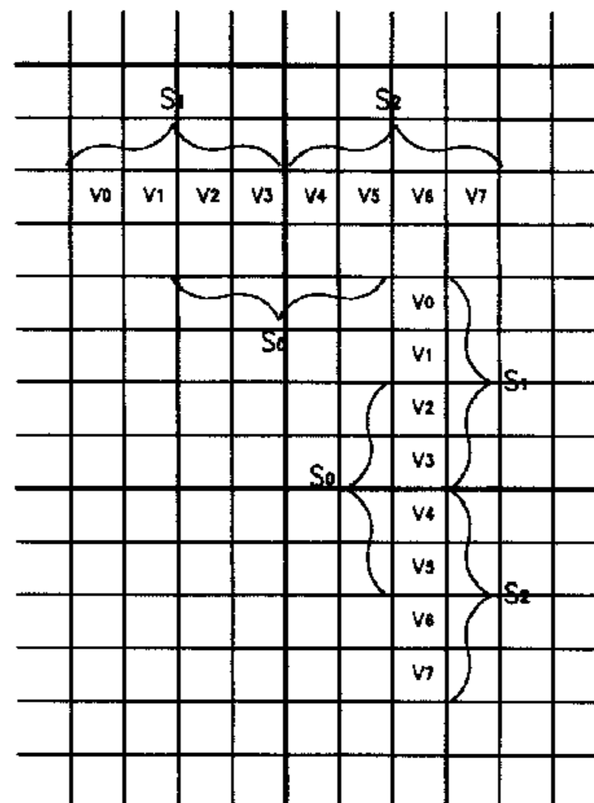
(block boundary)
