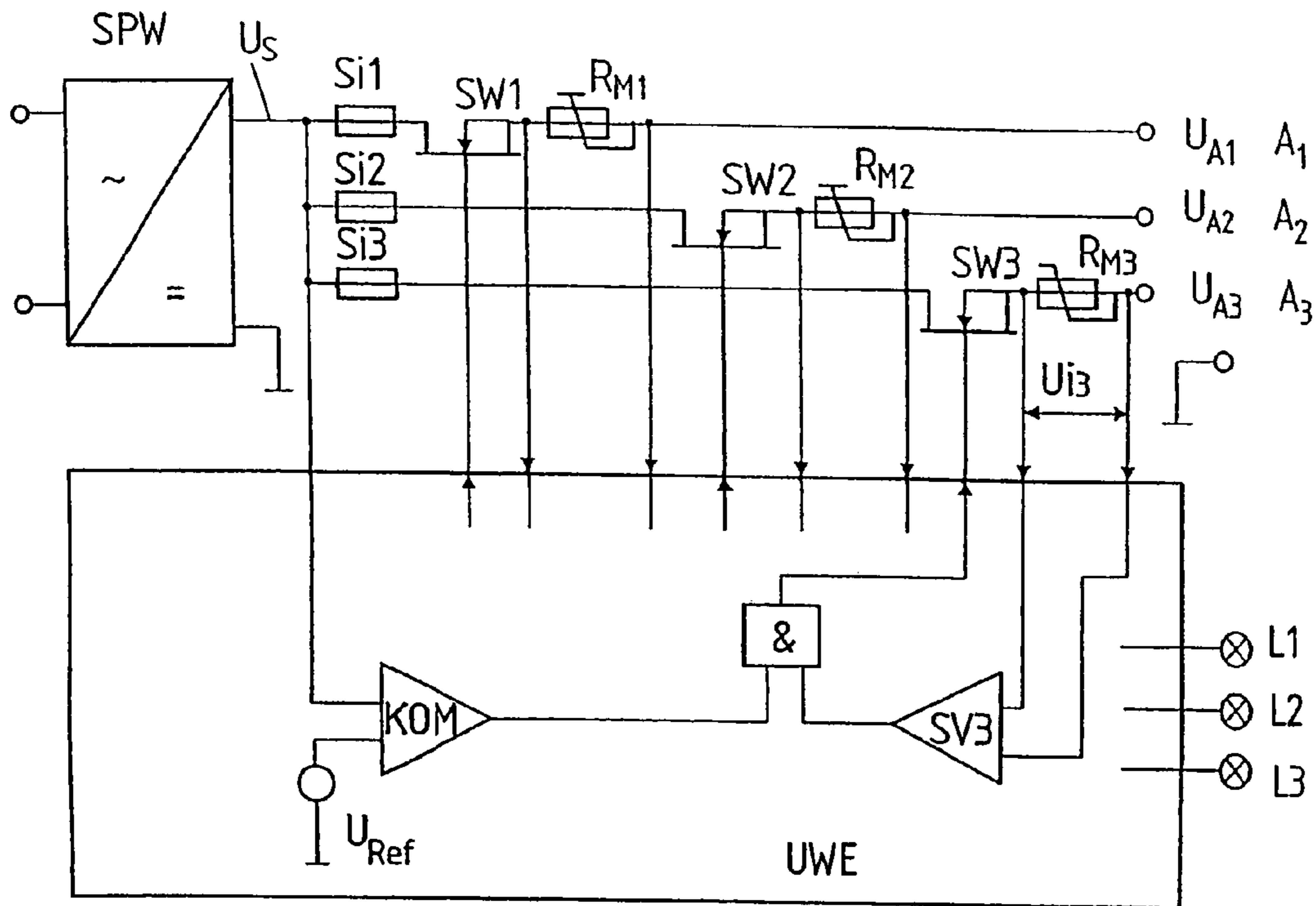
Fig. 1 (PRIOR ART)
