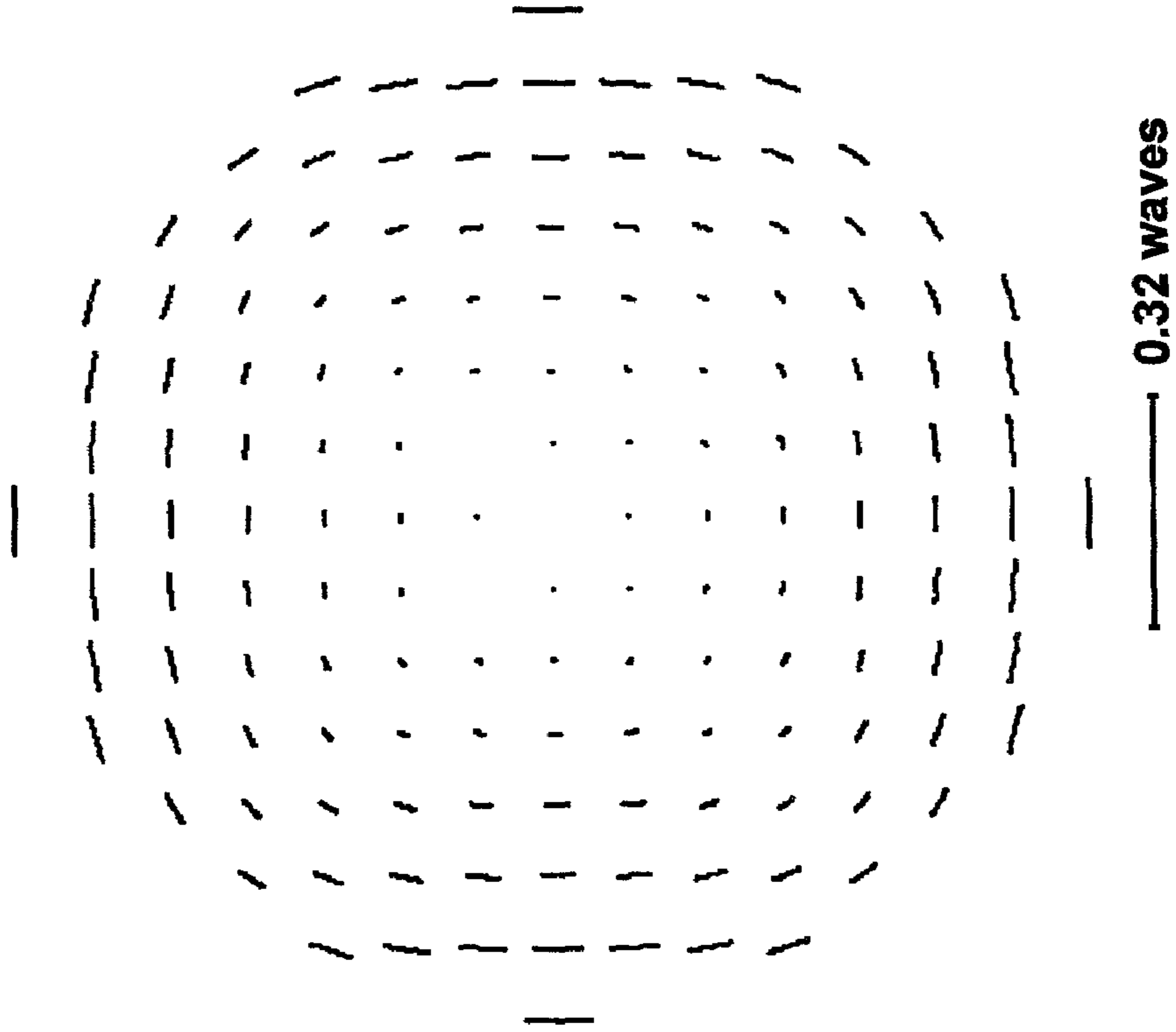
Net Retardance without Rotator, Extreme Field
