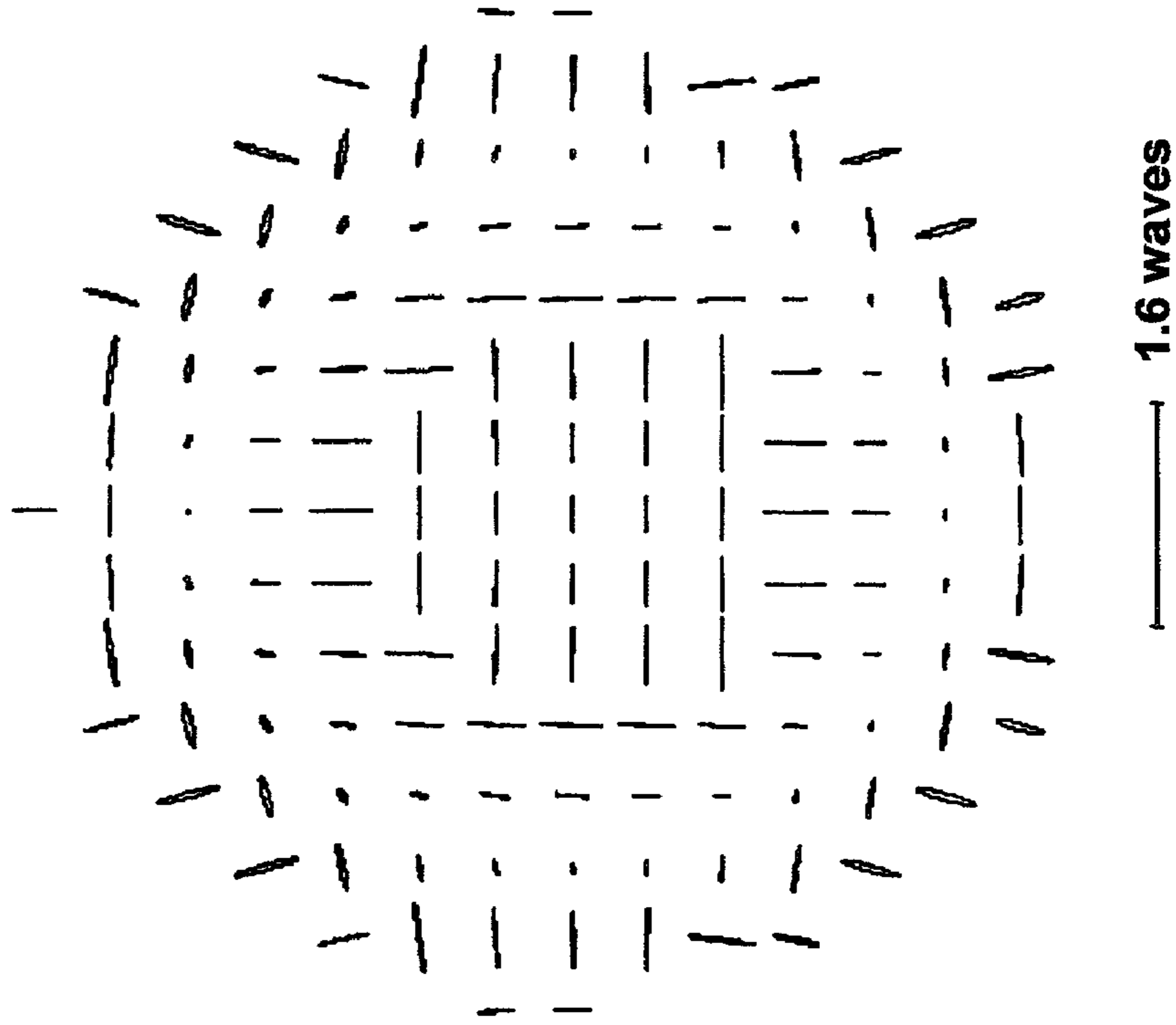
Retardance, Extreme Field
