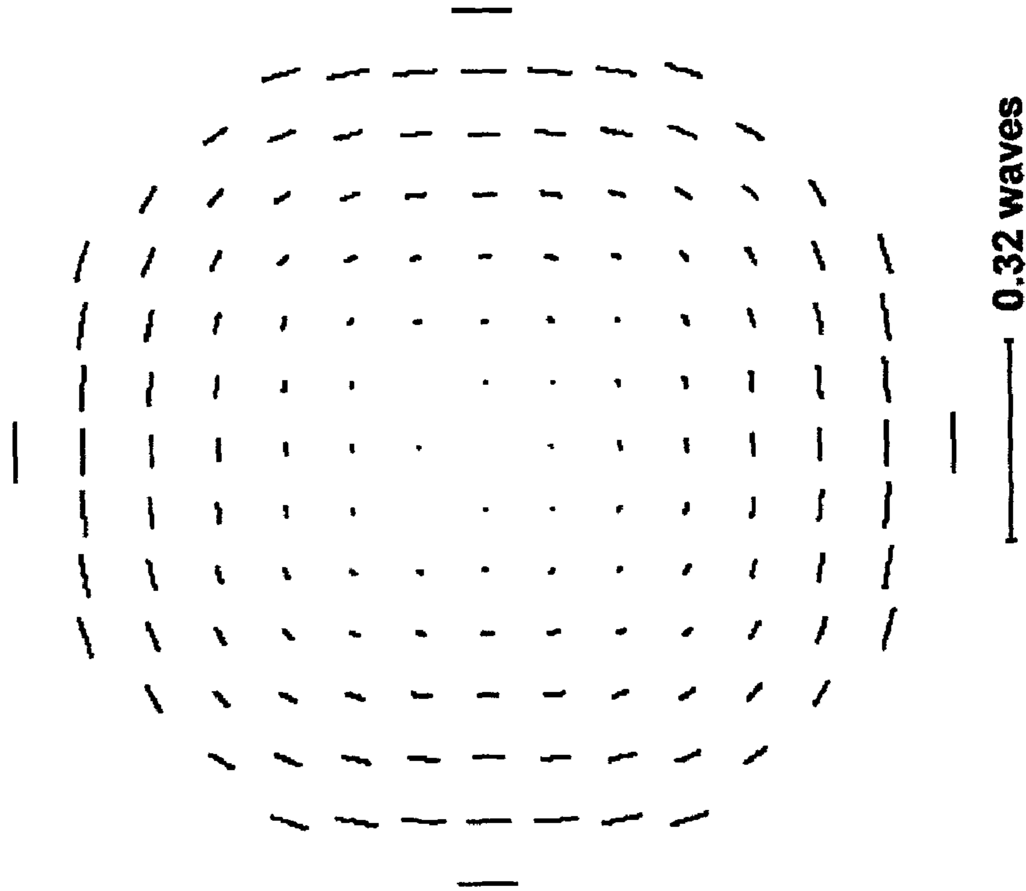
Net Retardance without Rotator, On-Axis Field
