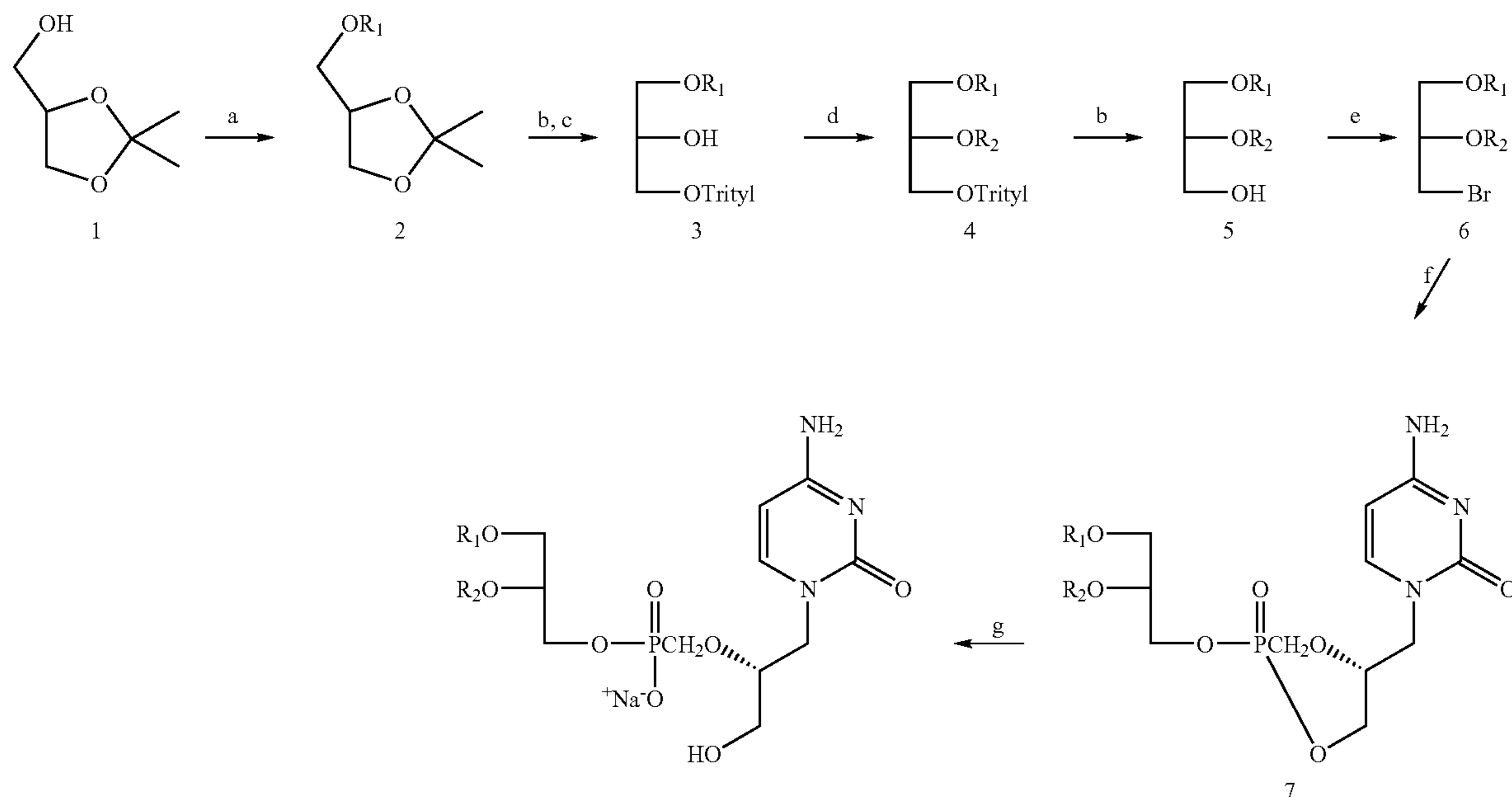
Scheme V
