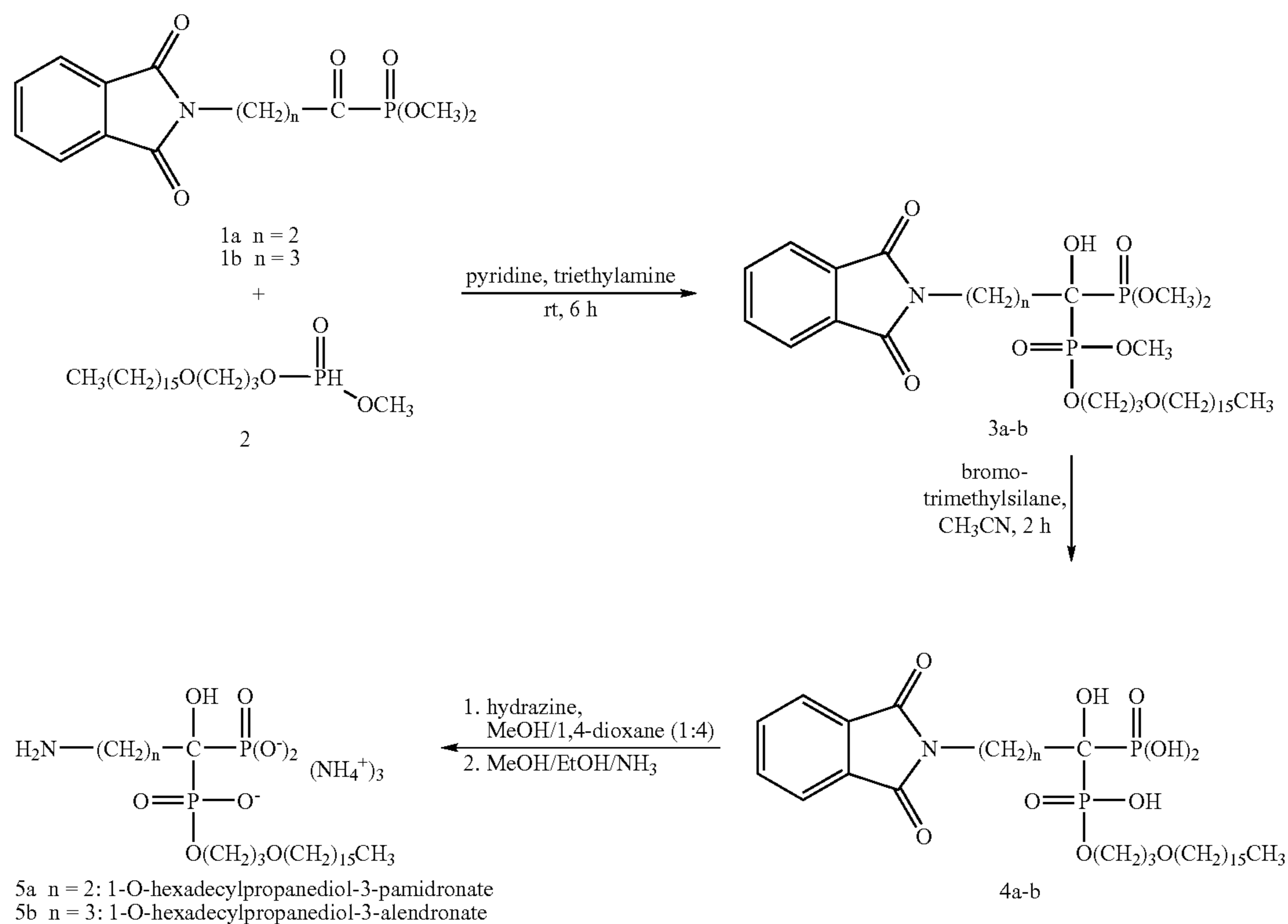
Scheme I
