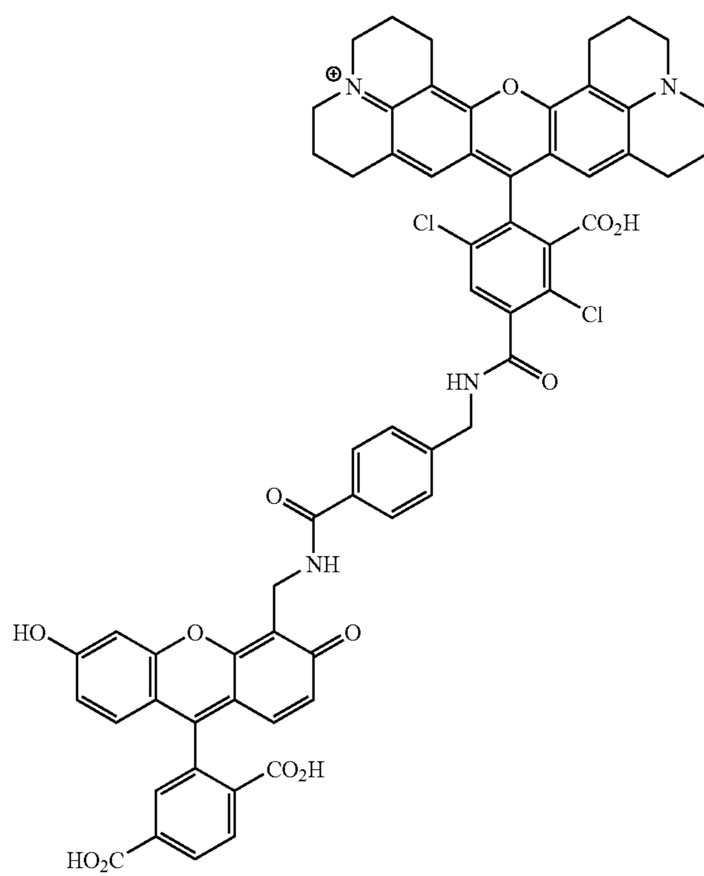
6-CFB-DROX-2
