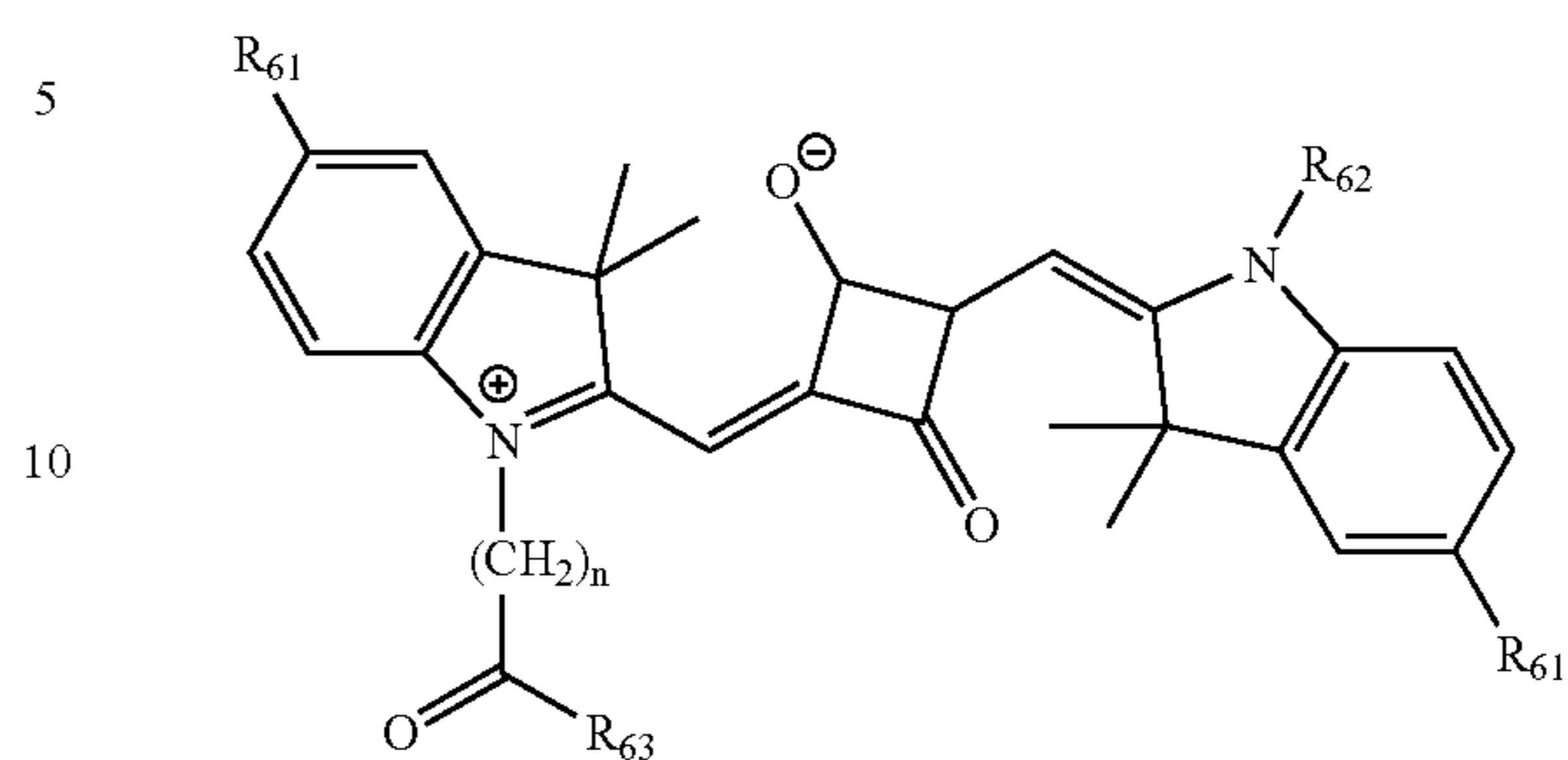
SQUARAINE
