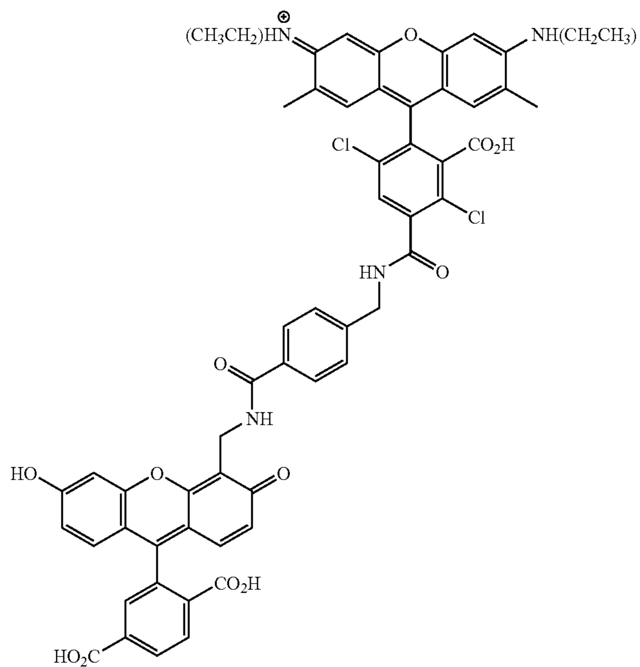
6-CFB-DR6G-2
