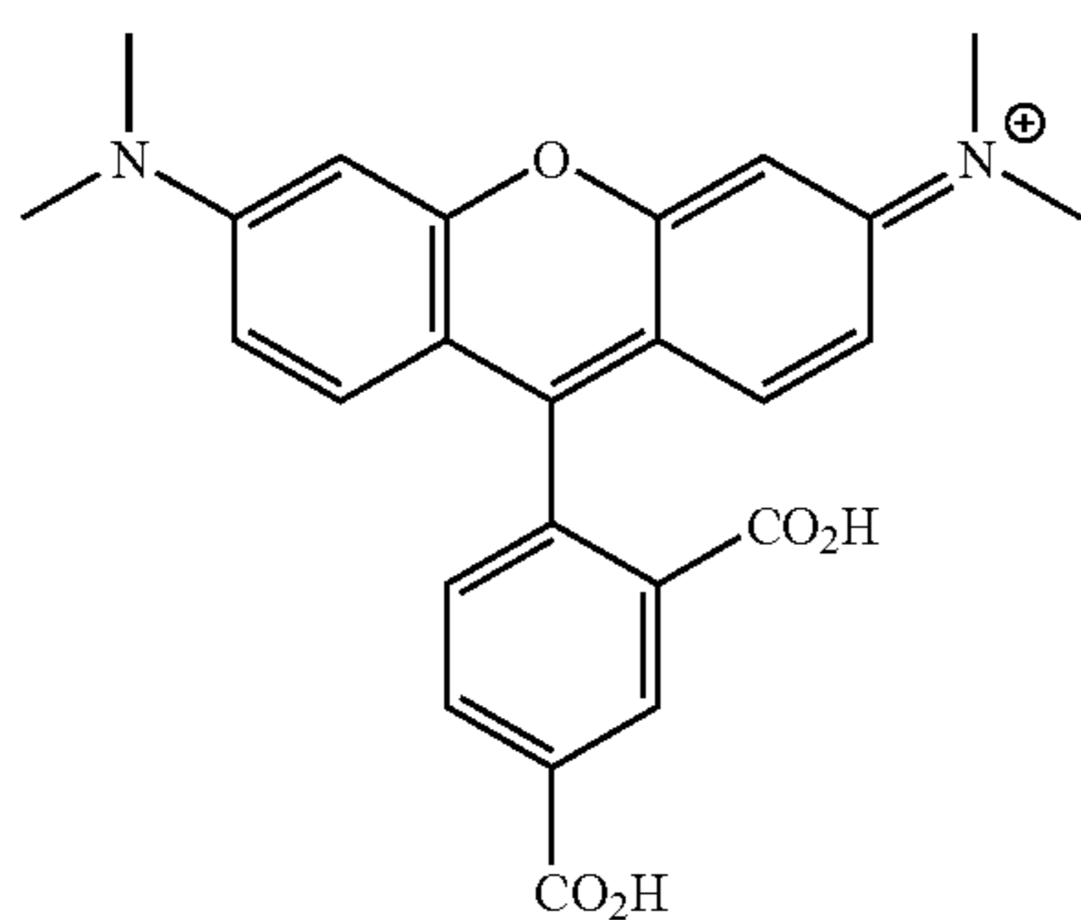
TAMRA
