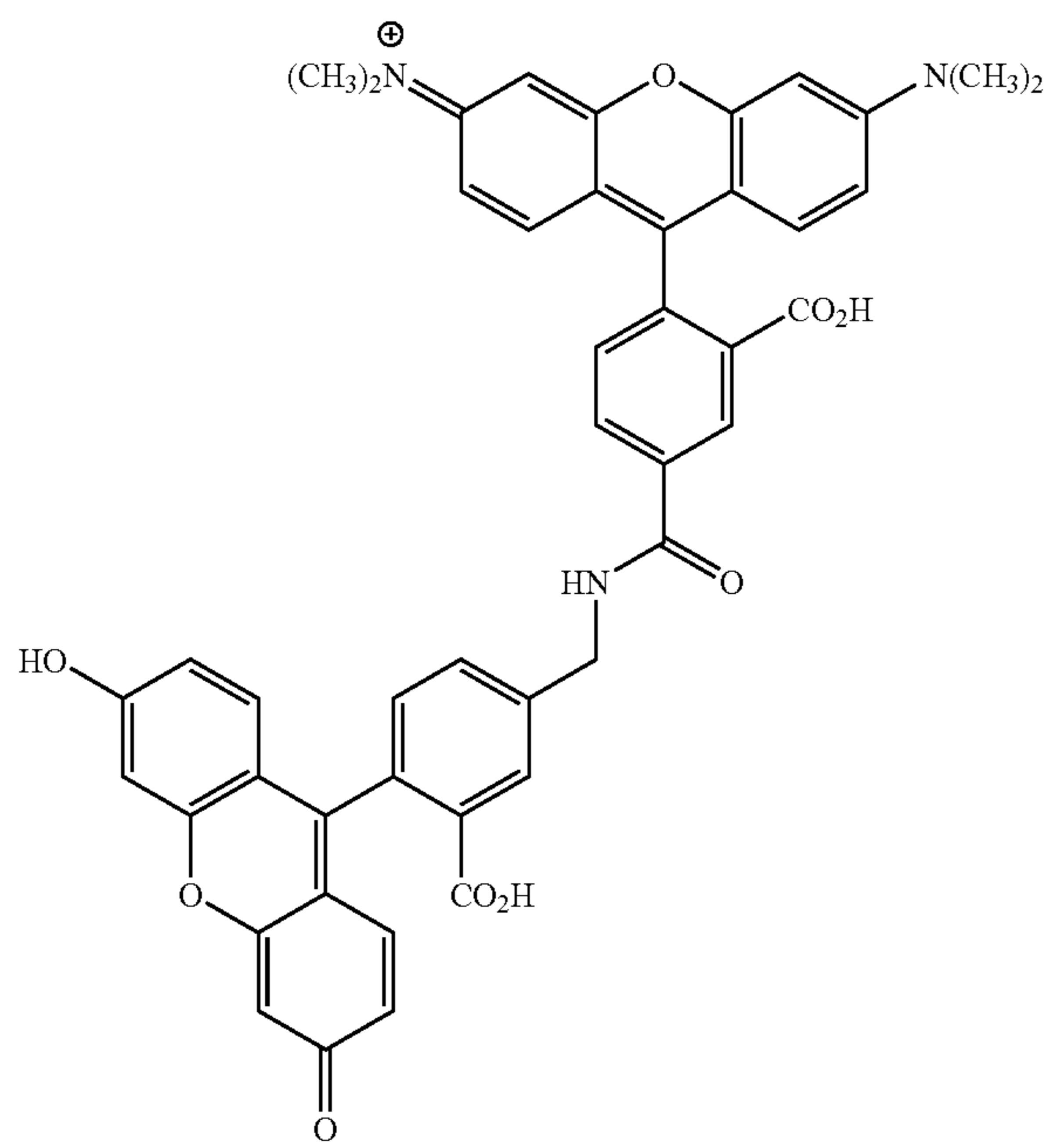
5TMR-5AMF
