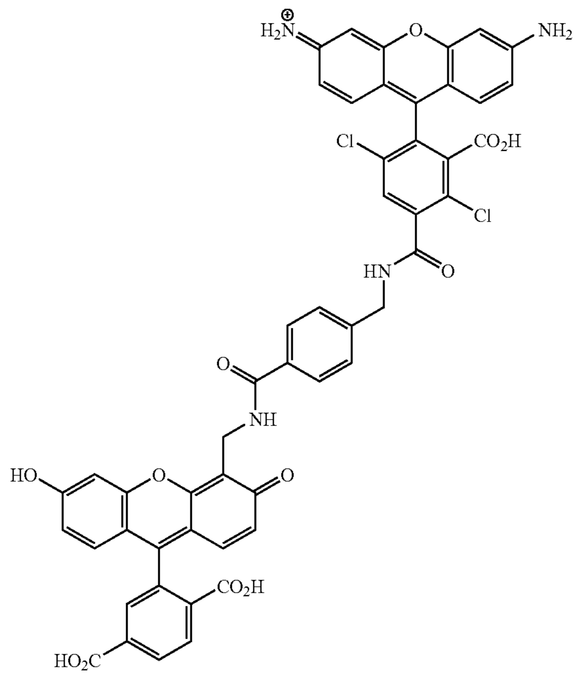
6-CFB-DR110-2
