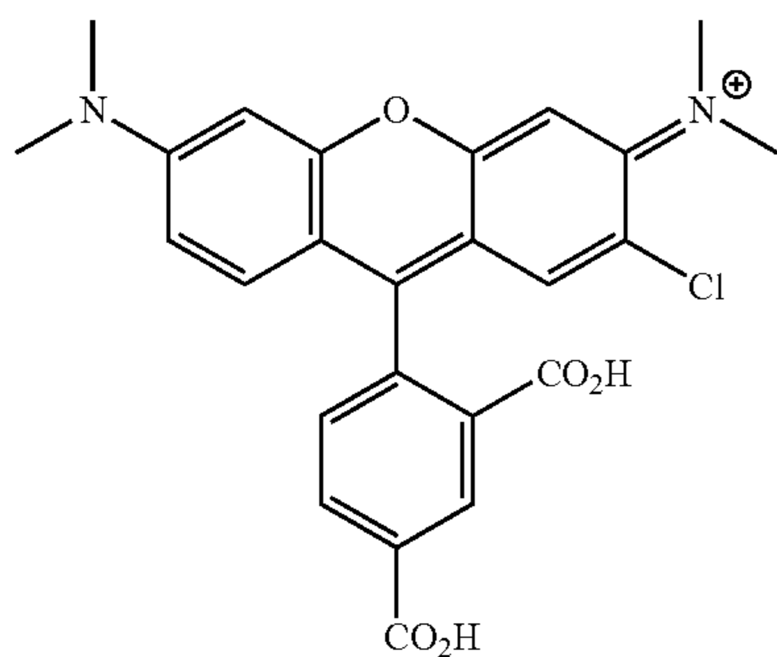
5-carboxyrhodamine
