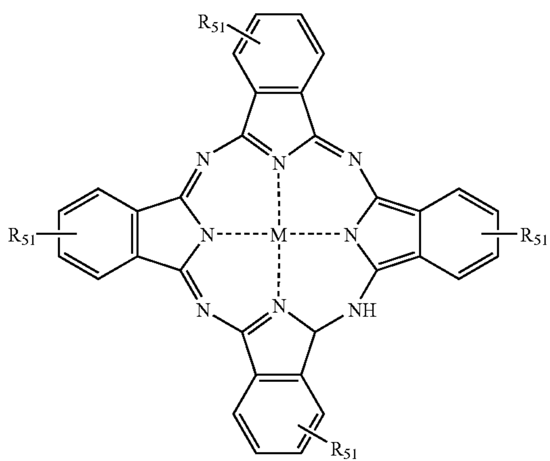
PHTHALOCYANINE
