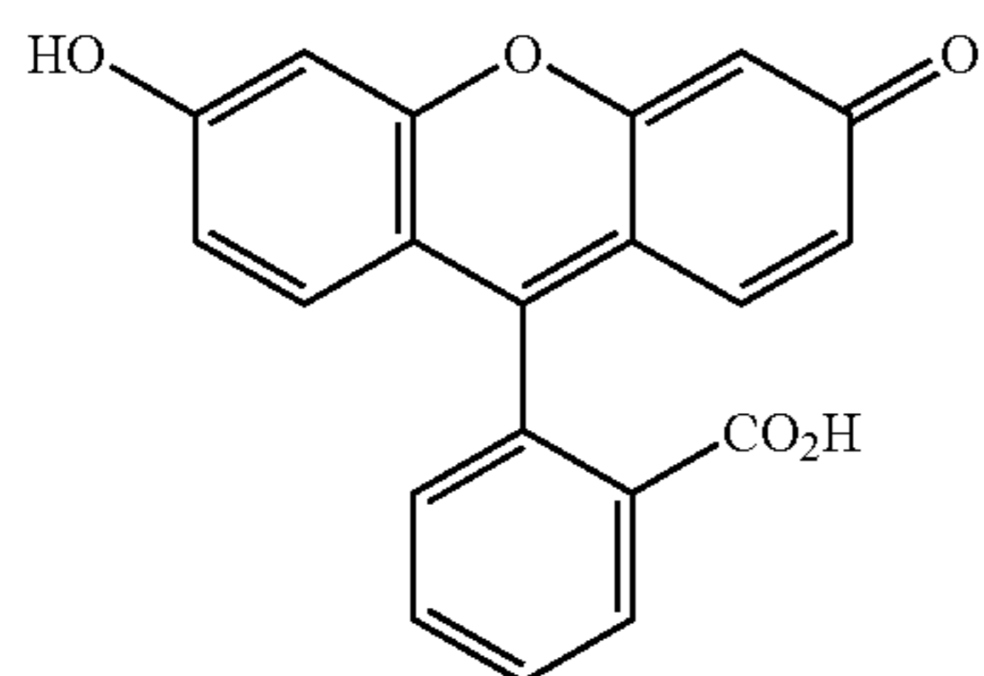
Fluorescein
