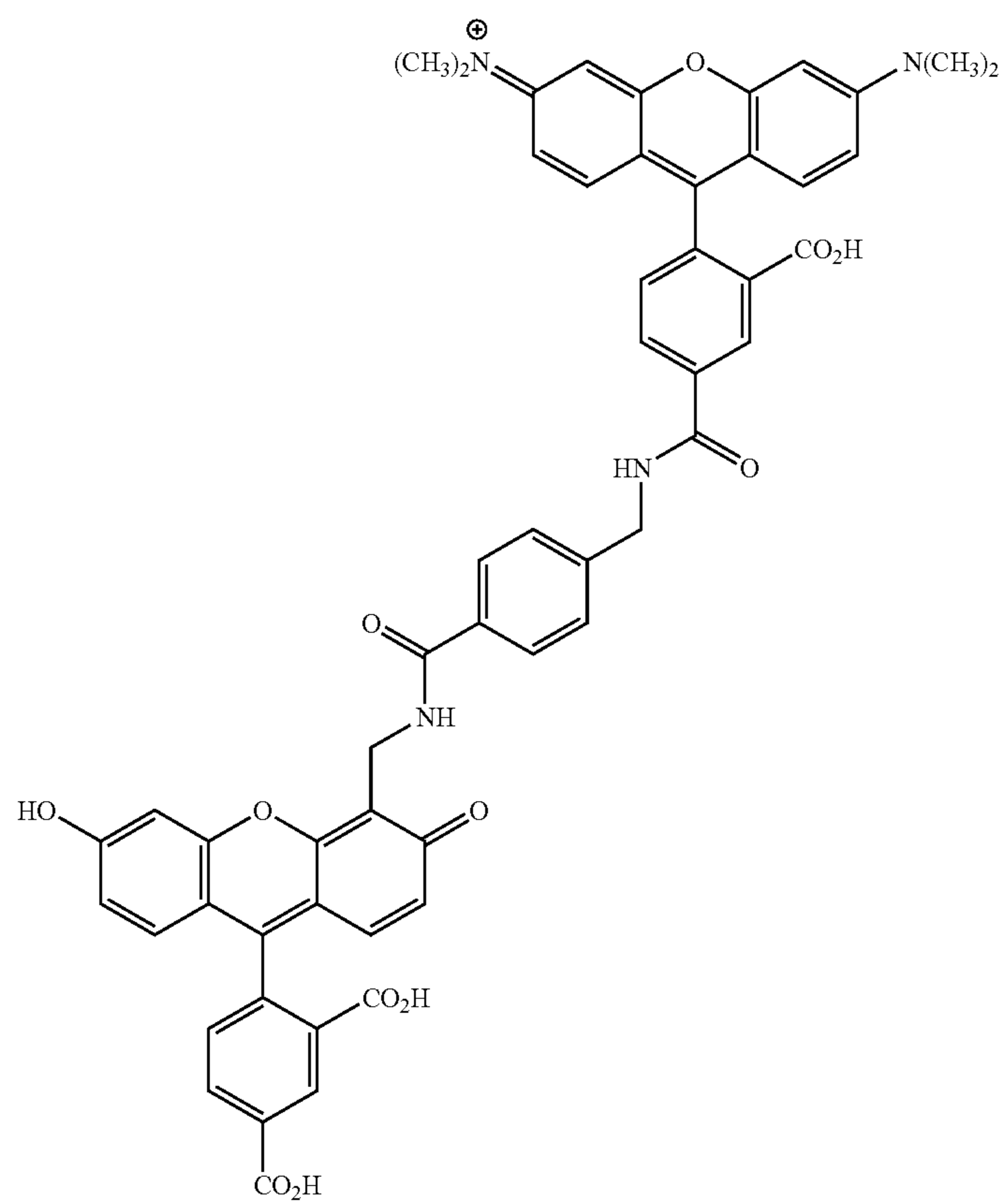
5-TMR-B-CF
