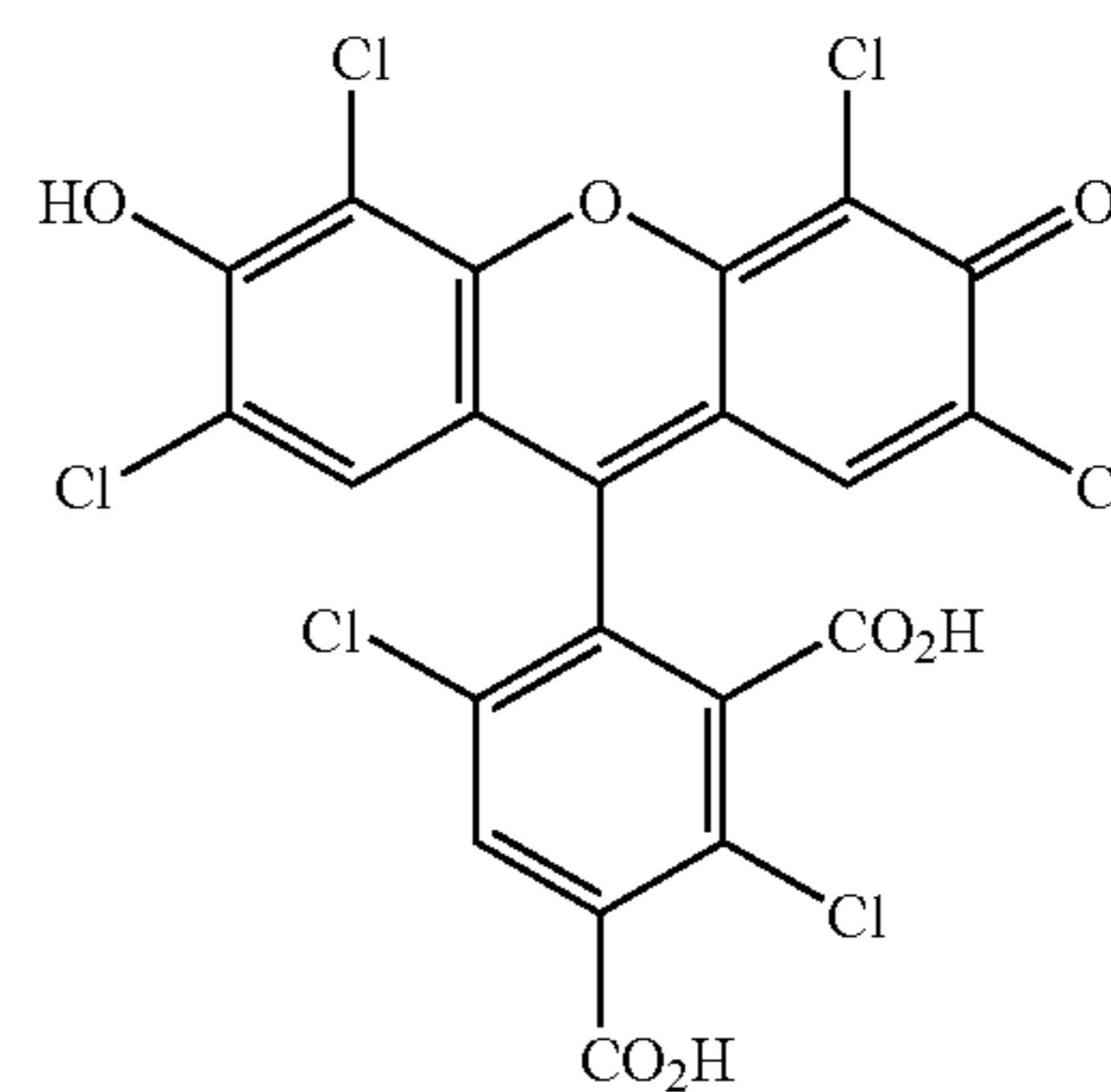
5-carboxy-HEX
