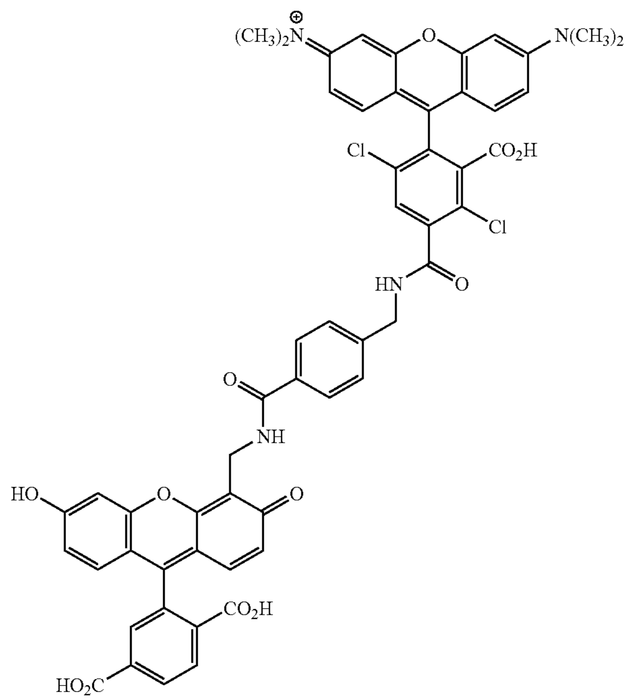
6-CFB-DTMR-2
