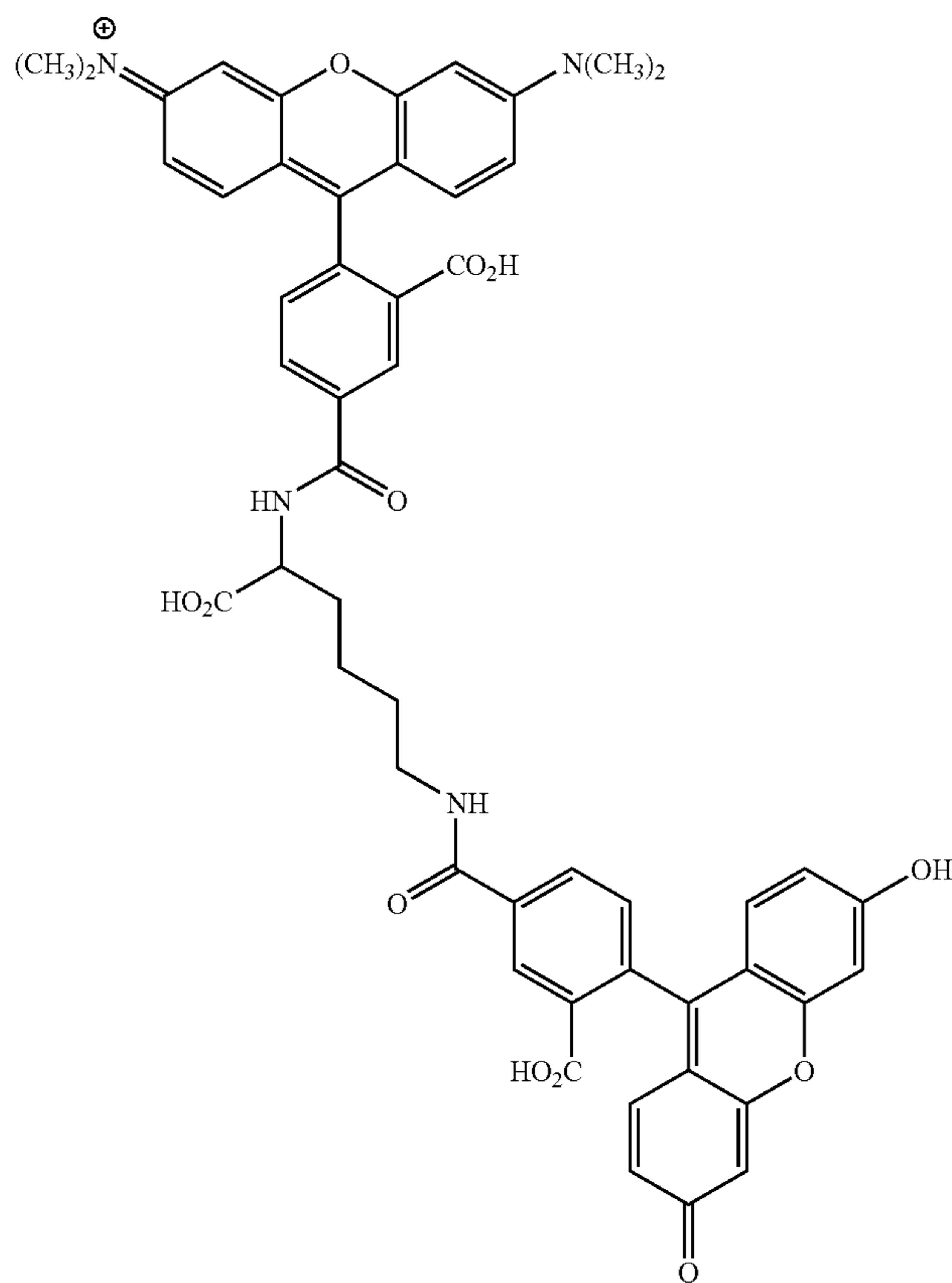
5TMR-lys-5FAM
