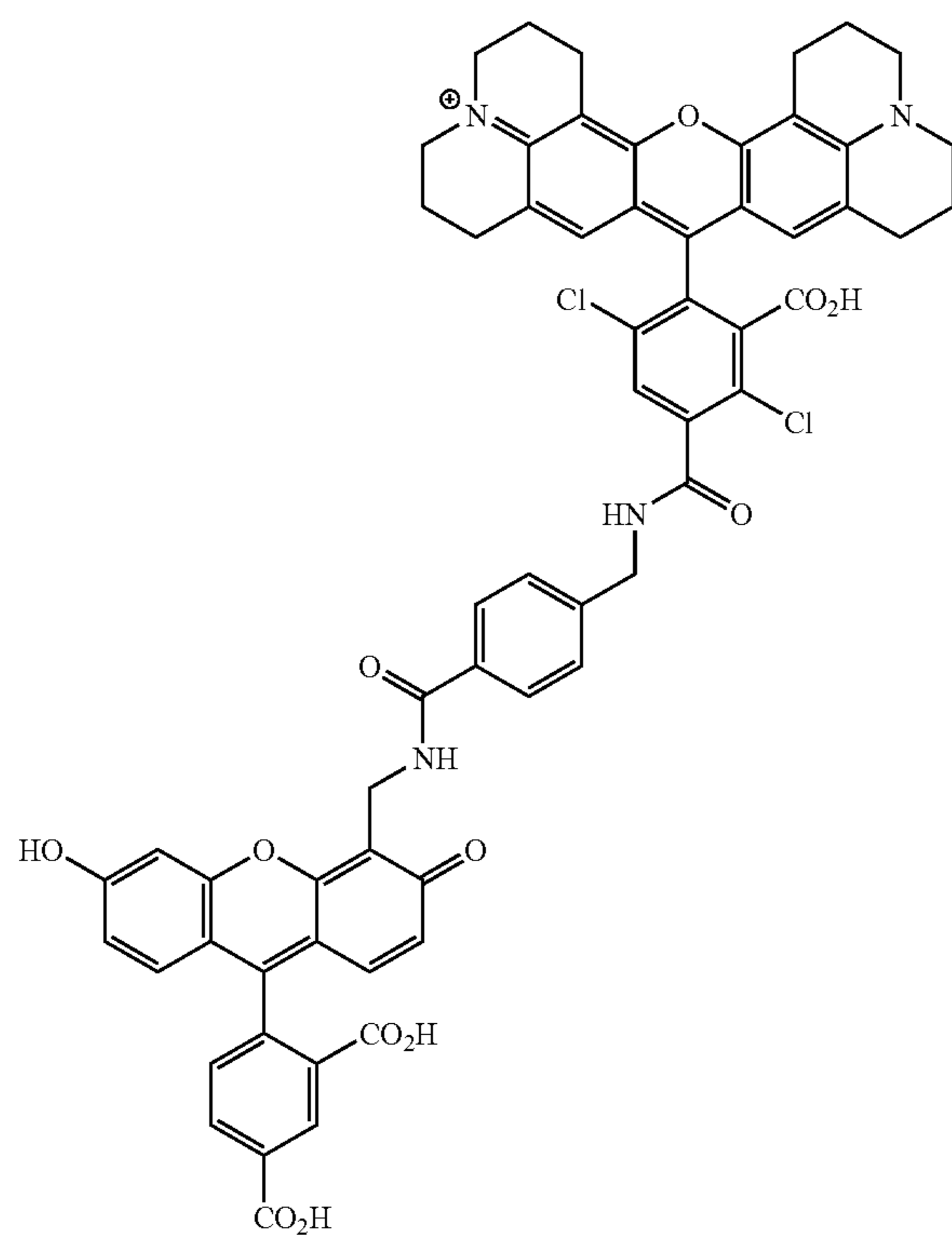
5-CFB-DROX-2
