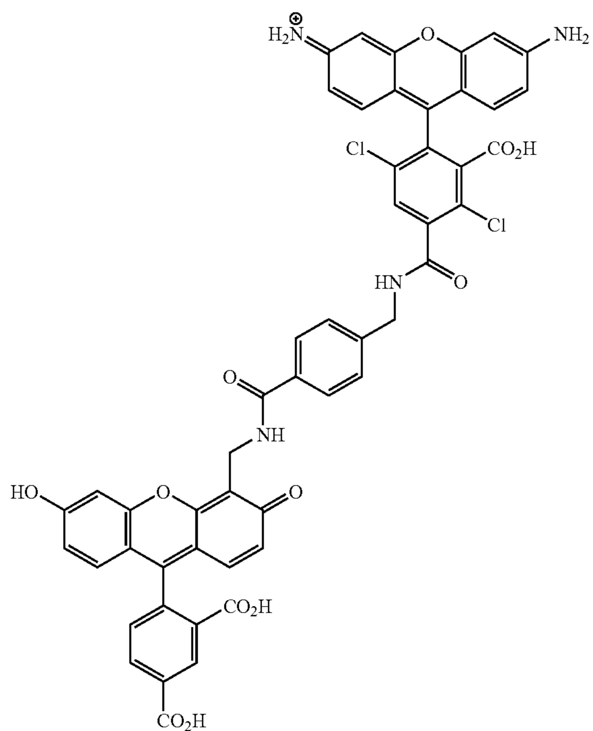
5-CFB-DR110-2
