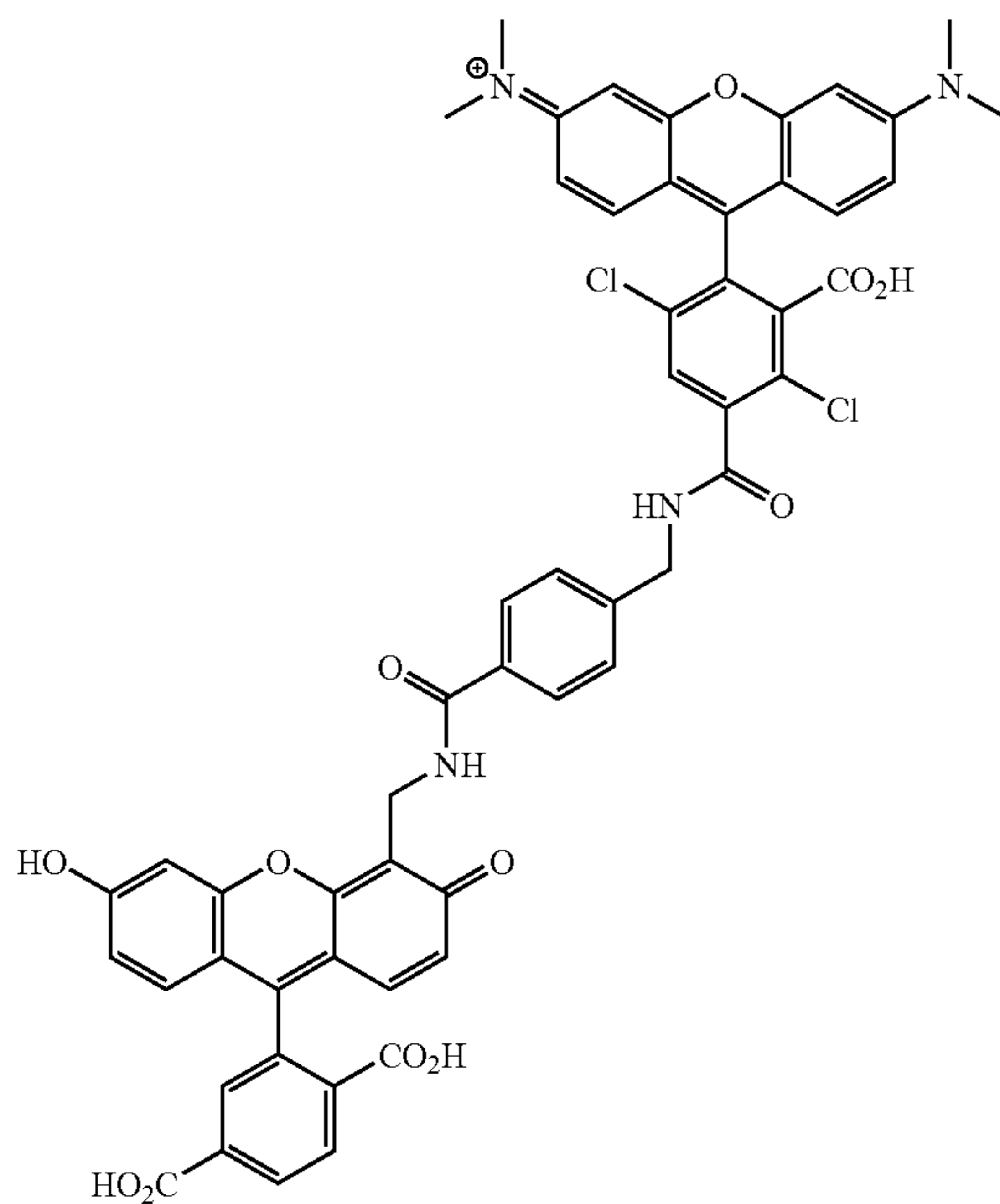
6-CF-B-DTMR-2
