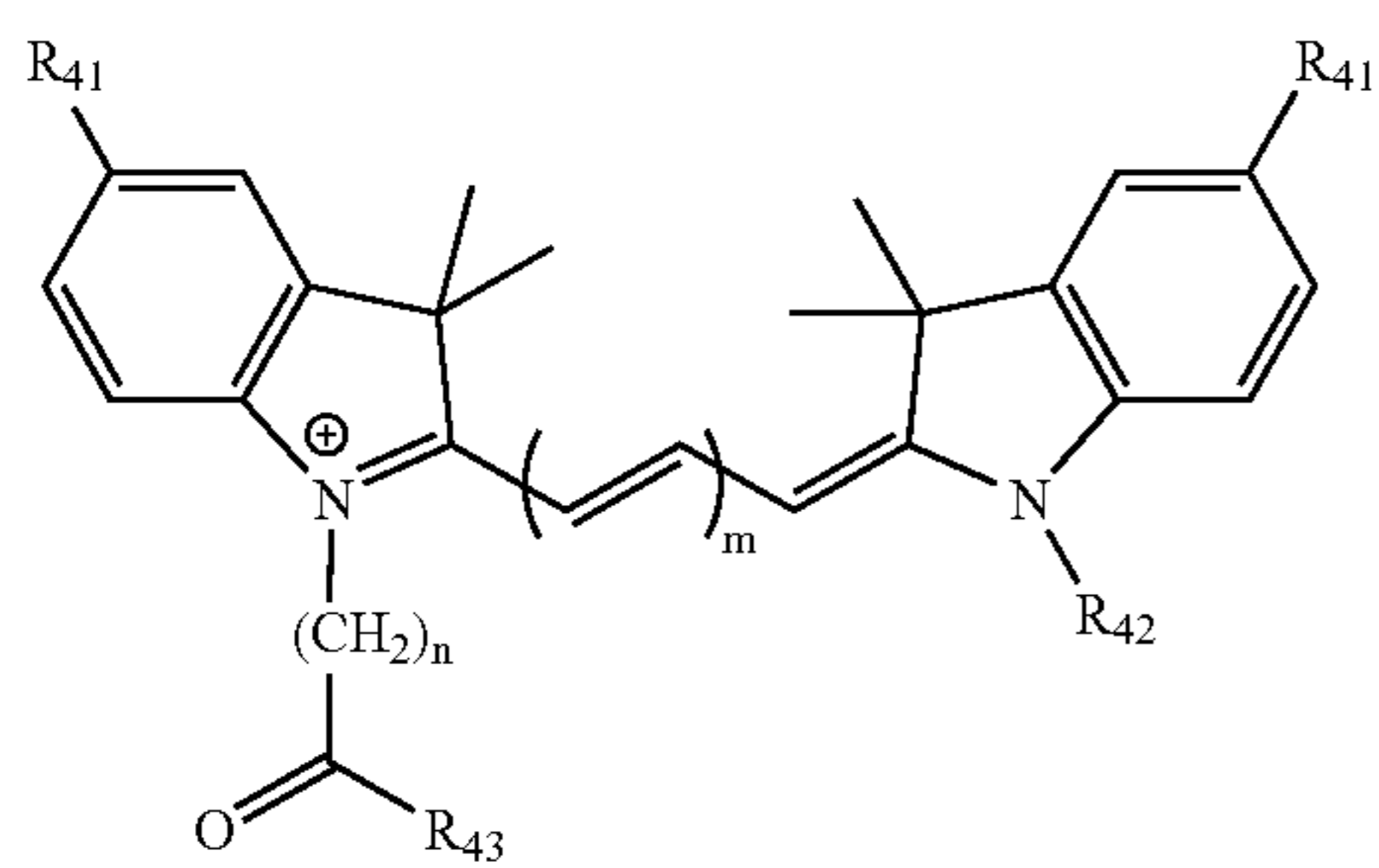
CYANINE
