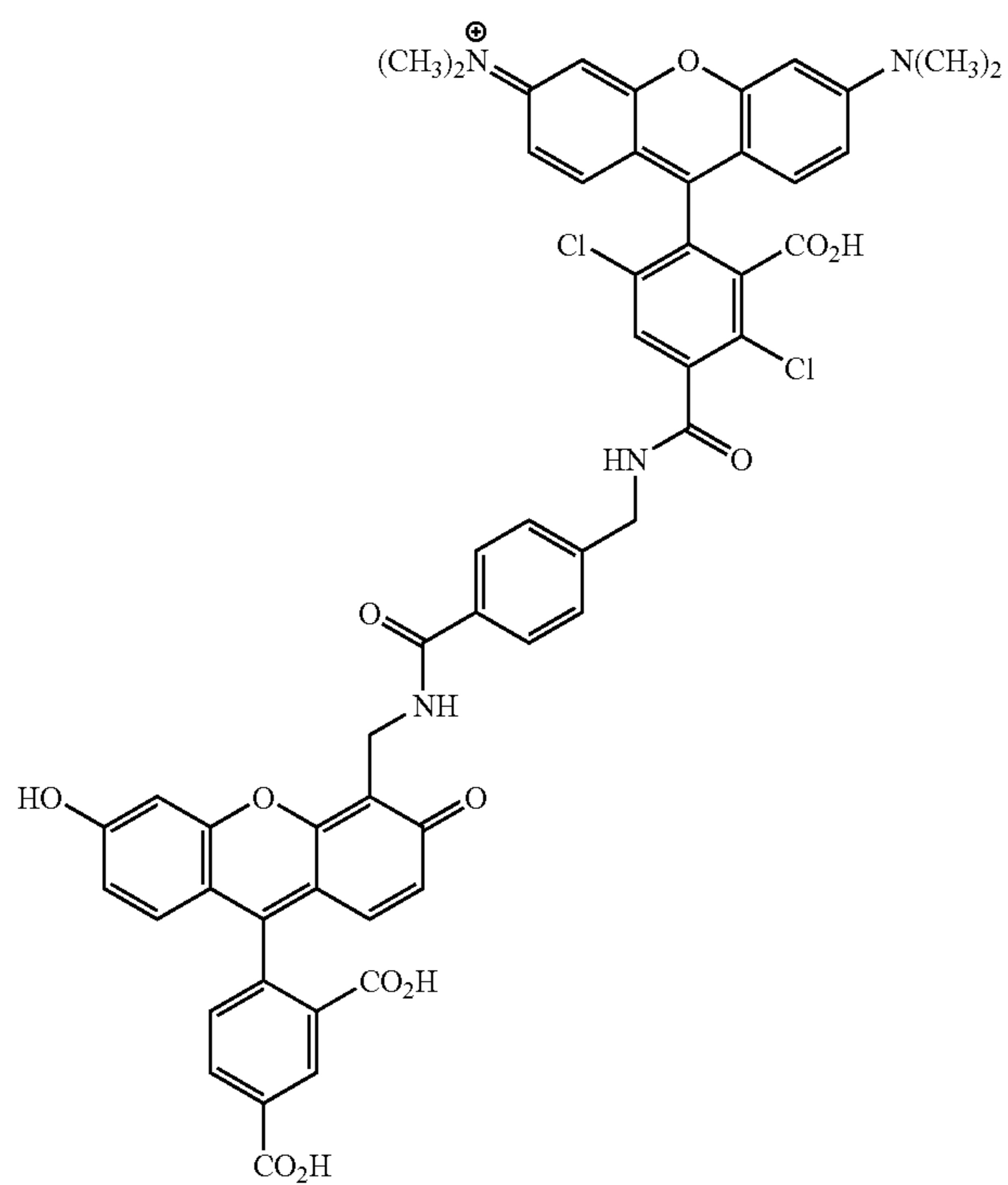
5-CFB-DTMR-2
