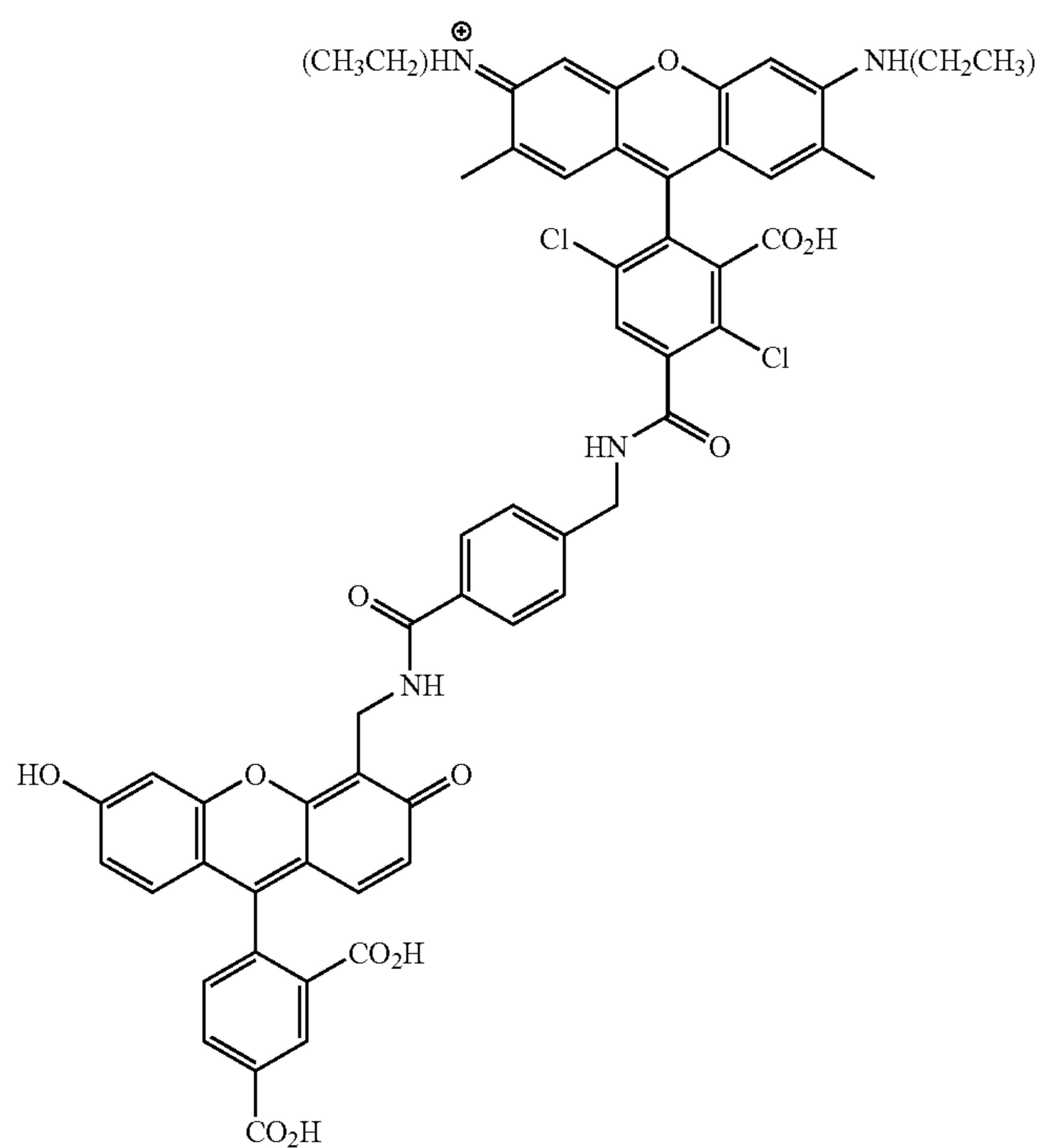
5-CFB-DR6G-2
