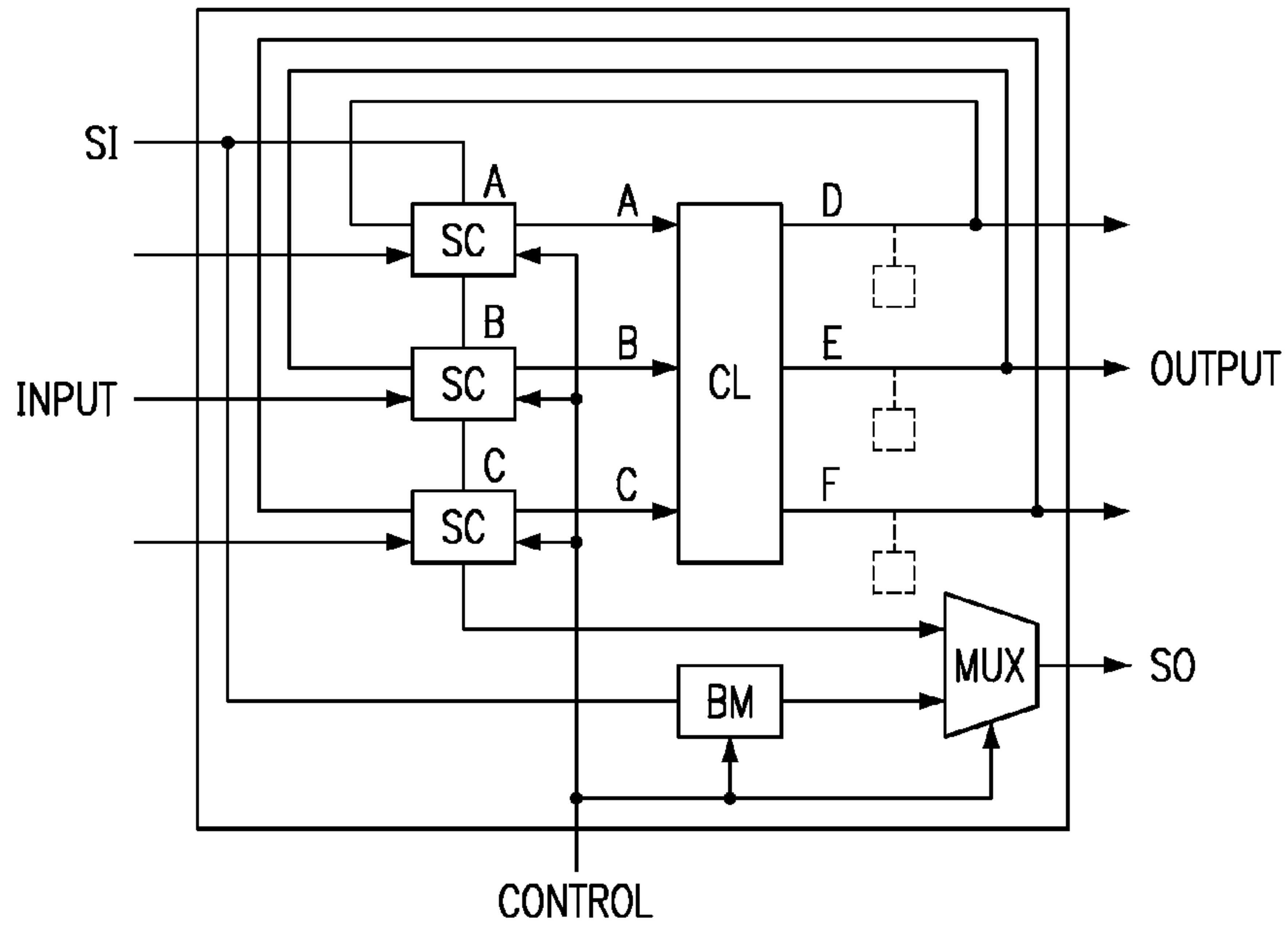
FIG. 3 (PRIOR ART)
