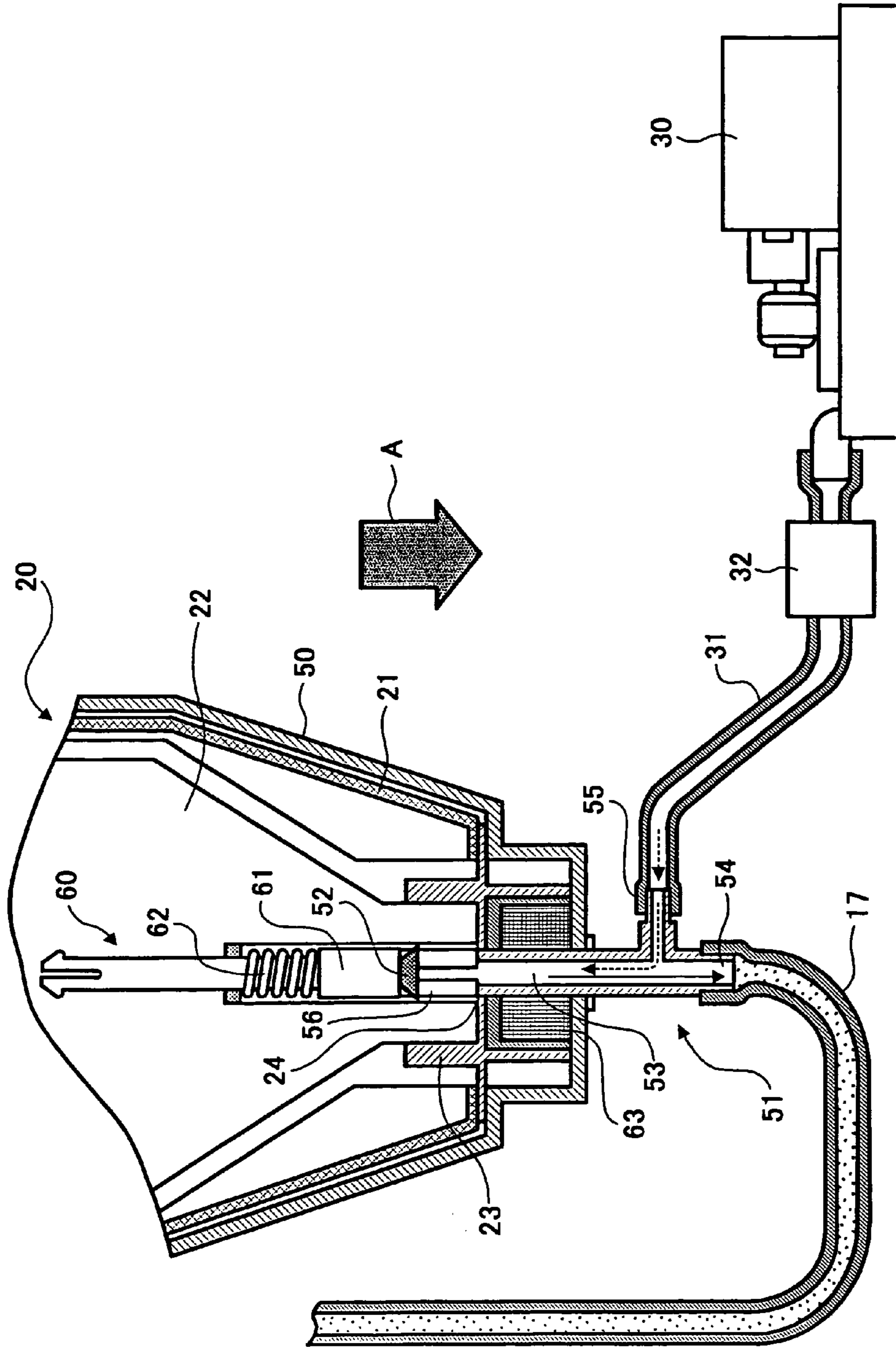
FIG. 6 PRIOR ART
