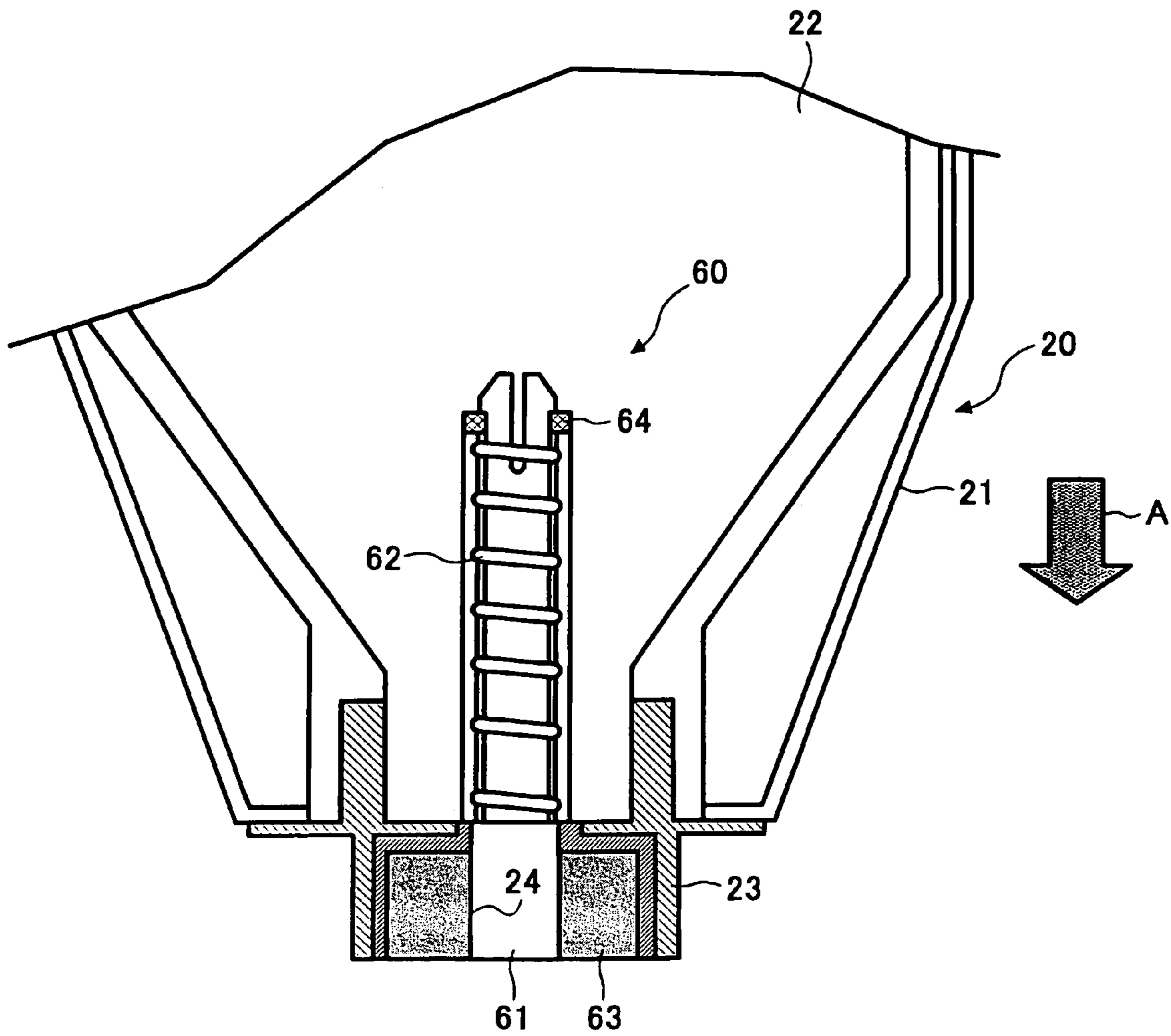
FIG. 5 PRIOR ART
