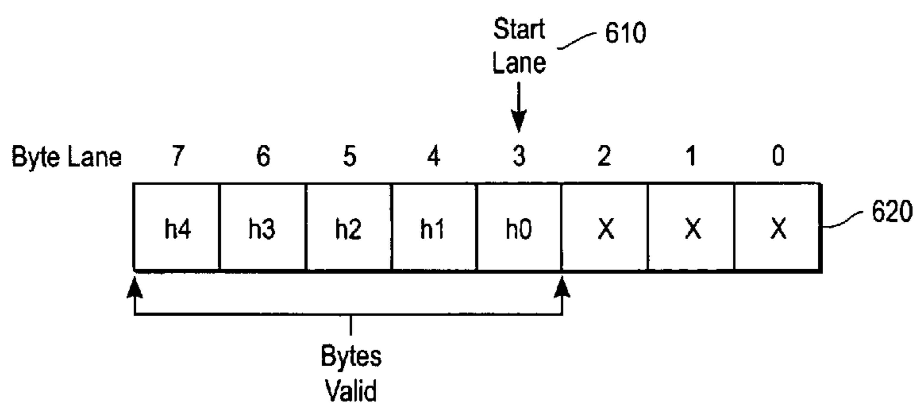
FIG. 5A Host Data
