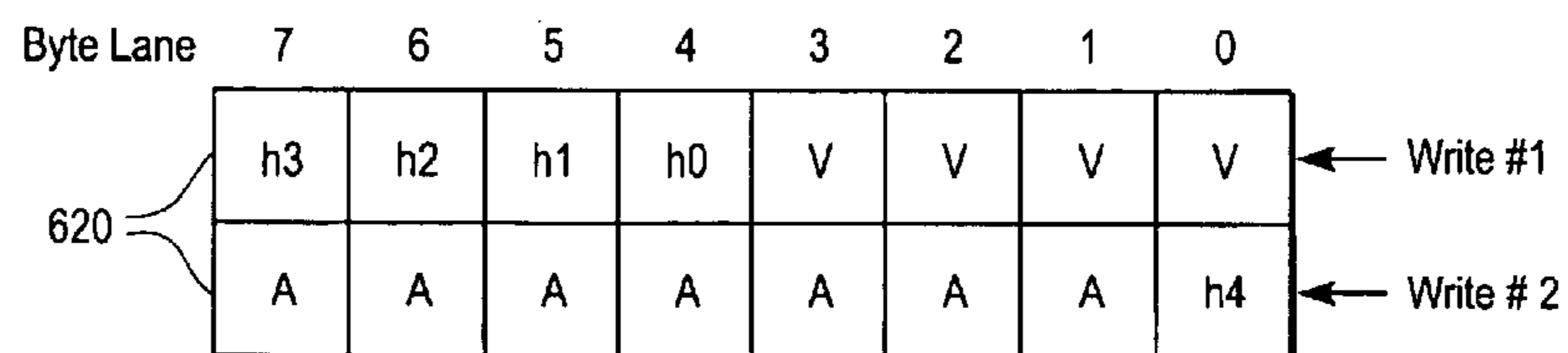
FIG. 5C Cell Buffer after Host Read
