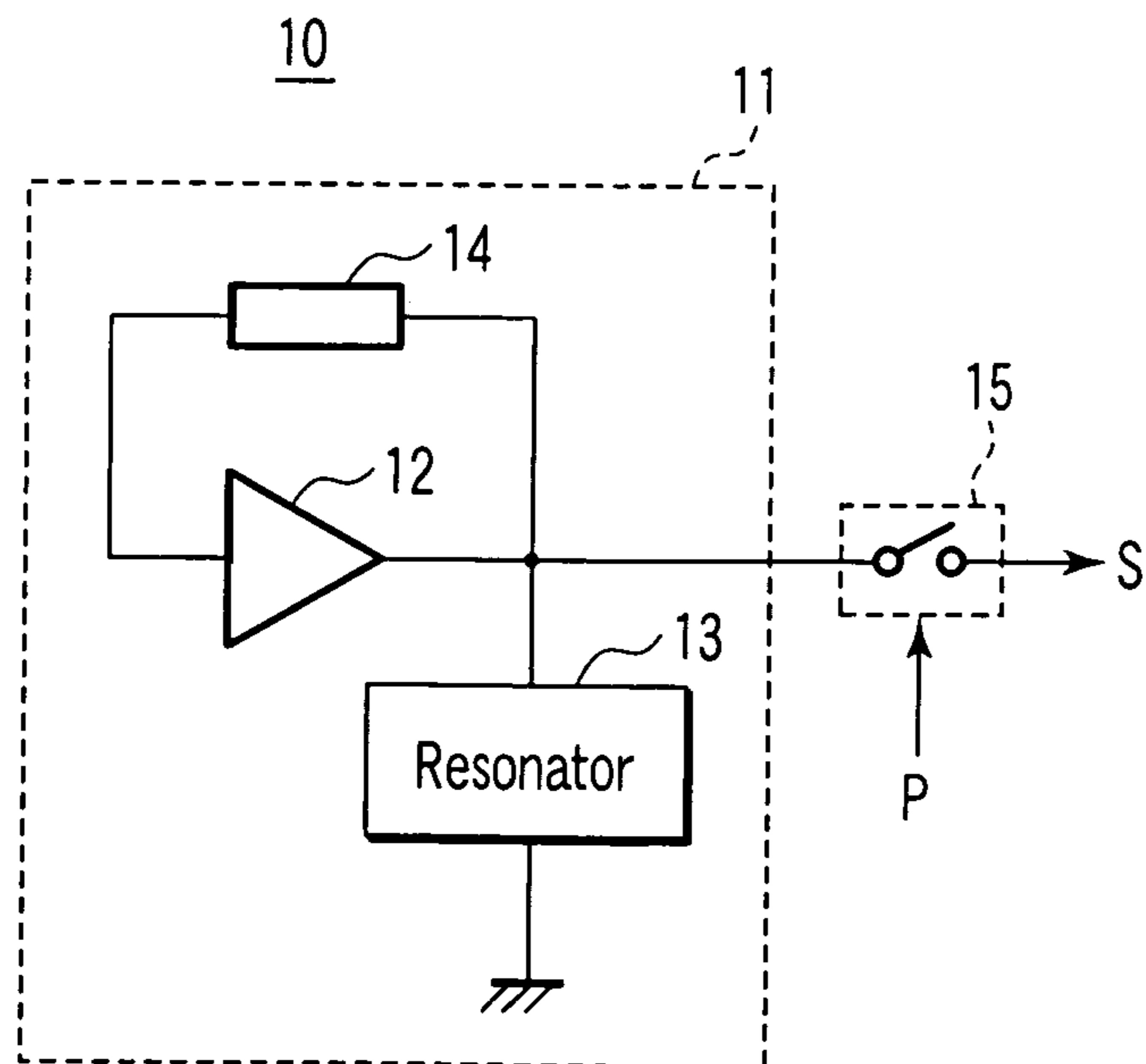
FIG. 11 (PRIOR ART)
