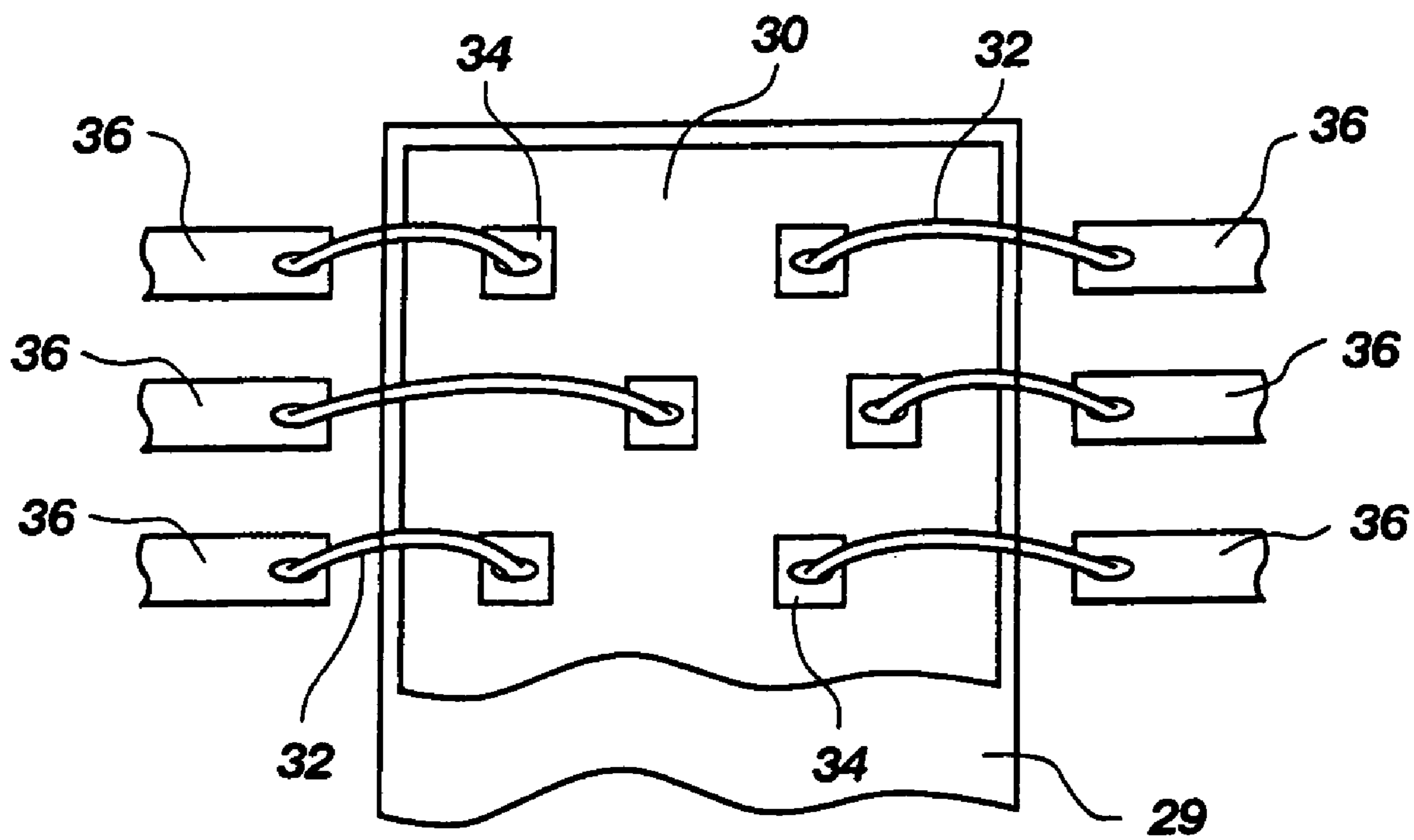
Fig. 6 (PRIOR ART)
