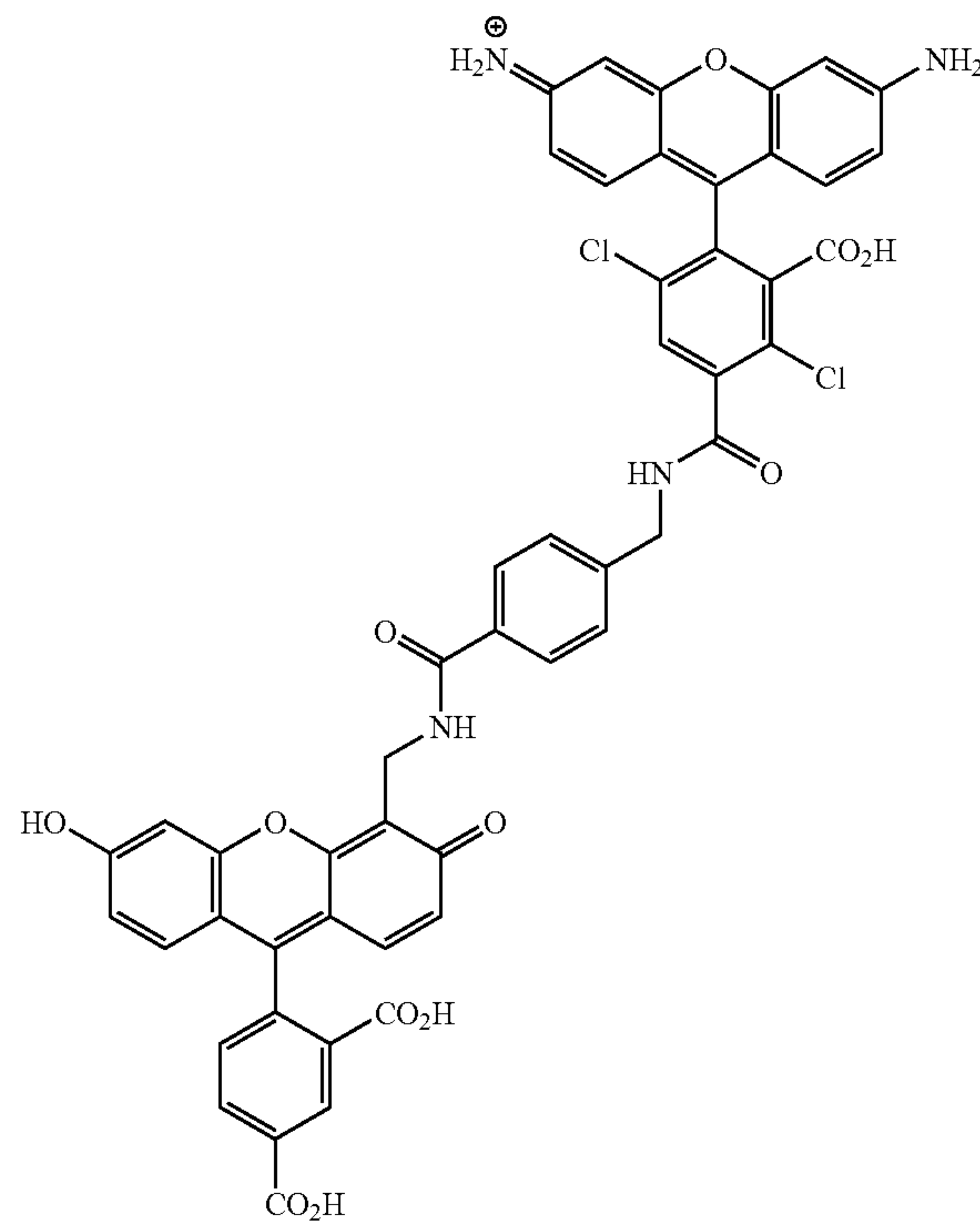
5-CFB-DR110-2
