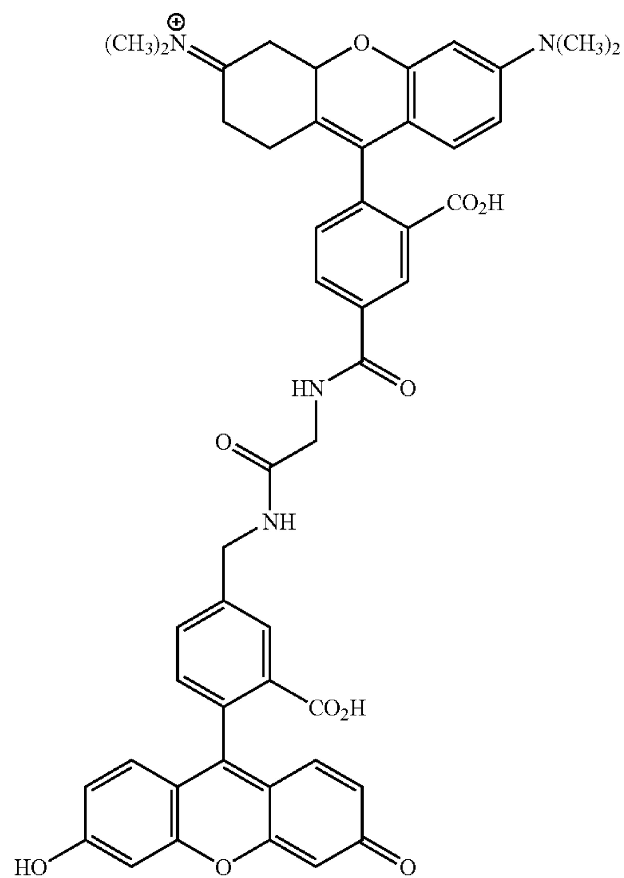
5TMR-gly-5AMF
