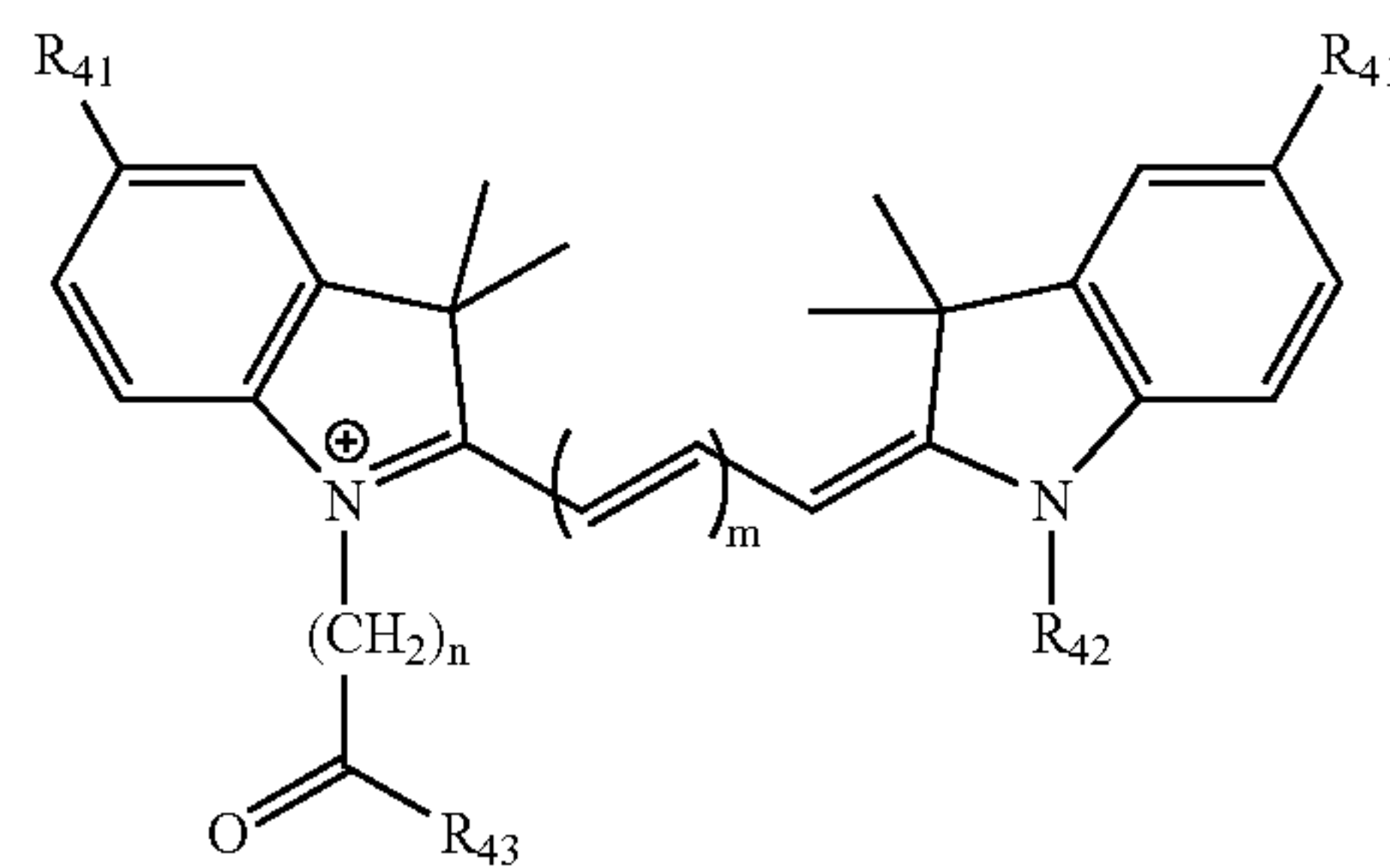
CYANINE
