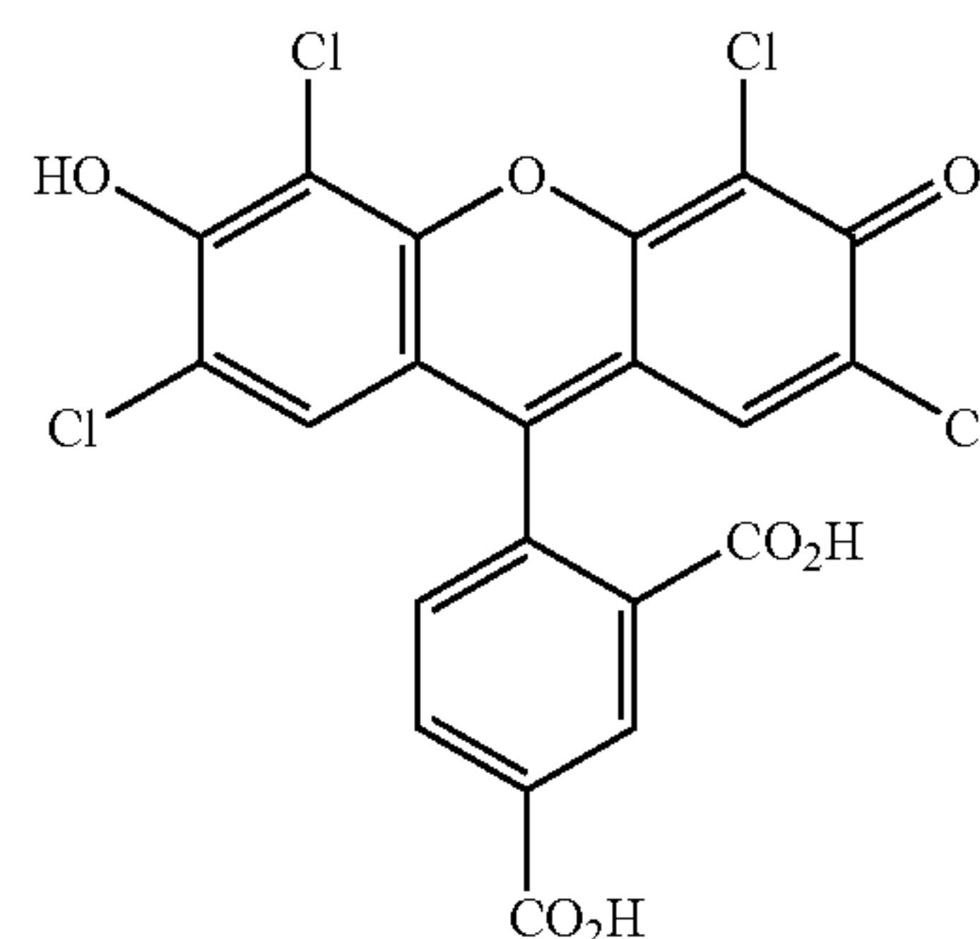
ZOE
