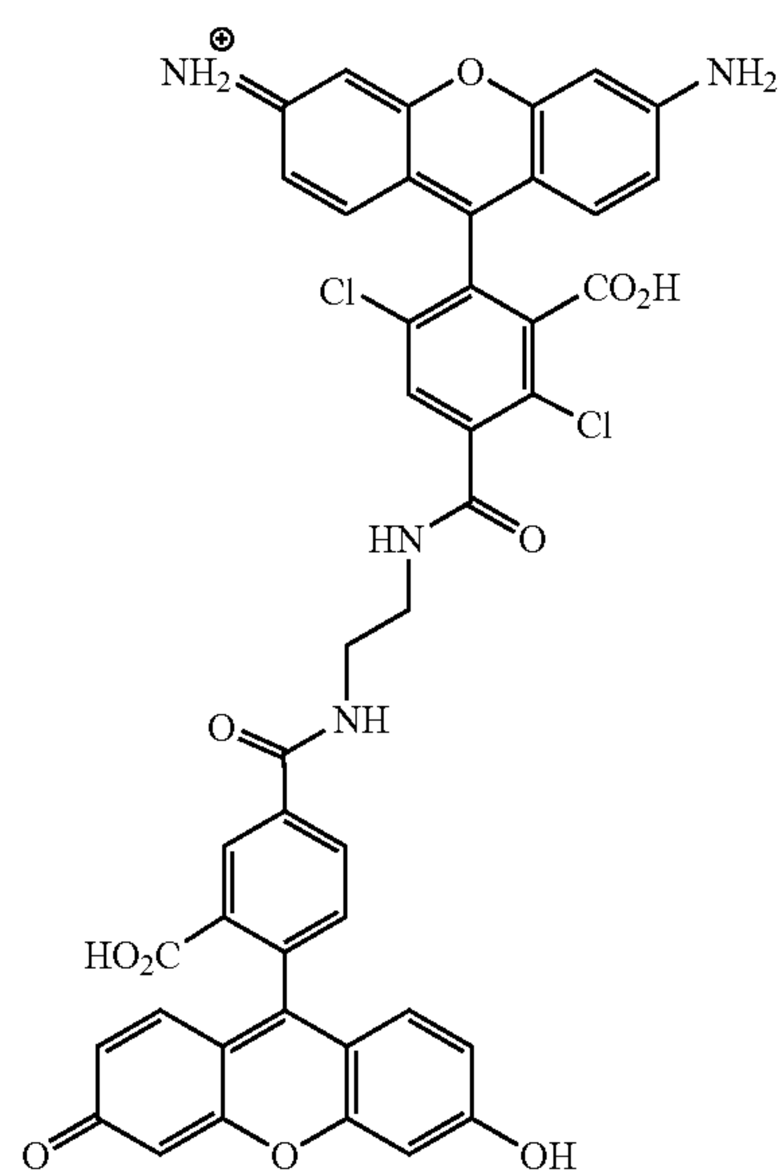
5TMR-5AMF
