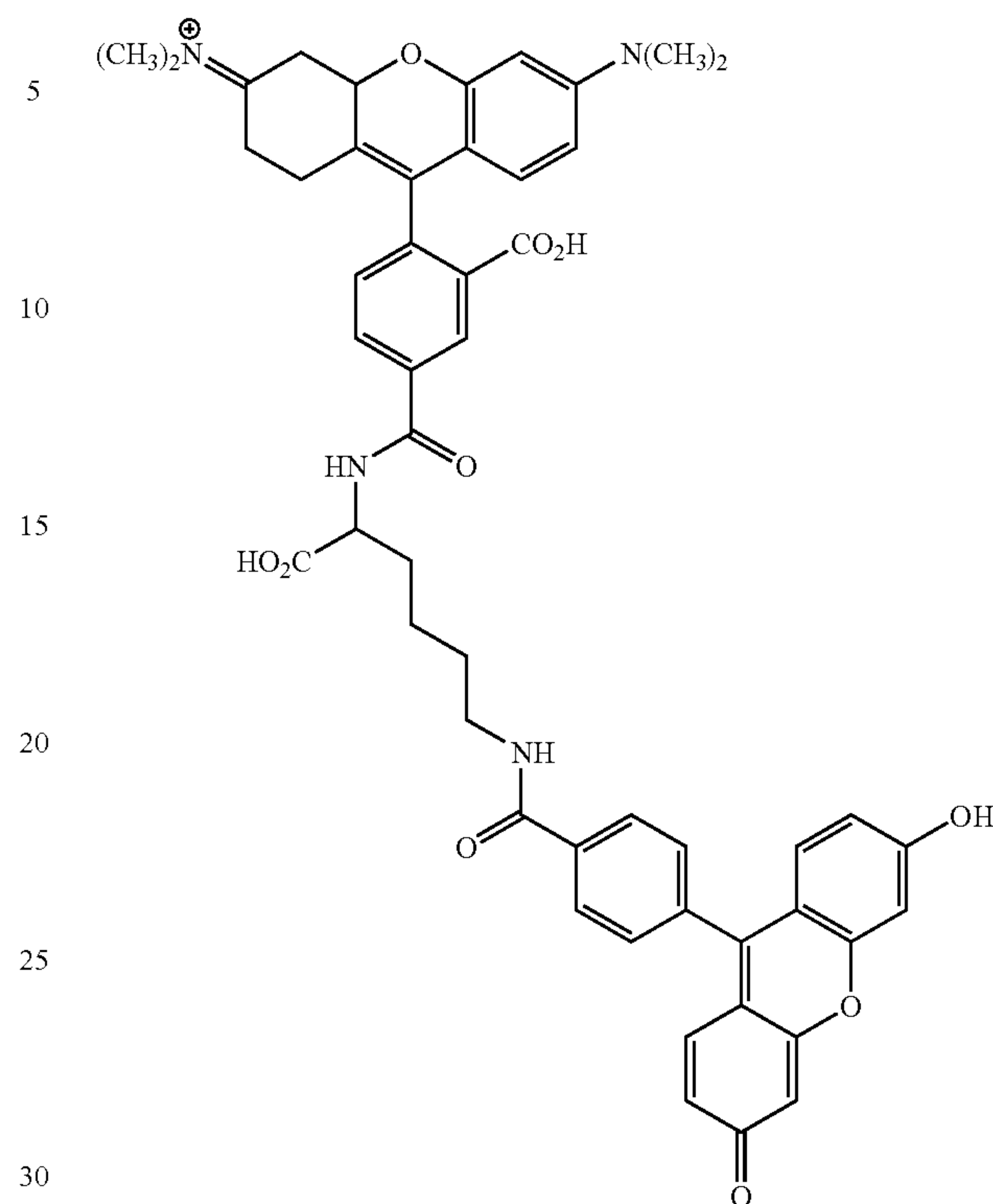
5TMR-lys-5FAM
