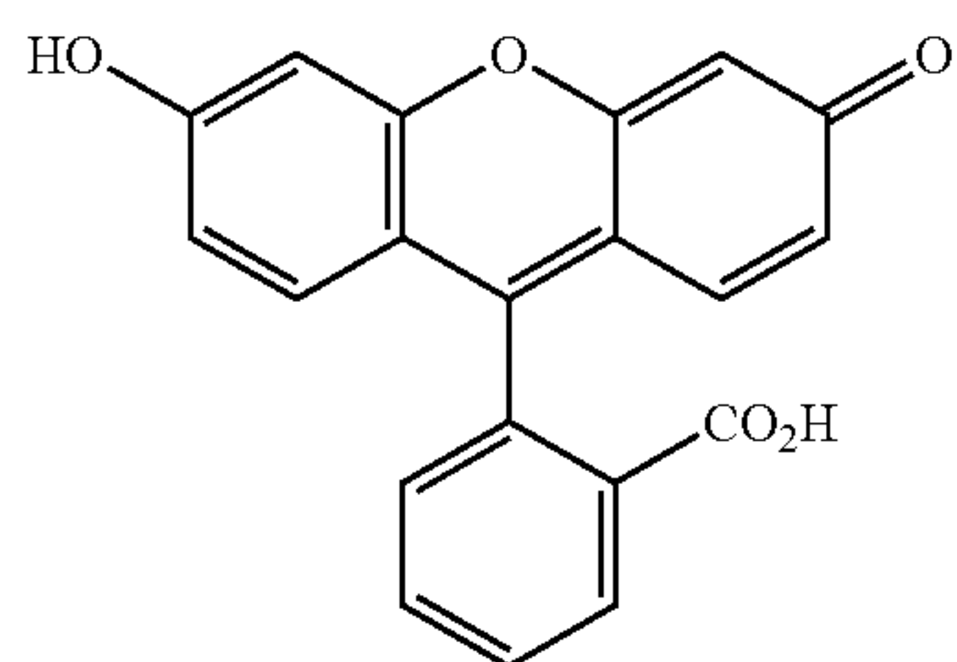
Fluorescein
