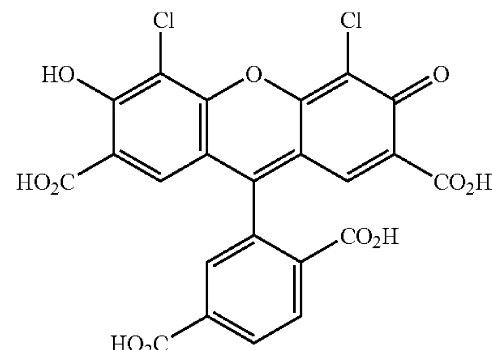
JOE
