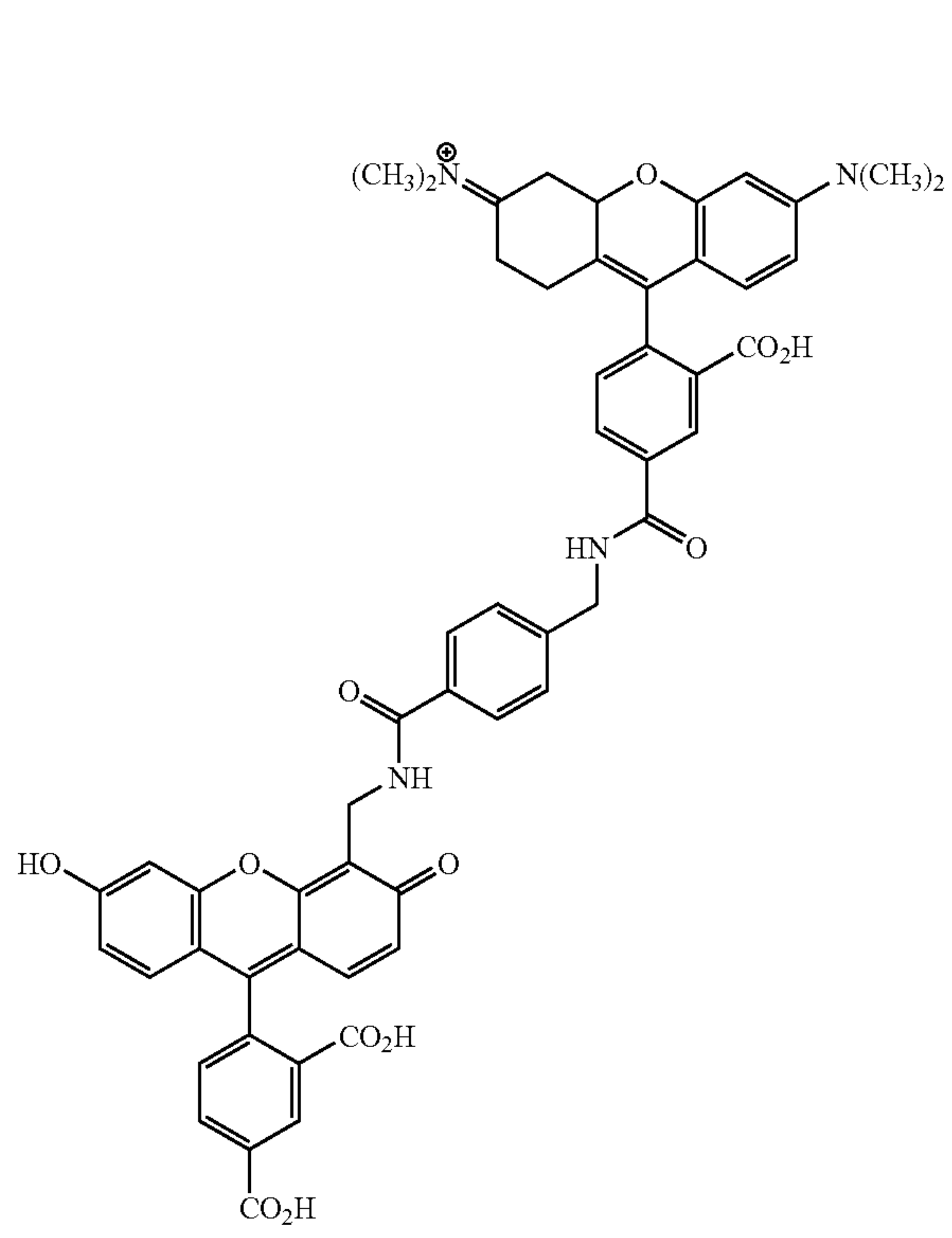
5-TMR-B-CF
