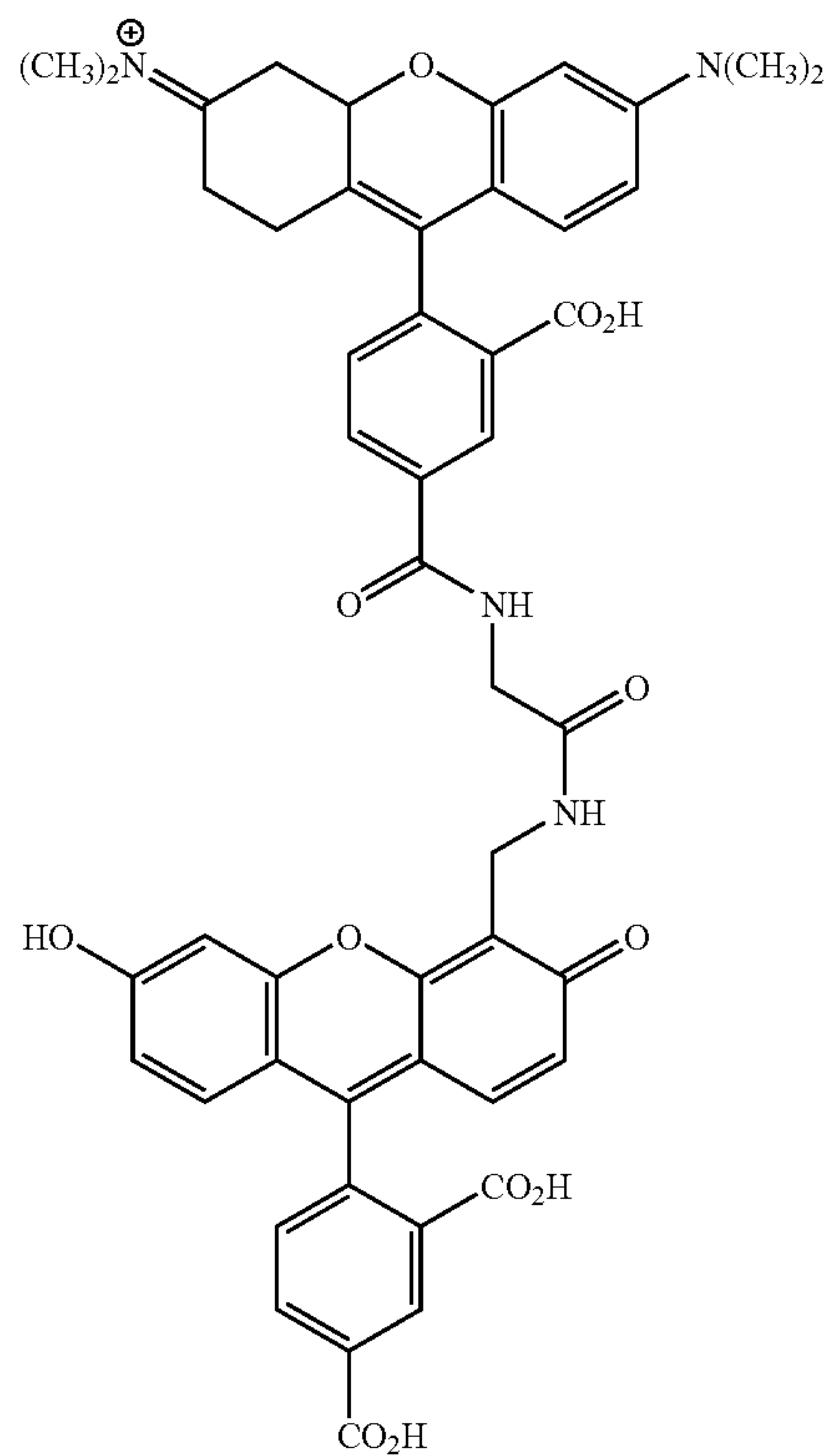
5TMR-gly-CF
