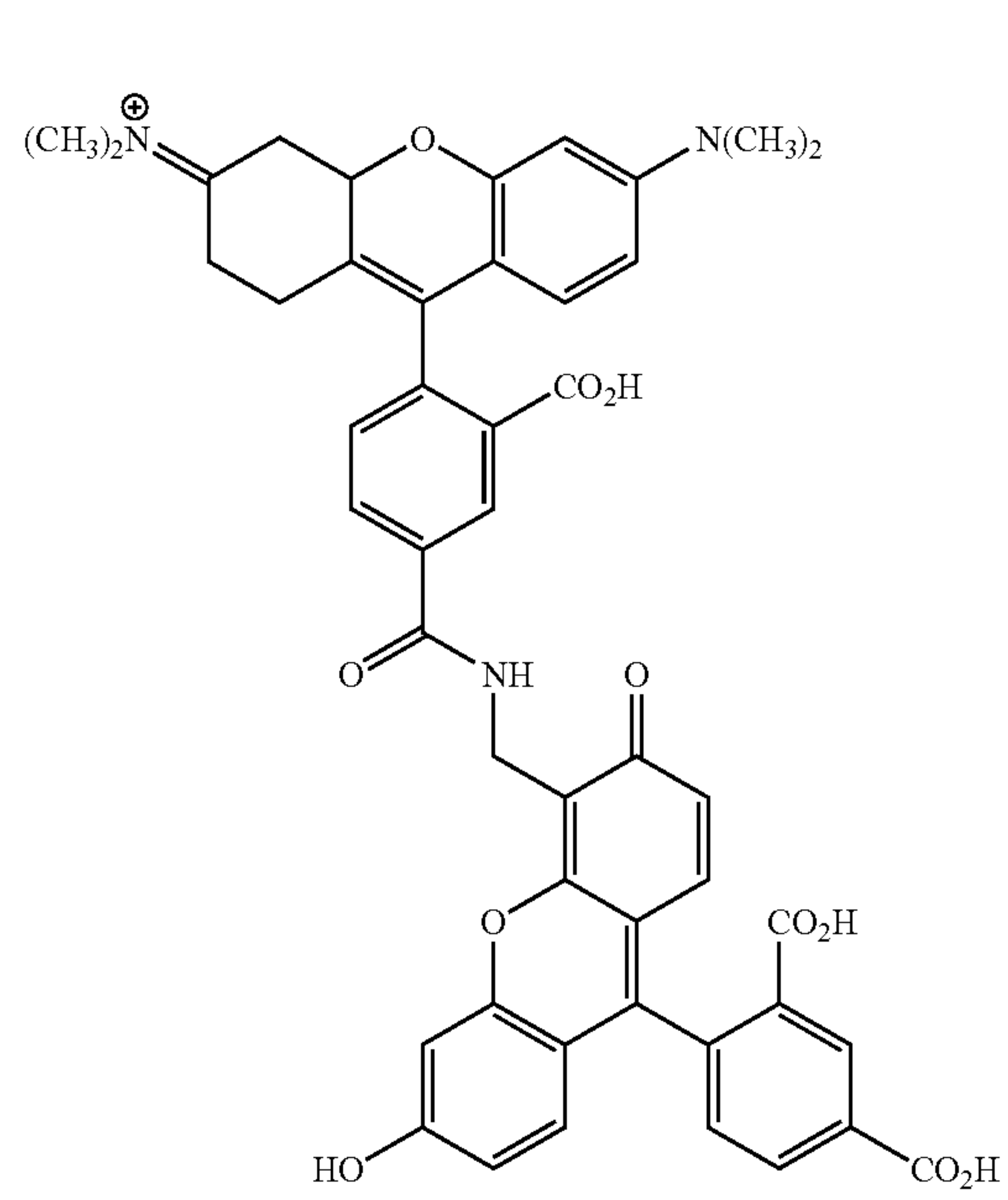
5TMR-CF
