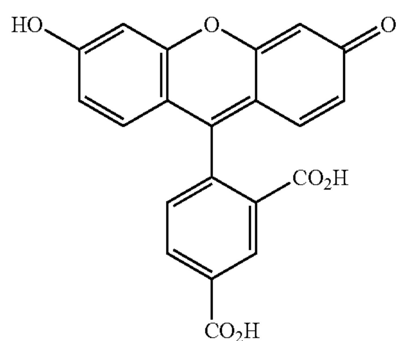
5-carboxyfluorescein
