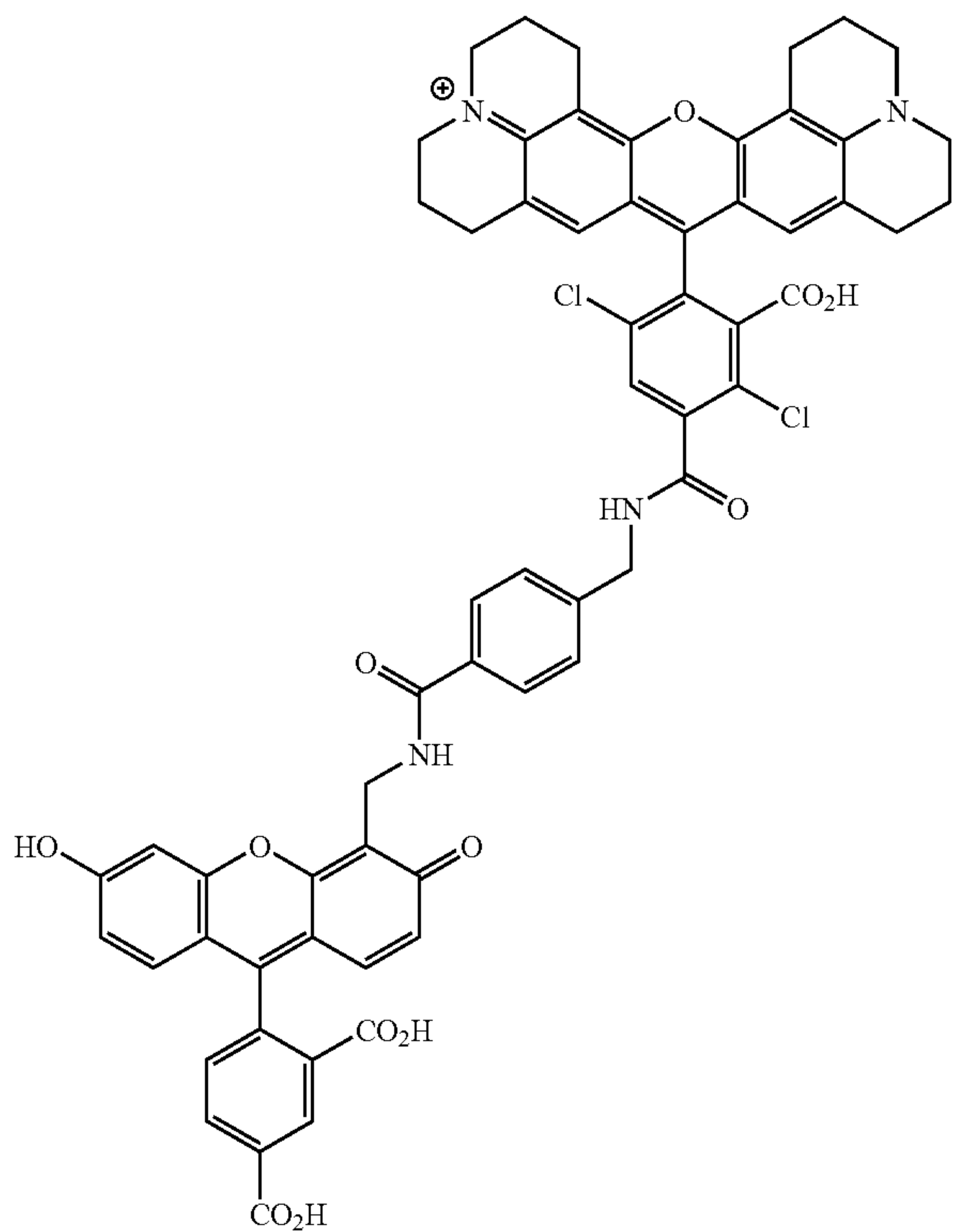
5-CFB-DROX-2
