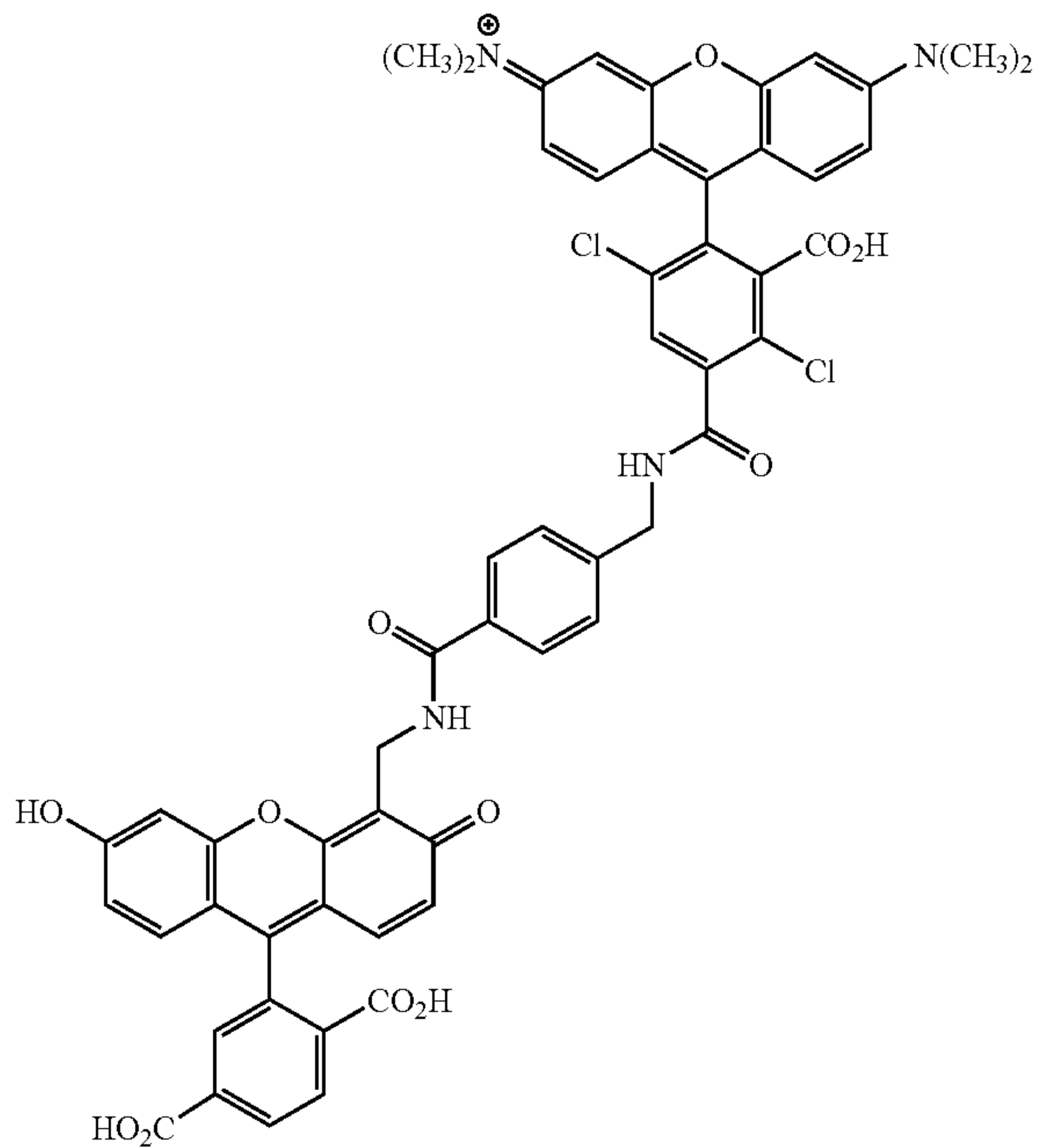
6-CFB-DTMR-2
