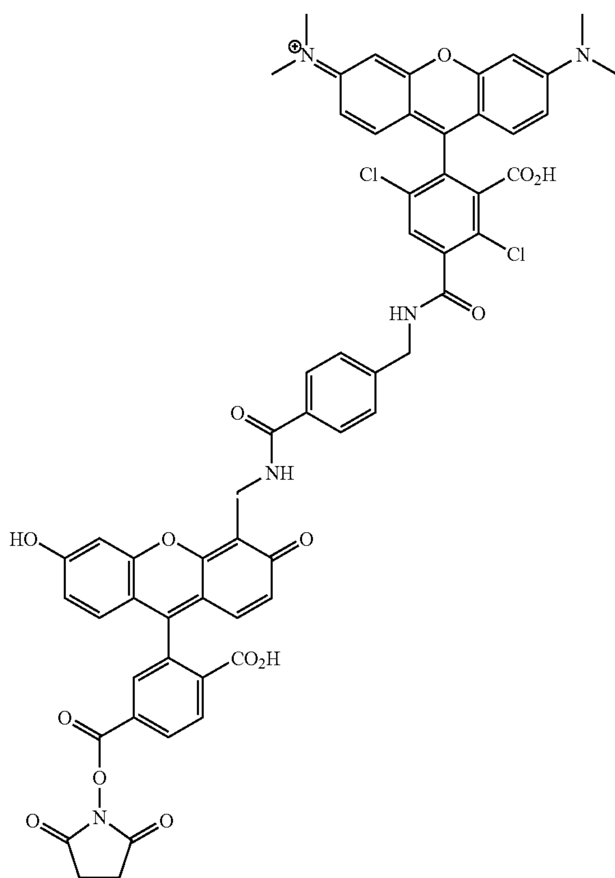
6-CFB-DTMR-2-NHS
