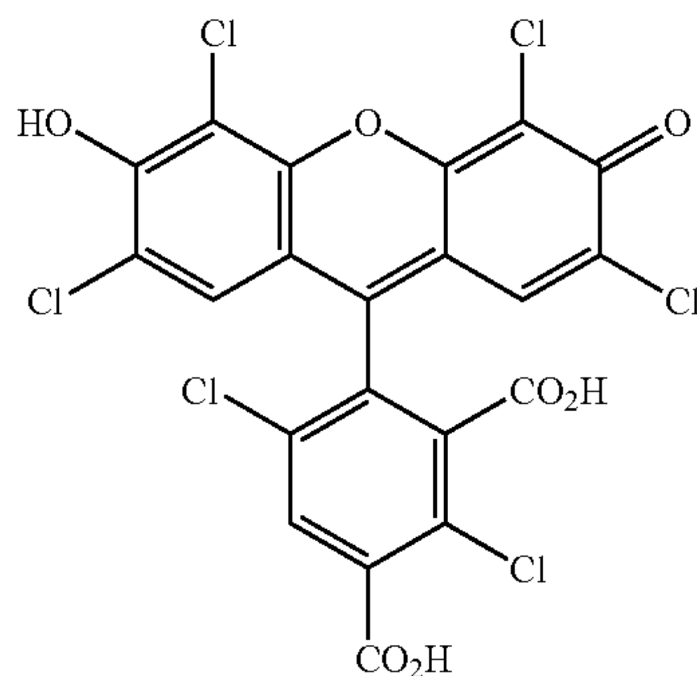
5-carboxy-HEX
