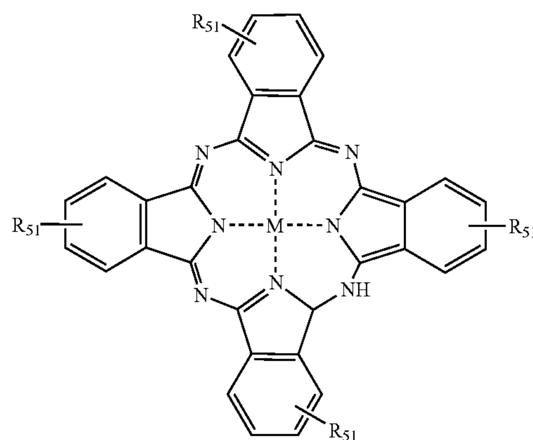
PHthalOCYANINE
