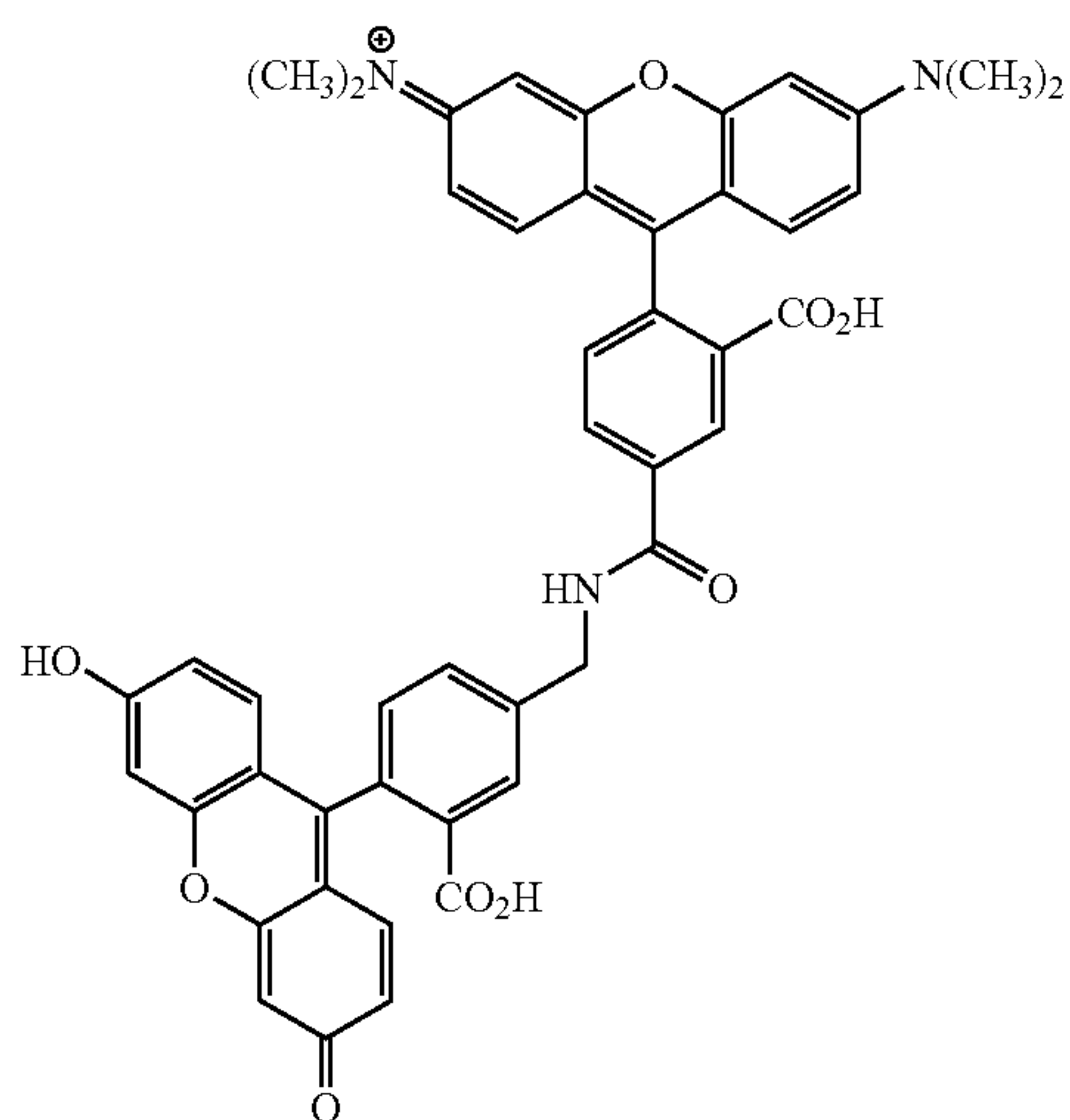
5TMR-5AMF
