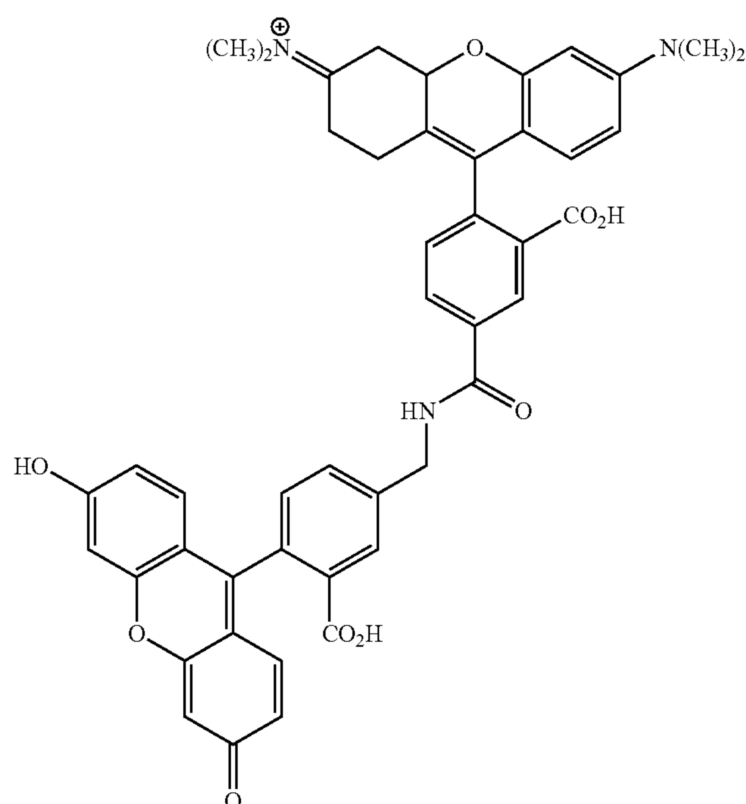
5TMR-5AMF
